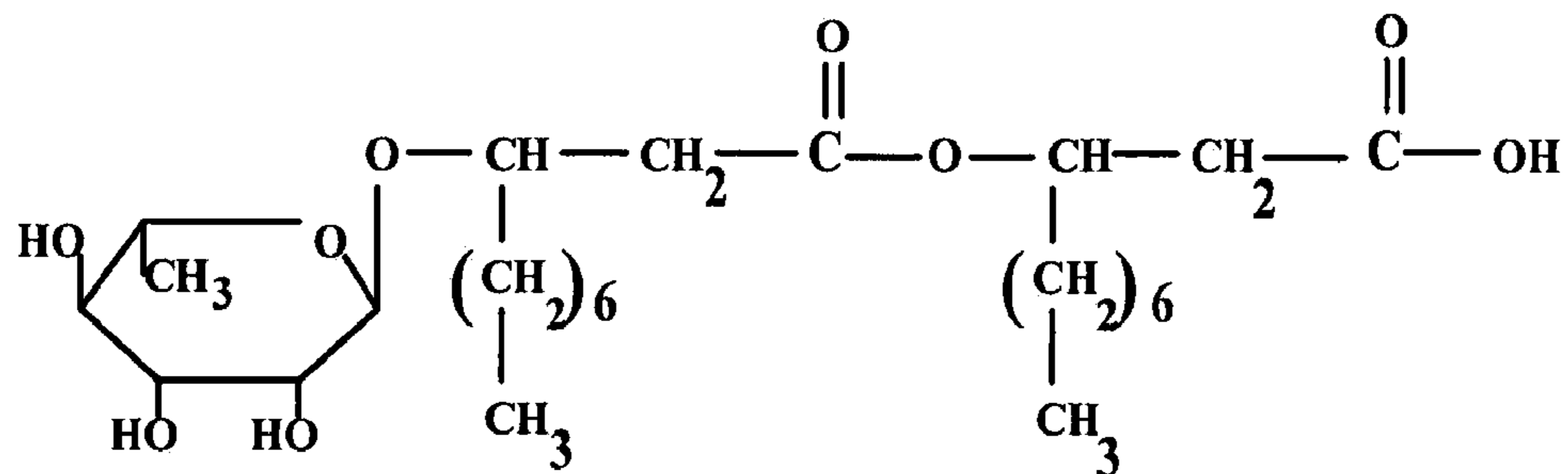
R1 -- \alpha -L-RHAMNOPYRANOSYL - \beta -HYDROXYDECANOYL - \beta -HYDROXYDECANOATE
