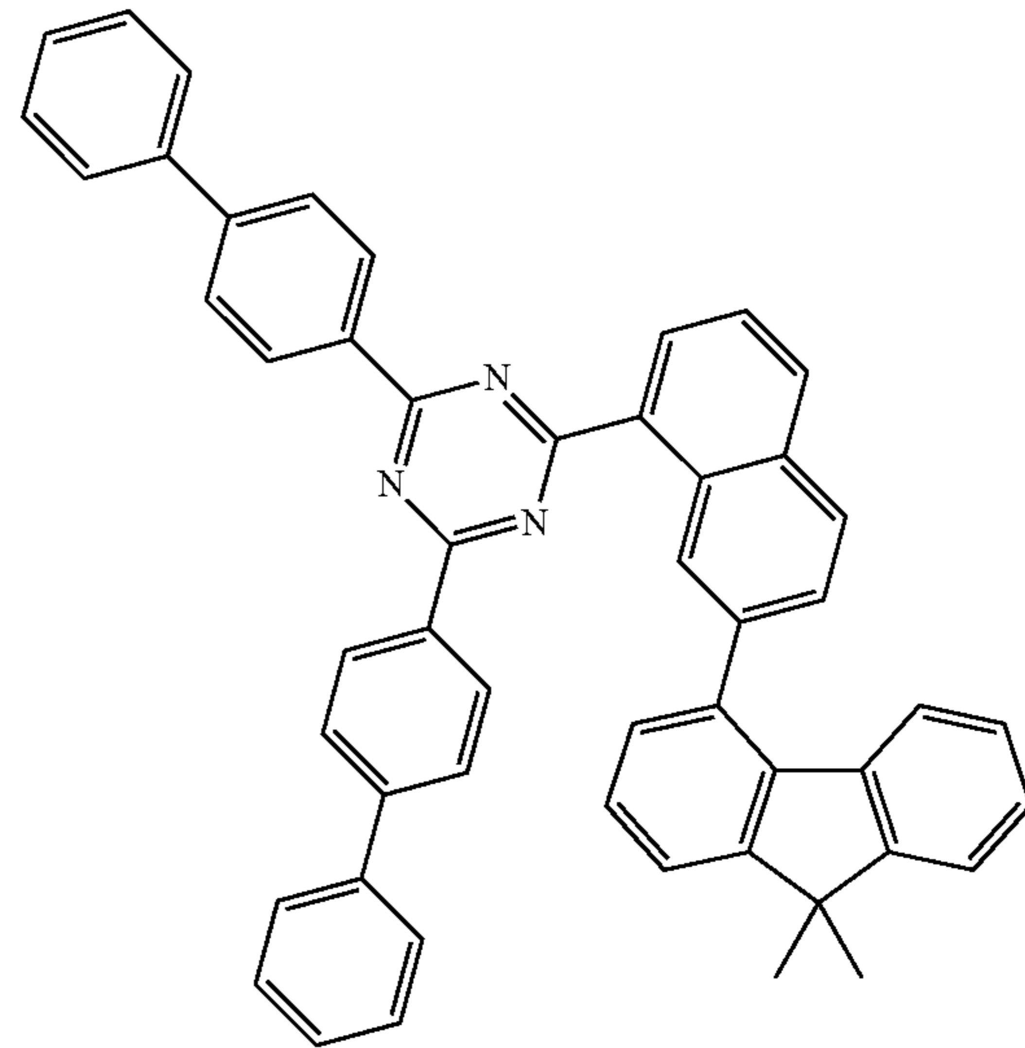
[Compound 32]
