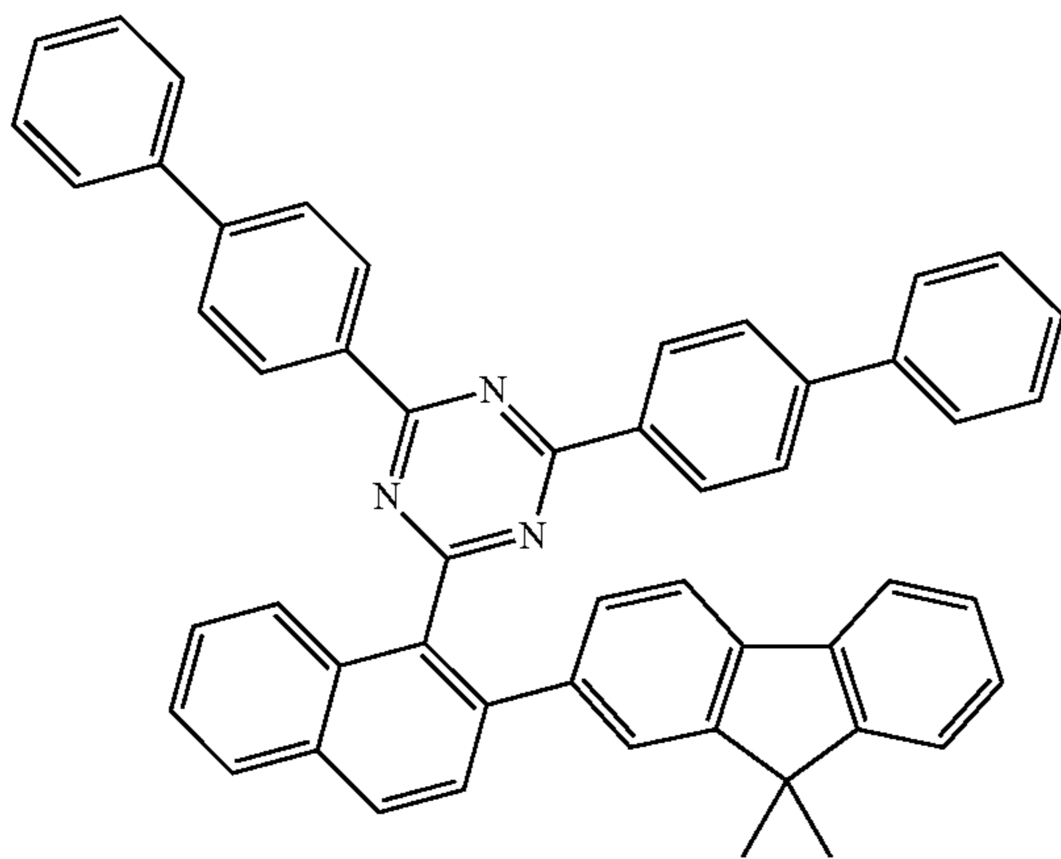
[Compound 23]
