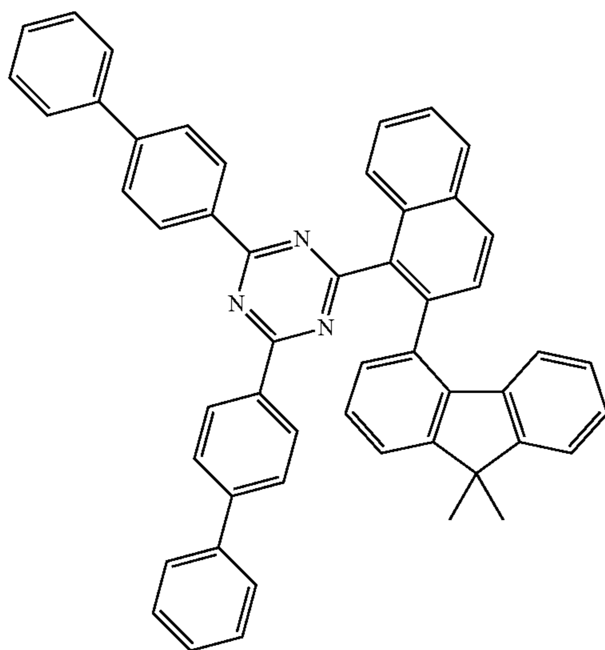
[Compound 24]
