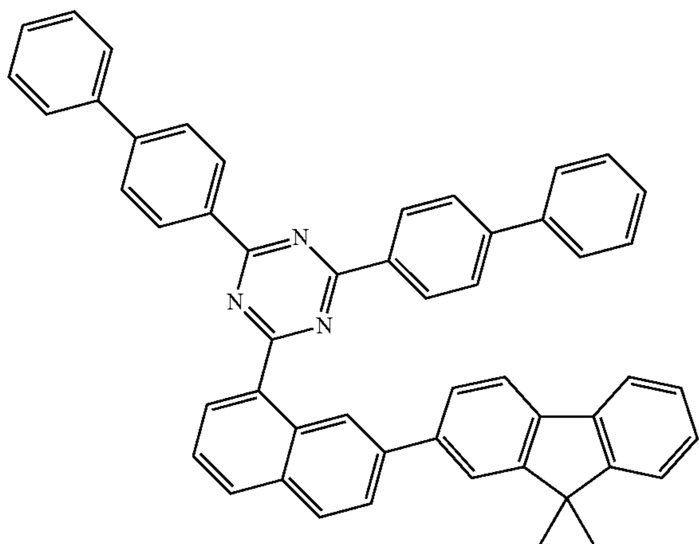
[Compound 31]
