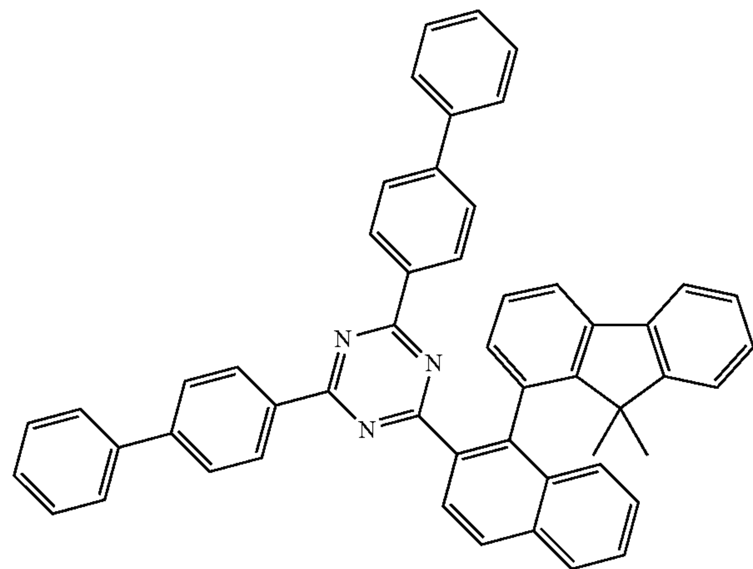
[Compound 213]
