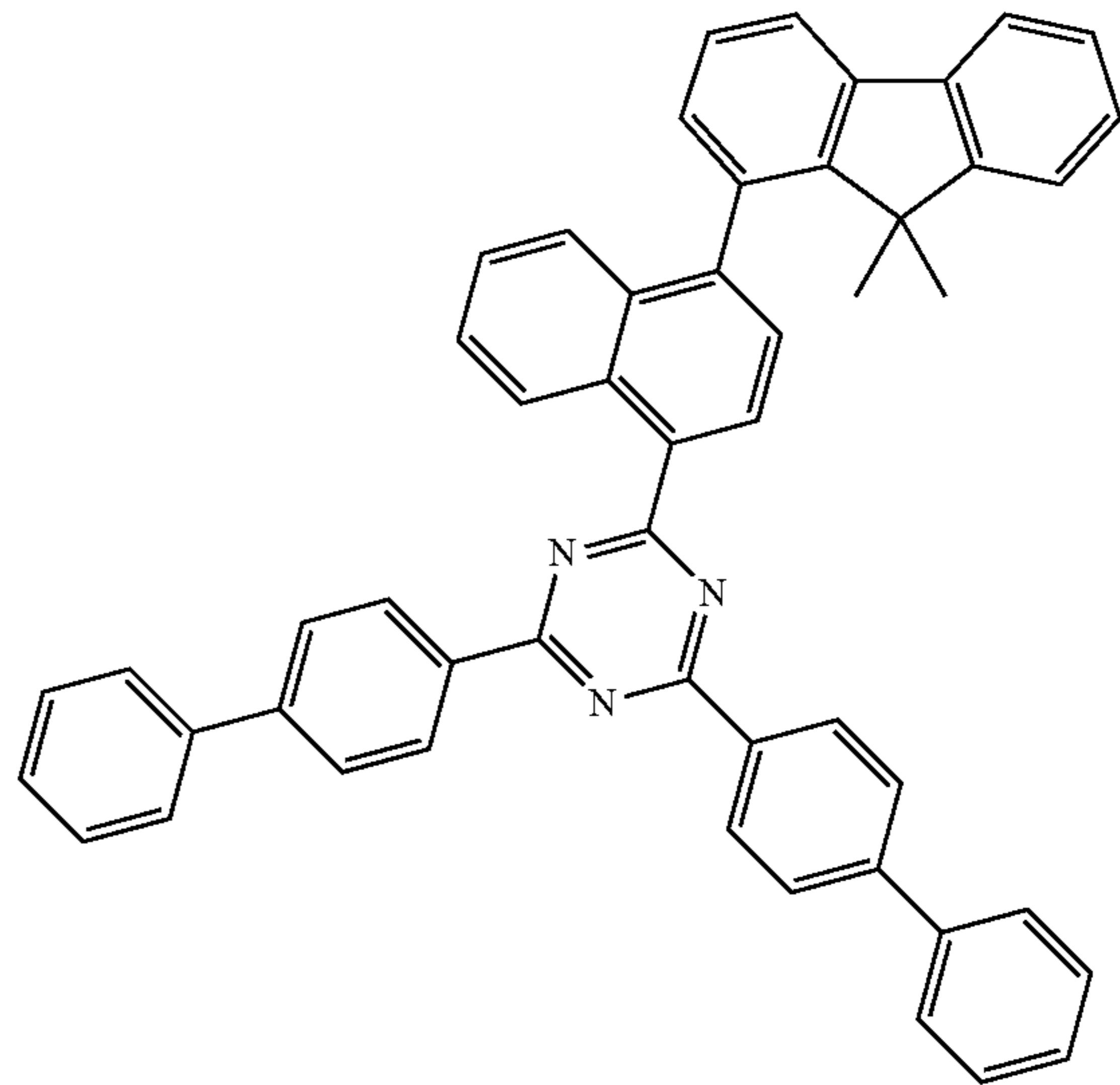
[Compound 37]
