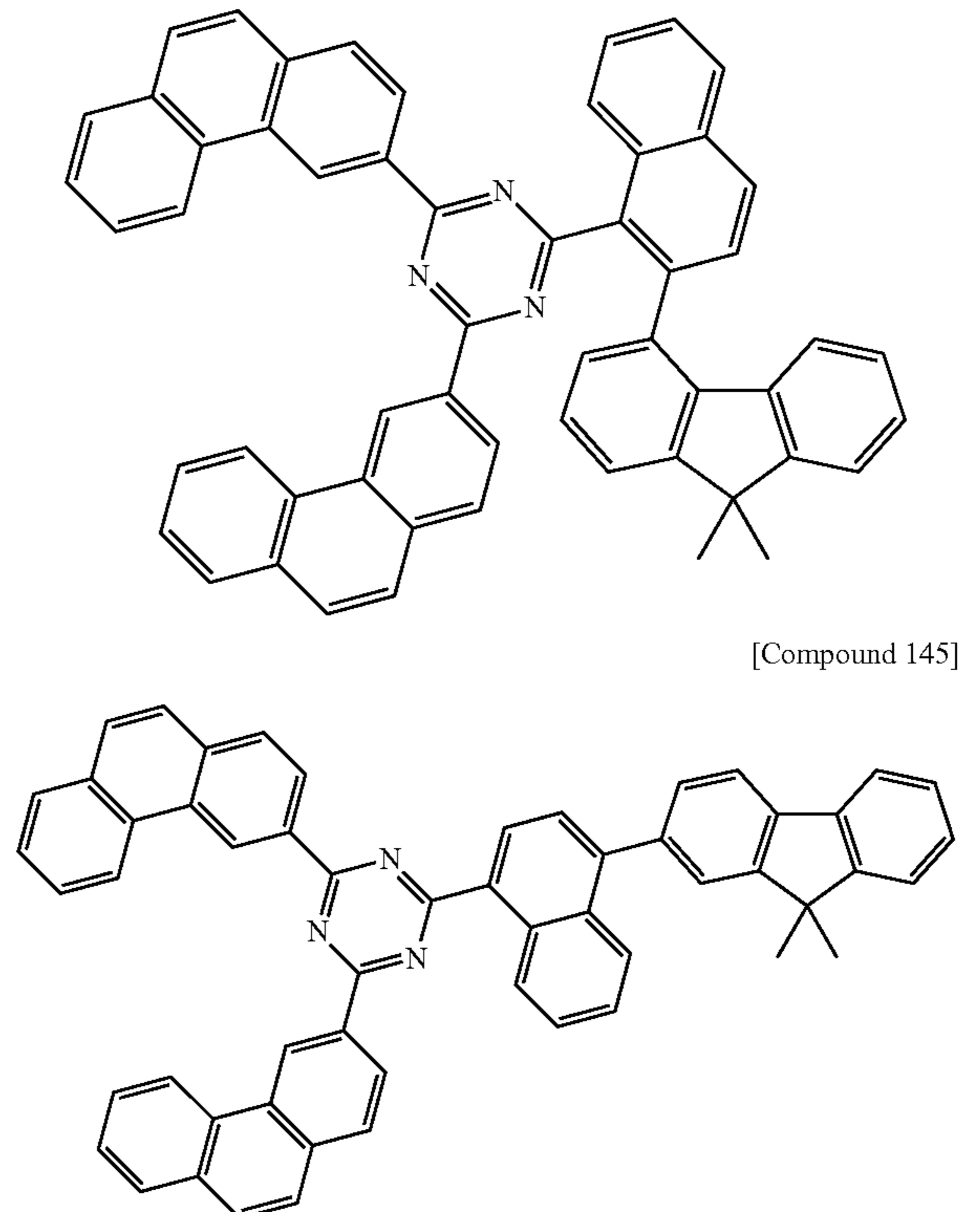
[Compound 144]
