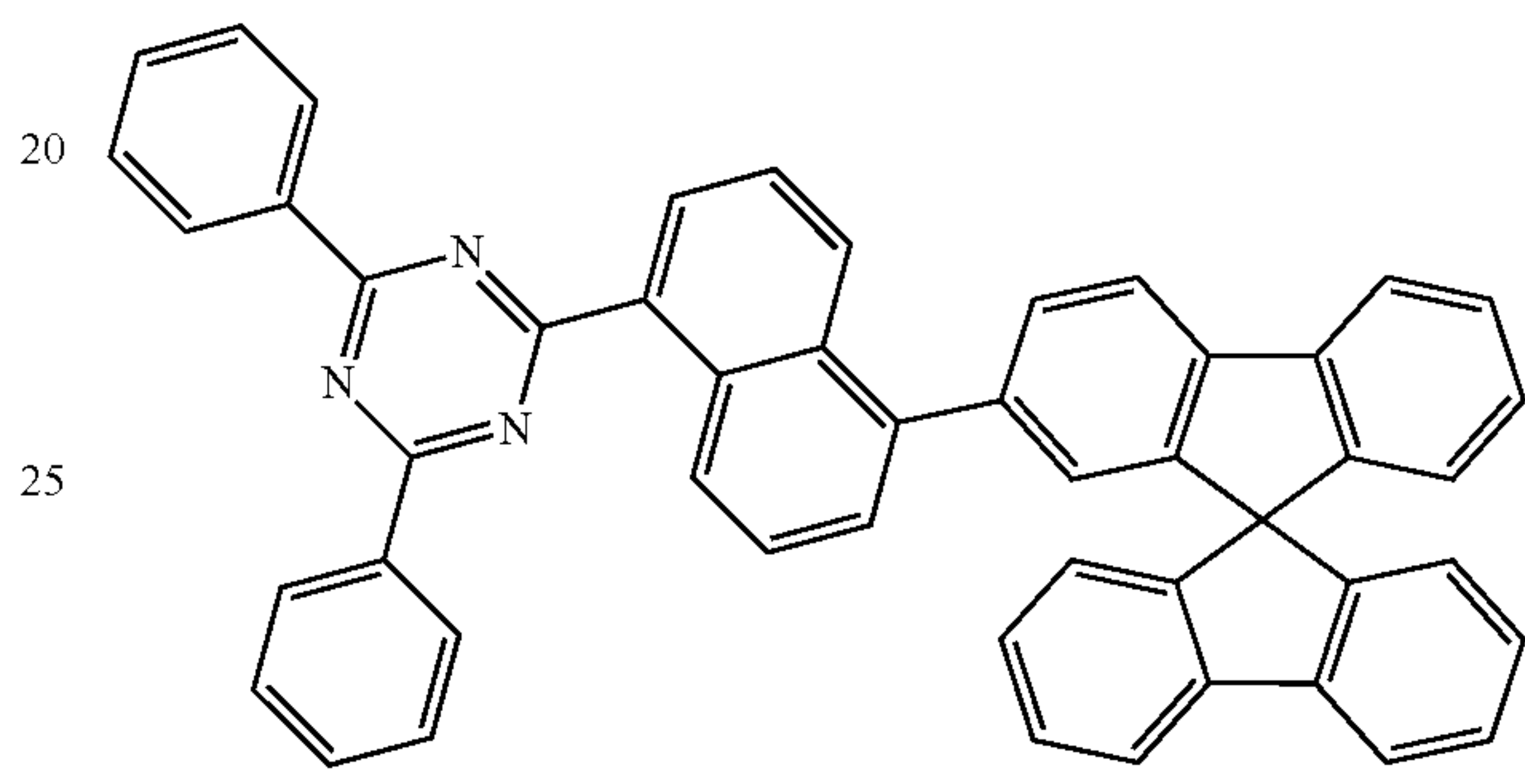
[Compound 8]
