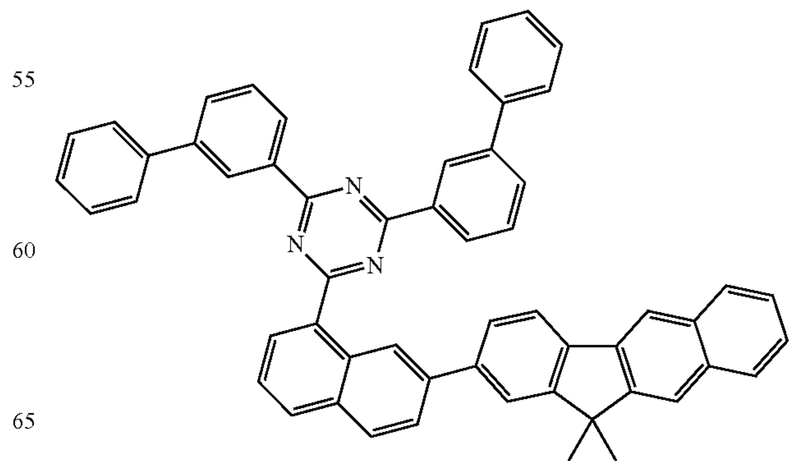
[Compound 245]
