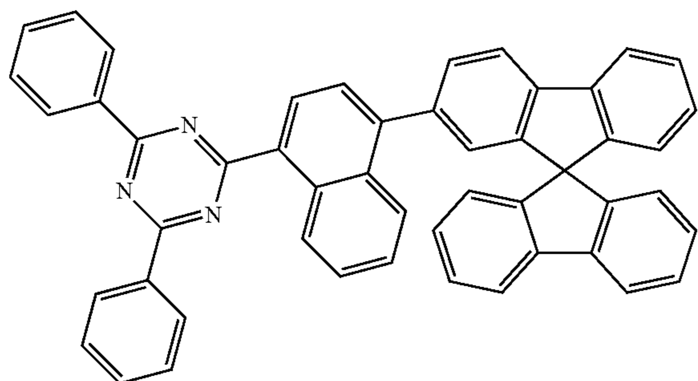
[Compound 6]
