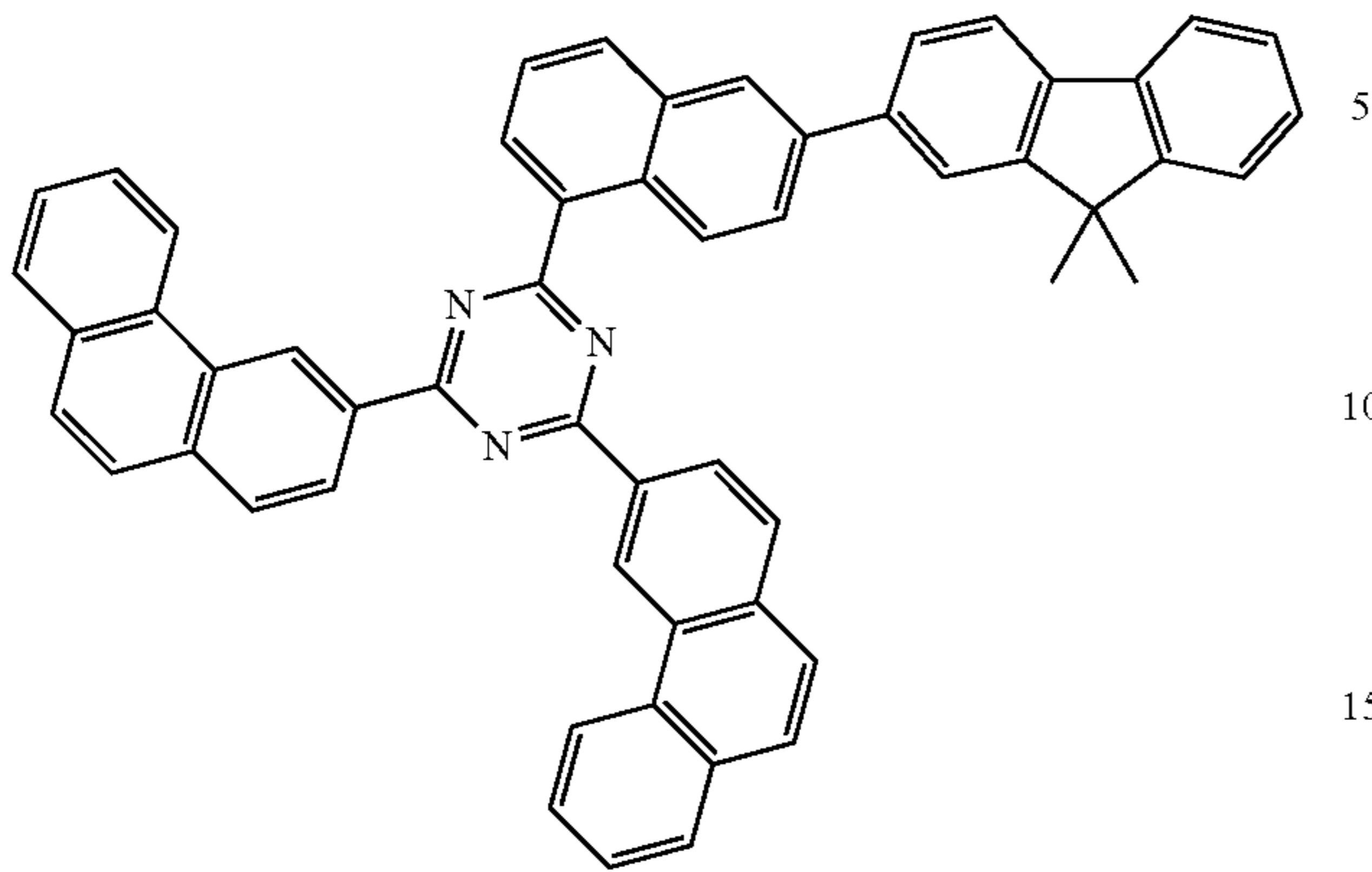
[Compound 150]
