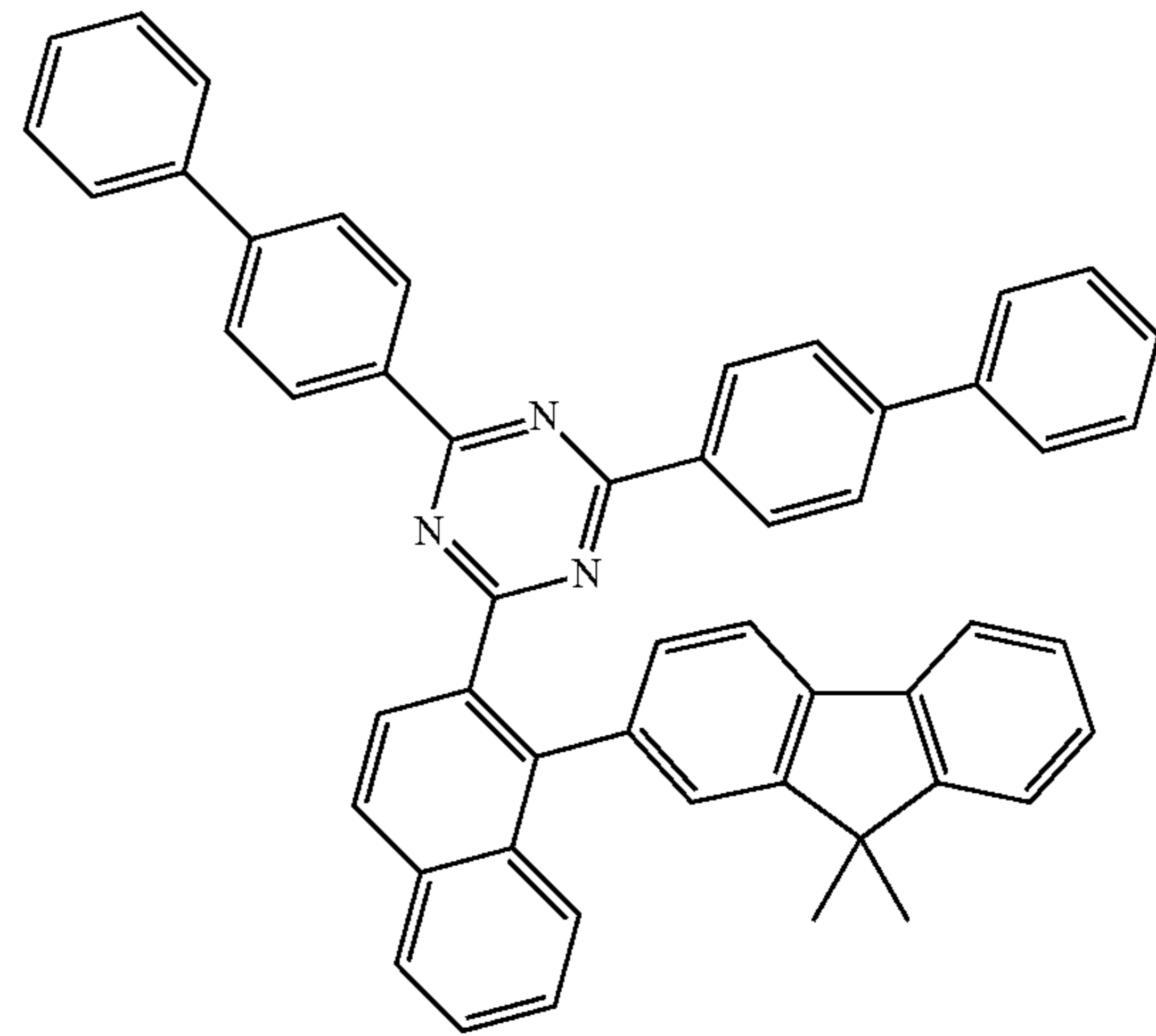
[Compound 211]
