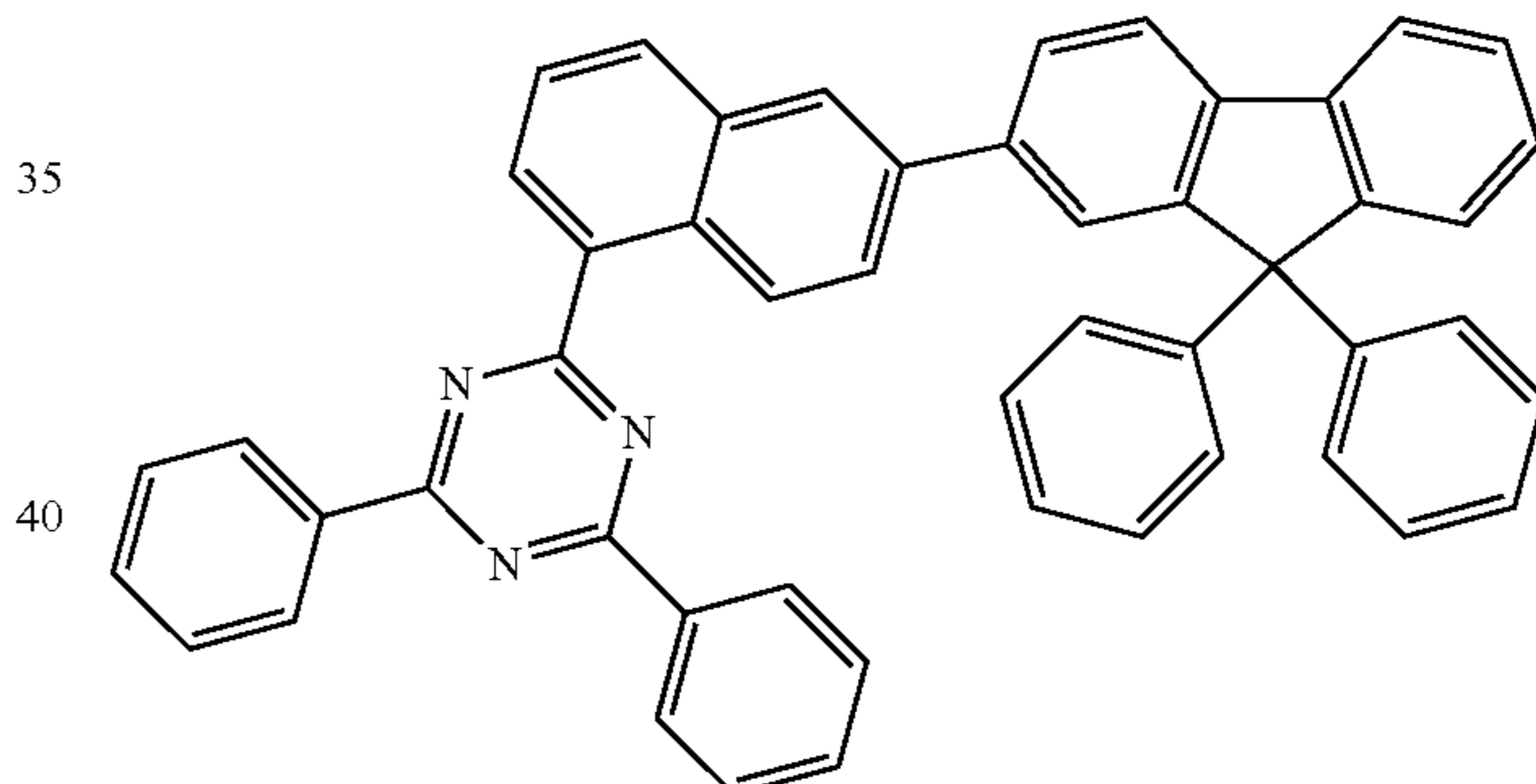
[Compound 9]
