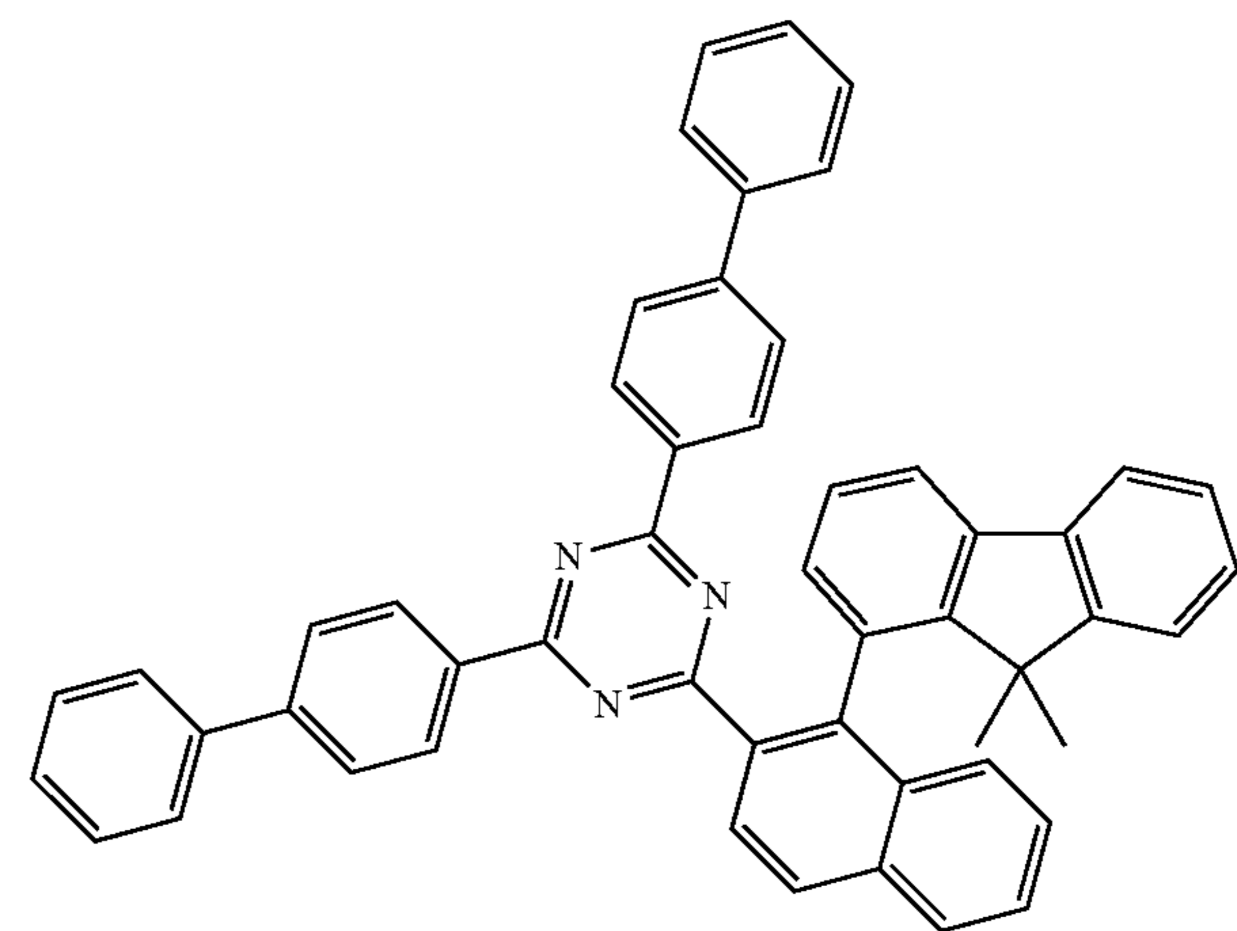
[Compound 213]
