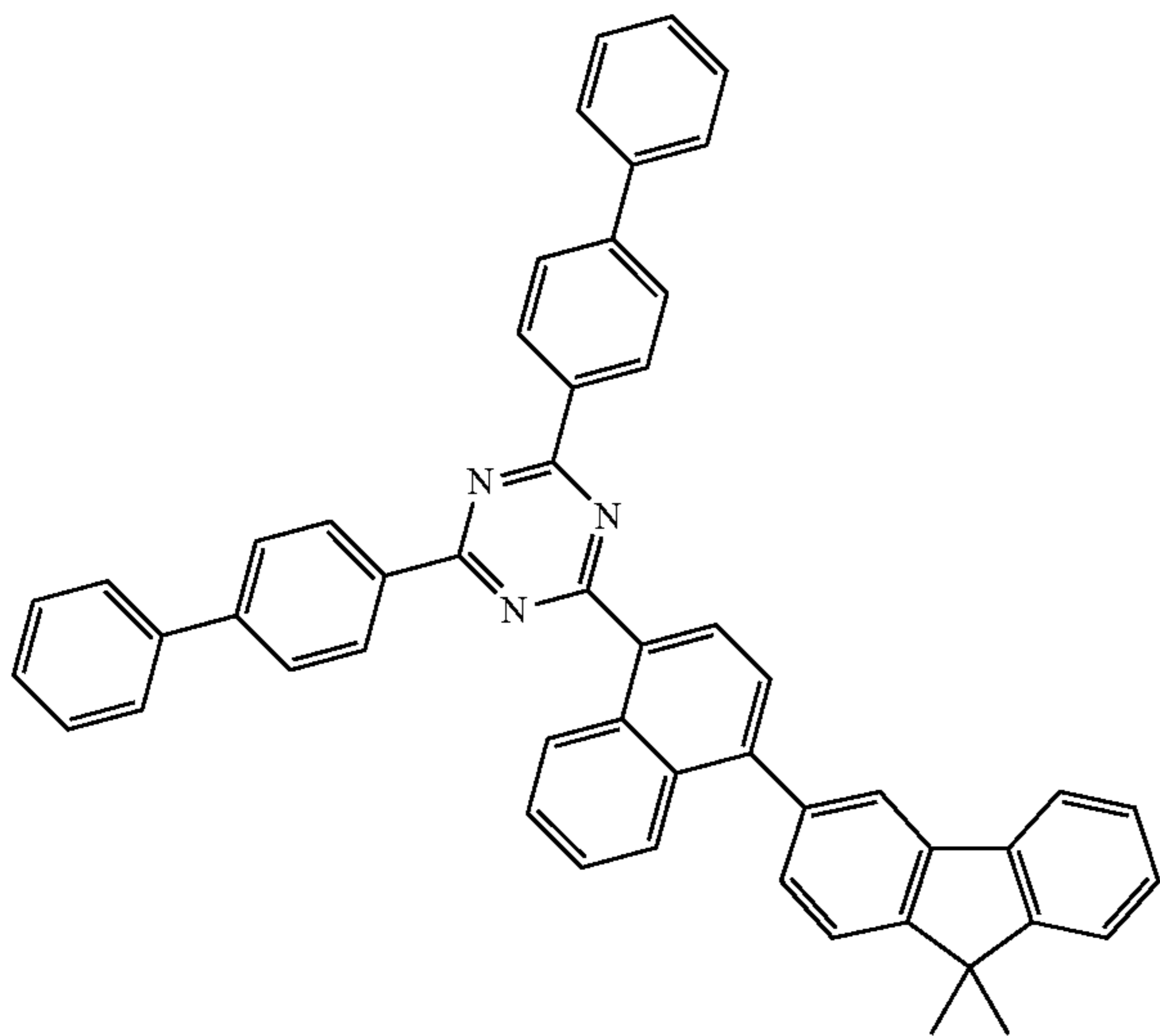
[Compound 36]
