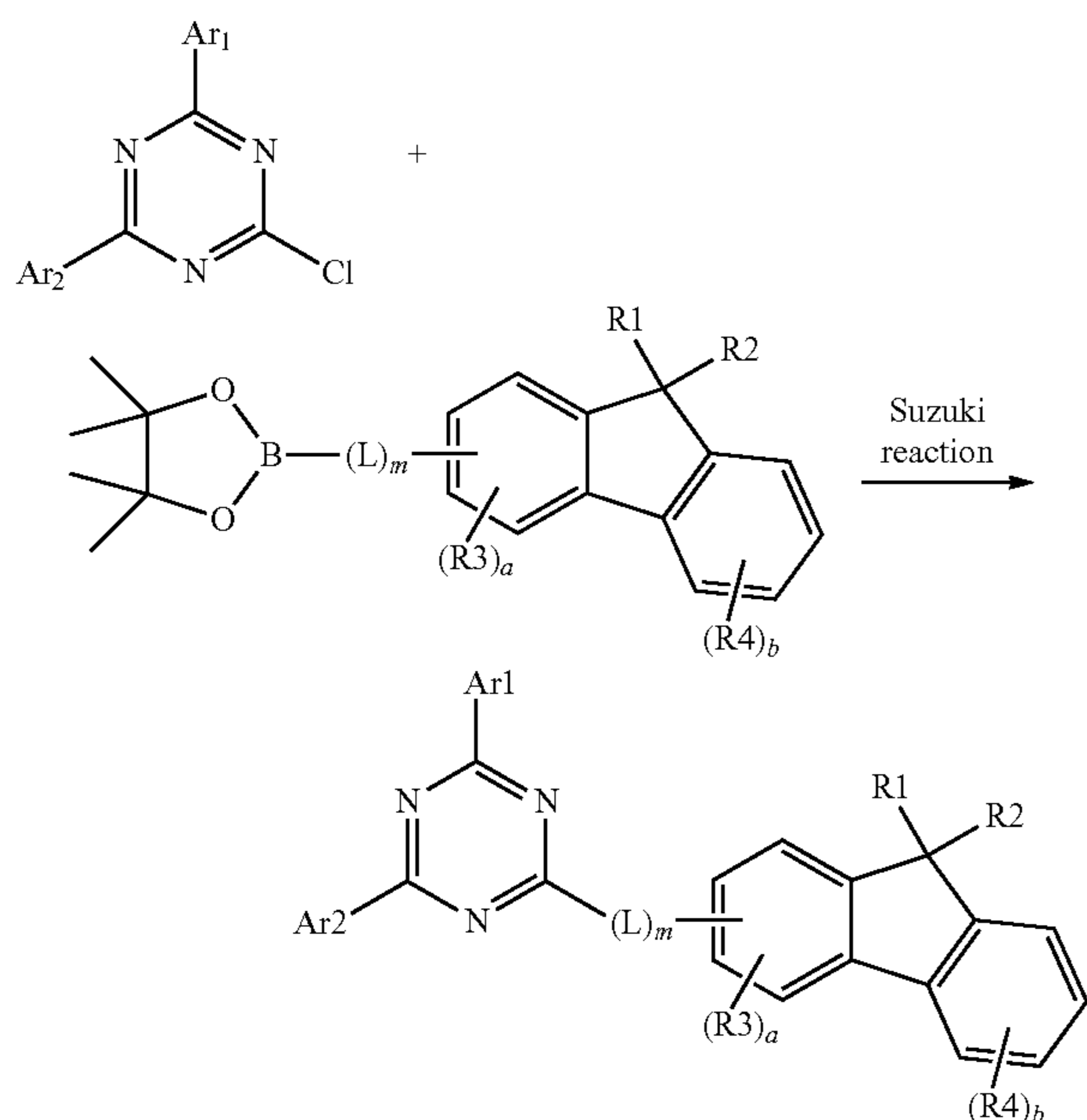
[Reaction Formula 1]
