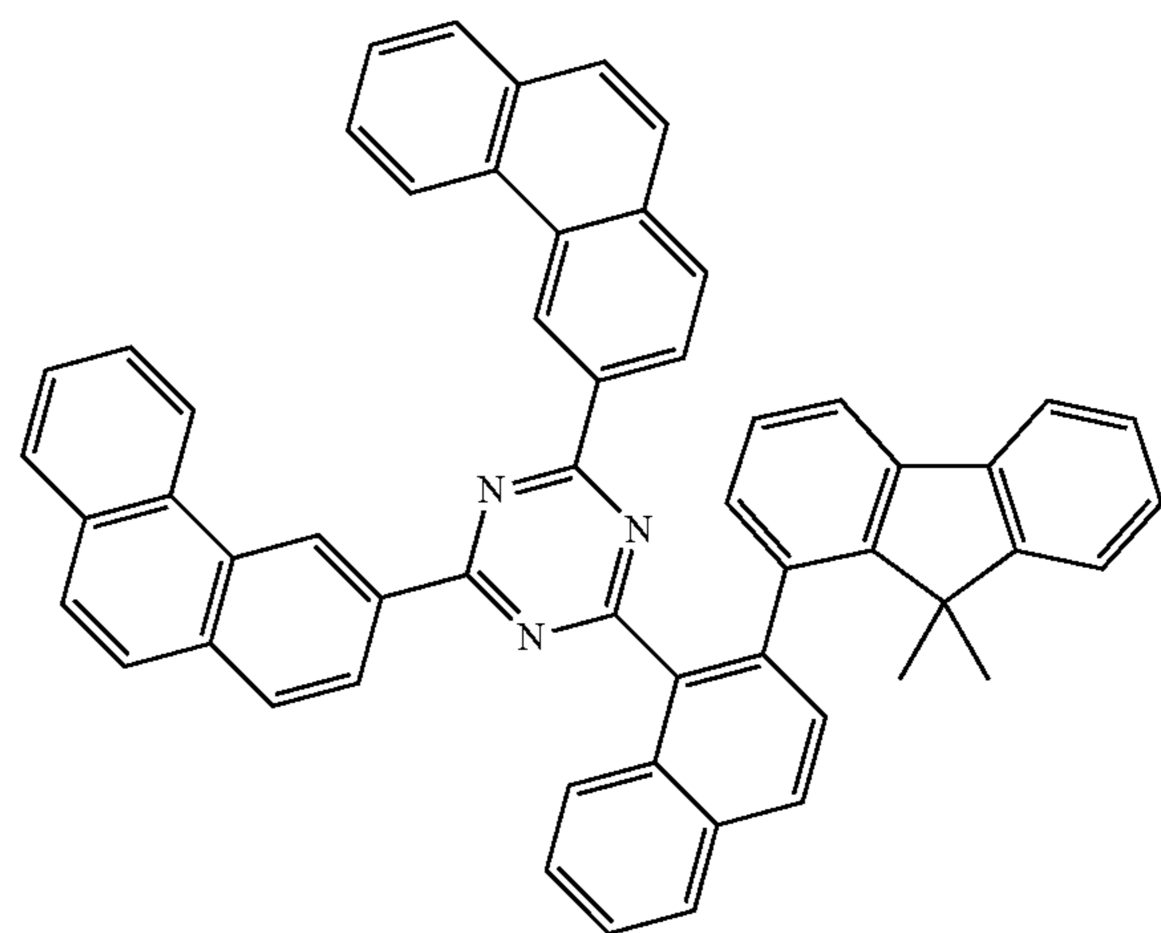
[Compound 153]
