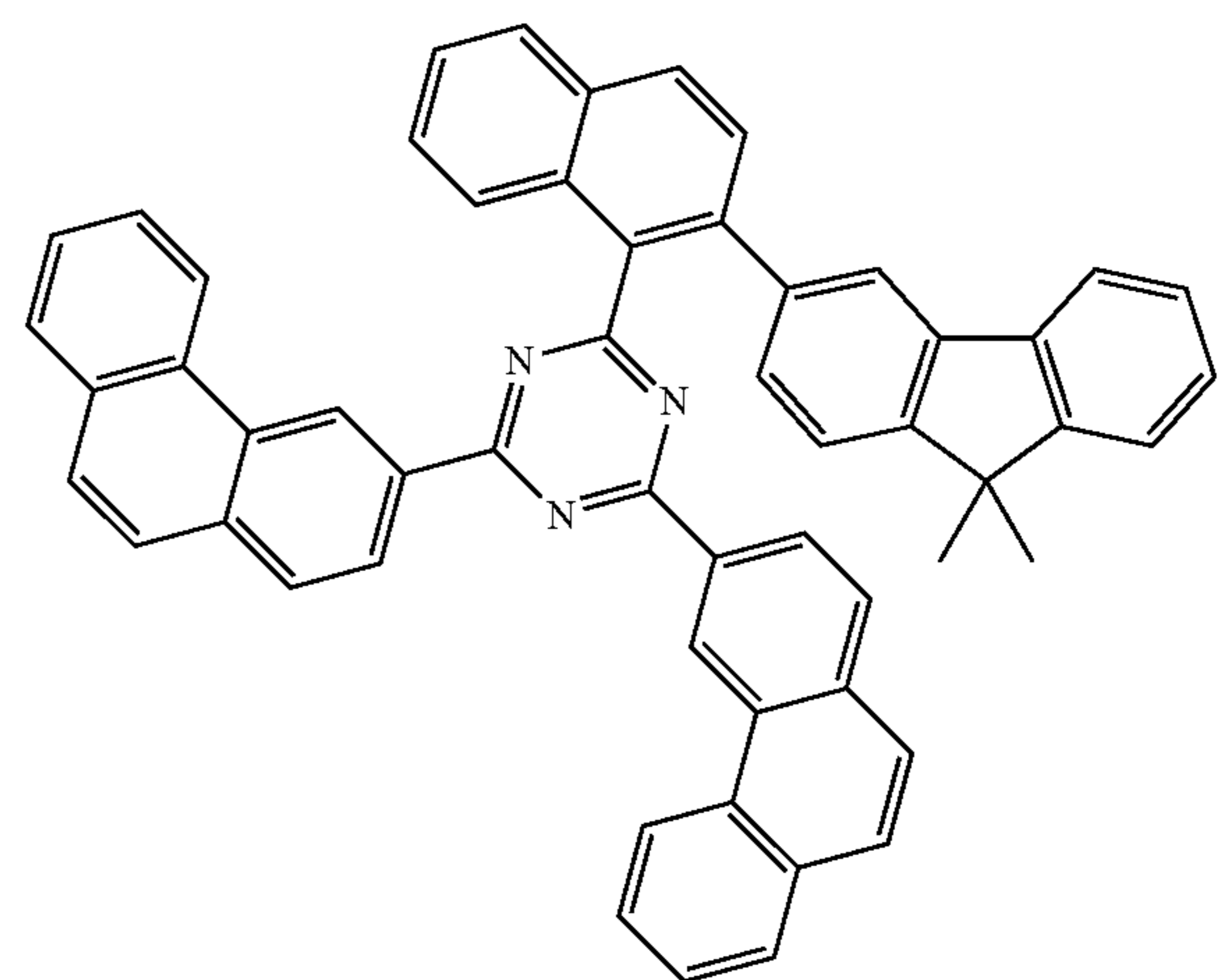
[Compound 154]
