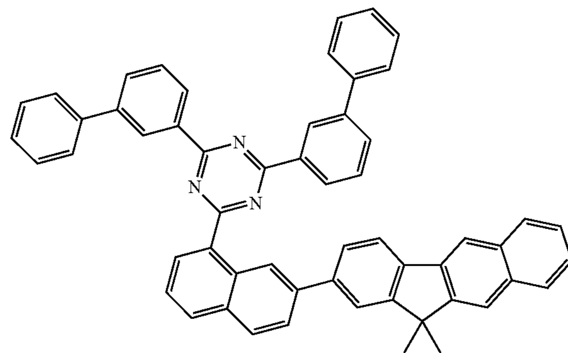
[Compound 245]
