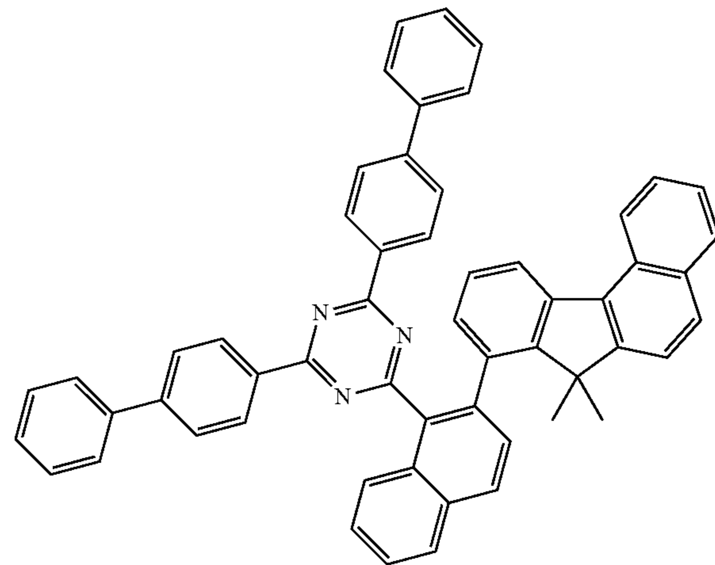
[Compound 244]
