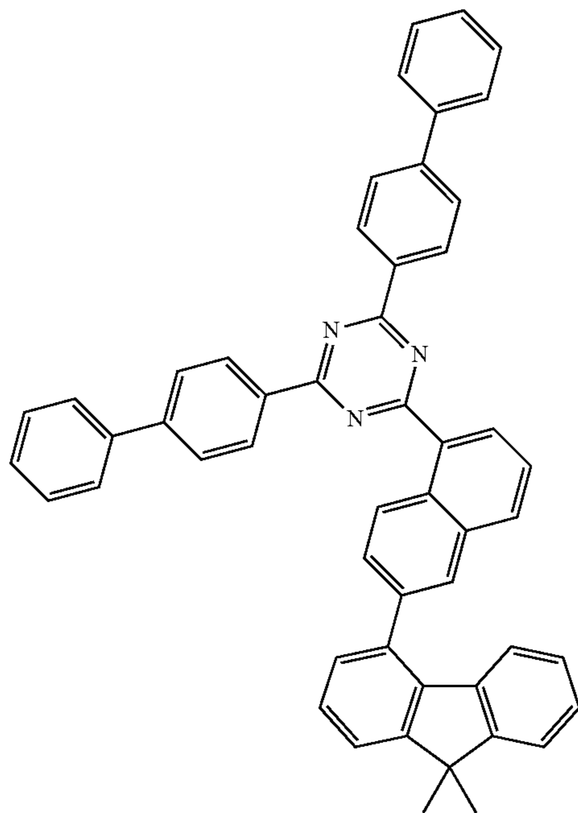
[Compound 30]
