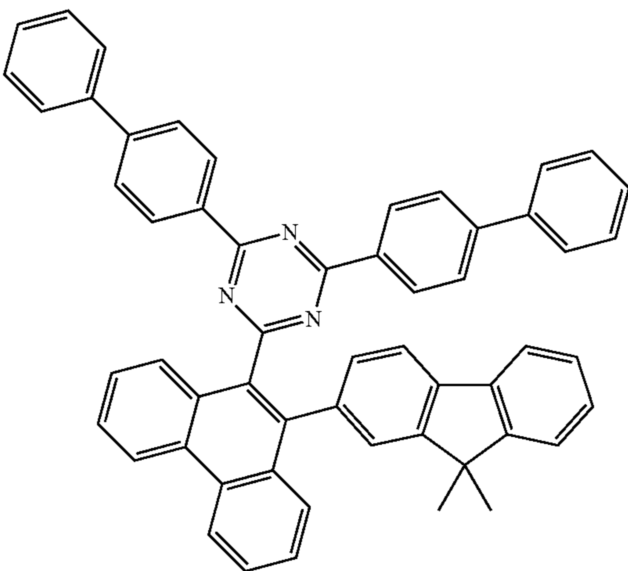
[Compound 191]
