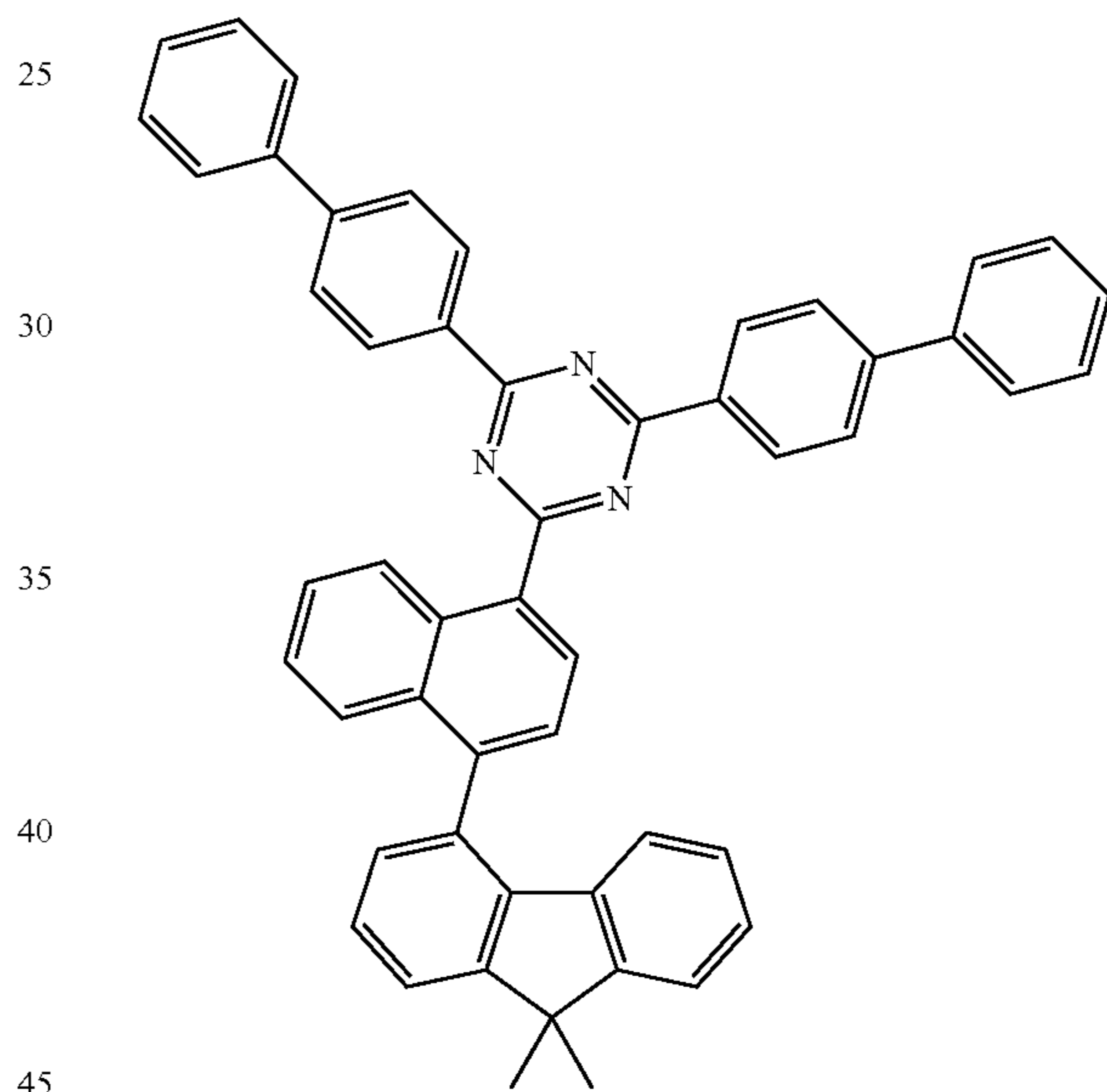
[Compound 26]
