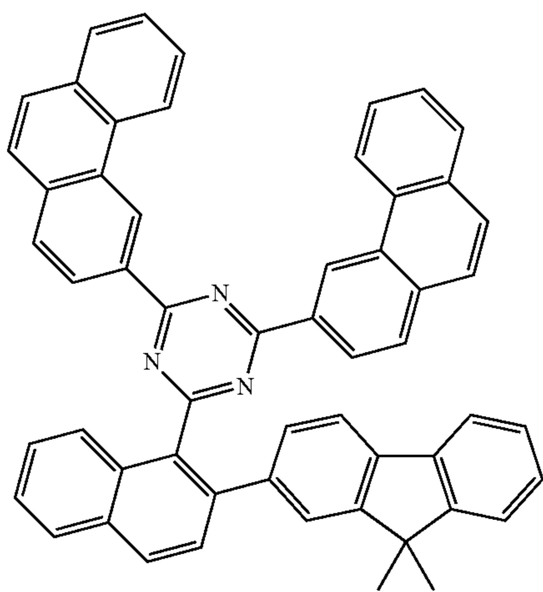
[Compound 144]
