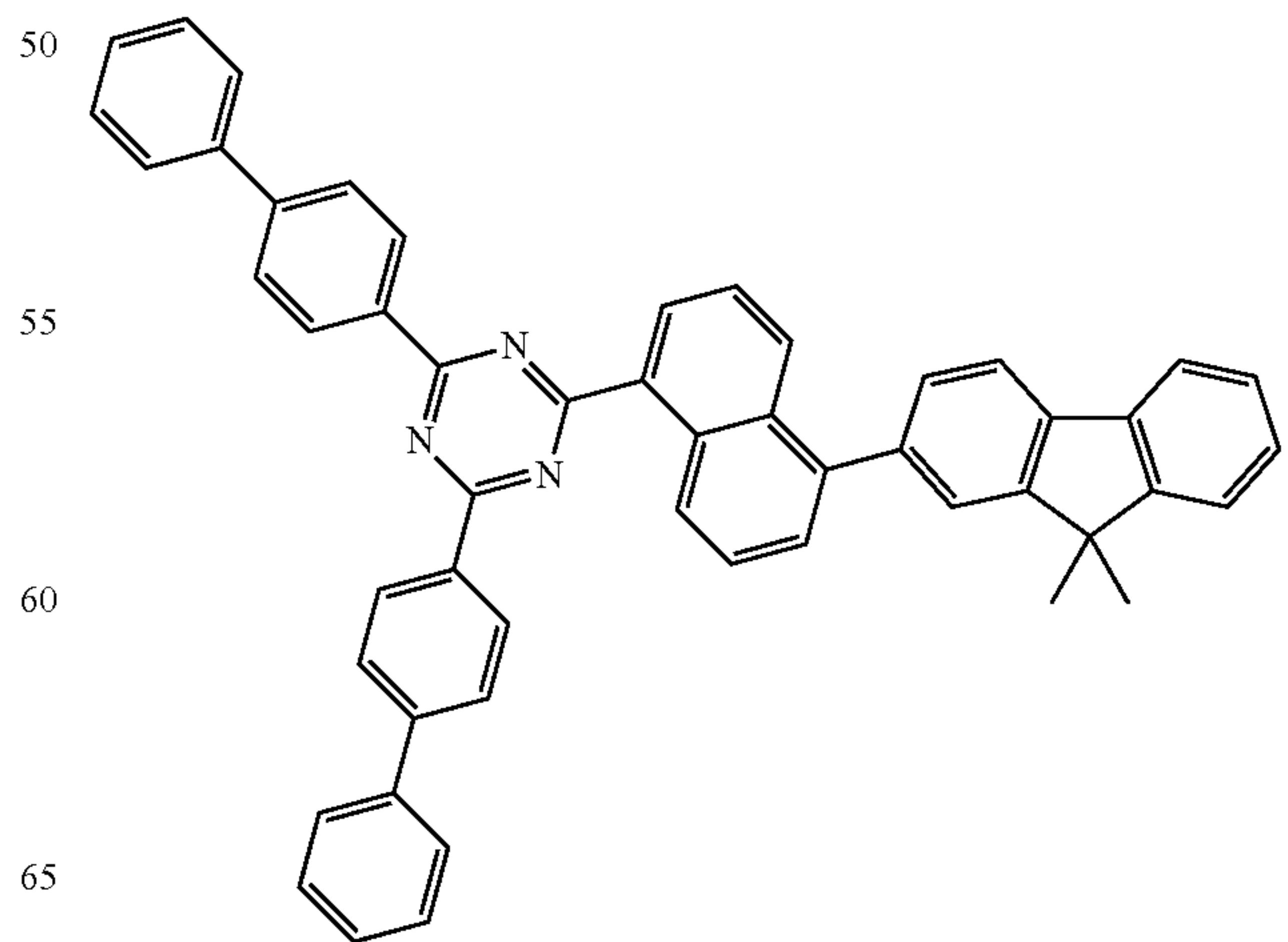
[Compound 27]
