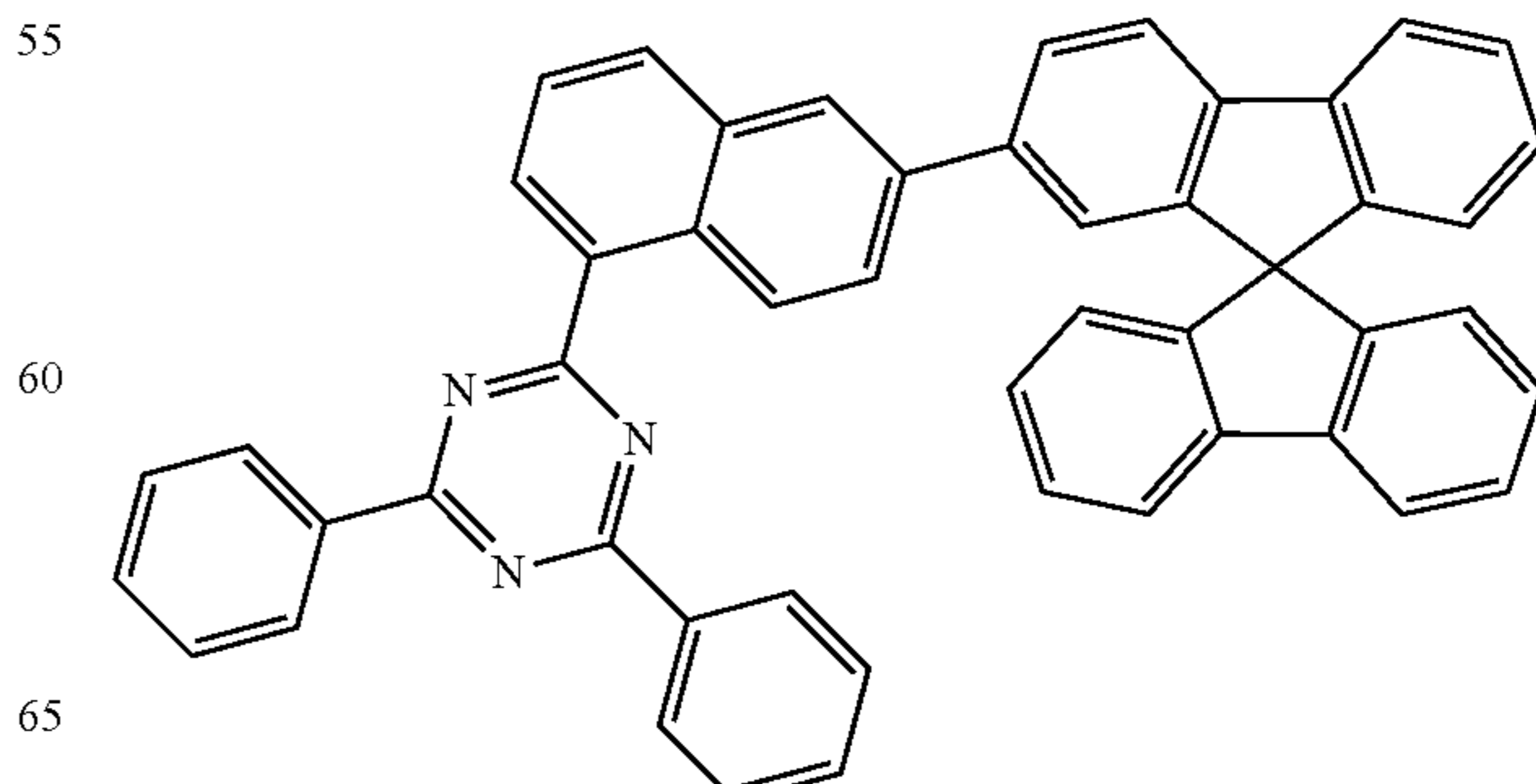
[Compound 10]
