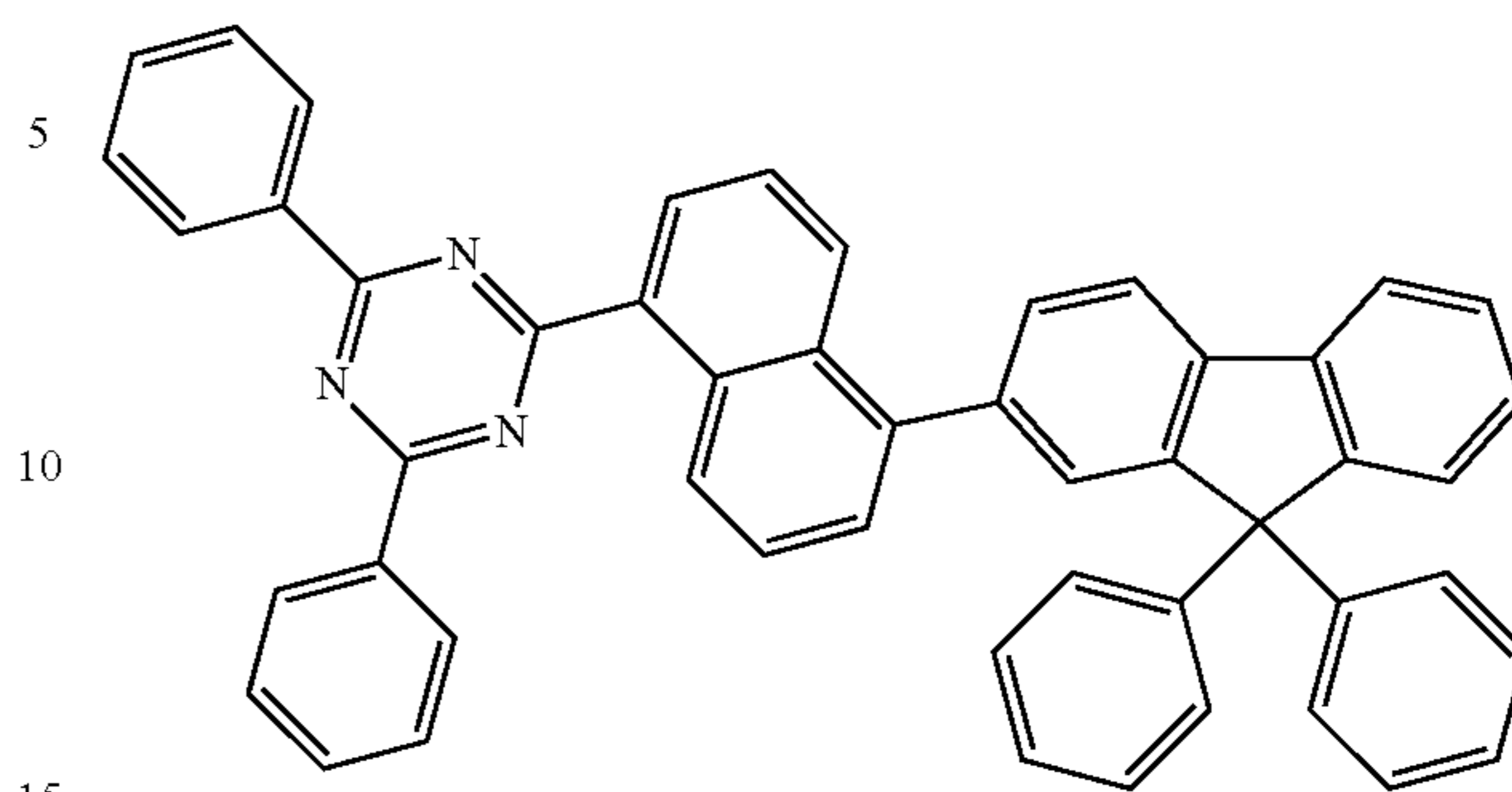
[Compound 7]
