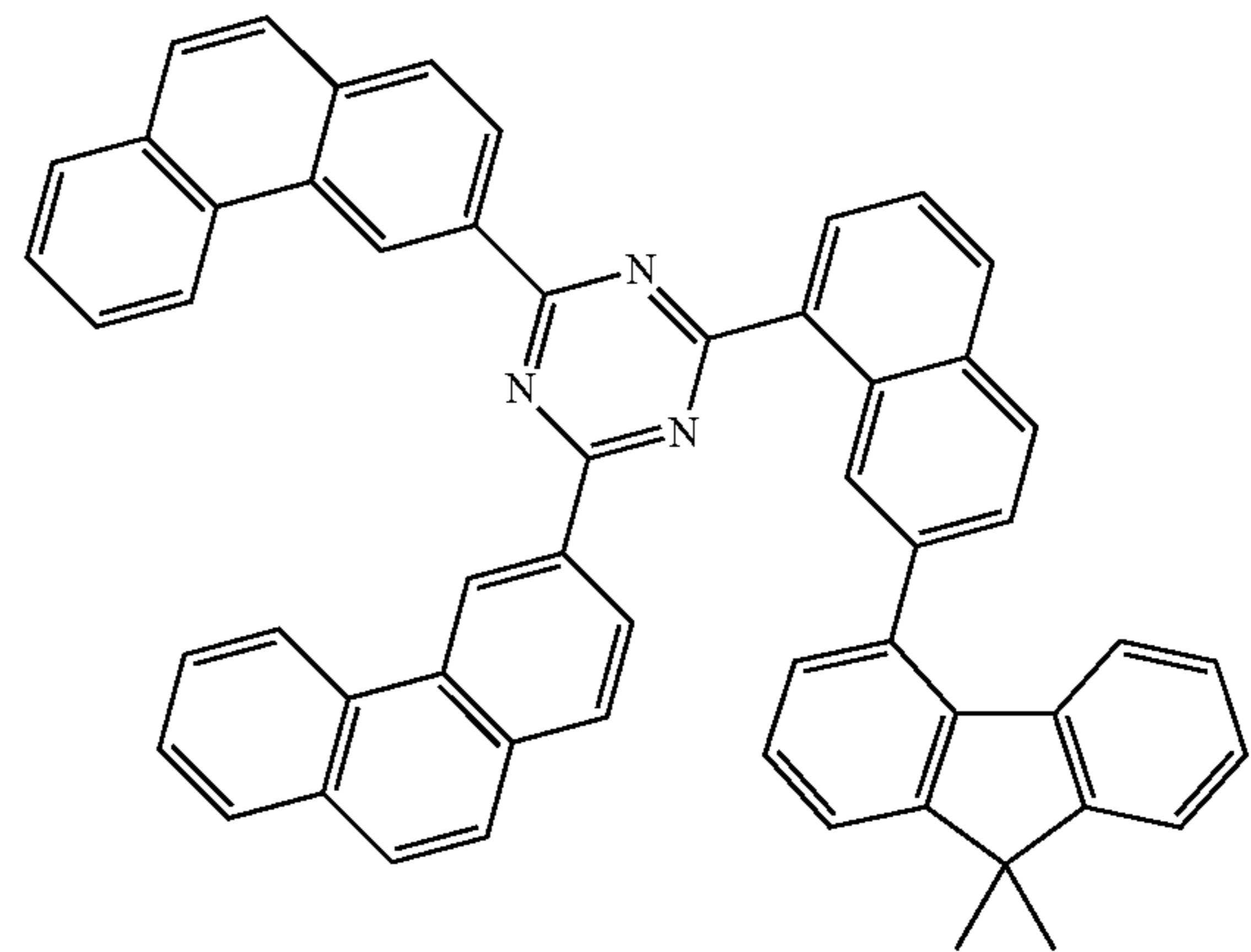
[Compound 152]
