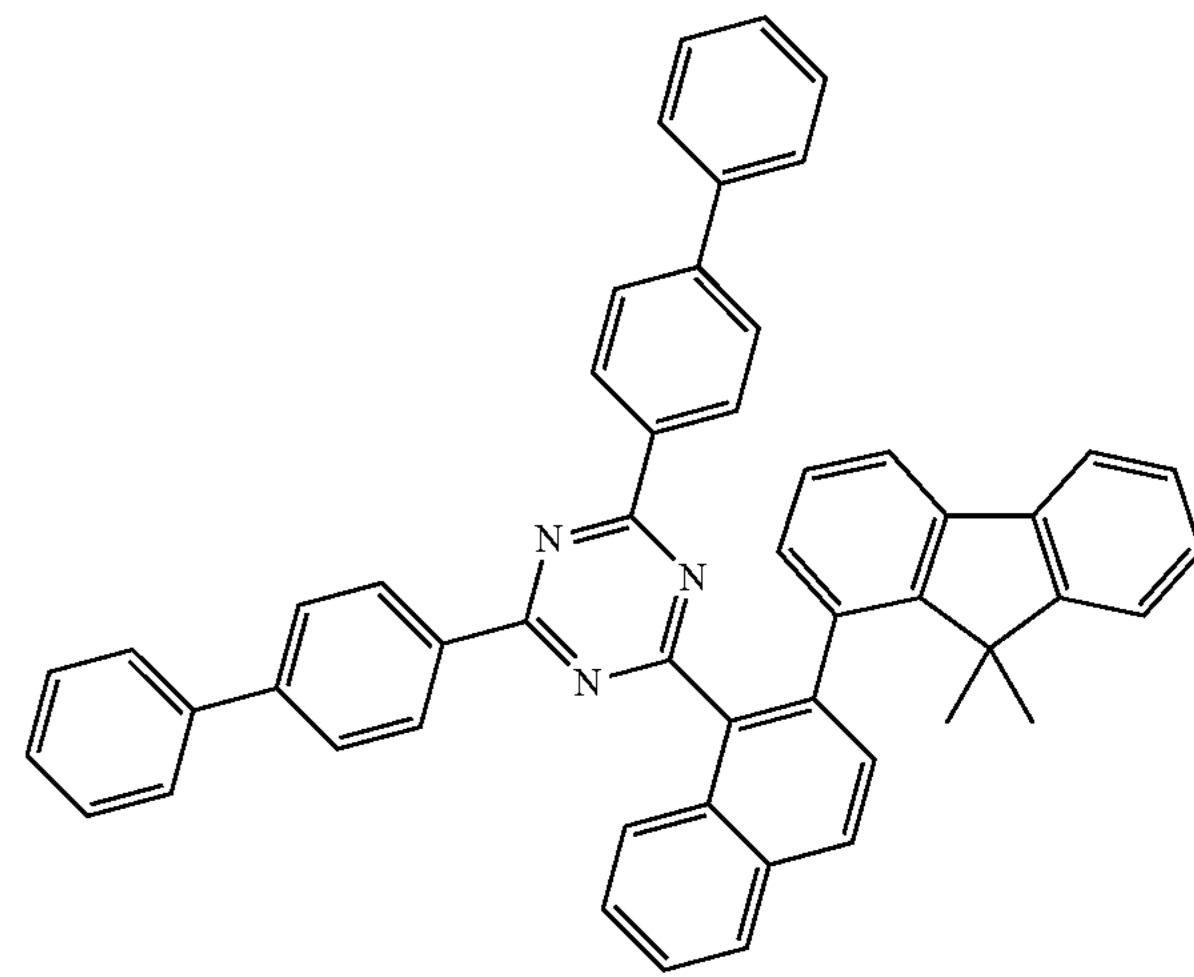
[Compound 33]
