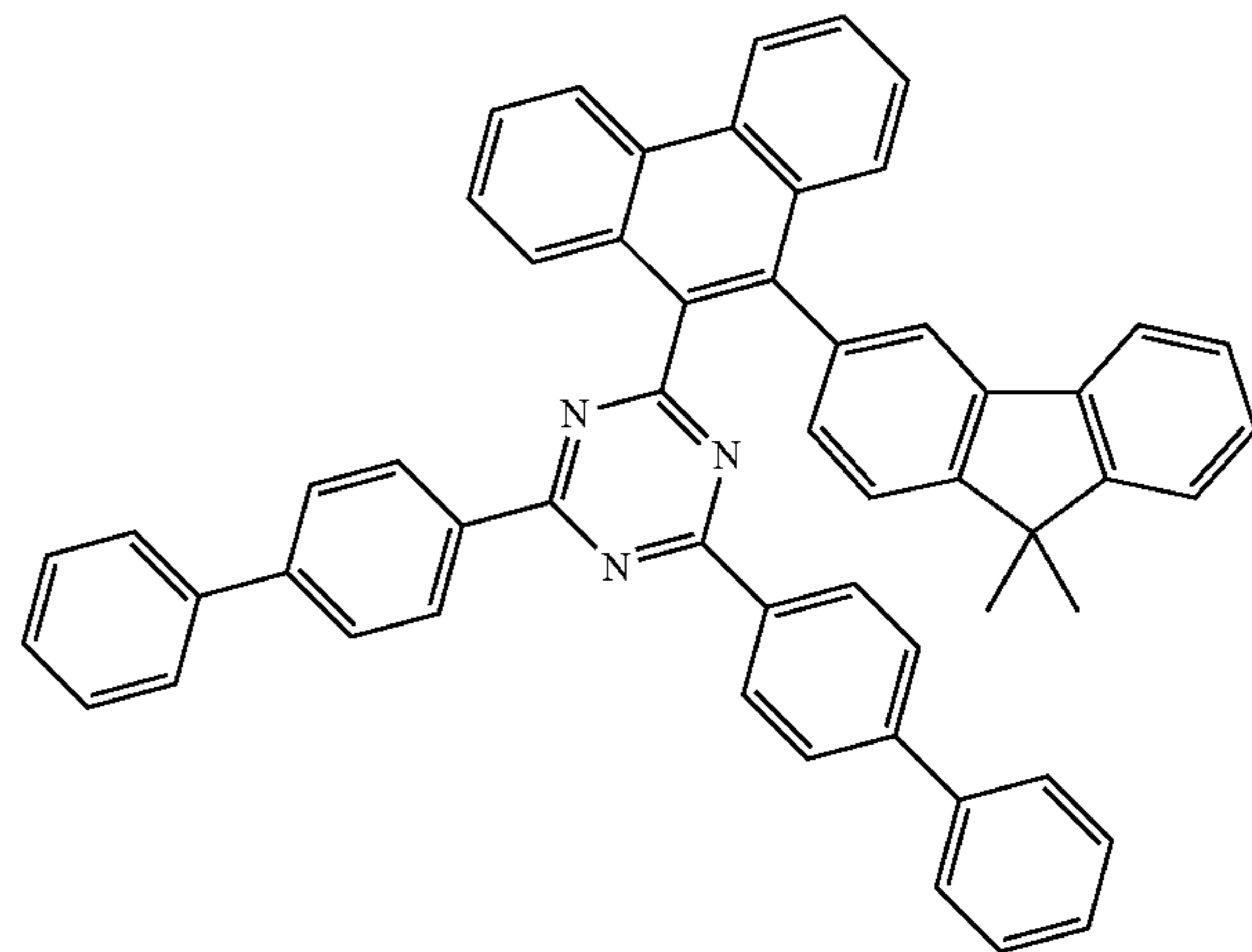
[Compound 194]
