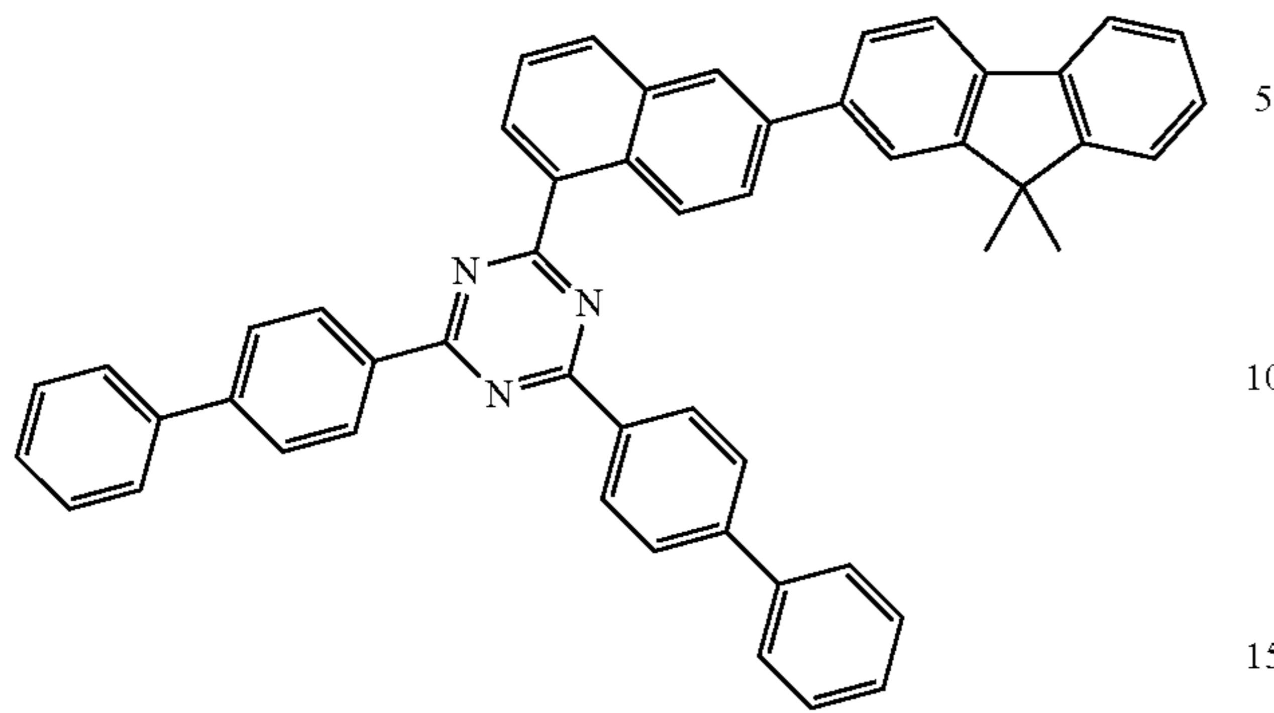
[Compound 29]
