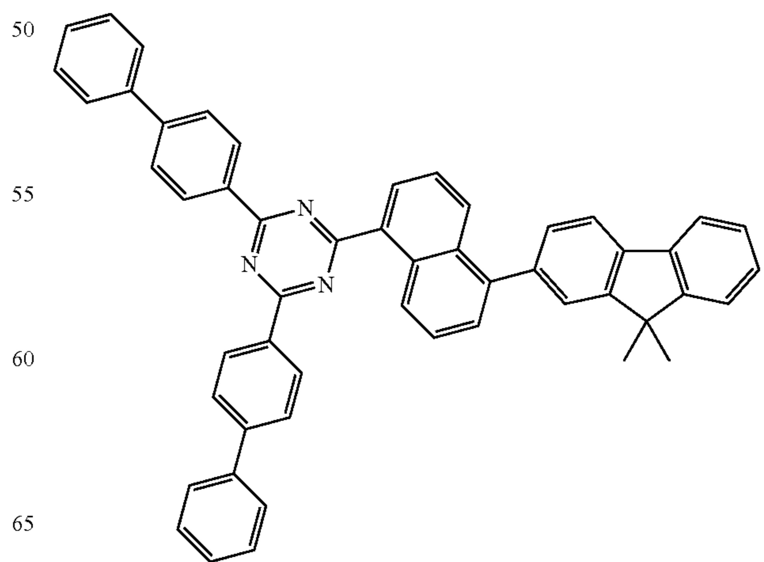
[Compound 27]
