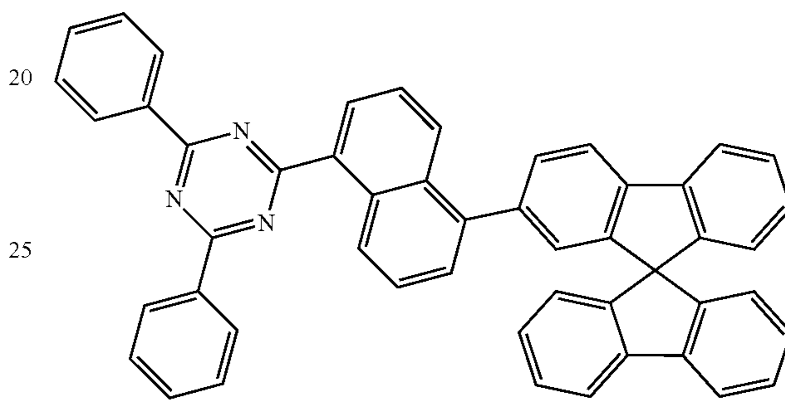
[Compound 8]
