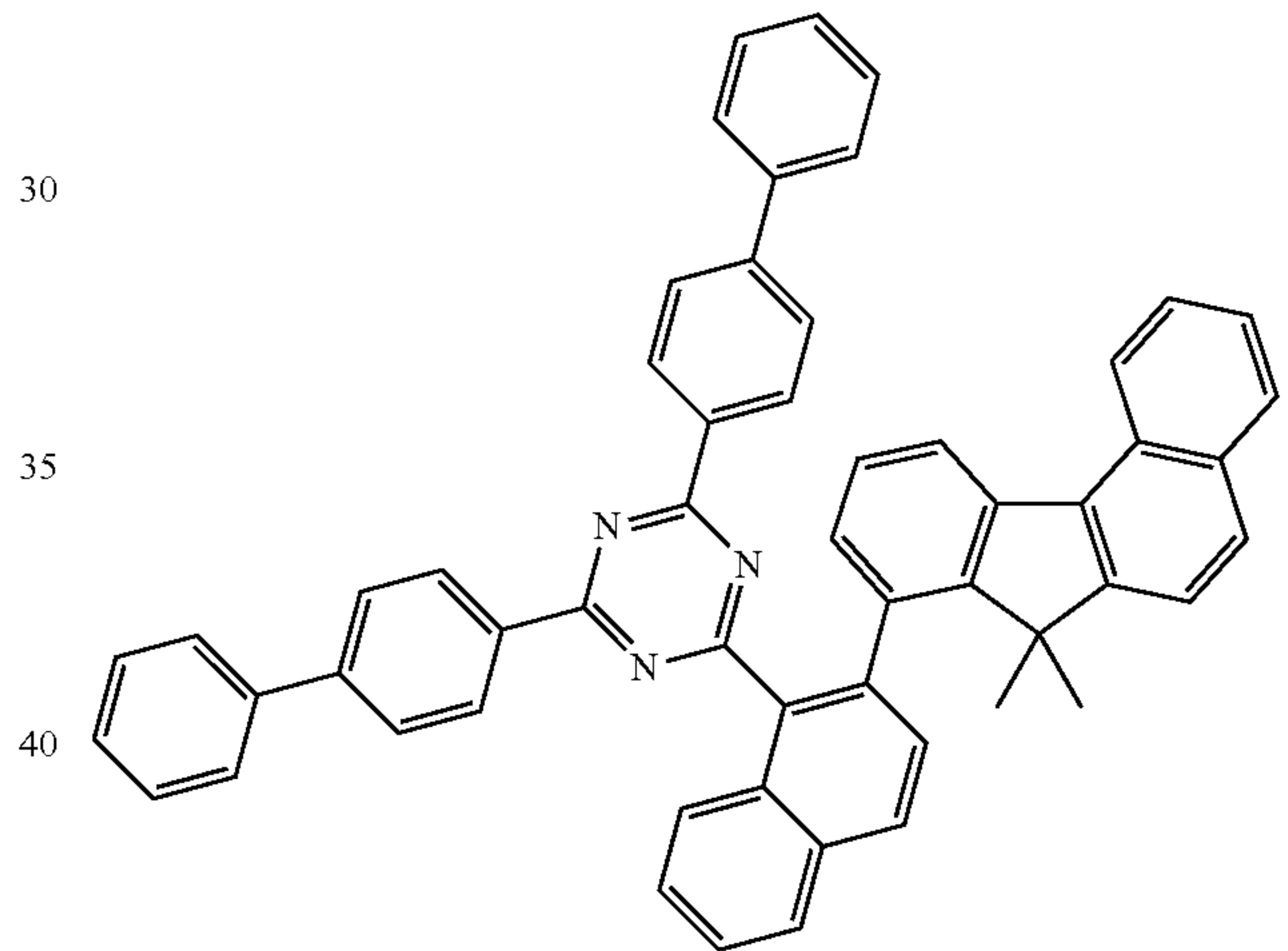
[Compound 244]
