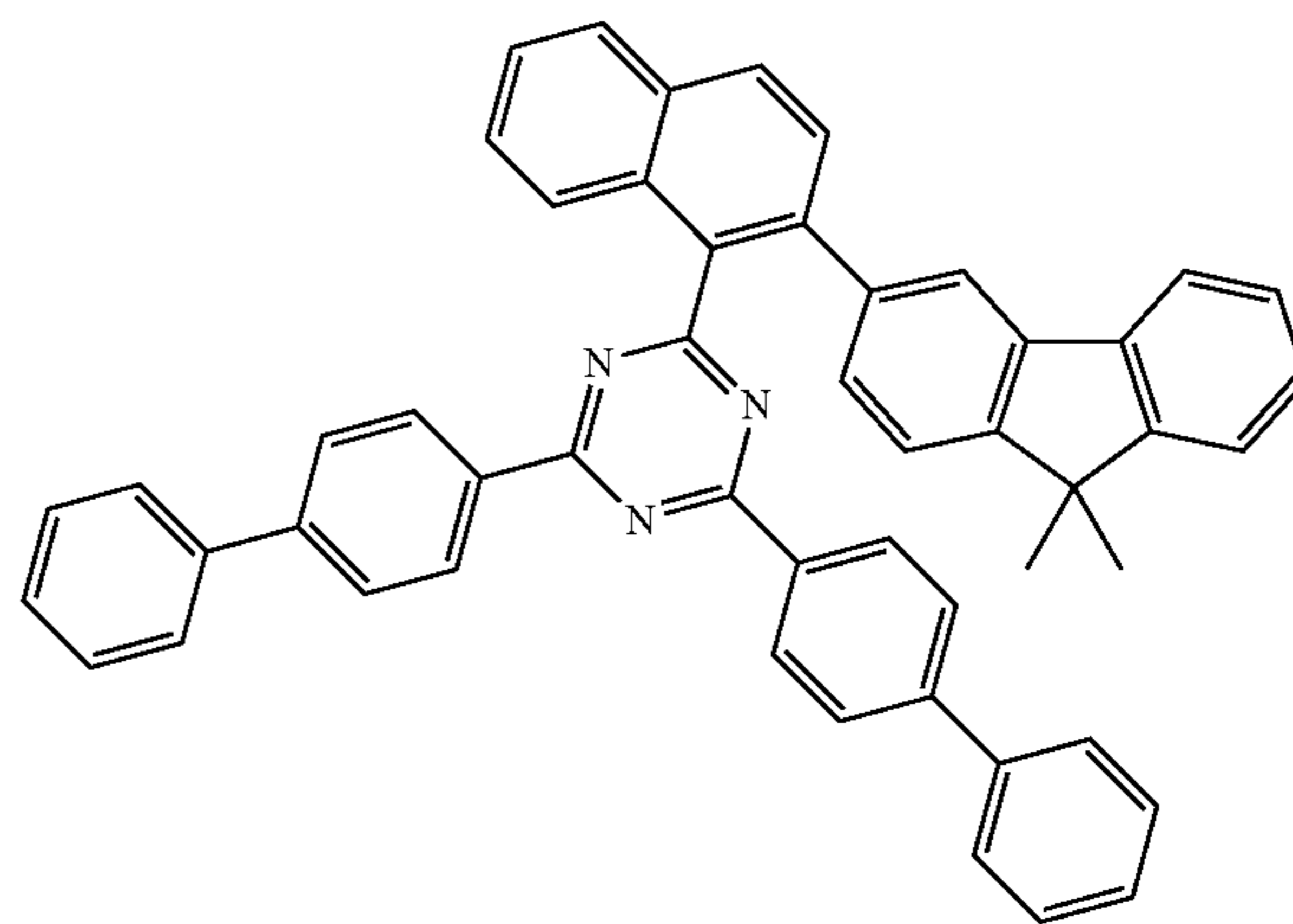
[Compound 34]
