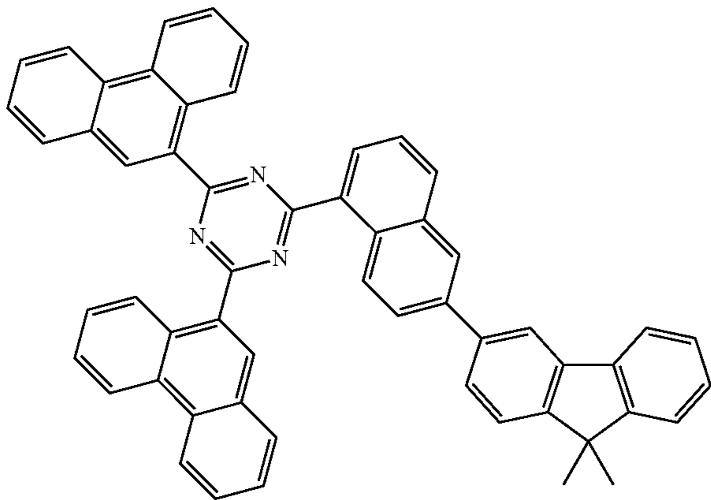
[Compound 140]
