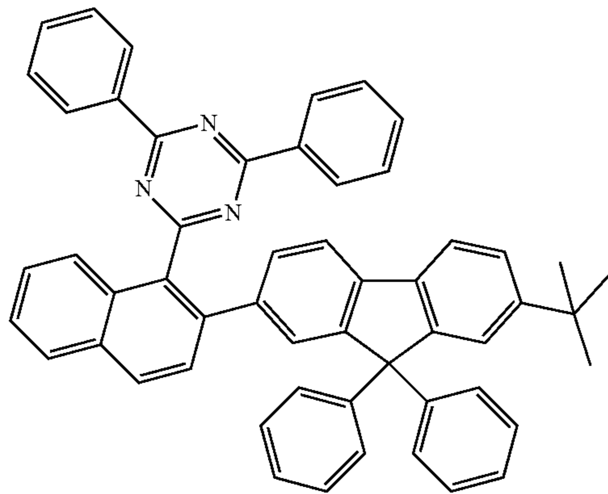
[Compound 241]
