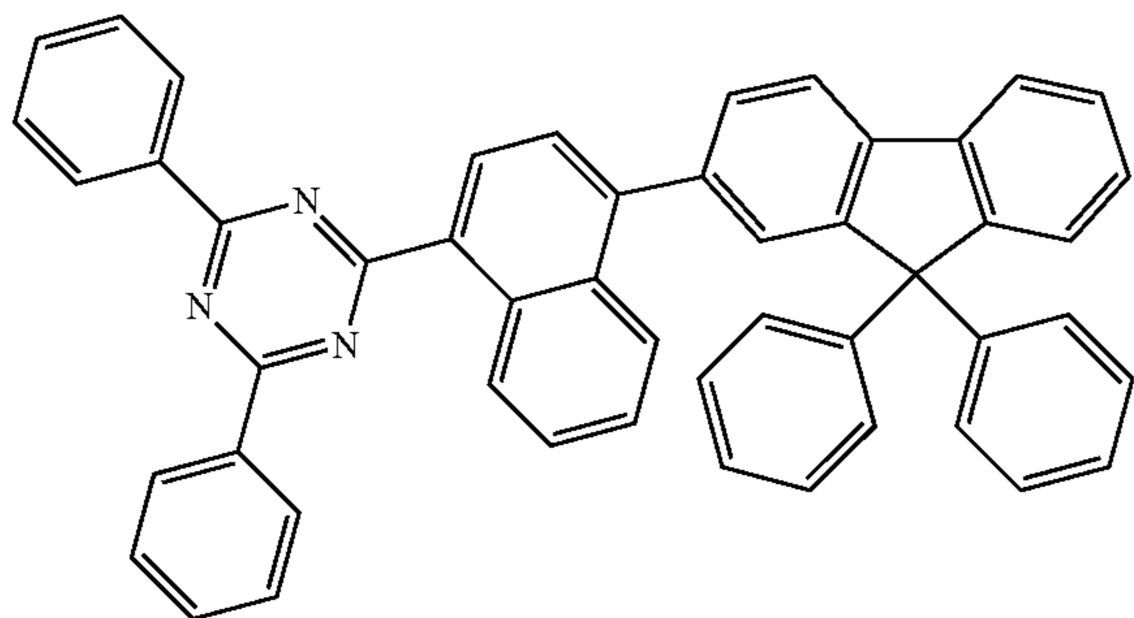
[Compound 5]
