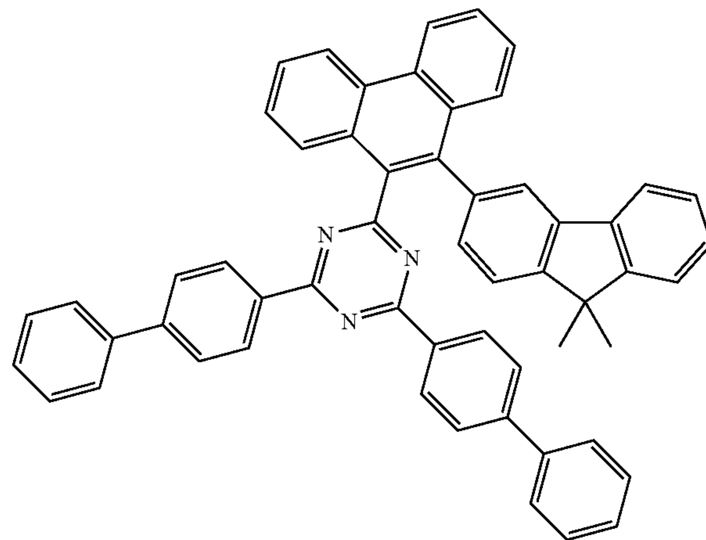
[Compound 194]
