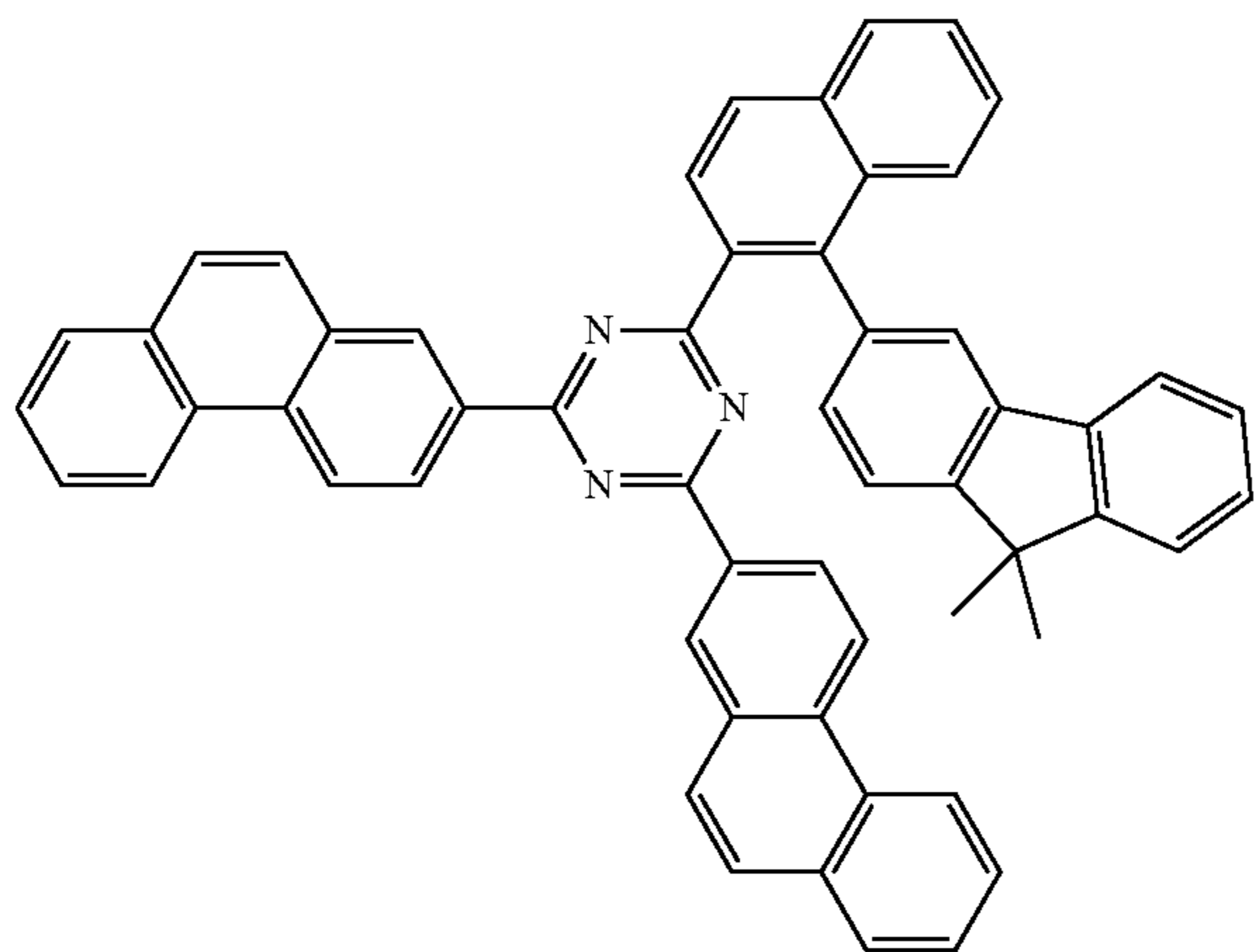
[Compound 3]
