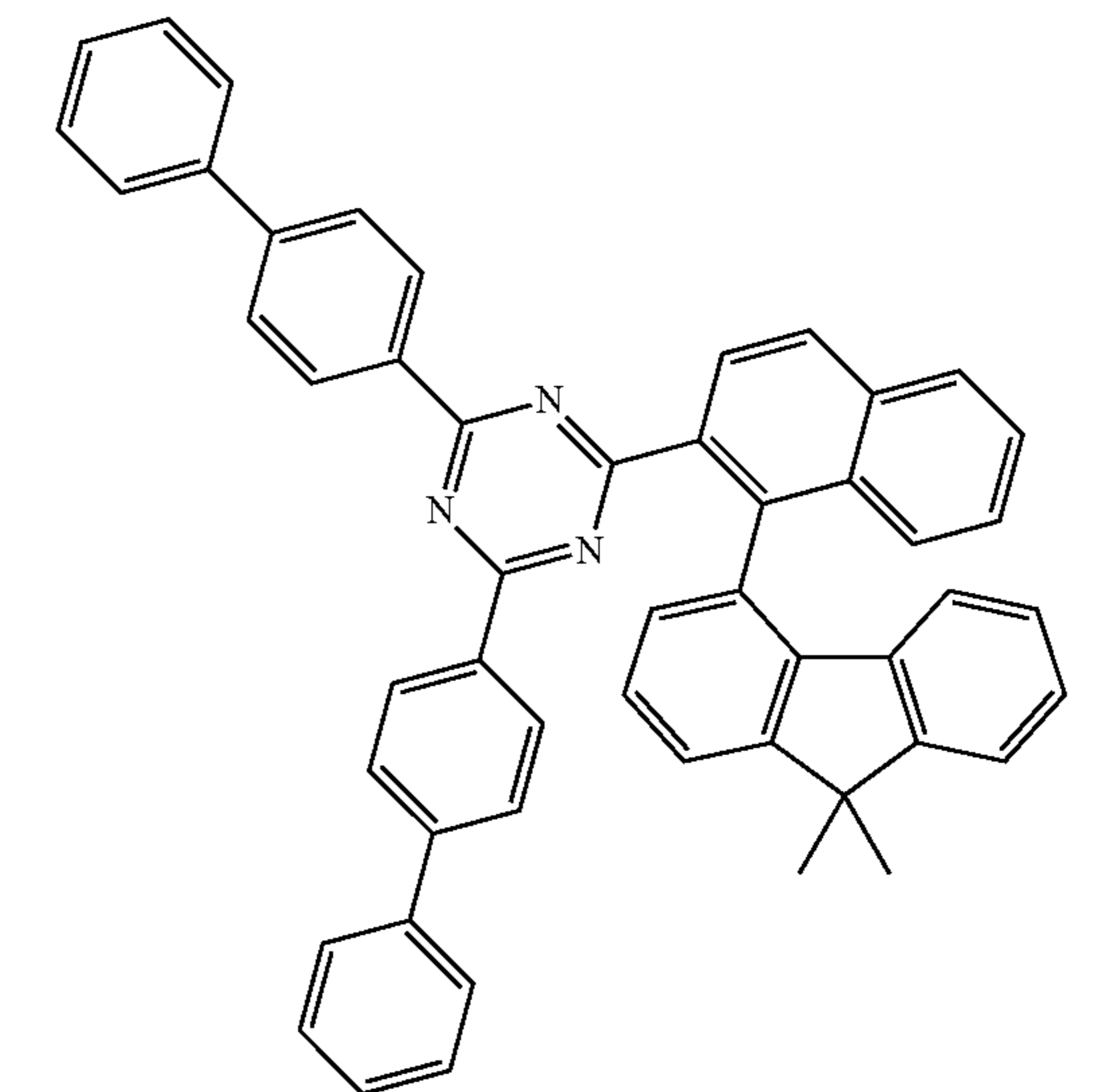
[Compound 212]
