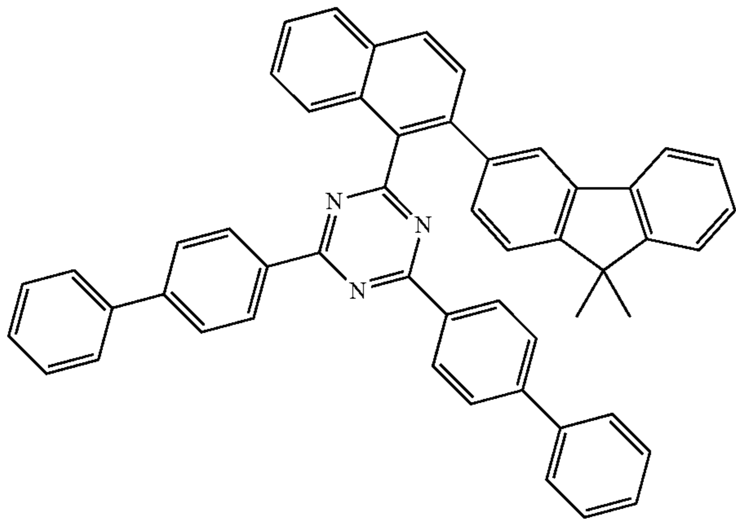
[Compound 34]
