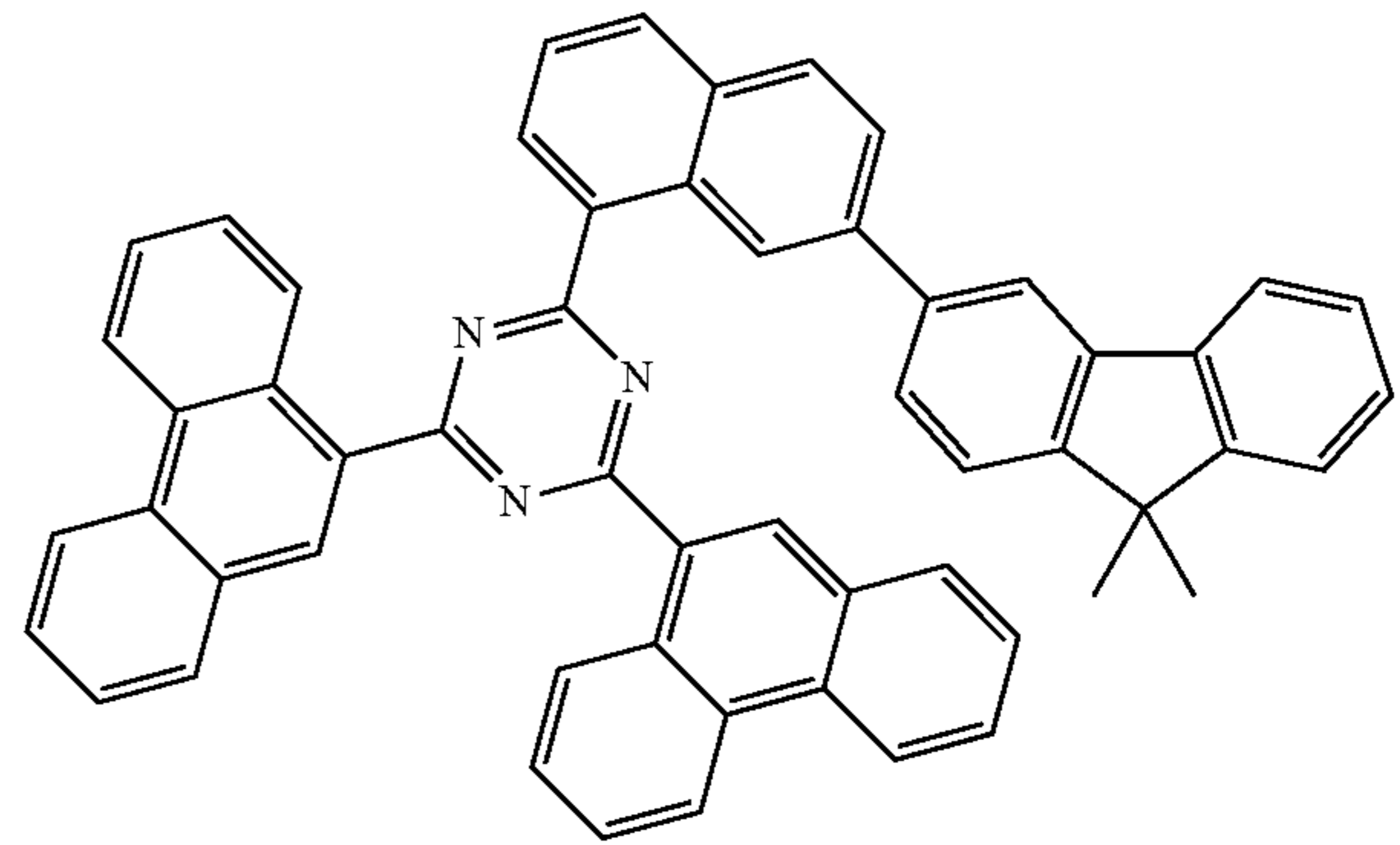
[Compound 142]
