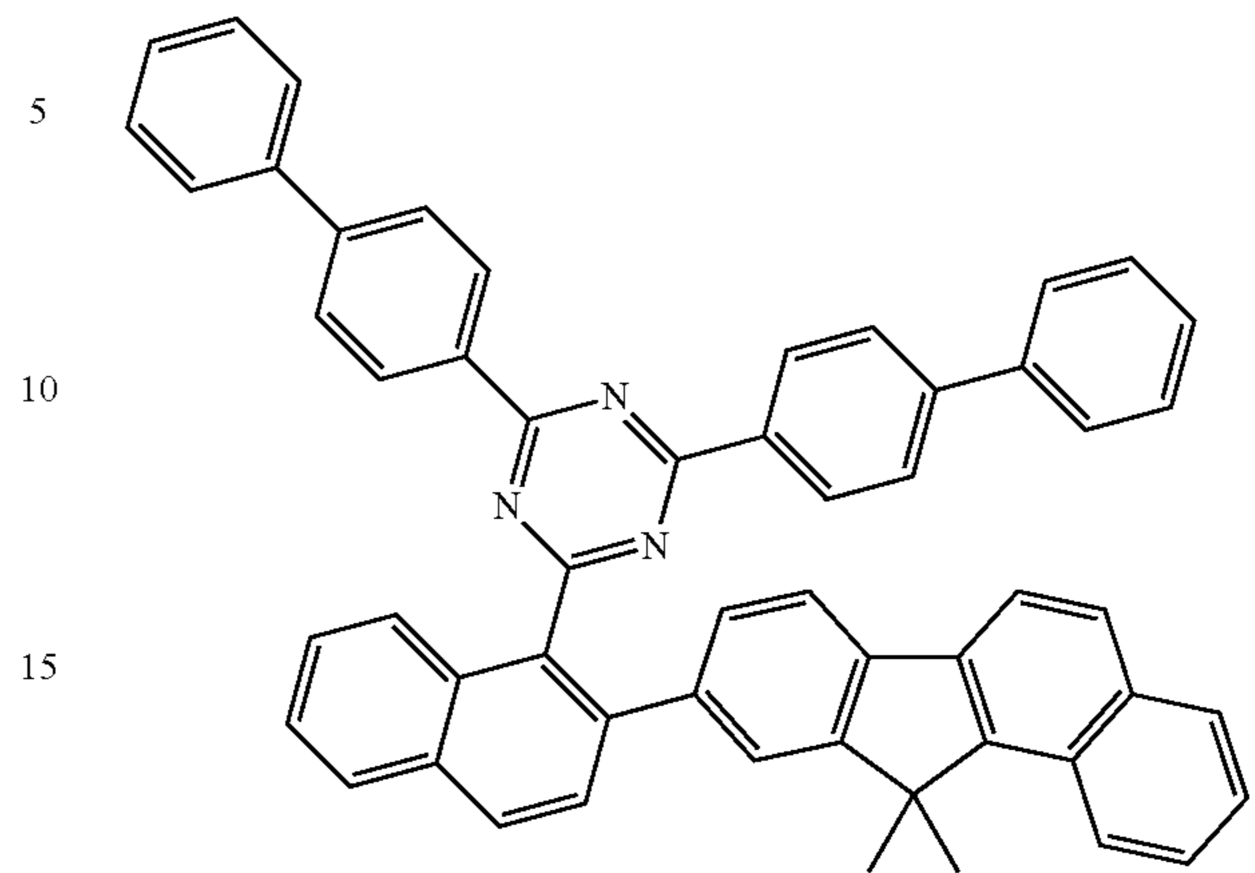
[Compound 243]
