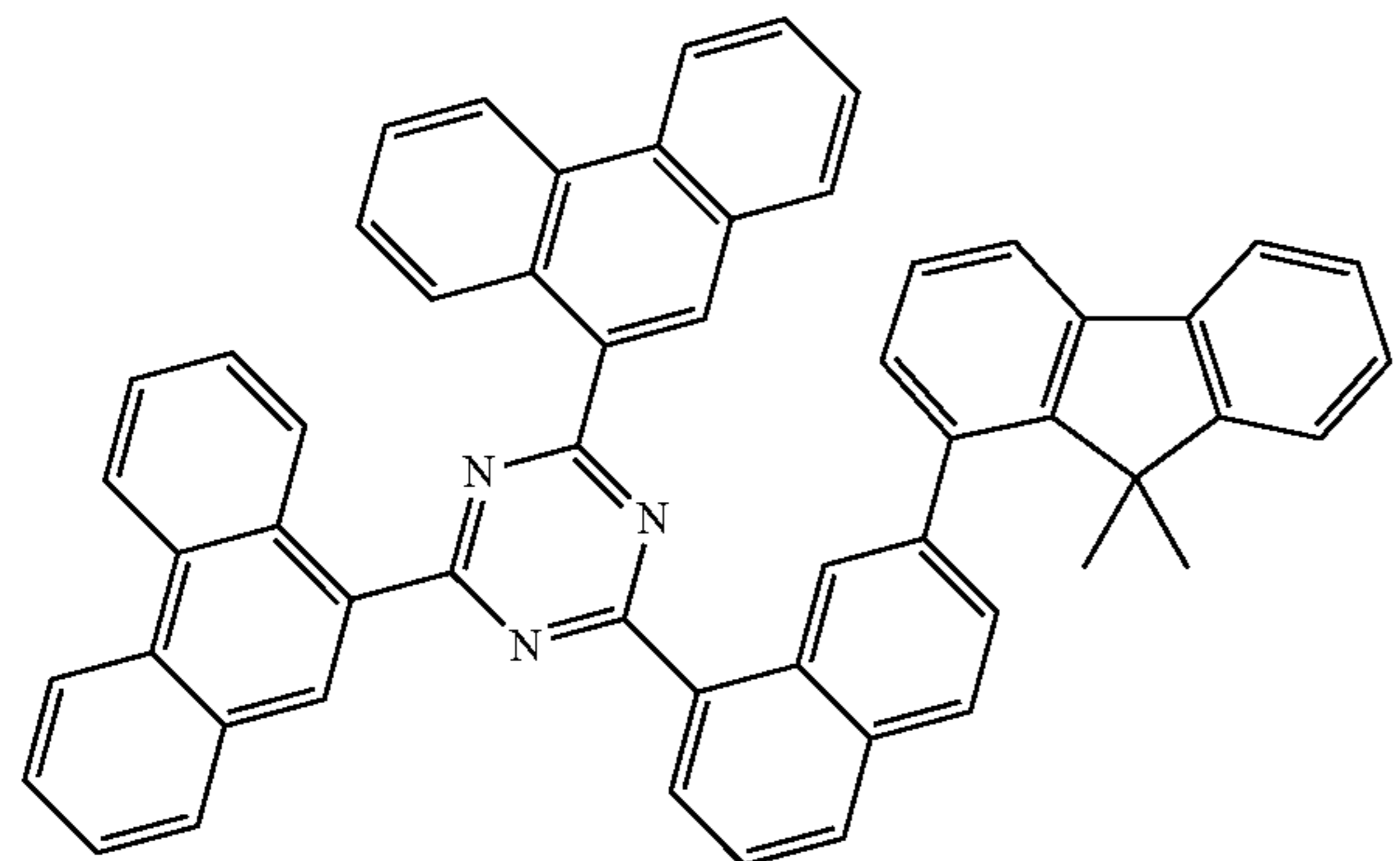
[Compound 141]
