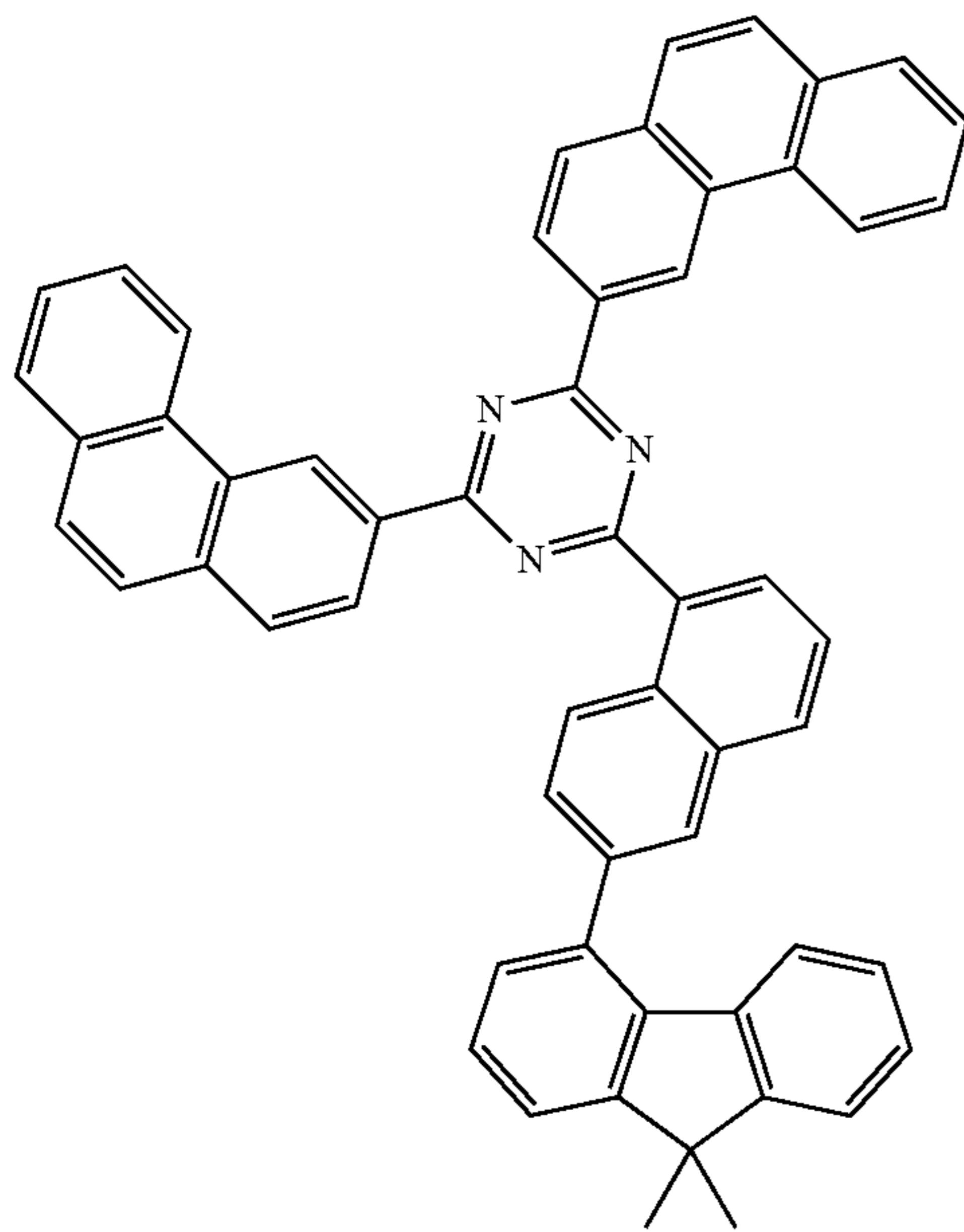
[Compound 150]
