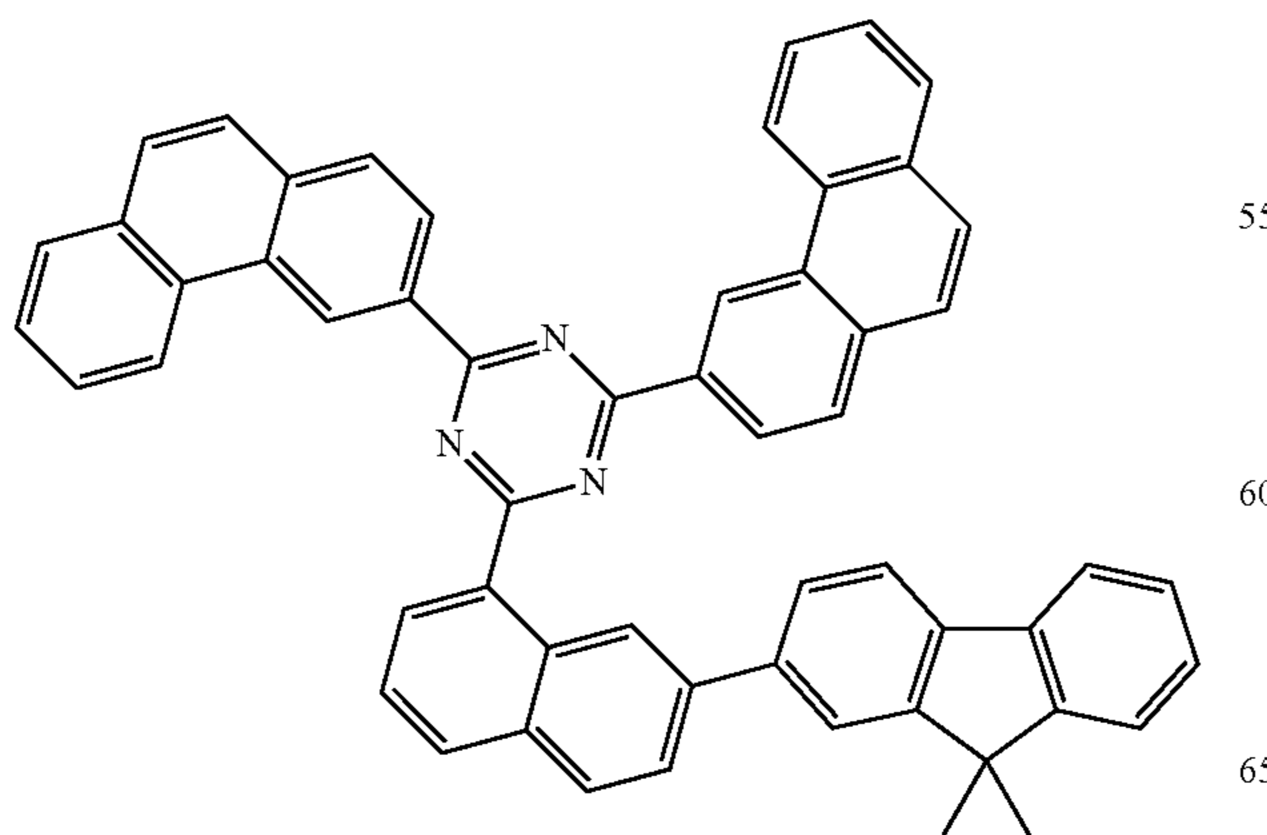
[Compound 151]
