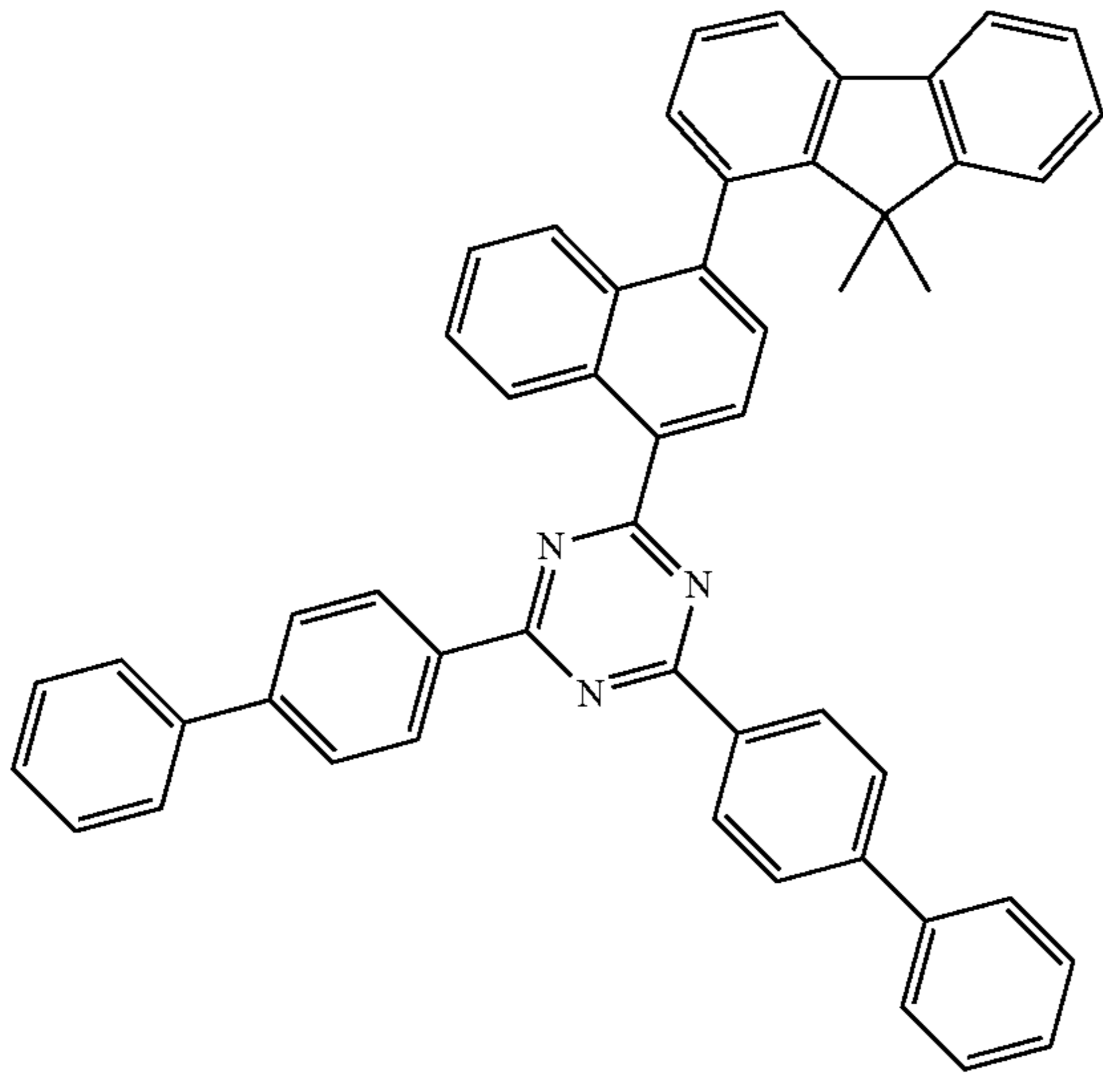
[Compound 35]
