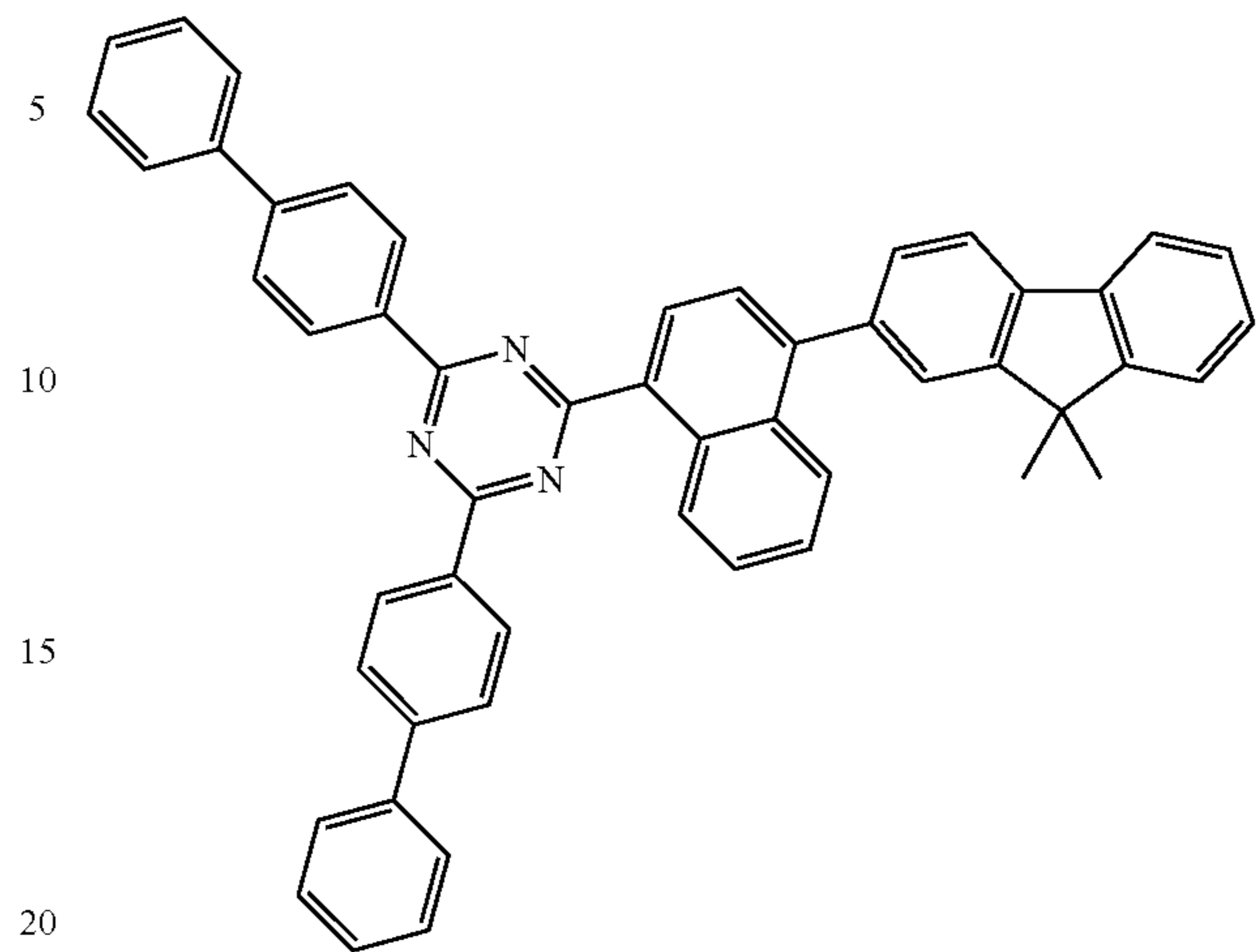
[Compound 25]
