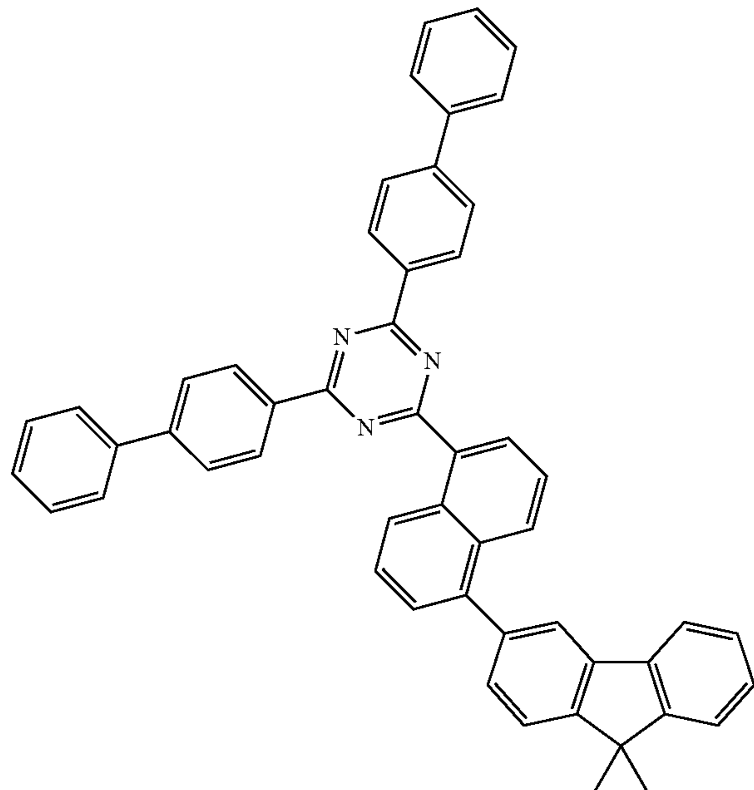
[Compound 38]
