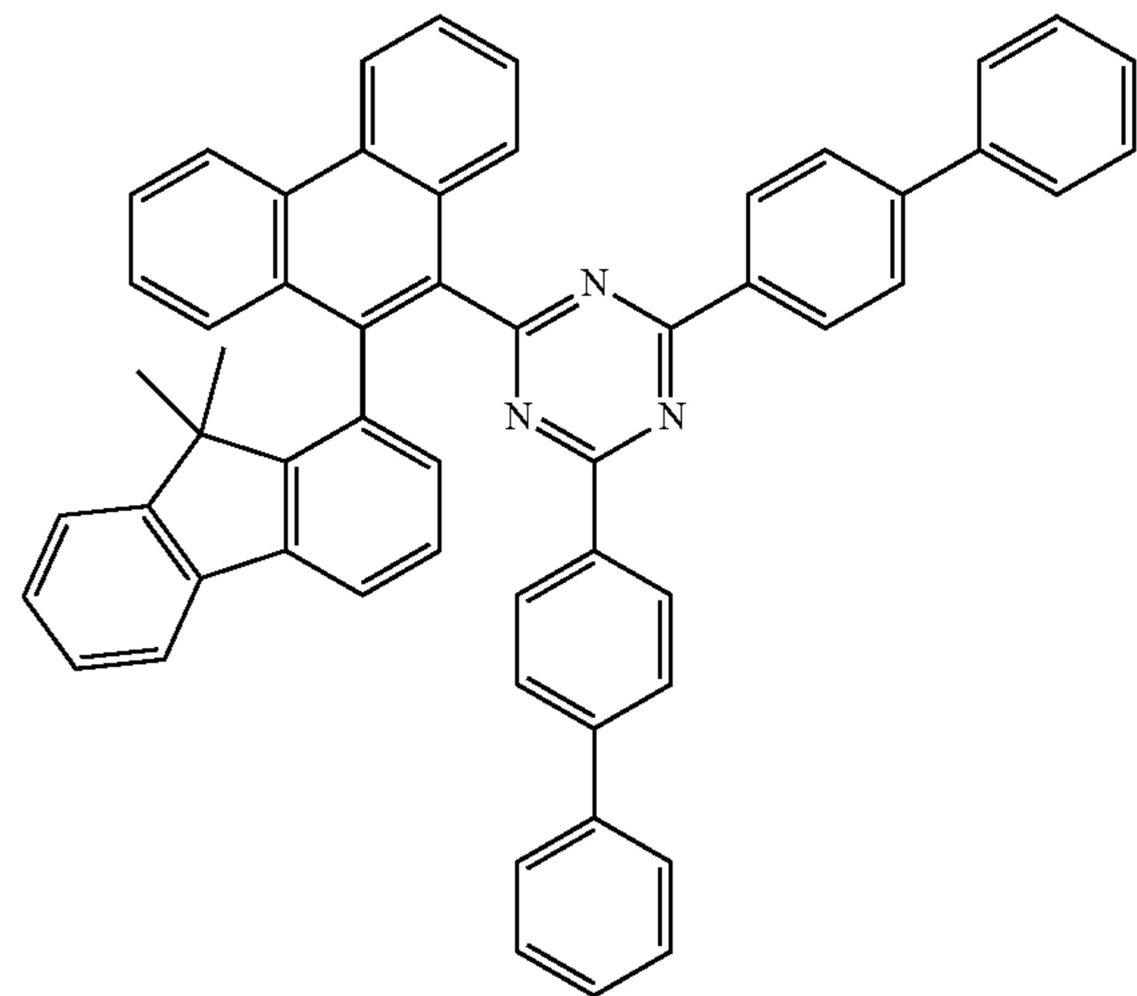
[Compound 193]
