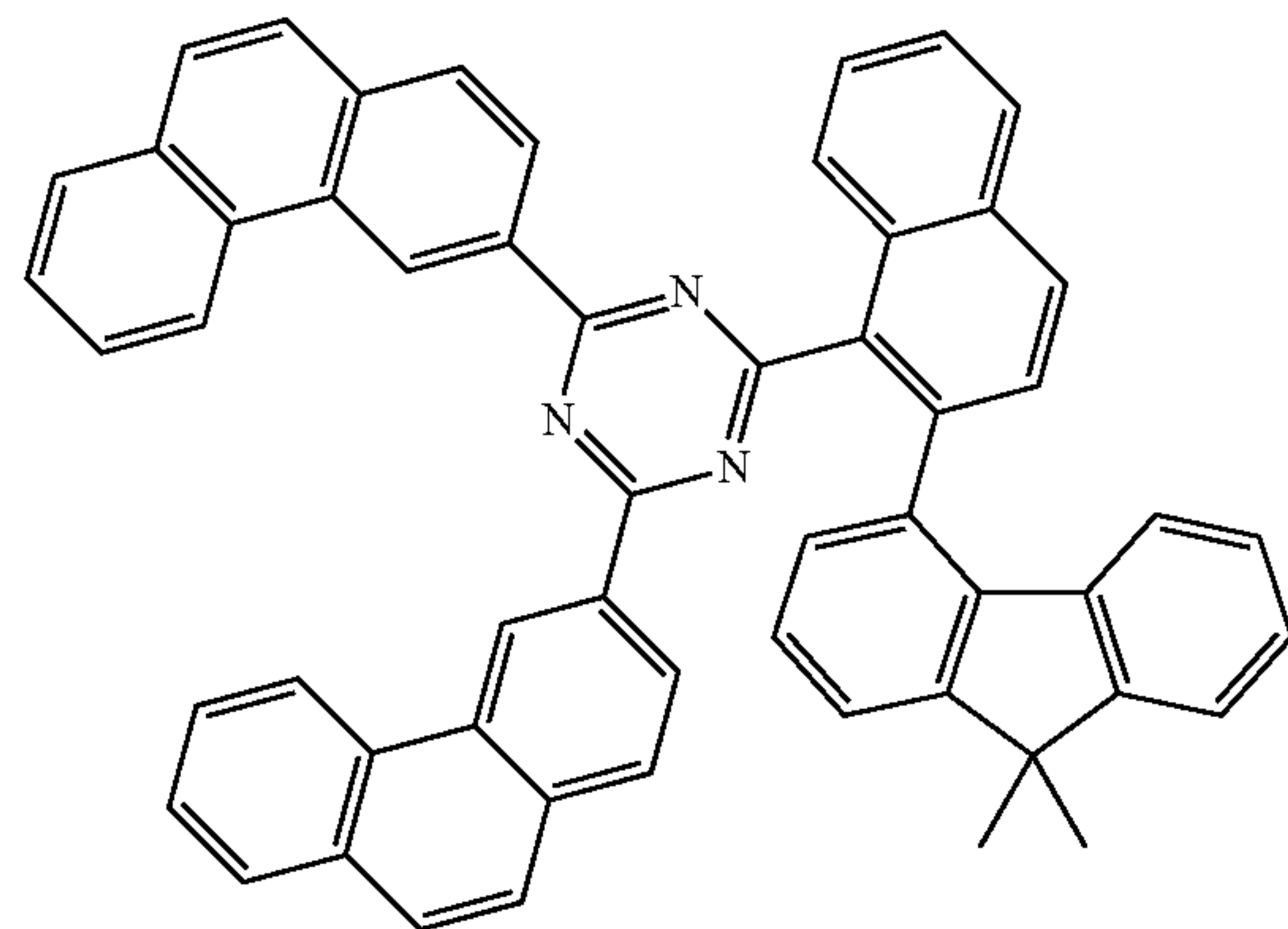
[Compound 145]
