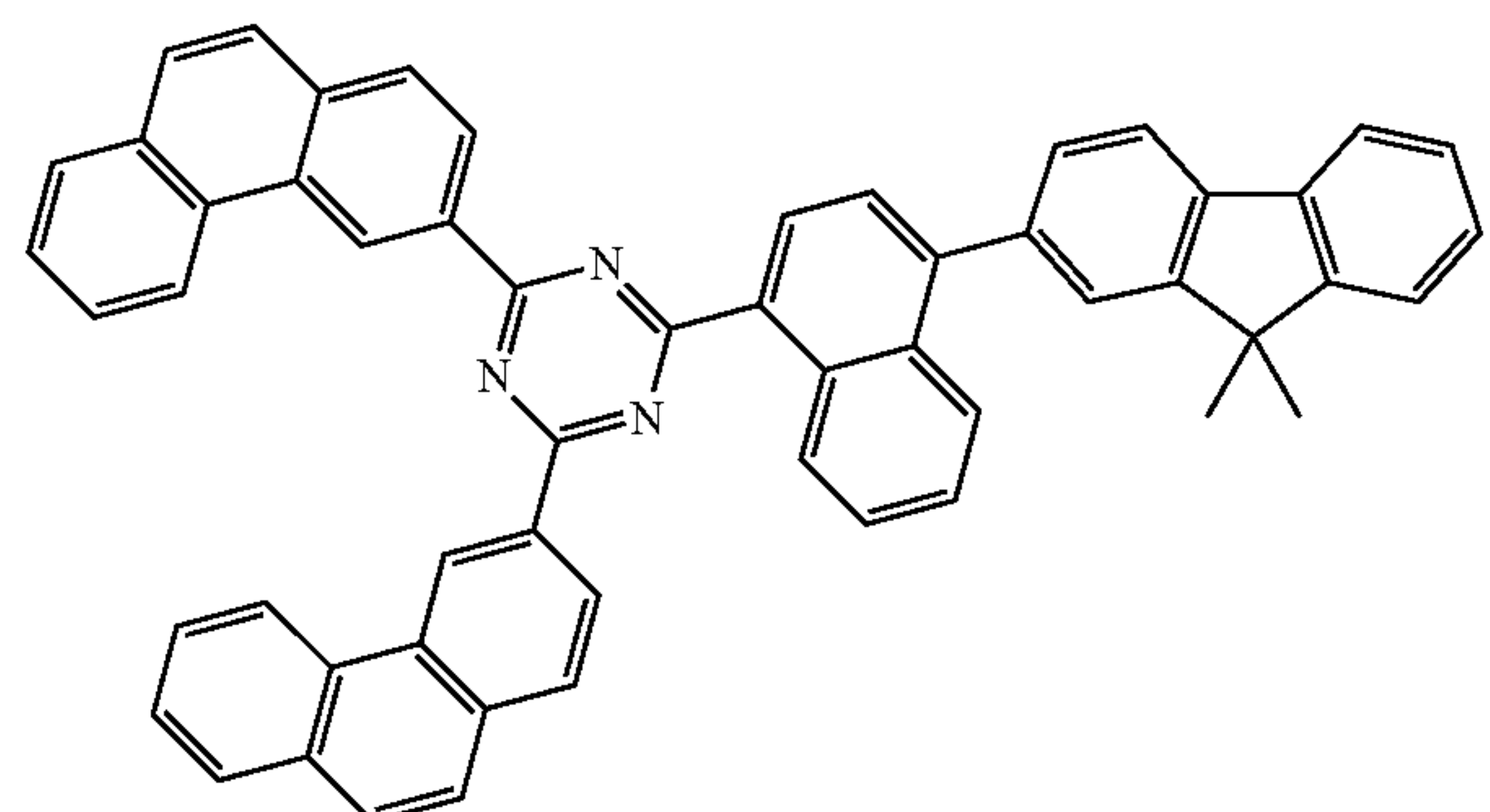
[Compound 145]
