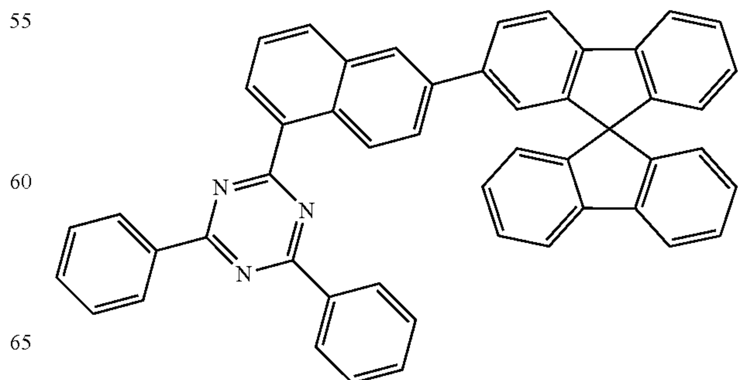
[Compound 10]
