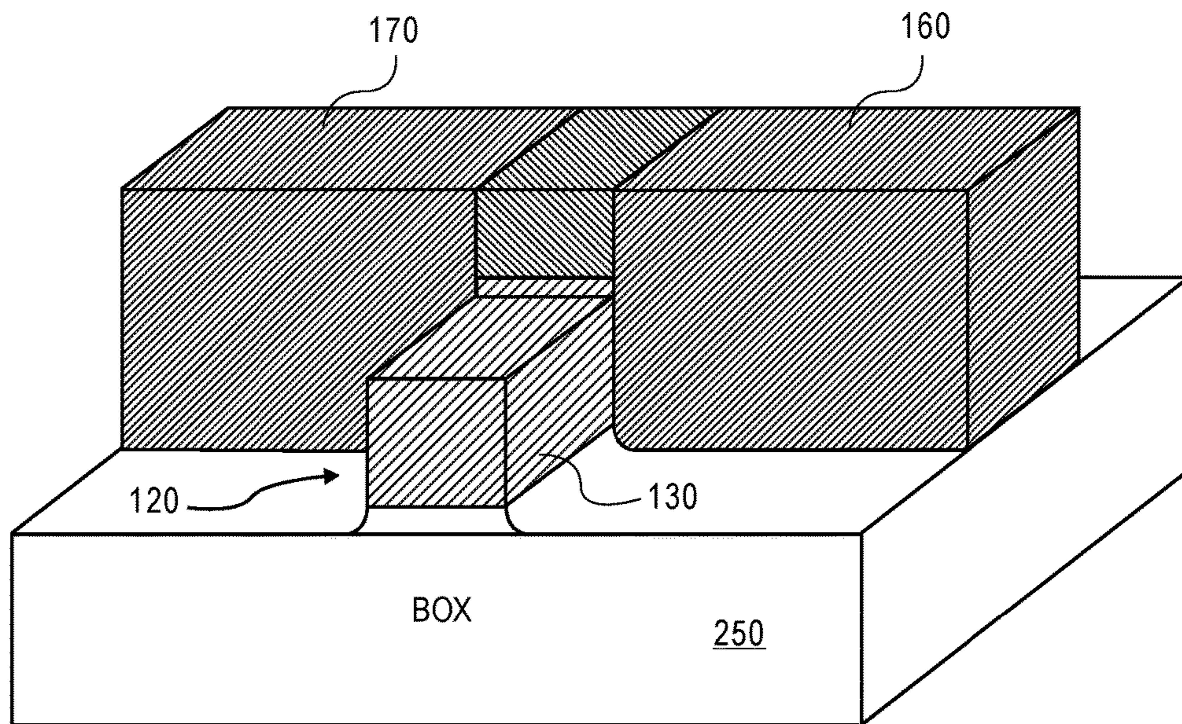
FIG. 2 (PRIOR ART)
