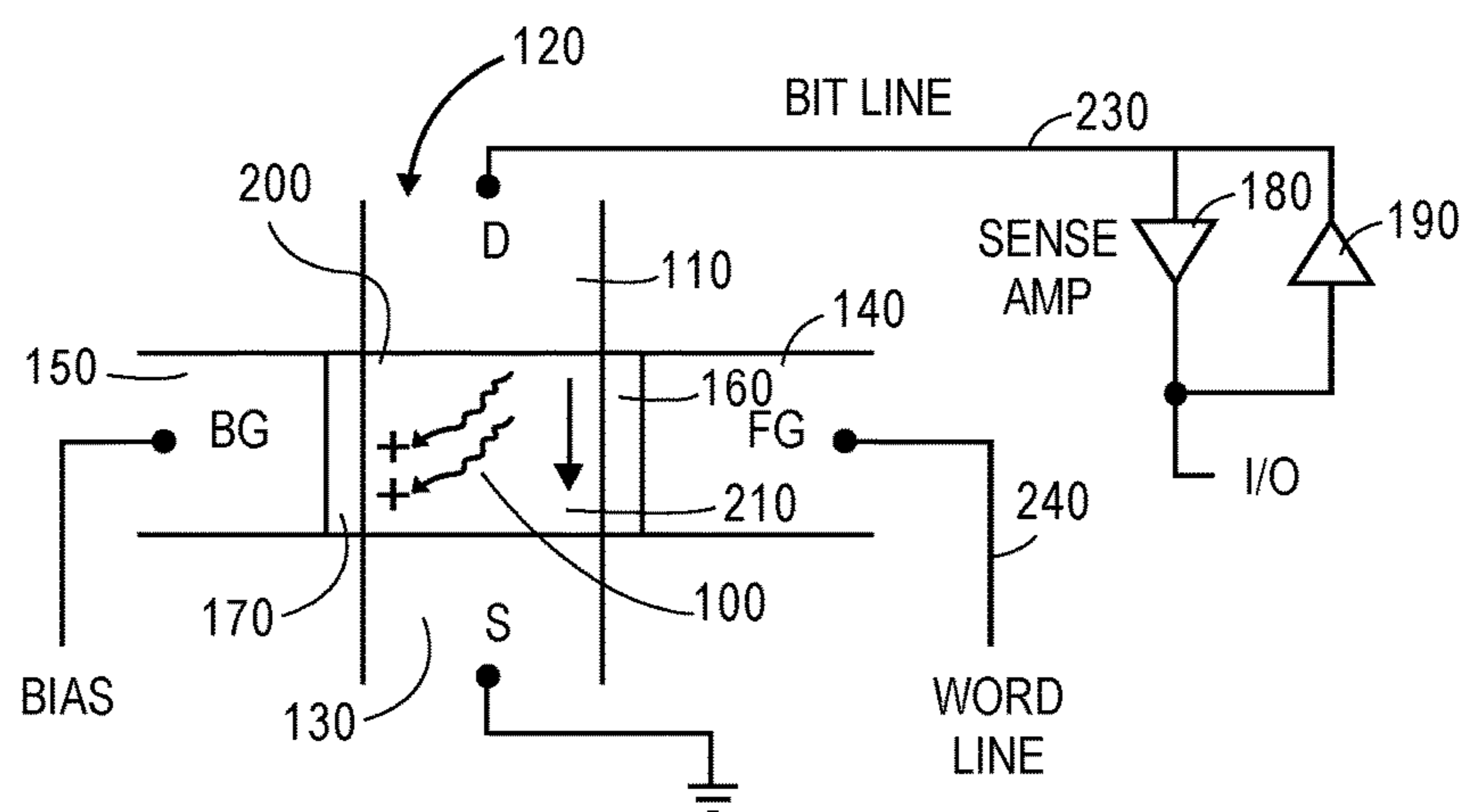
FIG. 1 (PRIOR ART)
