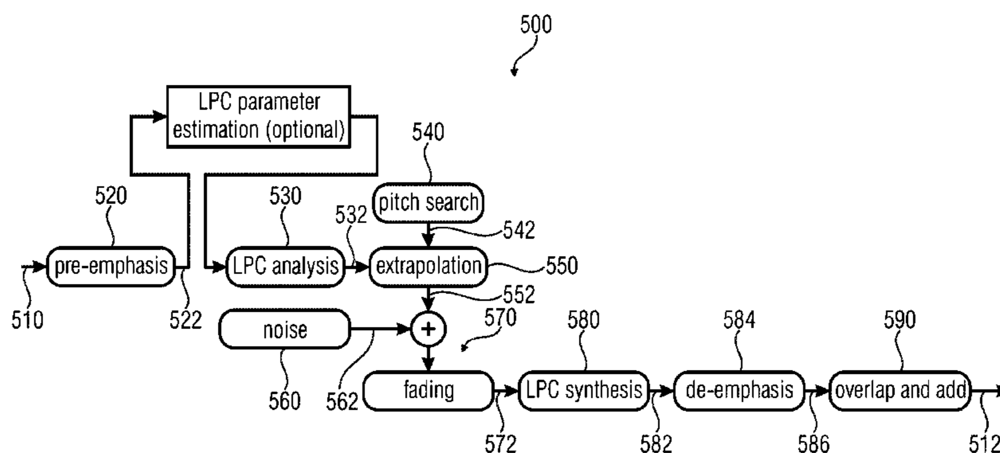
Time domain concealment overview for transform decoder
