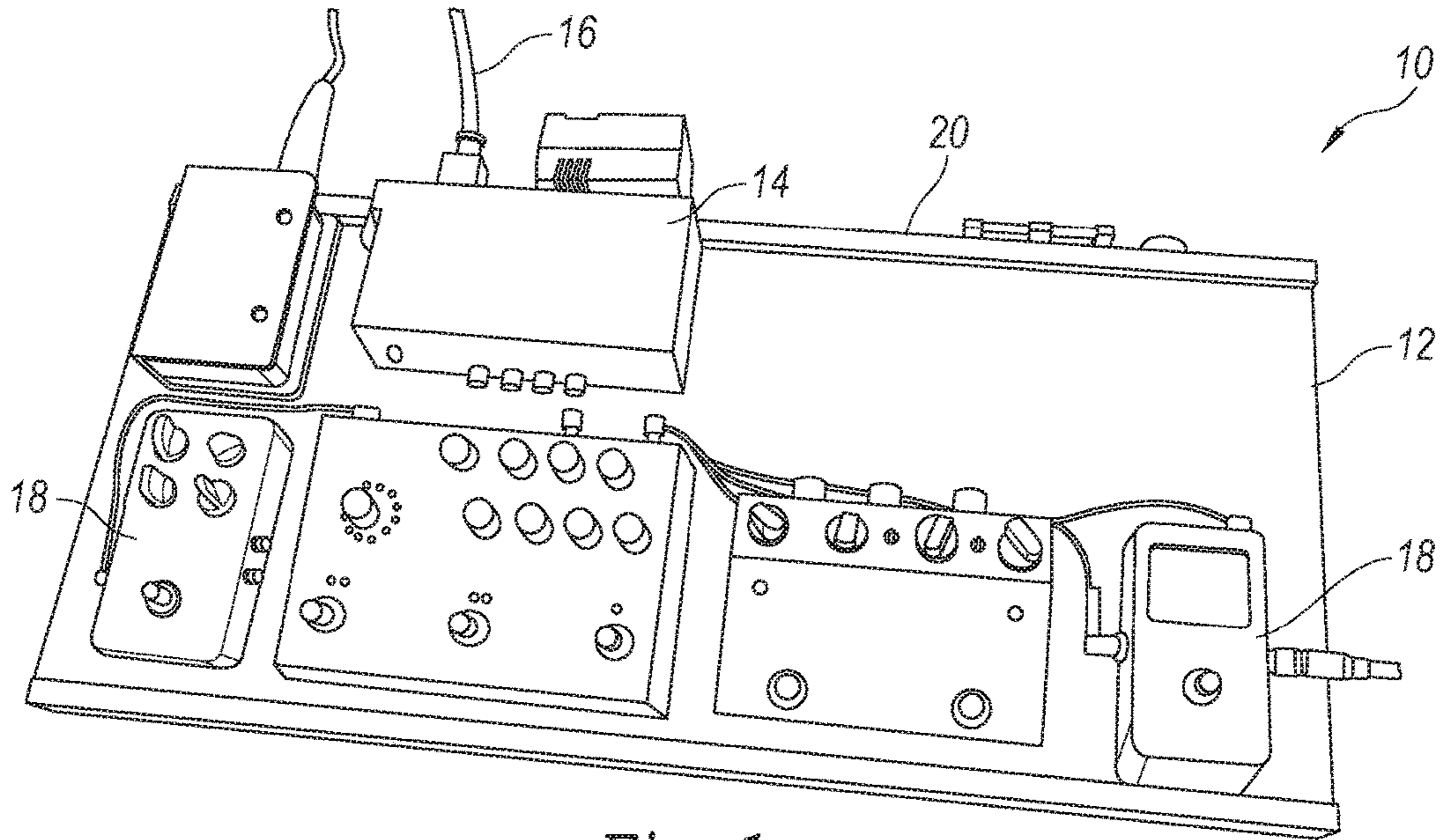
Fig. 1 (Prior Art)
