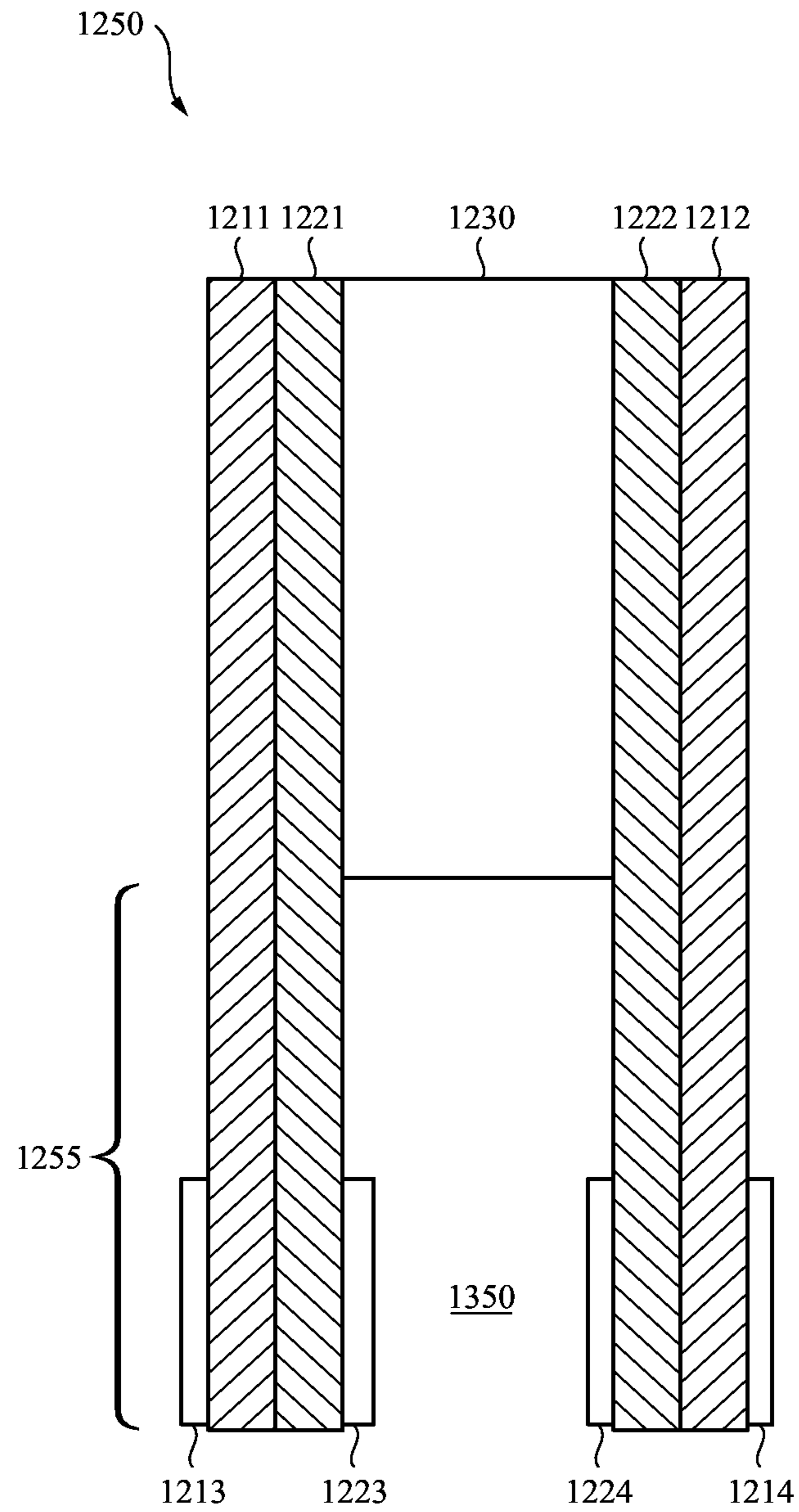
SECTION 3-3 FIG. 13
