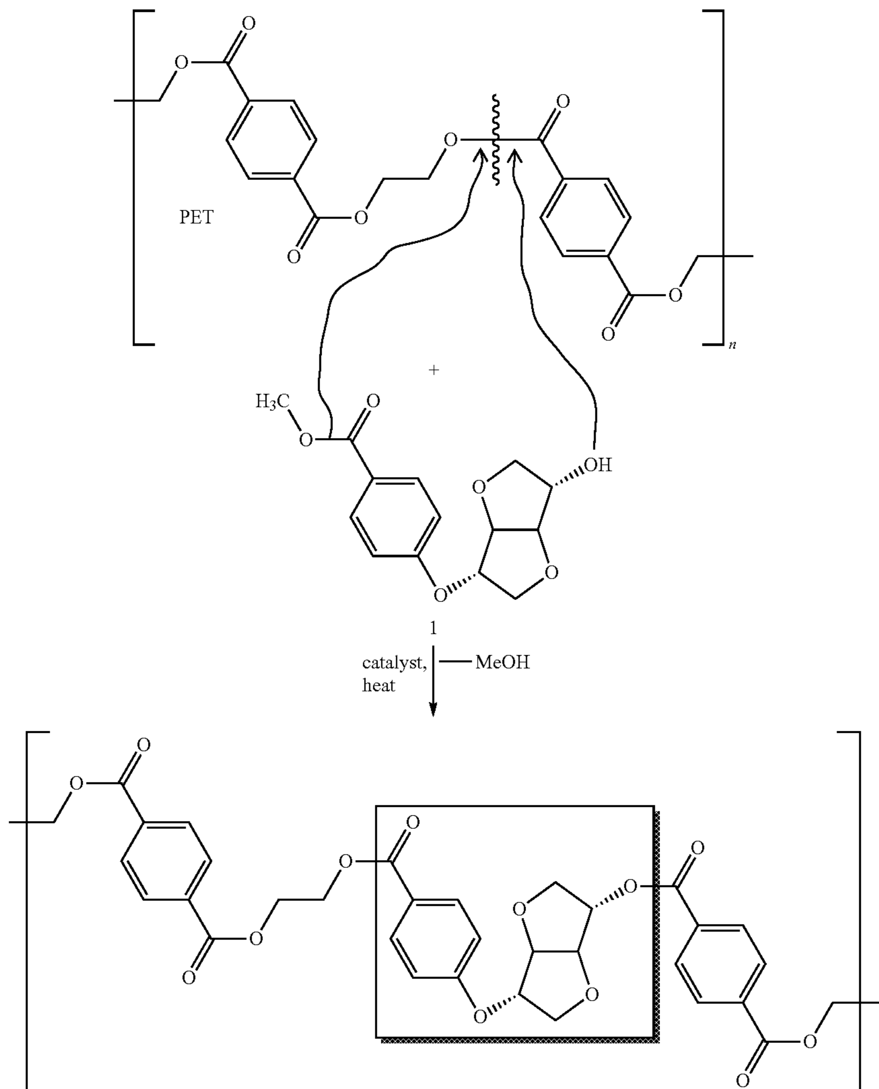
Scheme 3: Incorporation of AB monomer 1 into PET to form novel copolymer.
