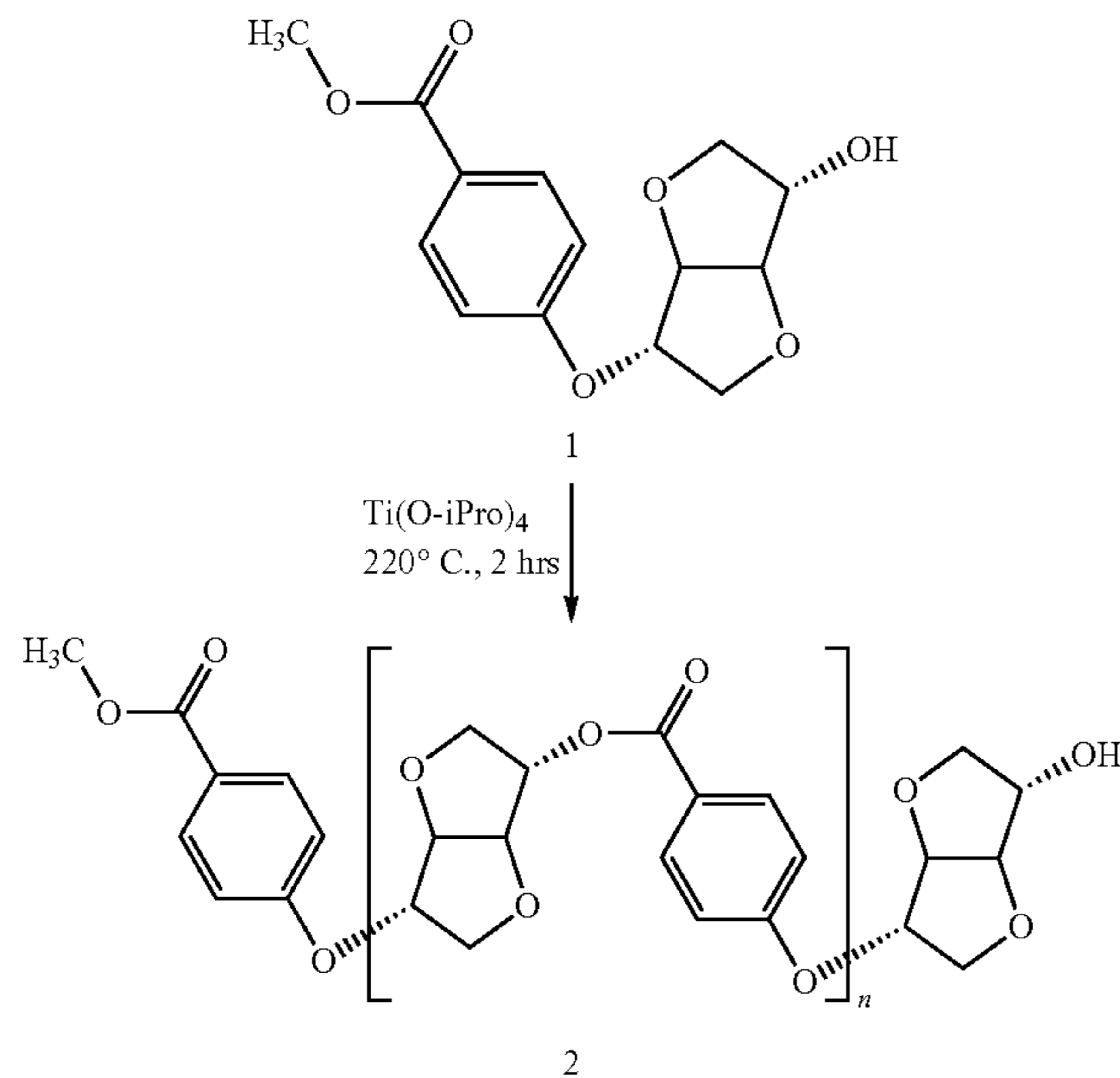
Scheme 2: Polymerization of Isoidide 2-(4-carbomethoxyphenyl) ether (1)
