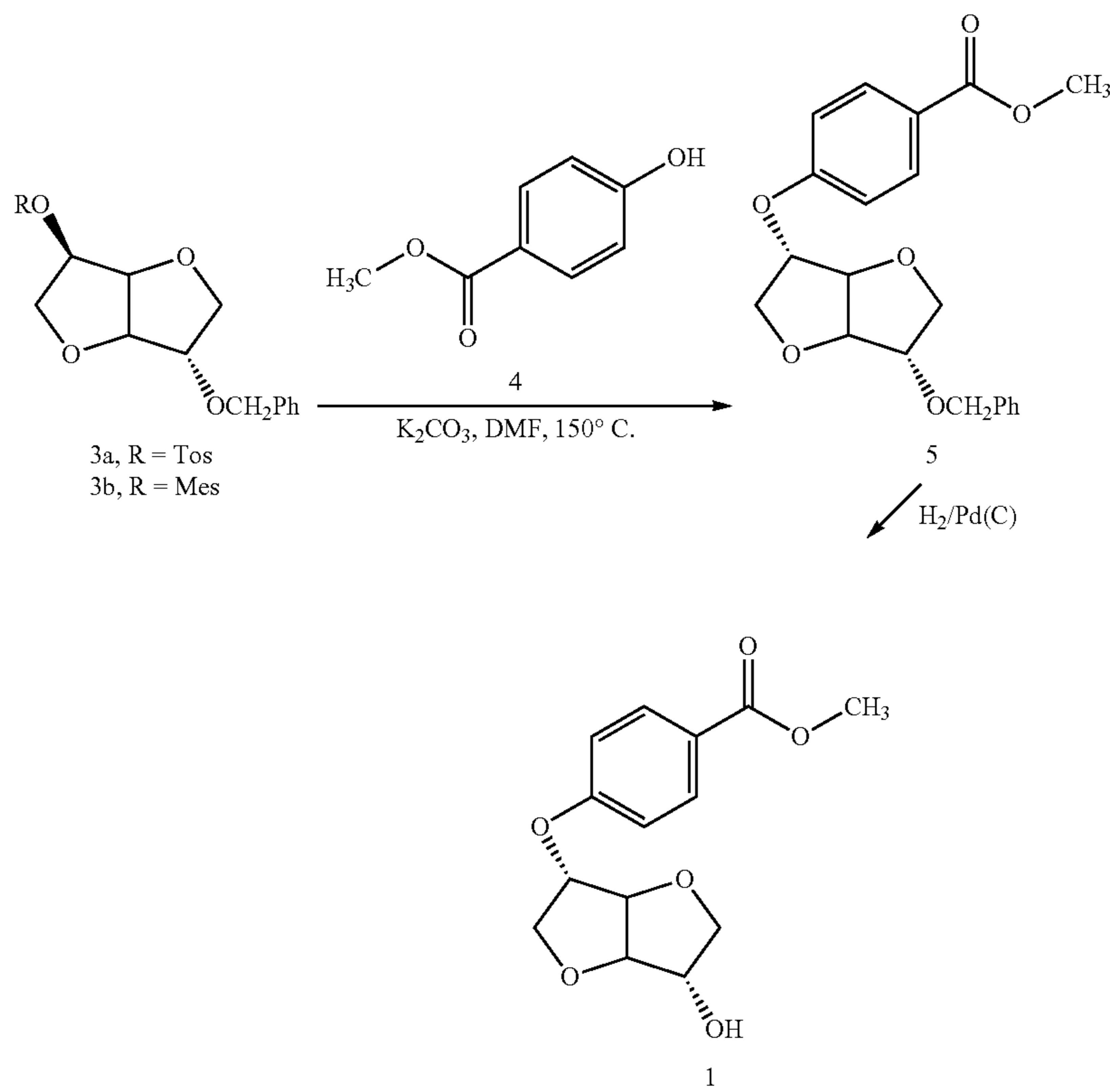
Scheme 1: Isoidide 2-(4-carbomethoxyphenyl) ether (1)
