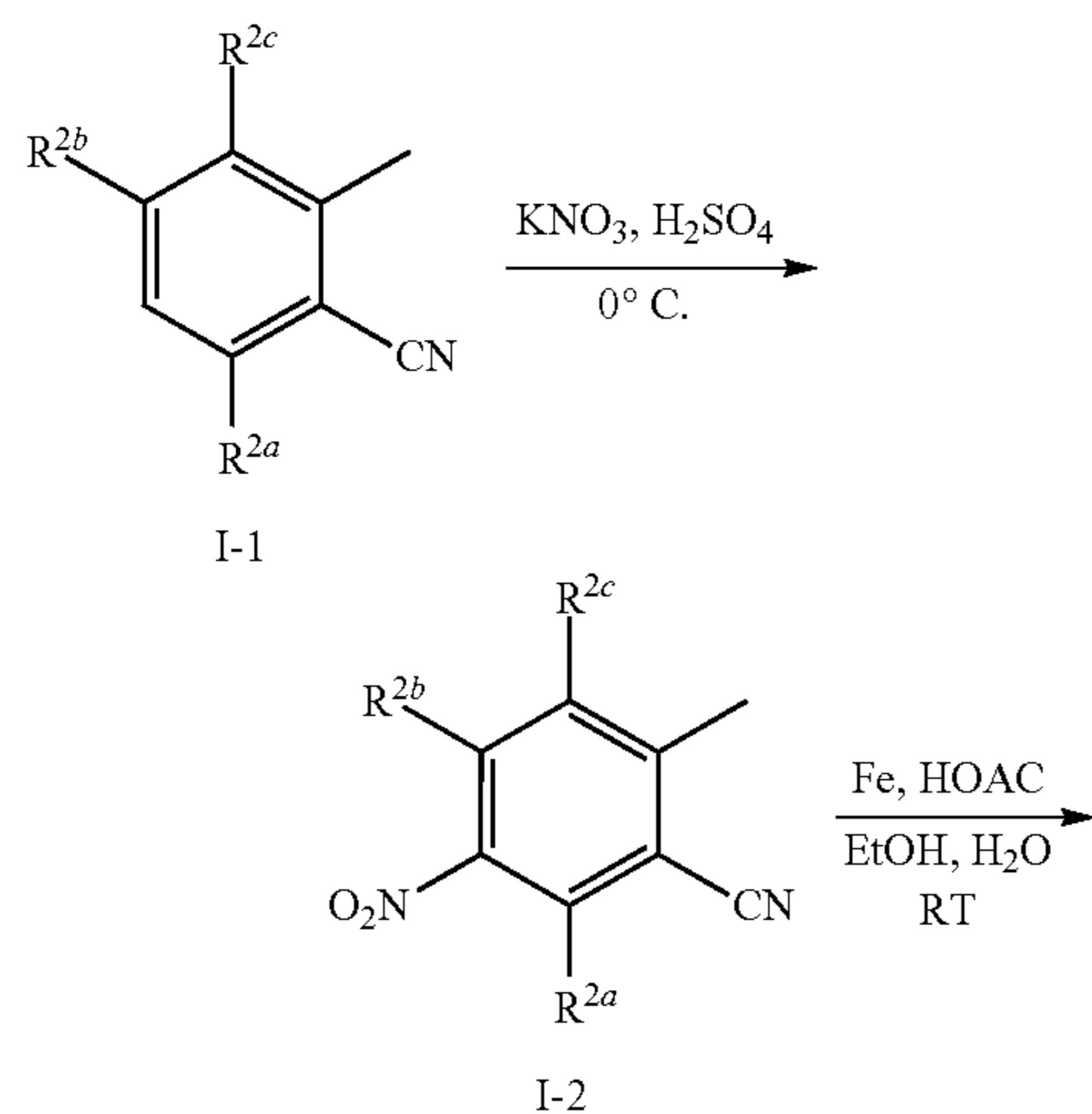
General Reaction Scheme 9
