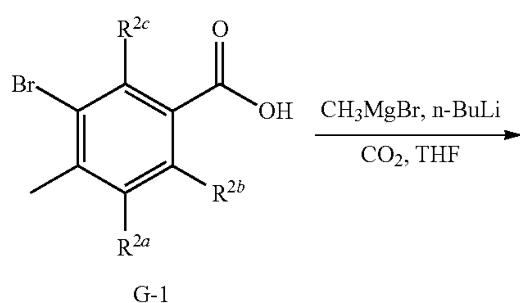
General Reaction Scheme 7
