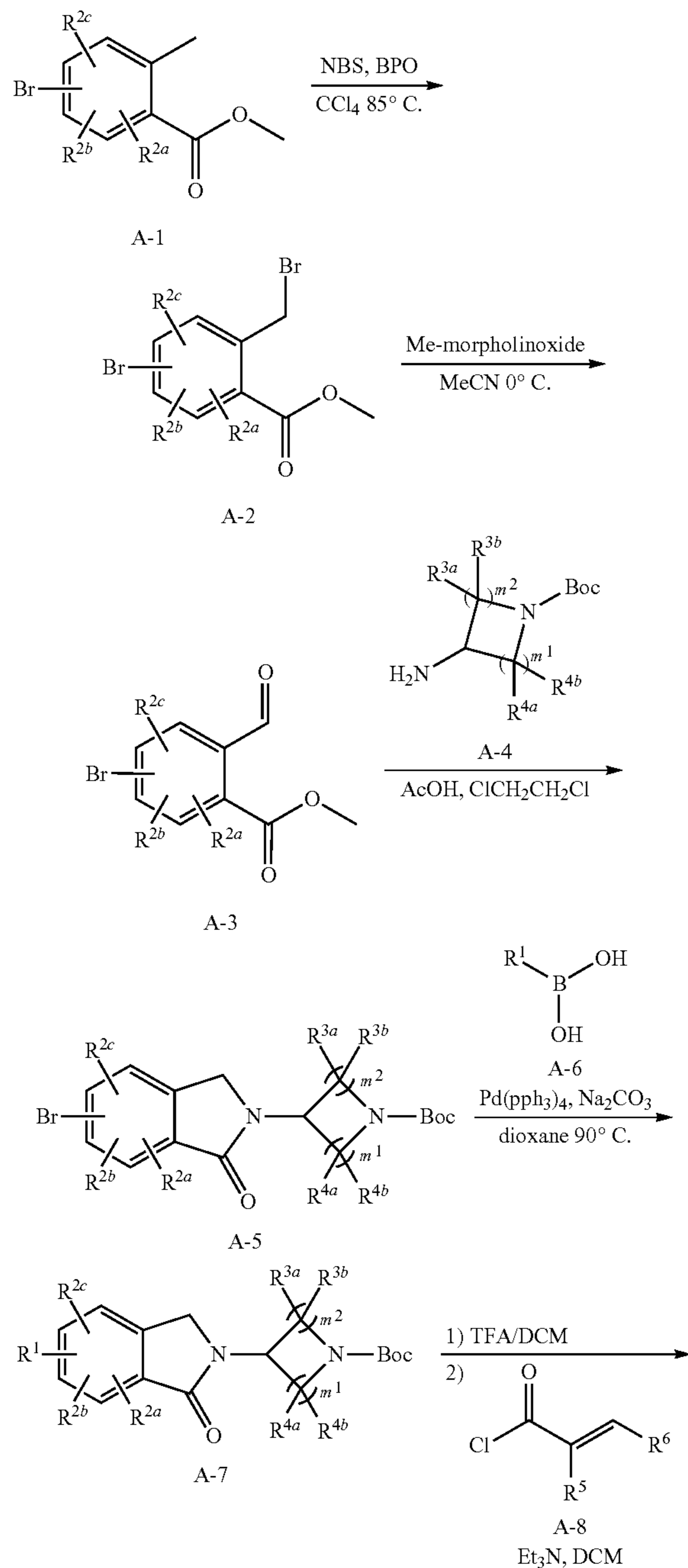
General Reaction Scheme 1
