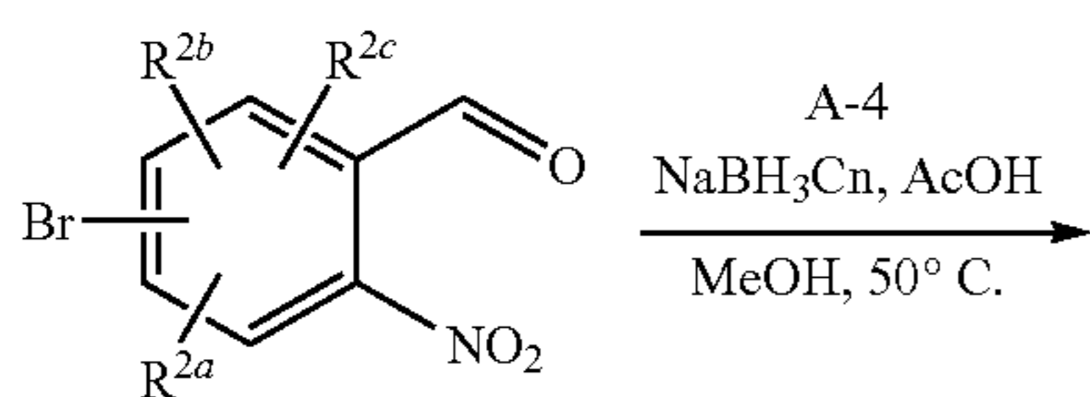
General Reaction Scheme 10
