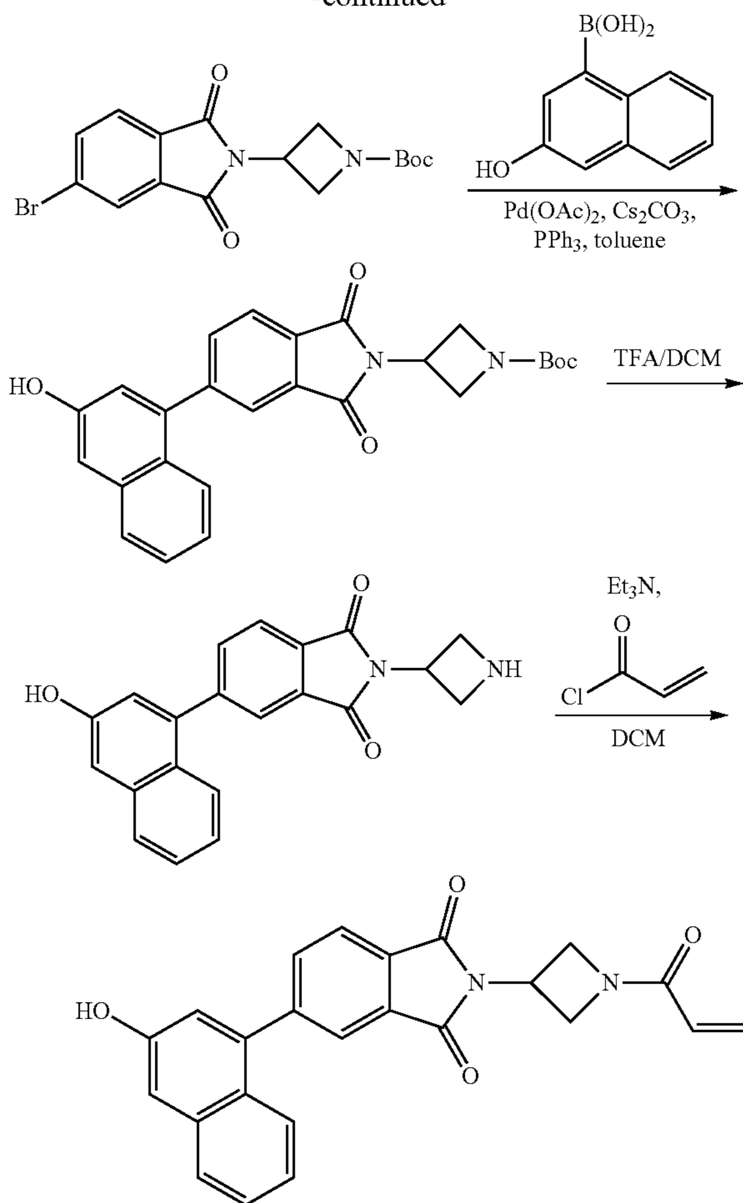
tert-Butyl 3-(5-bromo-1,3-dioxoisindolin-2-yl)azetidine-1-carboxylate
