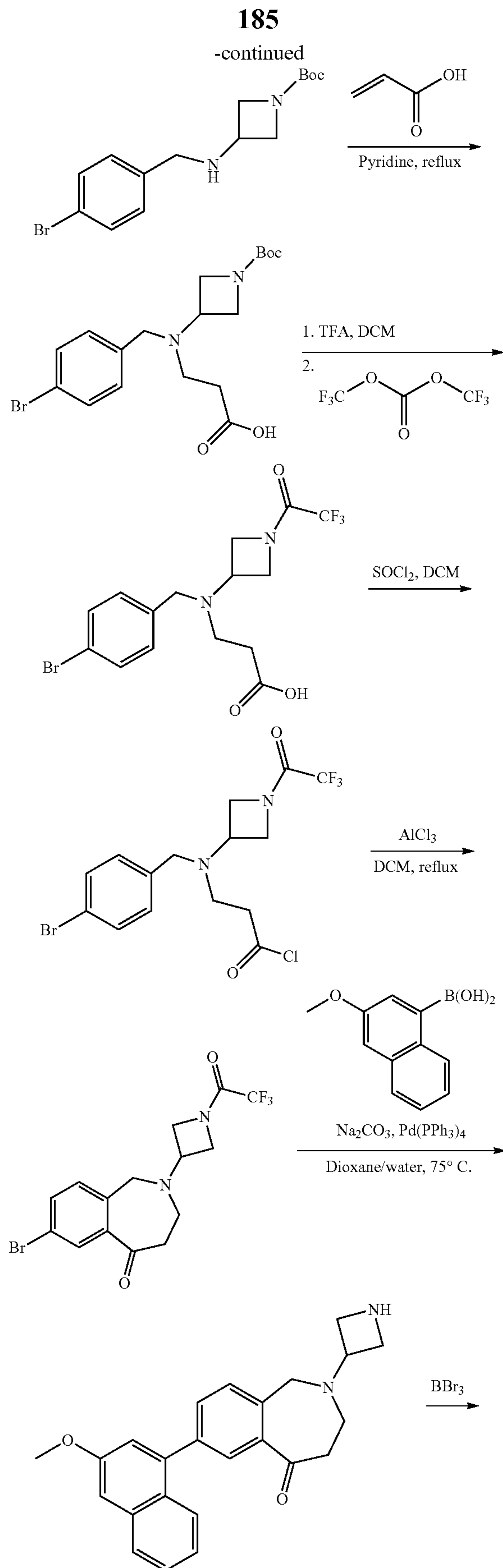
3-((4-Bromobenzyl)(1-(tert-butoxycarbonyl)azetidin-3-yl)amino)propanoic acid
