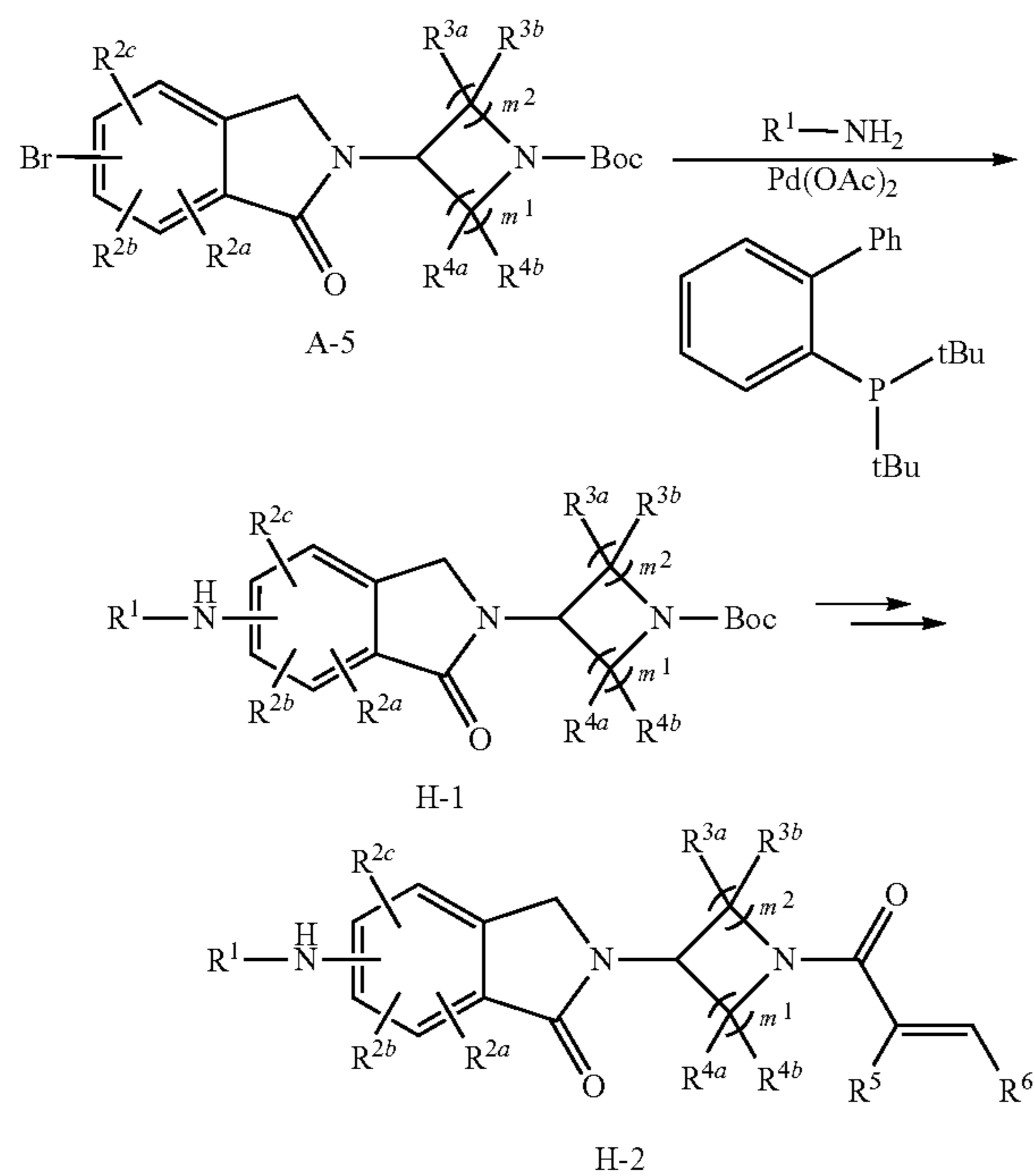
General Reaction Scheme 8
