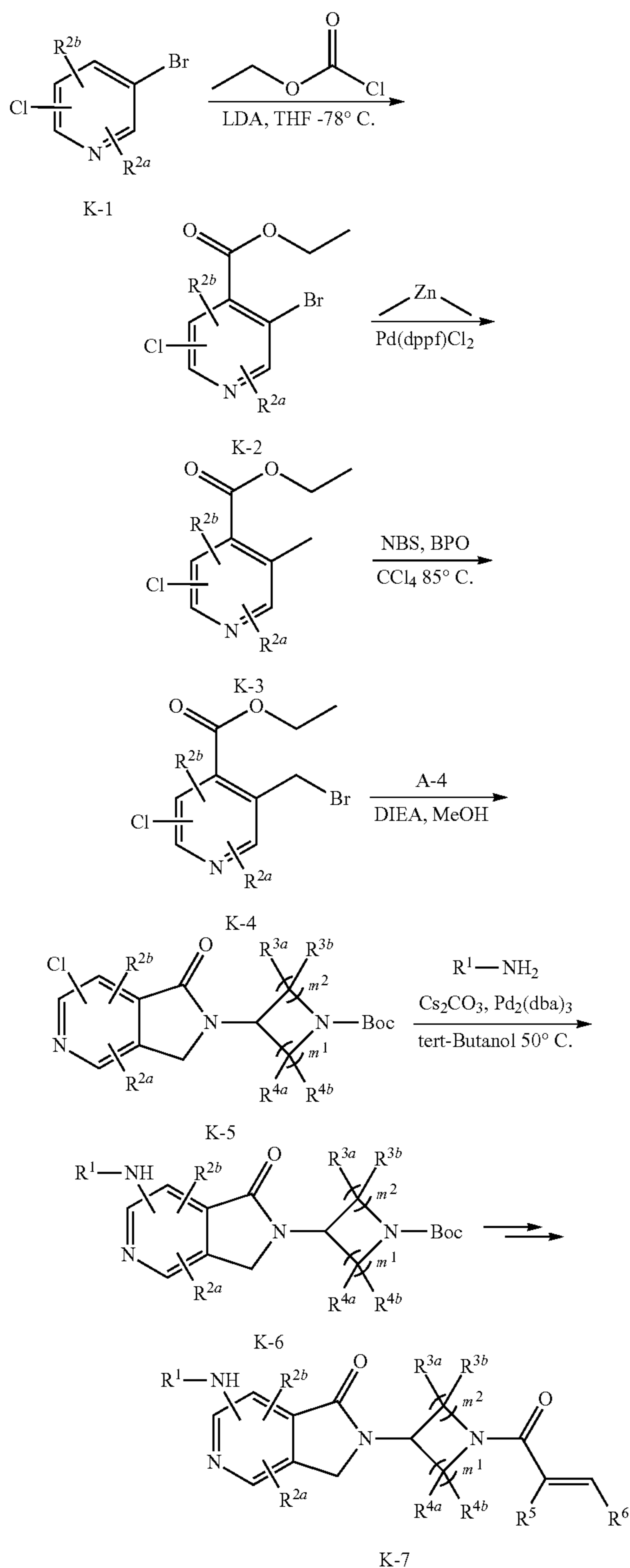
General Reaction Scheme 11
