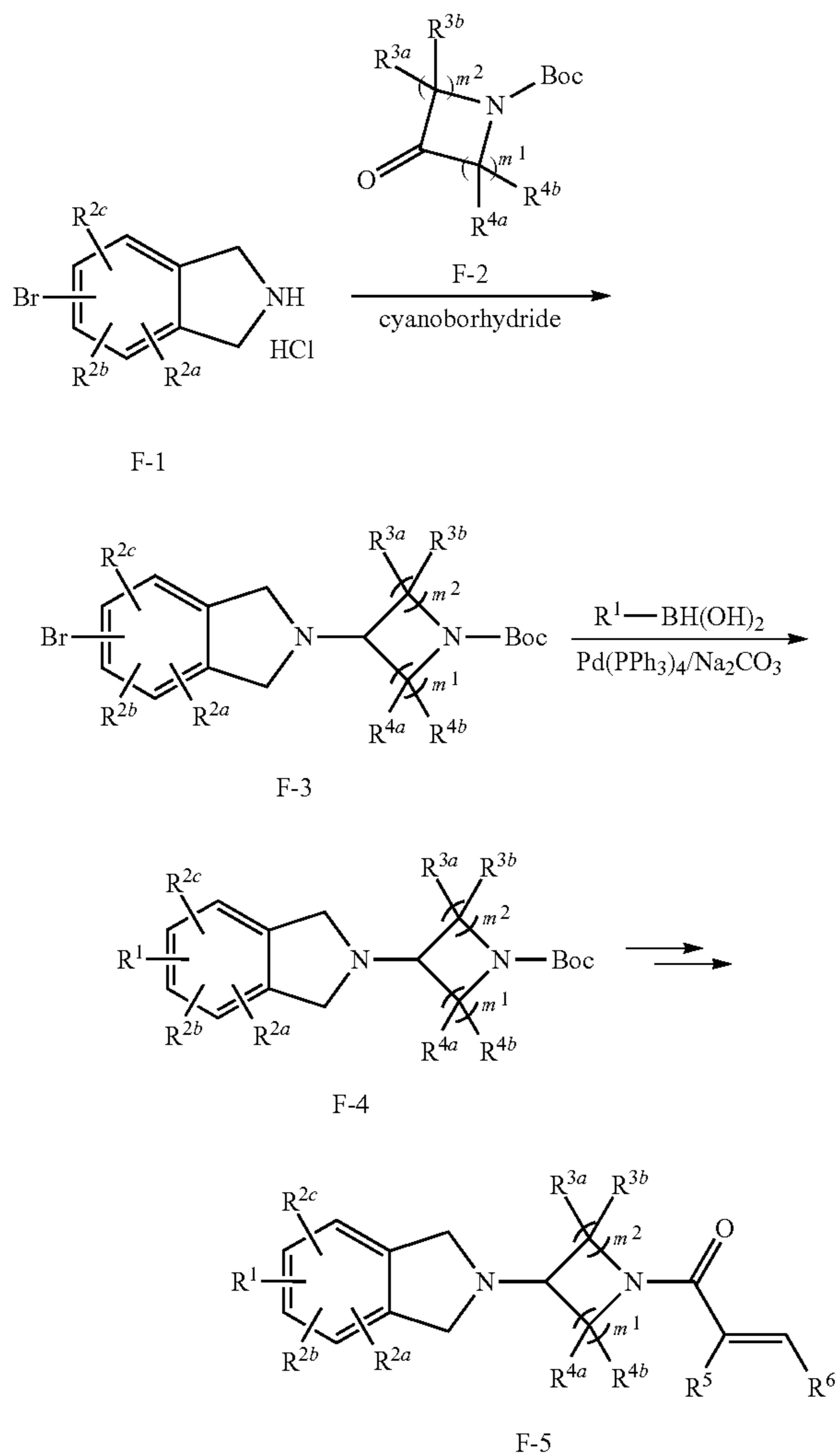
General Reaction Scheme 6
