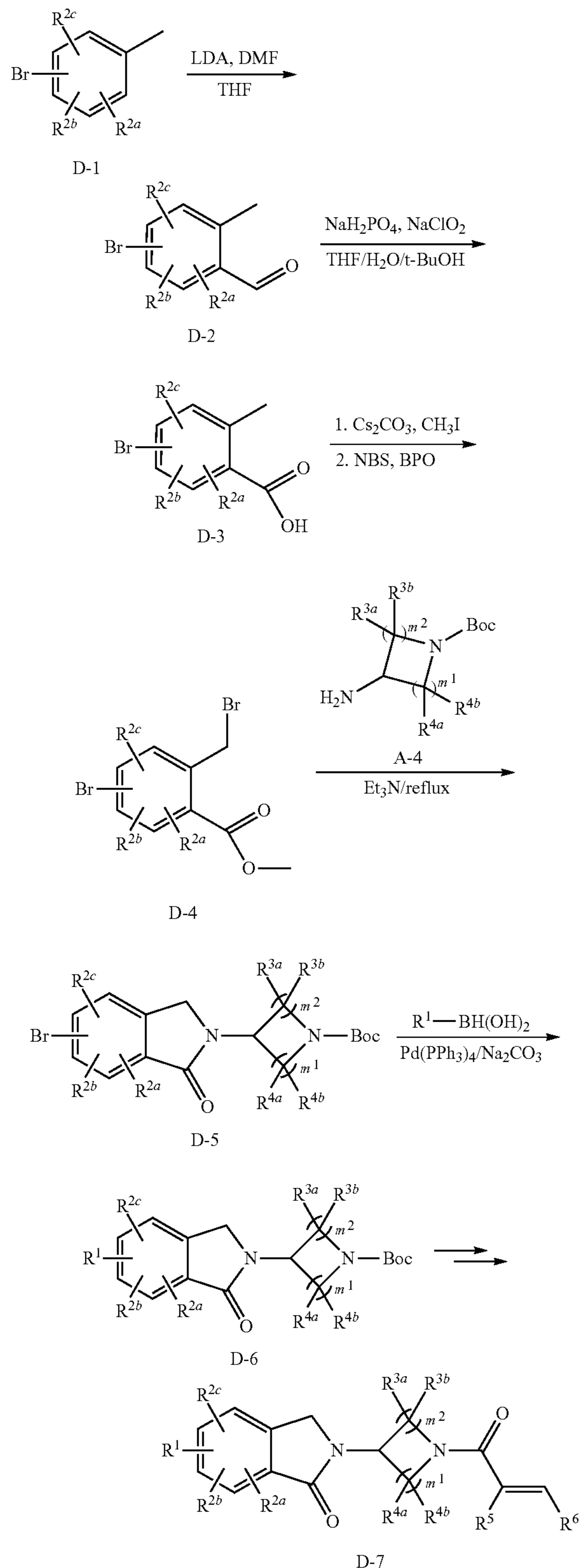
General Reaction Scheme 4
