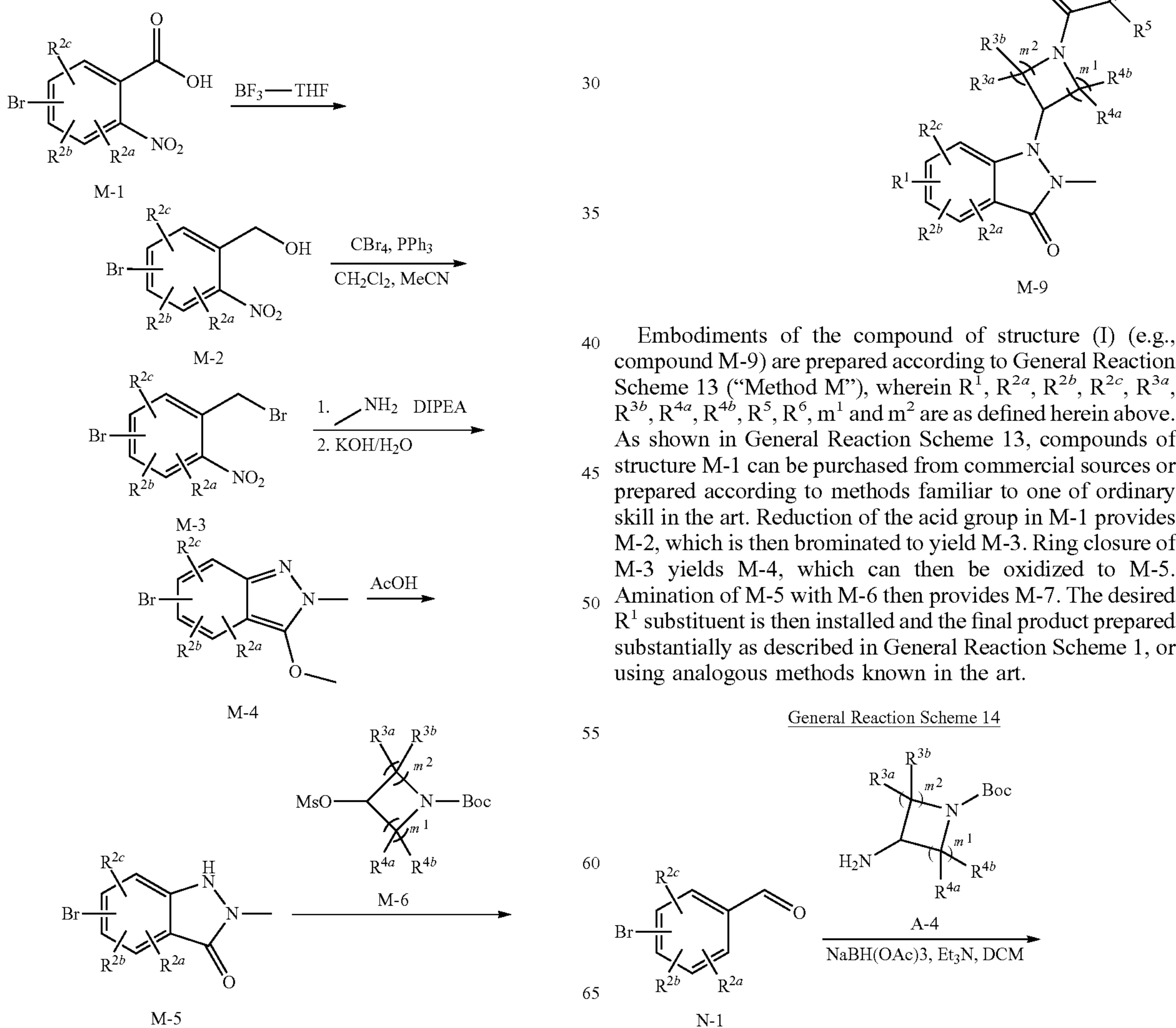
General Reaction Scheme 13
