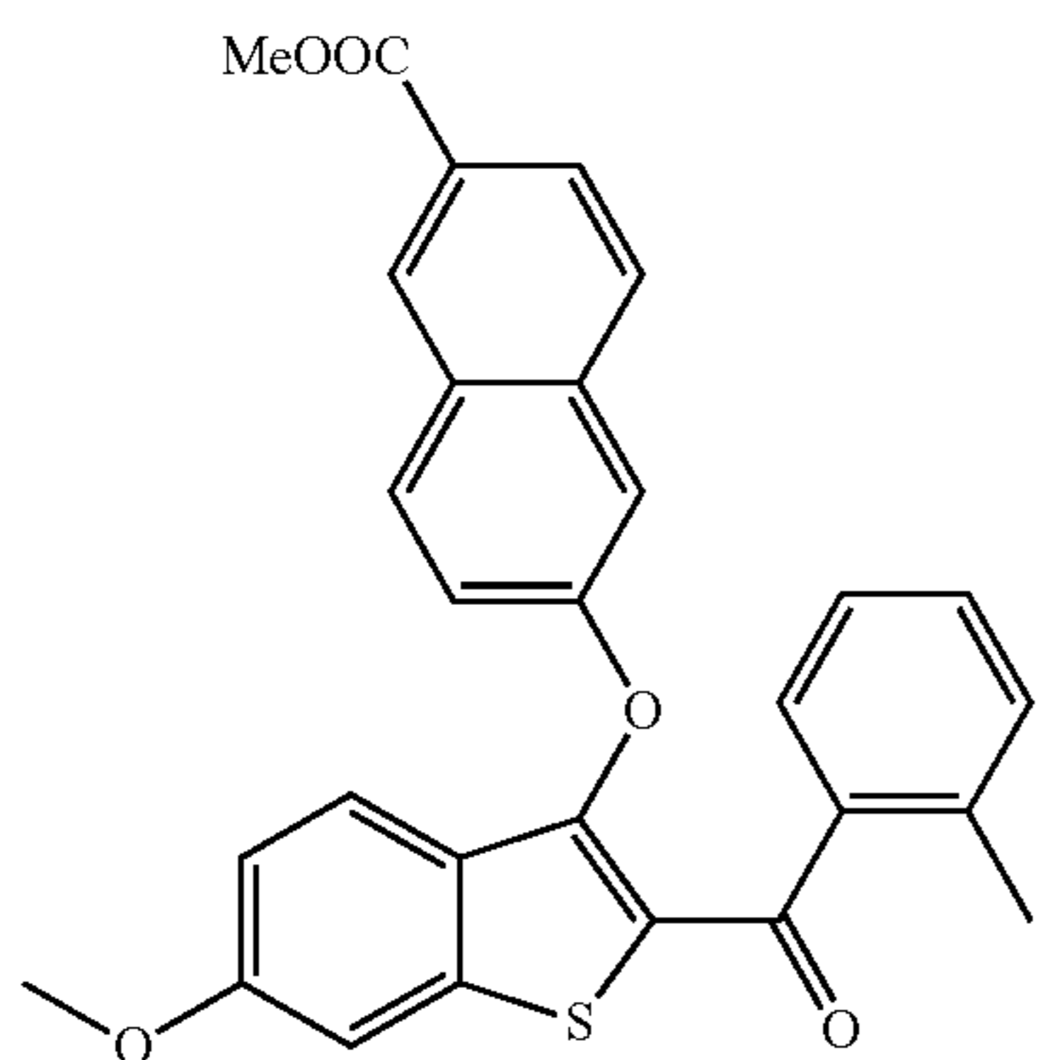
Methyl 6-((6-methoxy-2-(2-methylbenzoyl)benzo[b]thiophen-3-yl)oxy)-2-naphthoate
