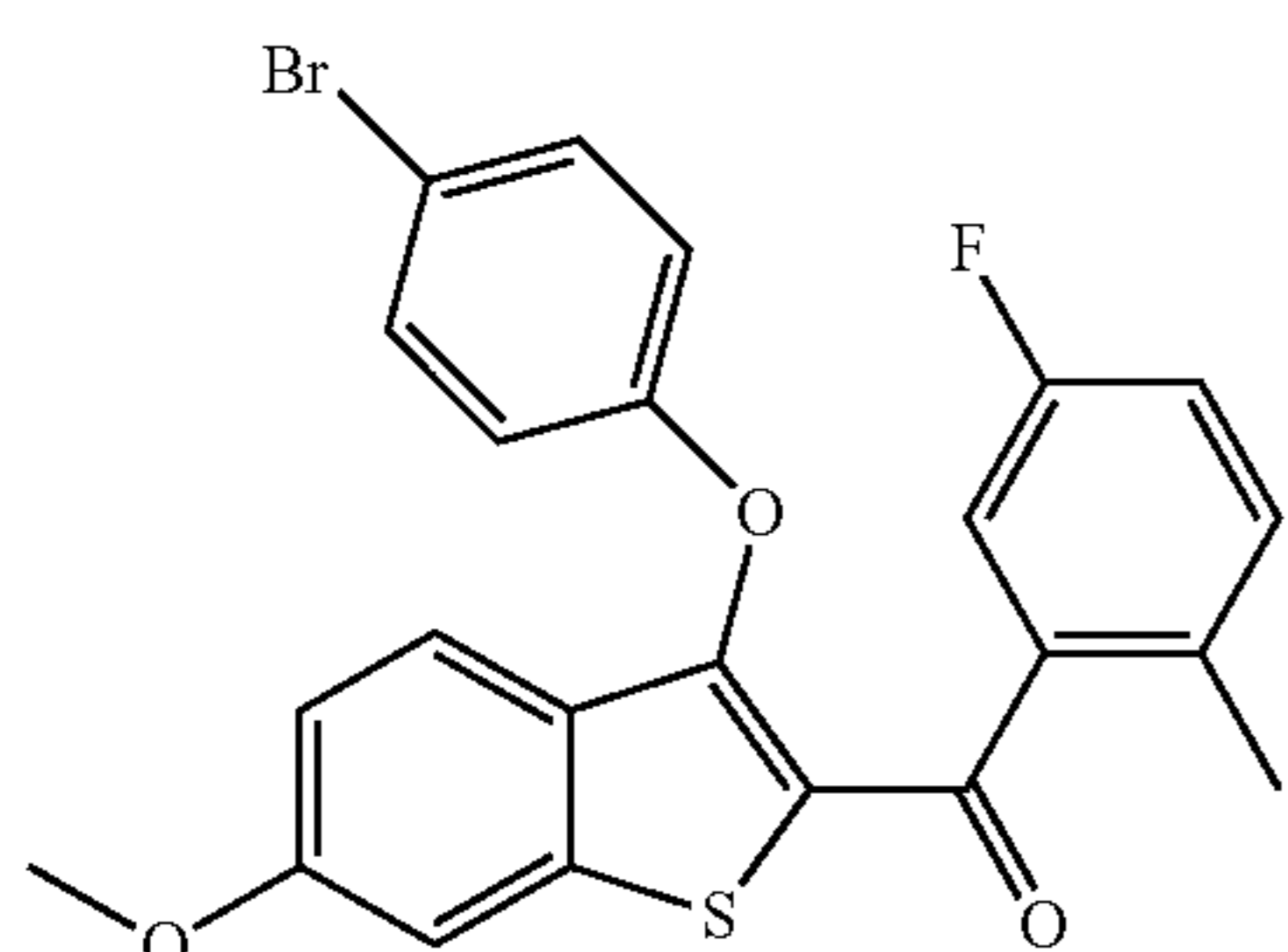
(3-(4-Bromophenoxy)-6-methoxybenzo[b]thiophen-2-yl)(5-fluoro-2-methylphenyl)methanone
