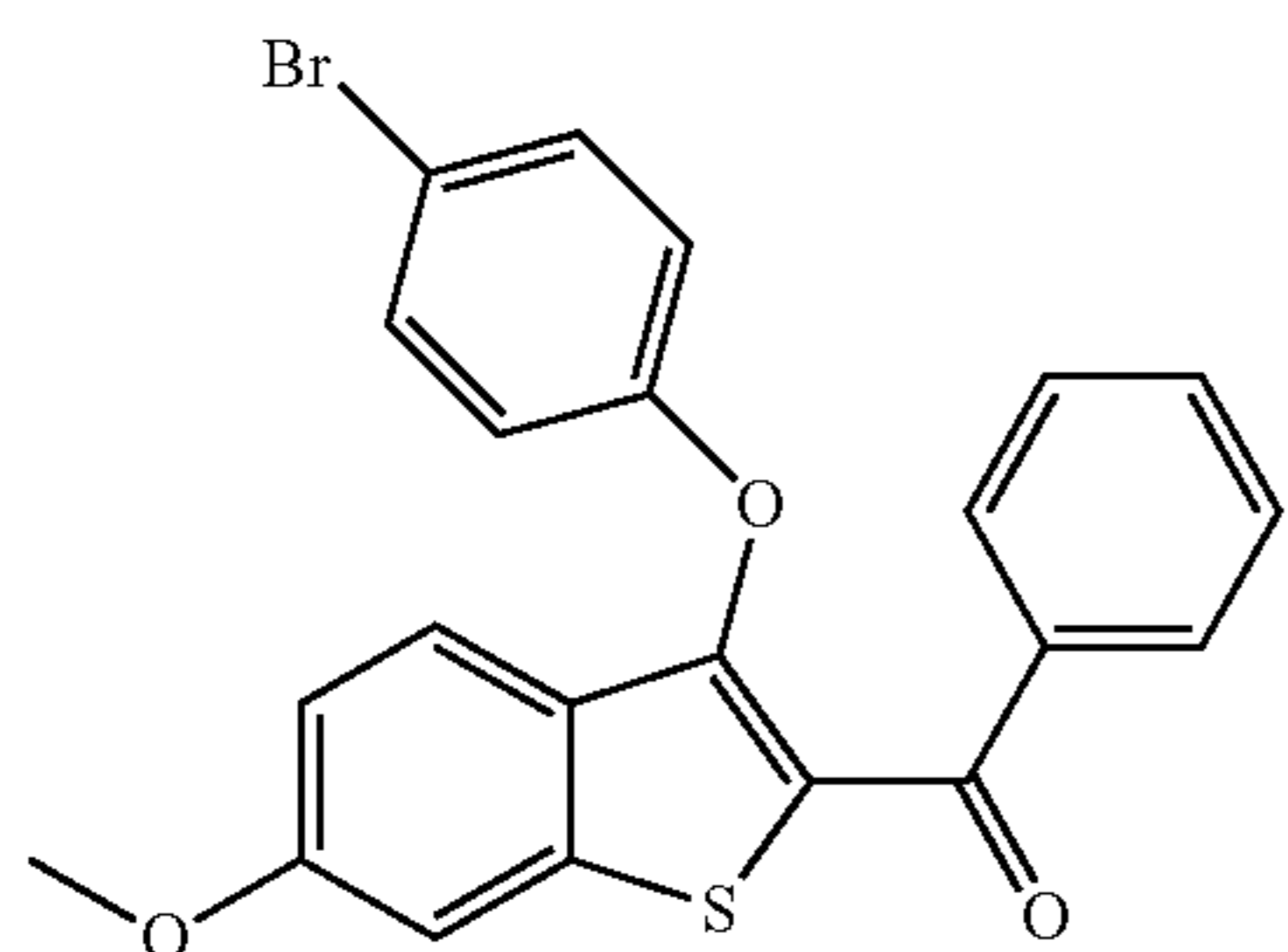
(3-(4-Bromophenoxy)-6-methoxybenzo[b]thiophen-2-yl)(phenyl)methanone
