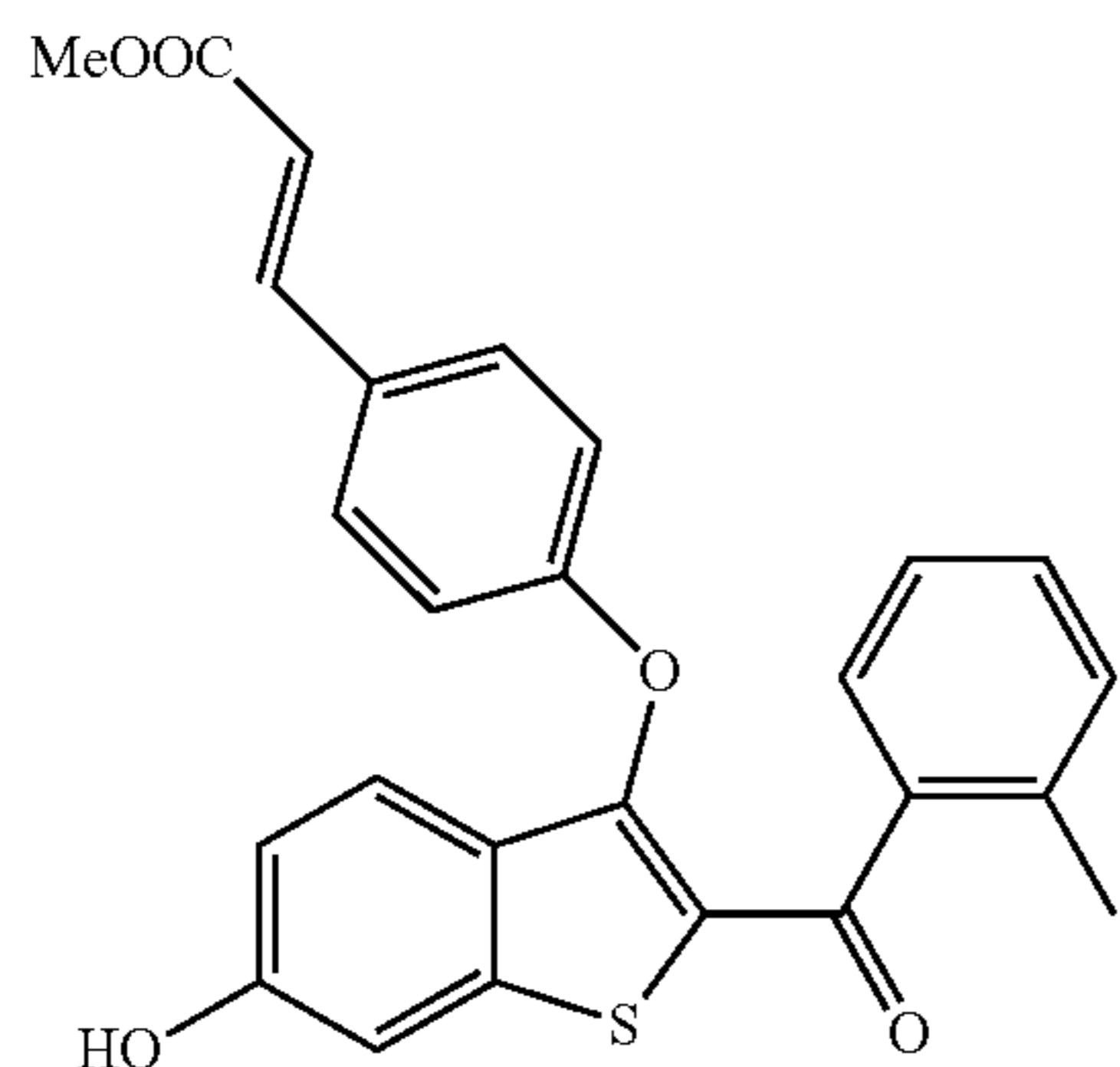
Methyl (E)-3-(4-((6-hydroxy-2-(2-methylbenzoyl)benzo[b]thiophen-3-yl)oxy)phenyl)acrylate
