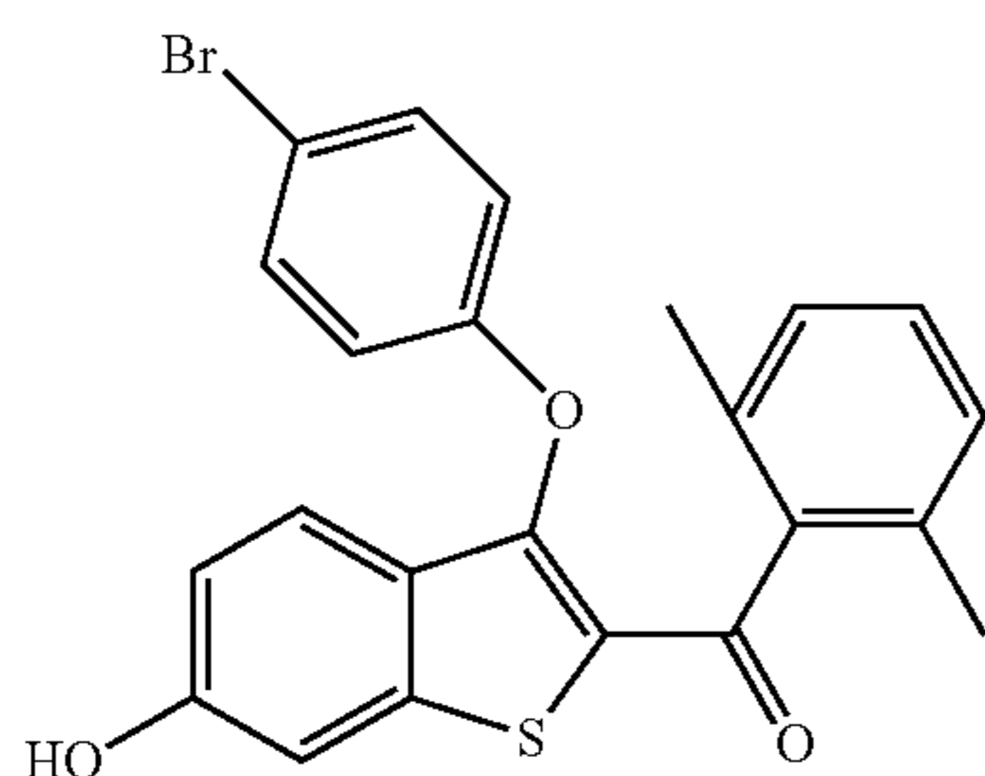
(3-(4-Bromophenoxy)-6-hydroxybenzo[b]thiophen-2-yl)(2,6-dimethylphenyl)methanone
