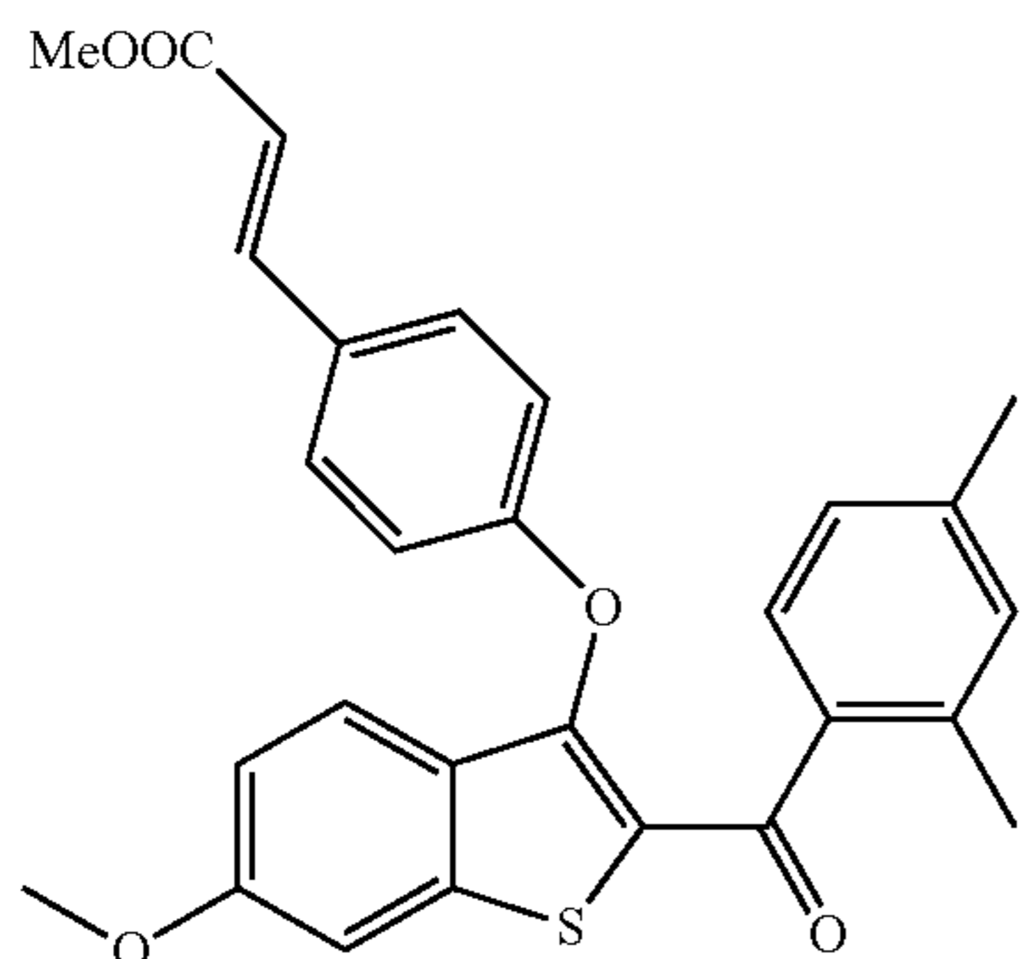
Methyl (E)-3-(4-((2-(2,4-dimethylbenzoyl)-6-methoxybenzo[b]thiophen-3-yl)oxy)phenyl)acrylate
