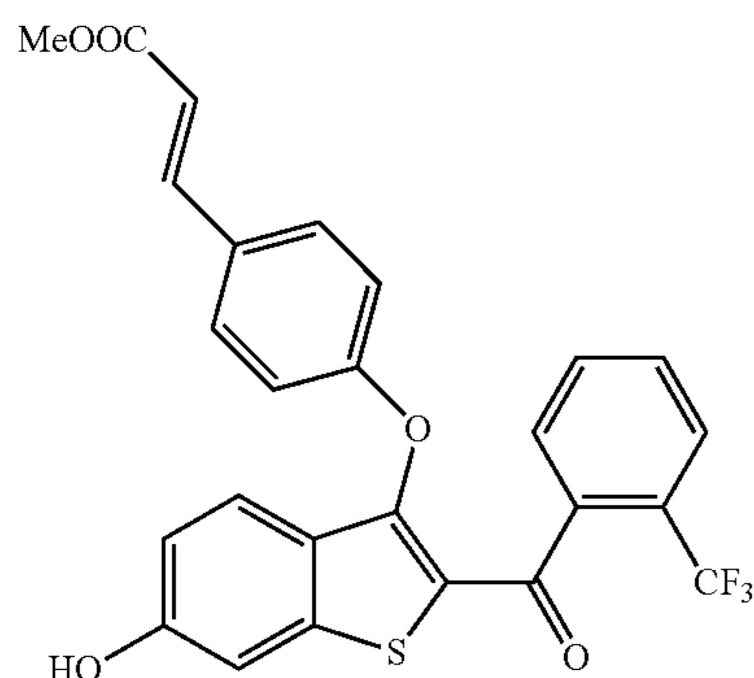
Methyl (E)-3-(4-((6-hydroxy-2-(2-(trifluoromethyl)benzoyl)benzo[b]thiophen-3-yl)oxy)phenyl)acrylate
