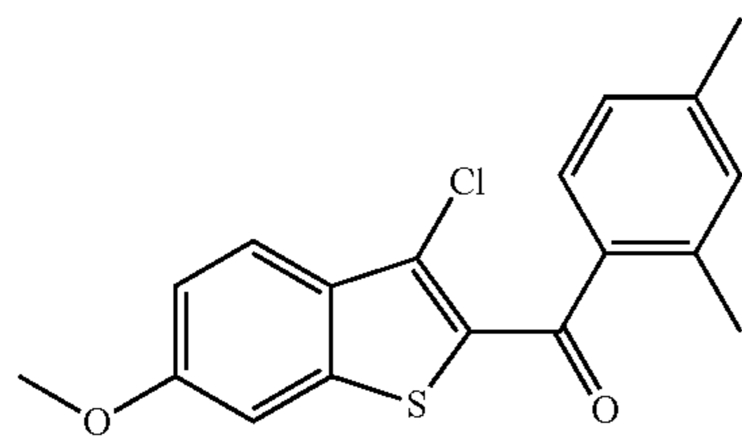
(3-chloro-6-methoxybenzo[b]thiophen-2-yl)(2,4-dimethylphenyl)methanone
