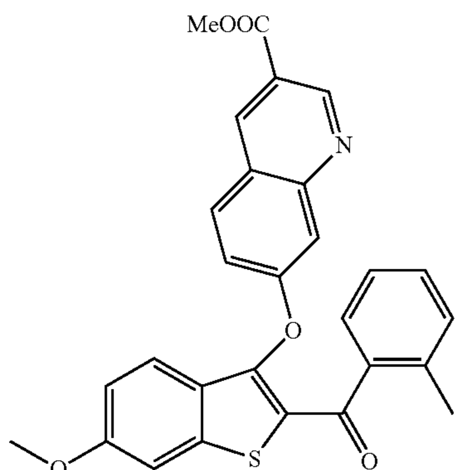
Methyl 7-((6-methoxy-2-(2-methylbenzoyl)benzo[b]thiophen-3-yl)oxy)quinoline-3-carboxylate
