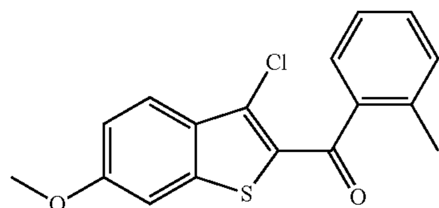
(3-chloro-6-methoxybenzo[b]thiophen-2-yl)(o-tolyl)methanone
