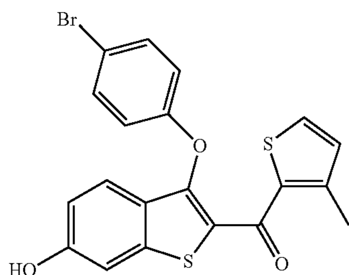
(3-(4-Bromophenoxy)-6-hydroxybenzo[b]thiophen-2-yl)(3-methylthiophen-2-yl)methanone
