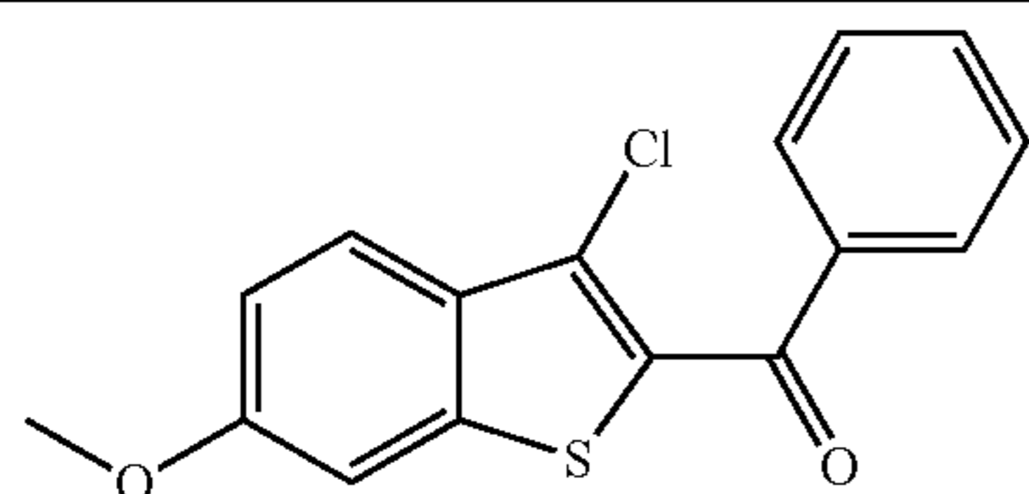
(3-chloro-6-methoxybenzo[b]thiophen-2-yl)(phenyl)methanone
