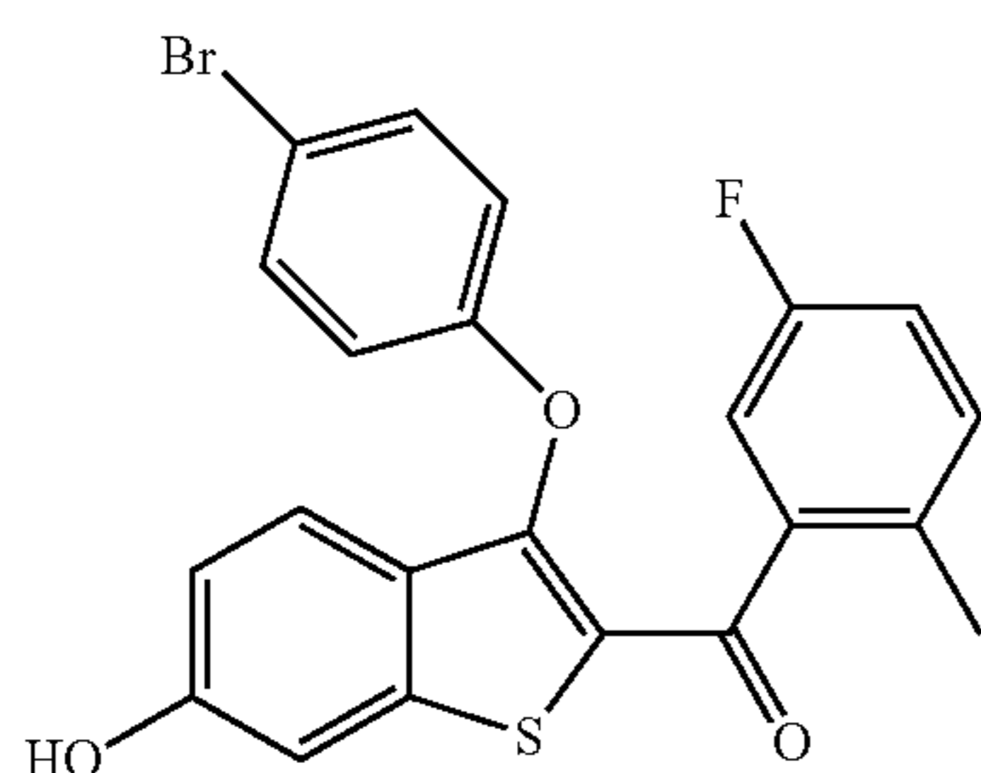
(3-(4-Bromophenoxy)-6-hydroxybenzo[b]thiophen-2-yl)(5-fluoro-2-methylphenyl)methanone
