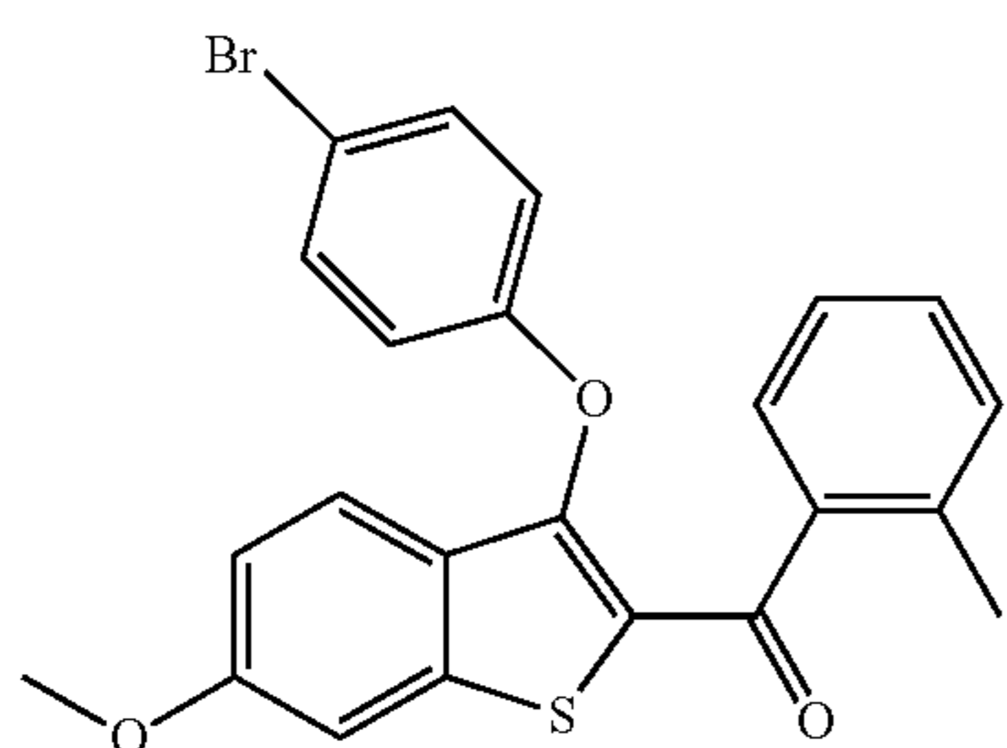
(3-(4-Bromophenoxy)-6-methoxybenzo[b]thiophen-2-yl)(o-tolyl)methanone
