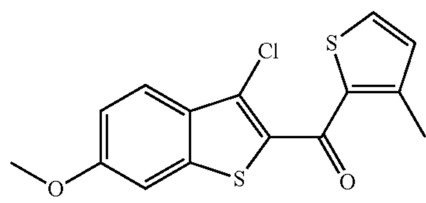
(3-chloro-6-methoxybenzo[b]thiophen-2-yl)(3-methylthiophen-2-yl)methanone
