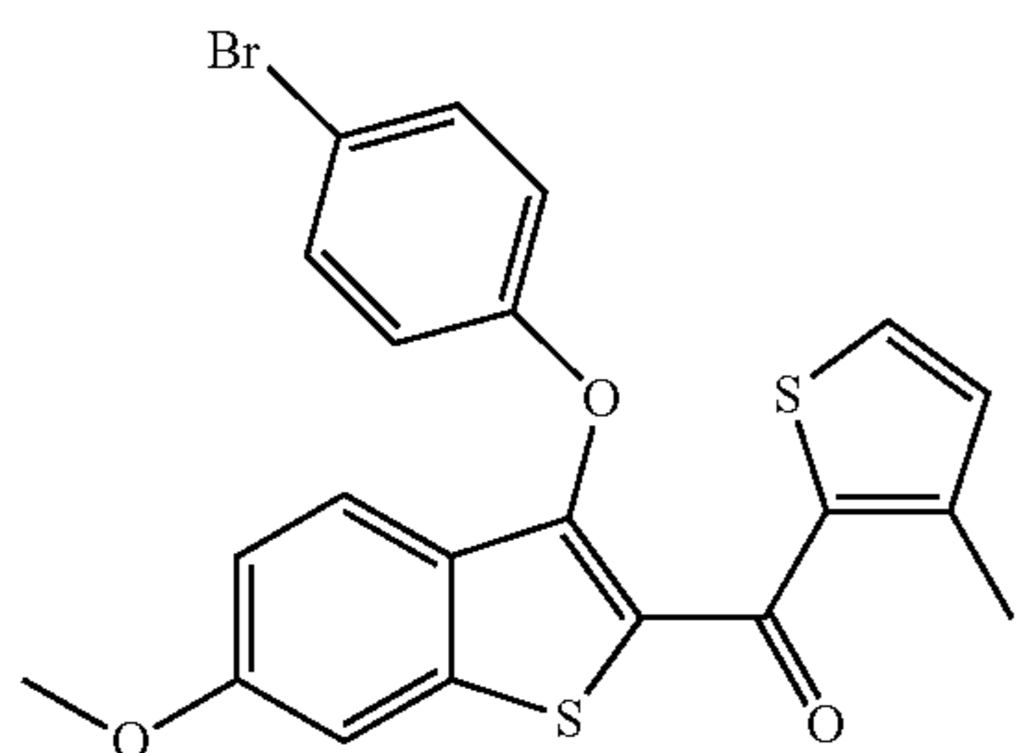
(3-(4-Bromophenoxy)-6-methoxybenzo[b]thiophen-2-yl)(3-methylthiophen-2-yl)methanone
