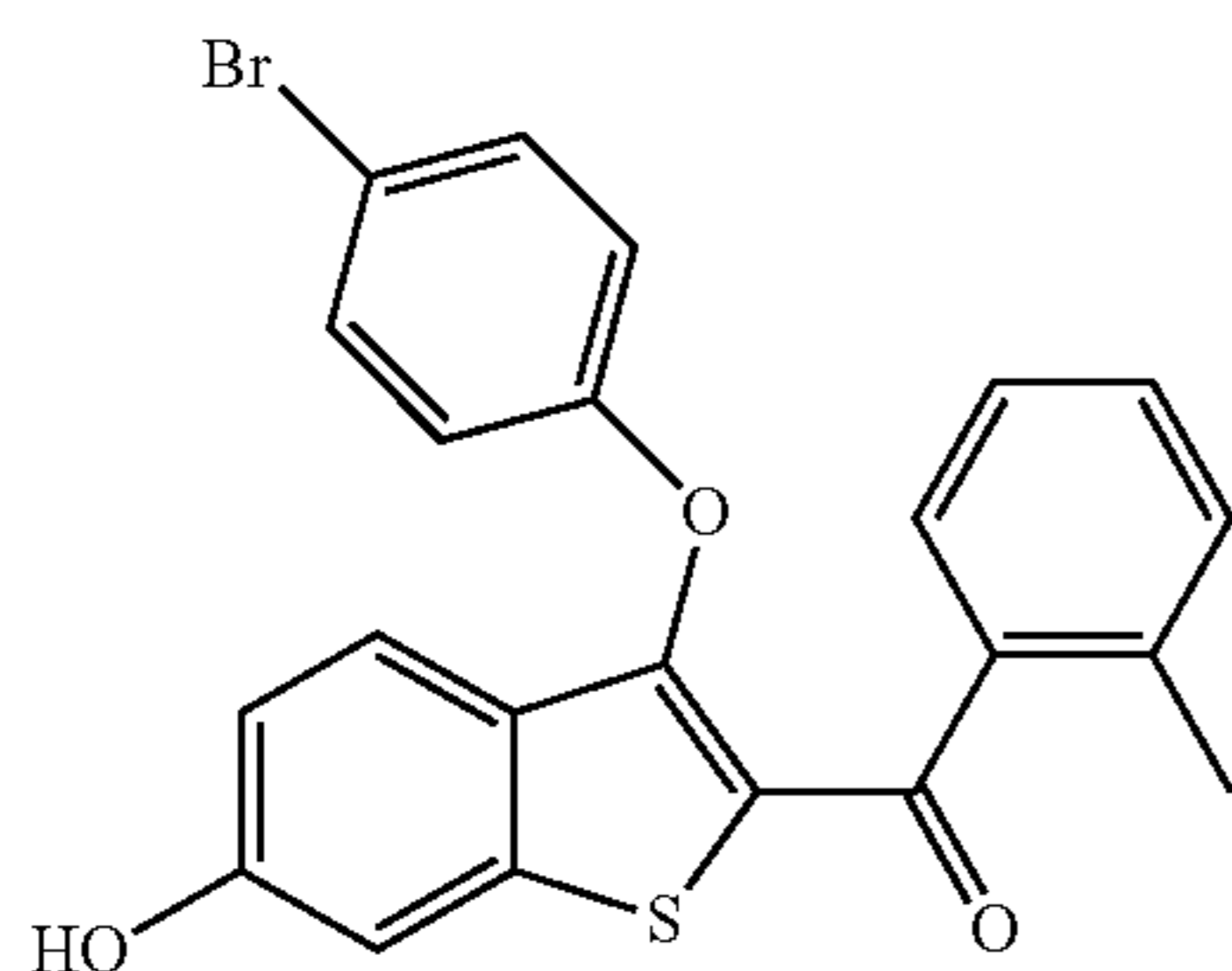
(3-(4-Bromophenoxy)-6-hydroxybenzo[b]thiophen-2-yl)(o-tolyl)methanone
