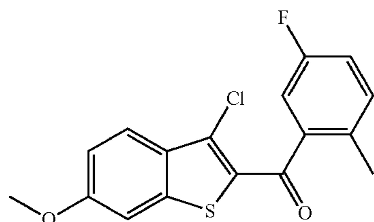
(3-chloro-6-methoxybenzo[b]thiophen-2-yl)(5-fluoro-2-methylphenyl)methanone
