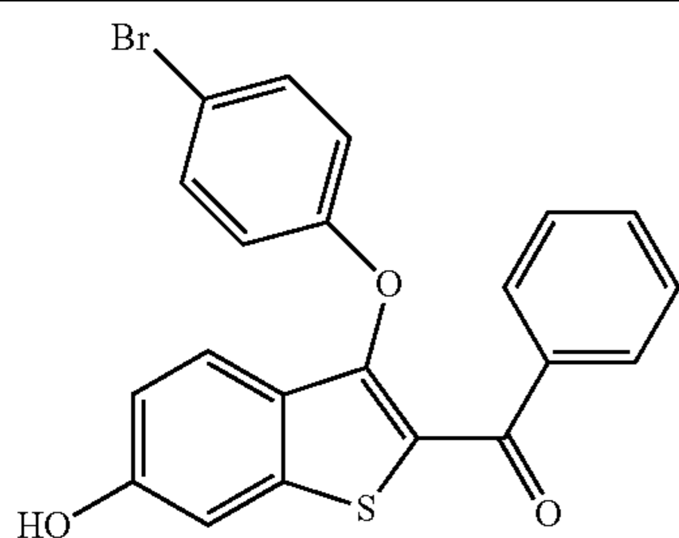
(3-(4-Bromophenoxy)-6-hydroxybenzo[b]thiophen-2-yl)(phenyl)methanone
