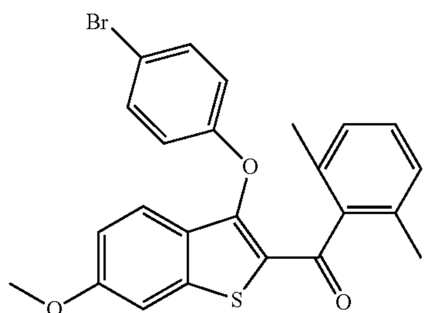
(3-(4-Bromophenoxy)-6-methoxybenzo[b]thiophen-2-yl)(2,6-dimethylphenyl)methanone
