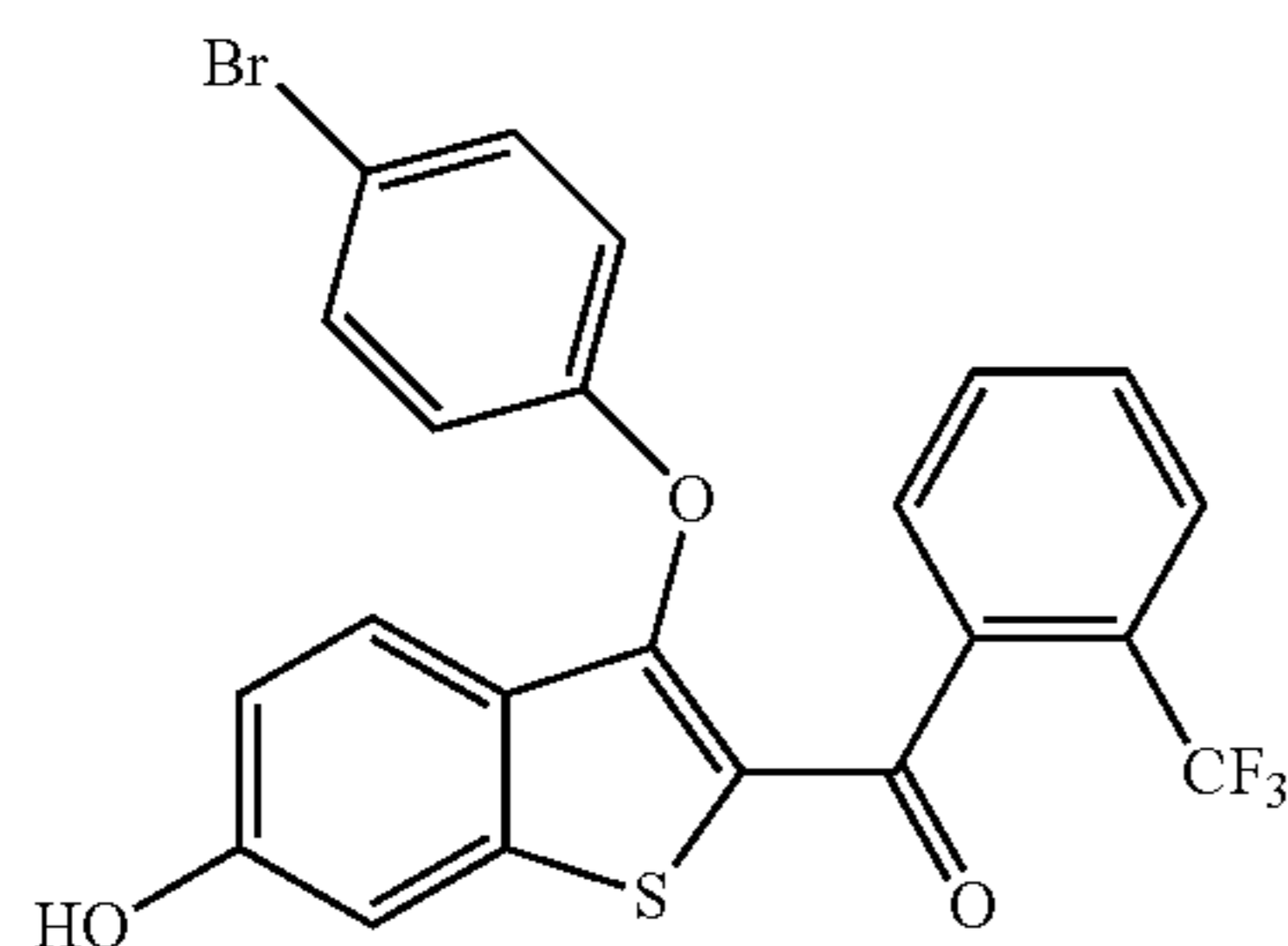
(3-(4-Bromophenoxy)-6-hydroxybenzo[b]thiophen-2-yl)(2-(trifluoromethyl)phenyl)methanone
