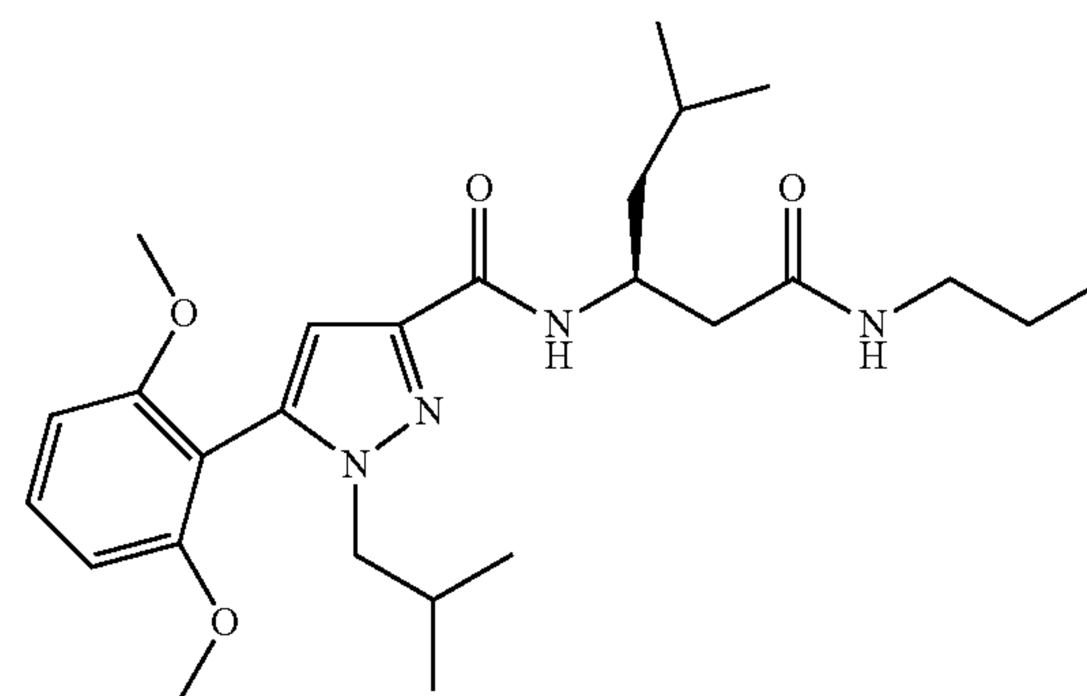
157: (S)-5-(2,6-dimethoxyphenyl)-1-isobutyl-N-(5-methyl-1-oxo-1-(propylamino)hexan-3-yl)-1H-pyrazole-3-carboxamide (Also see FIG. 1/Scheme 1).
