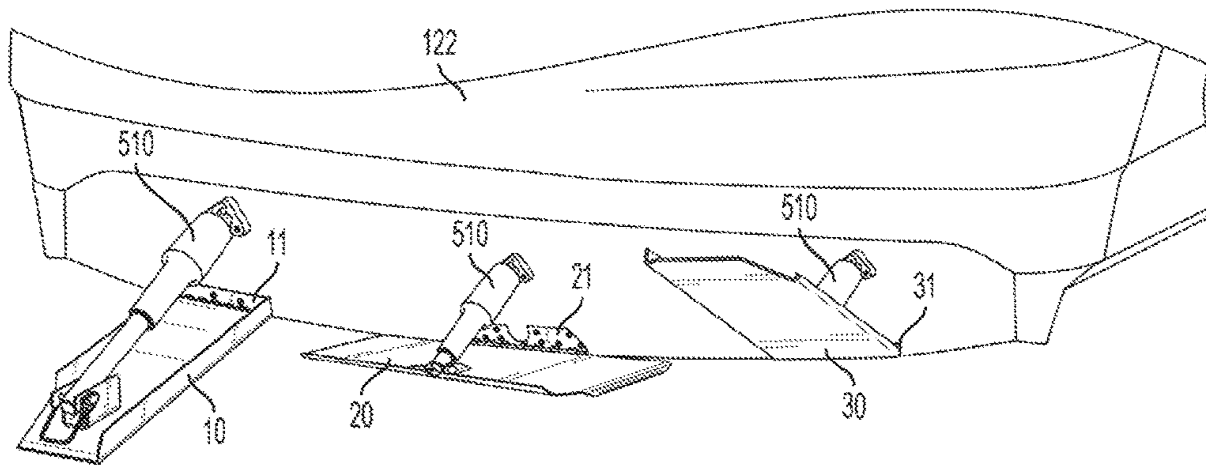
FIG. 1 PRIOR ART
