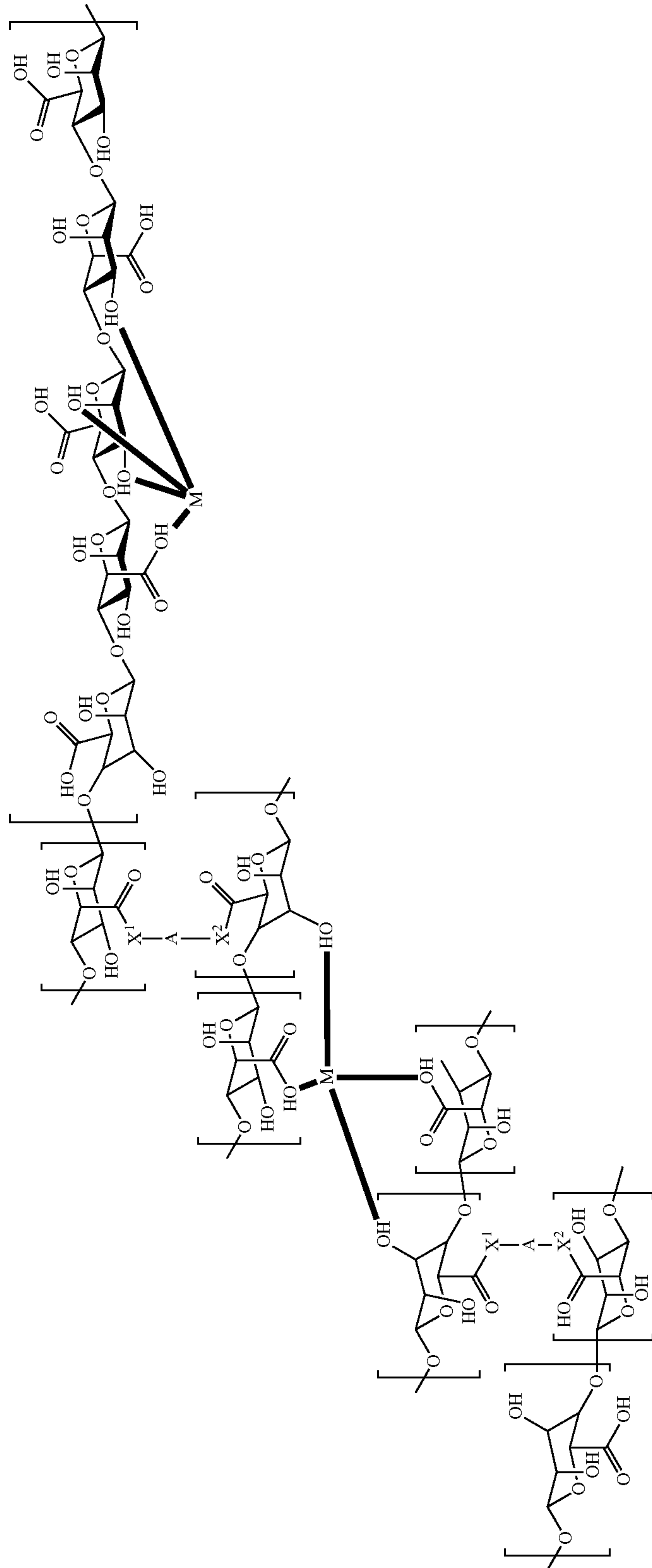
Formula IV
