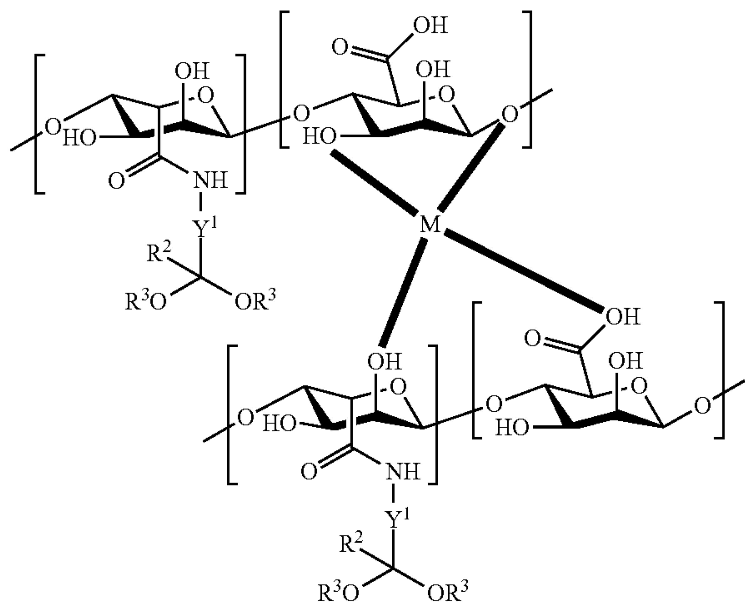
Formula VI
