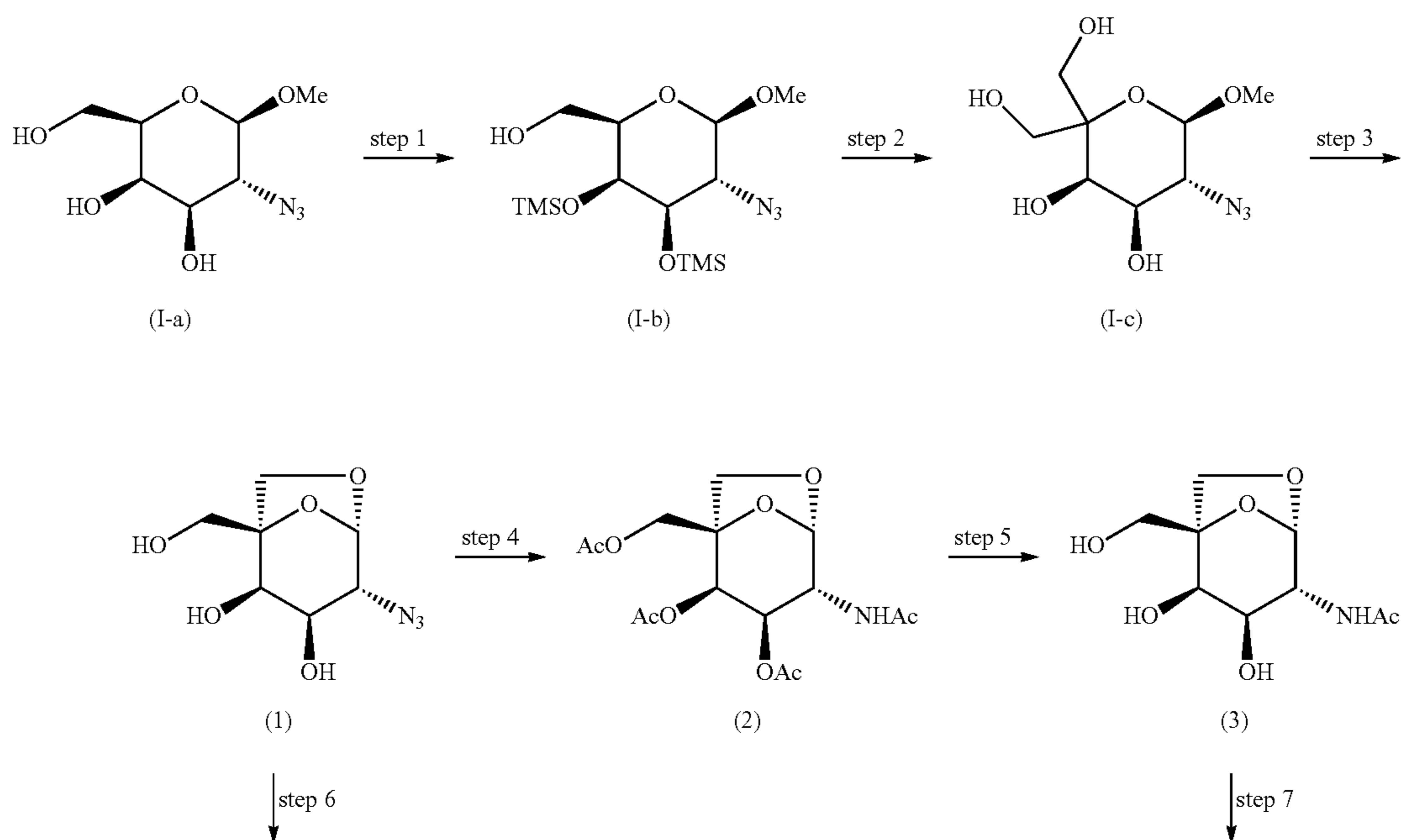
Scheme 1.
