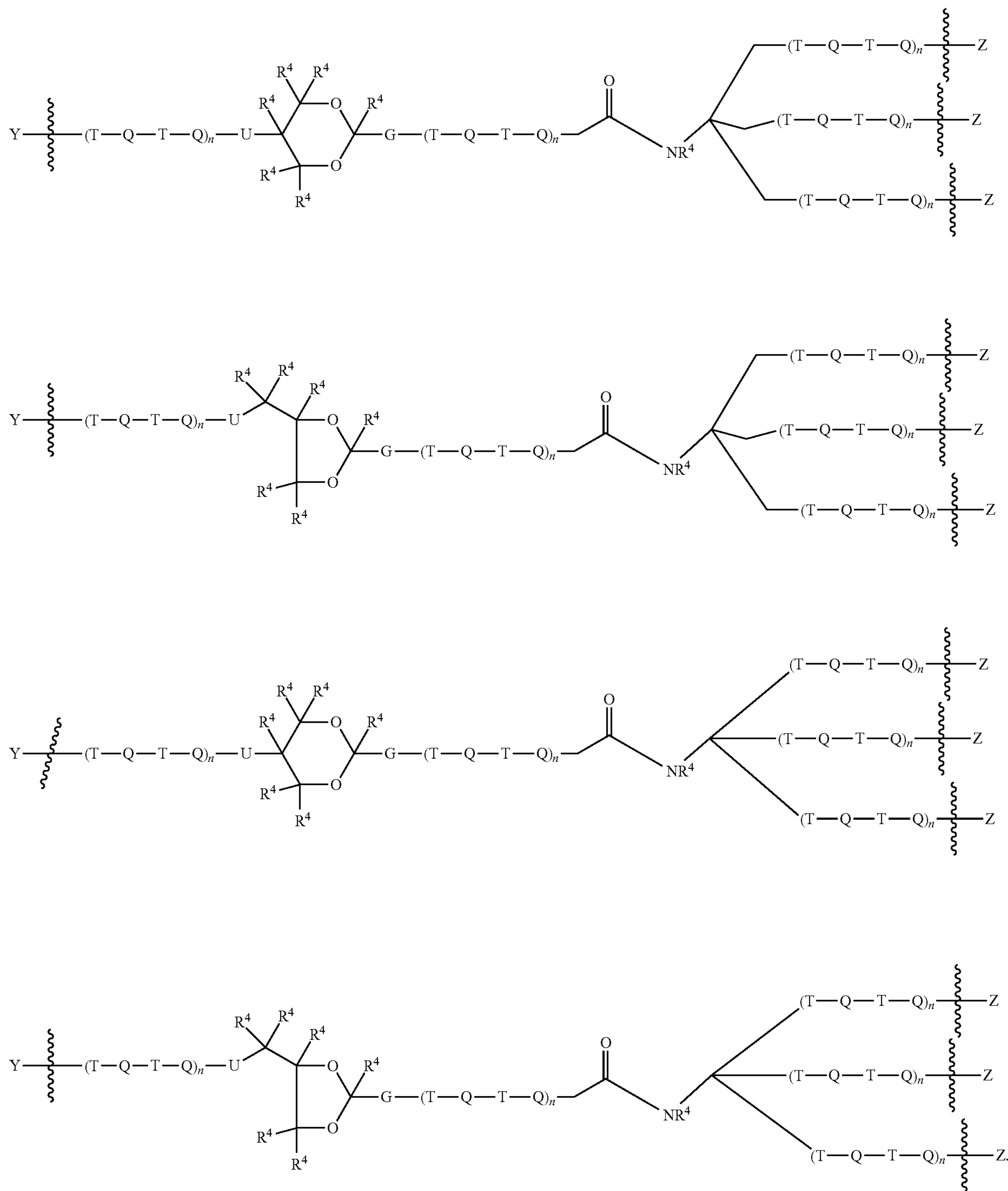
Scheme 3
