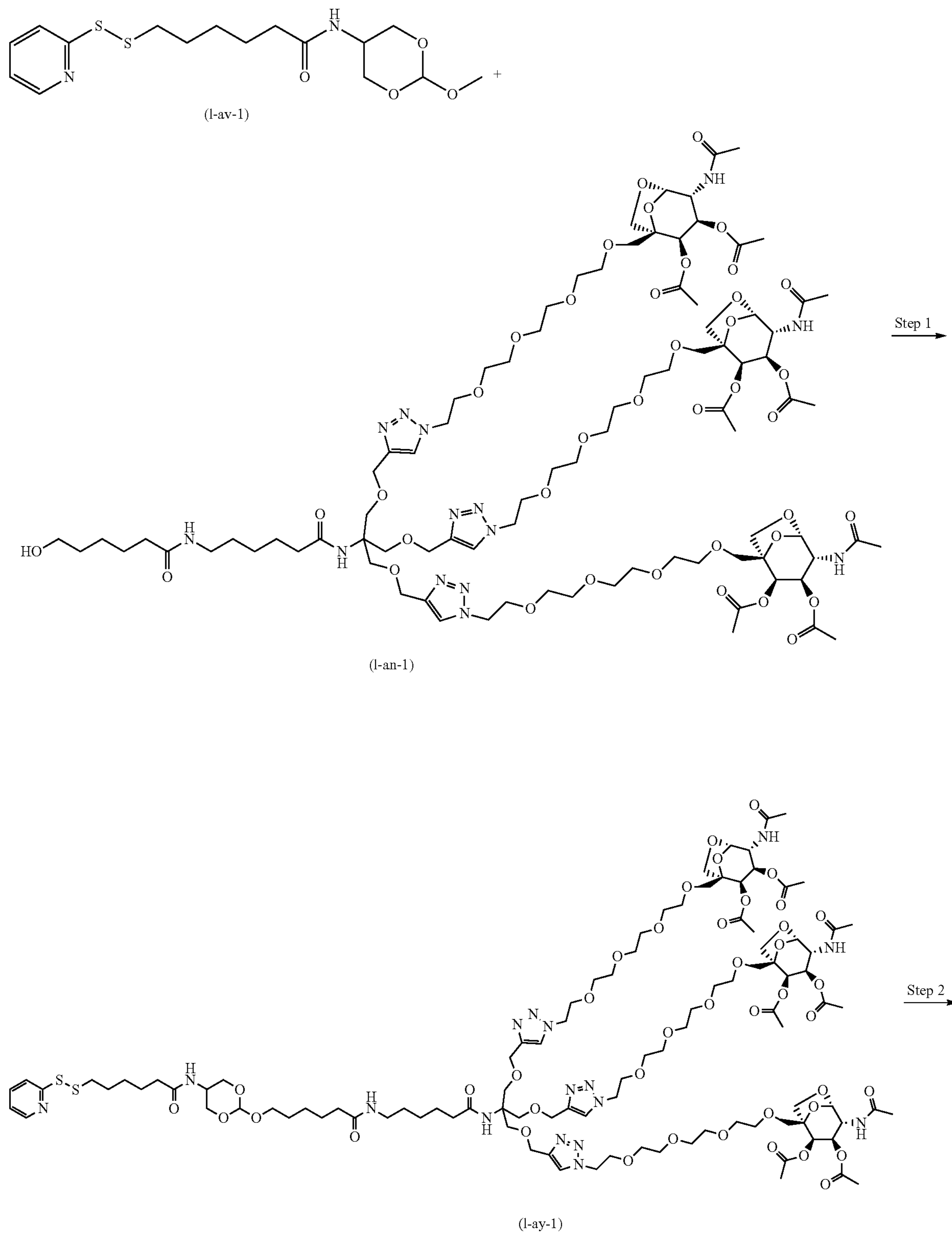
Scheme 5
