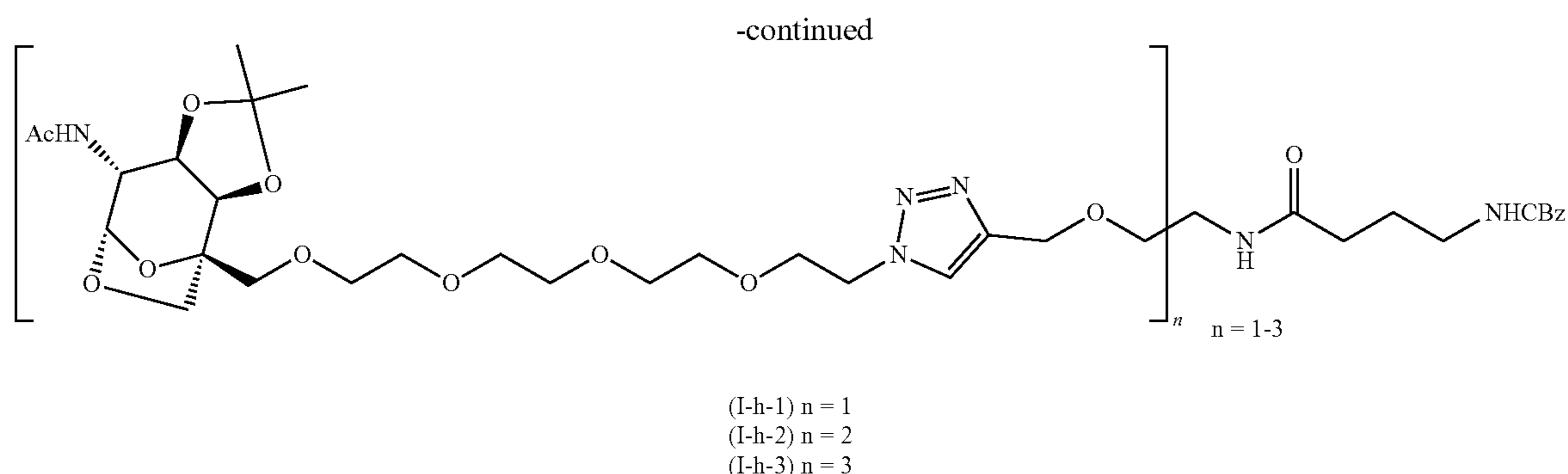
Intermediate (I-h-1)
