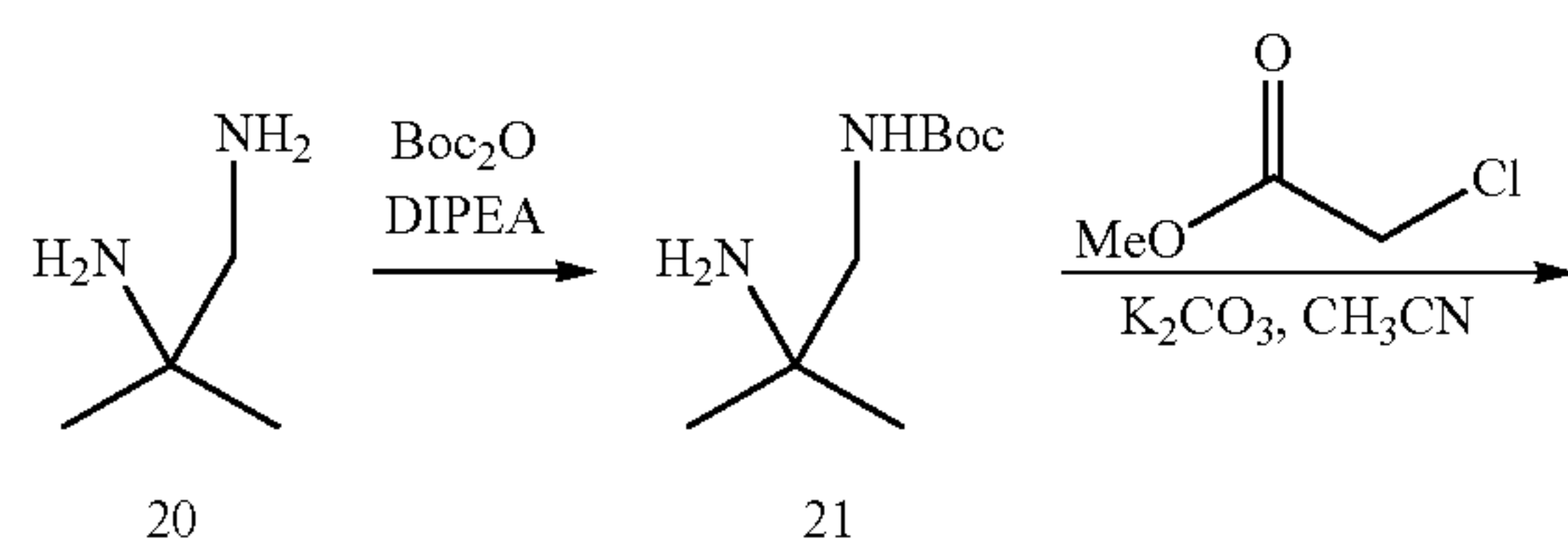
Scheme 5
