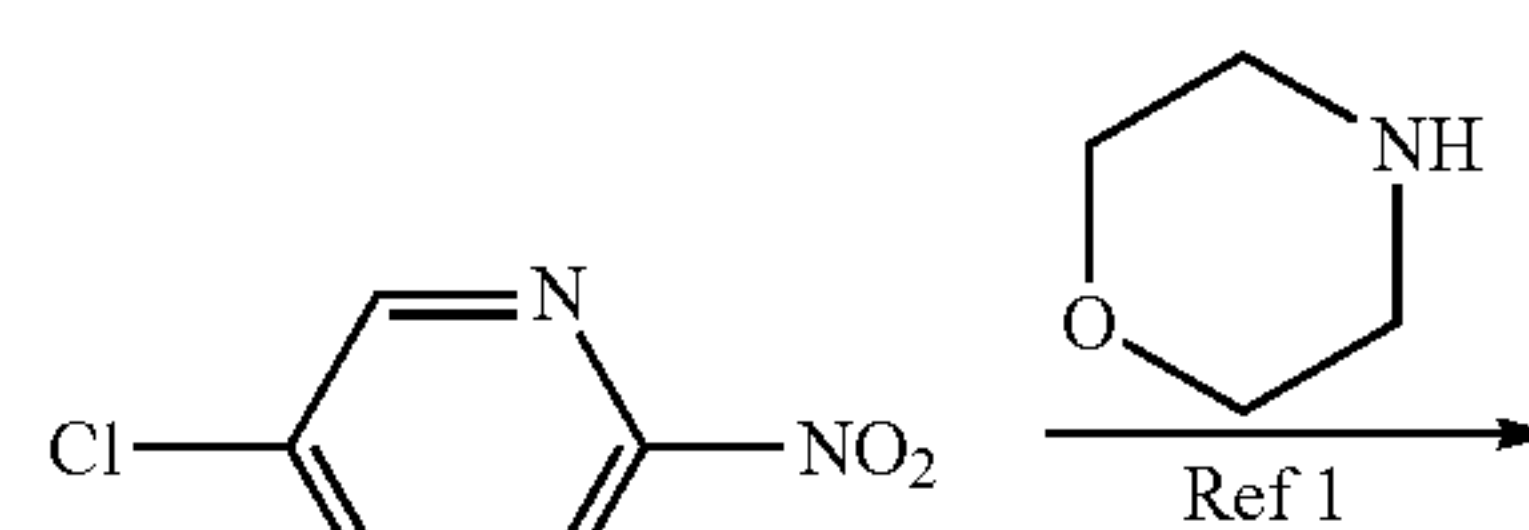
Scheme 7
