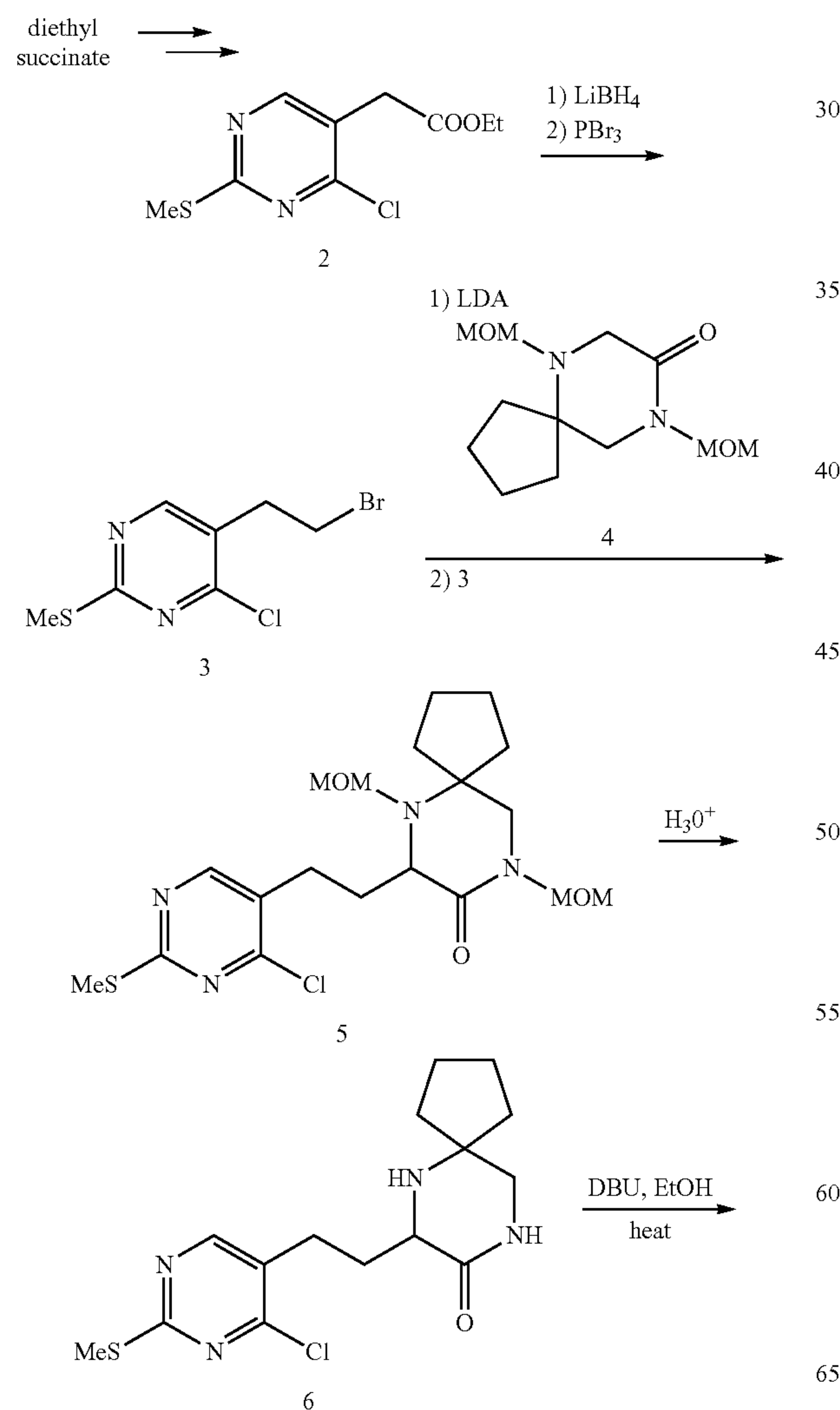
Scheme 1
