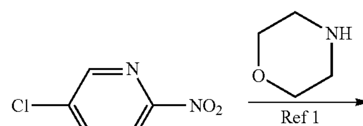
Scheme 8
