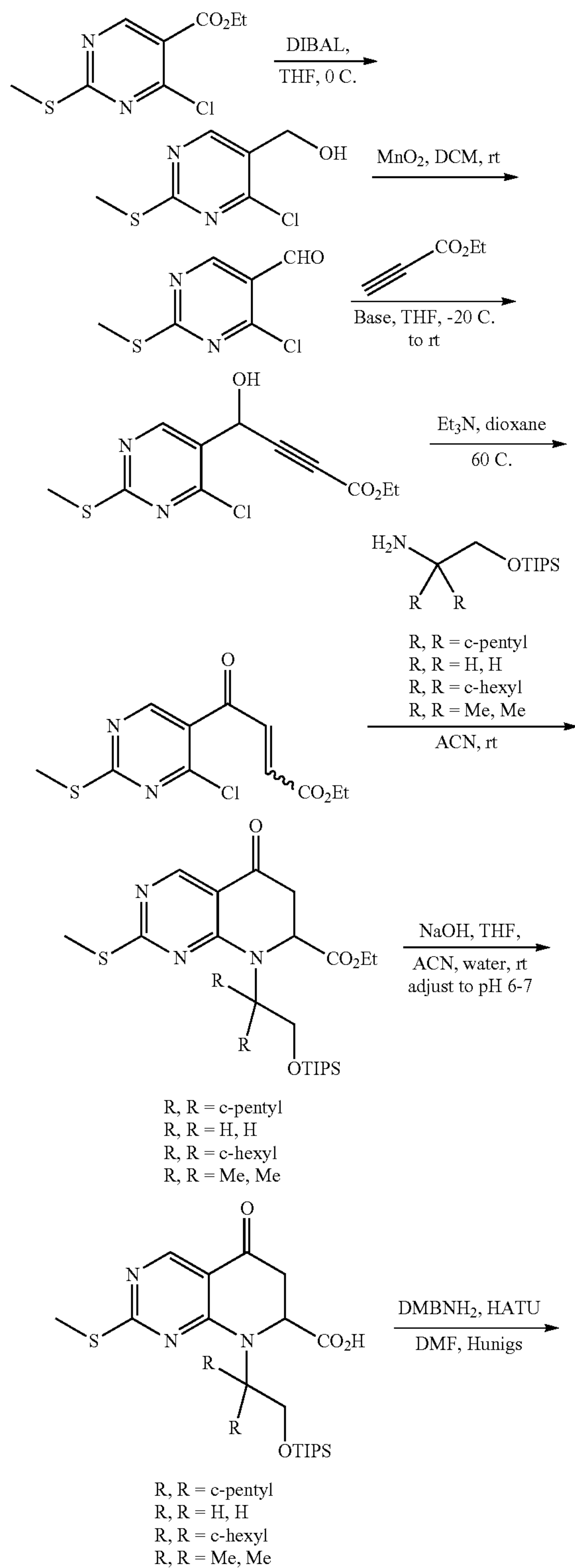
Scheme 9
