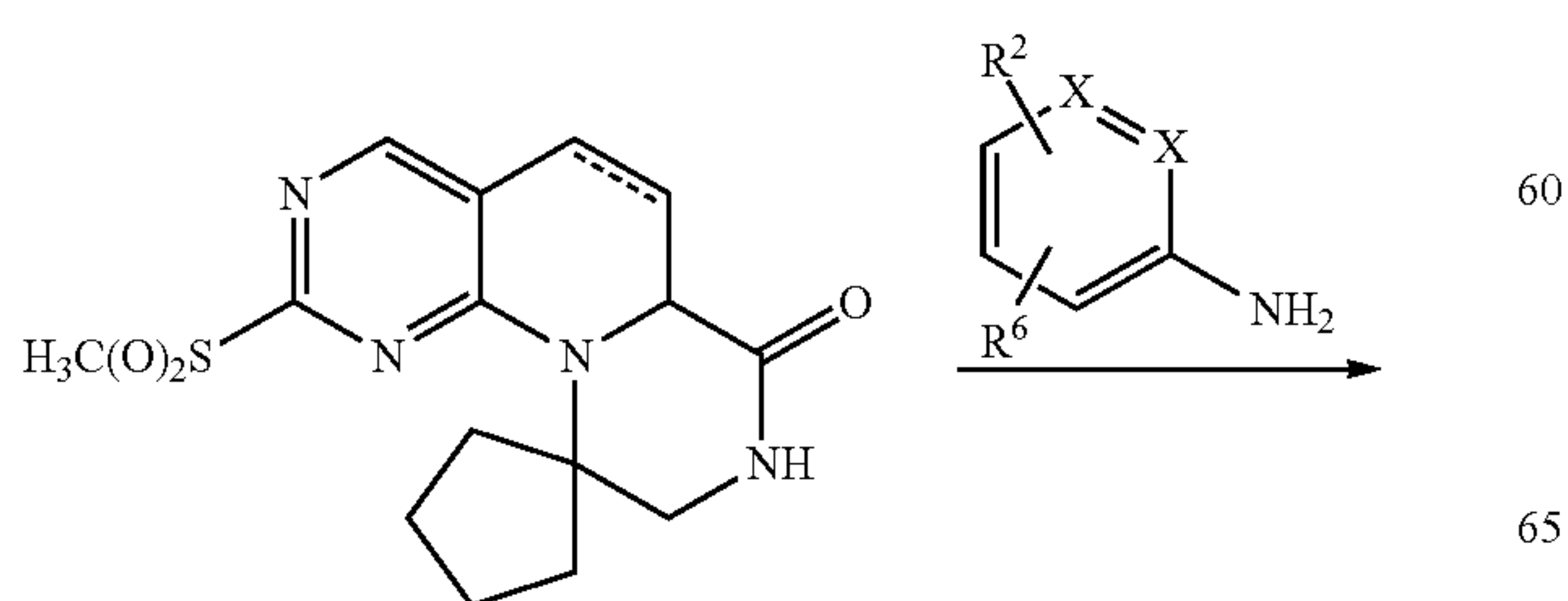
Scheme 4
