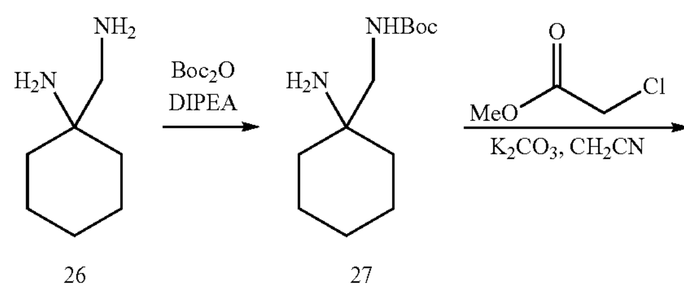
Scheme 6
