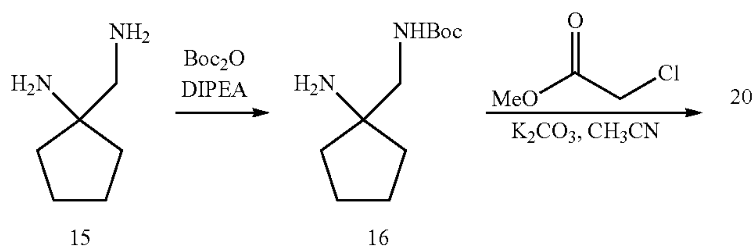
Scheme 3
