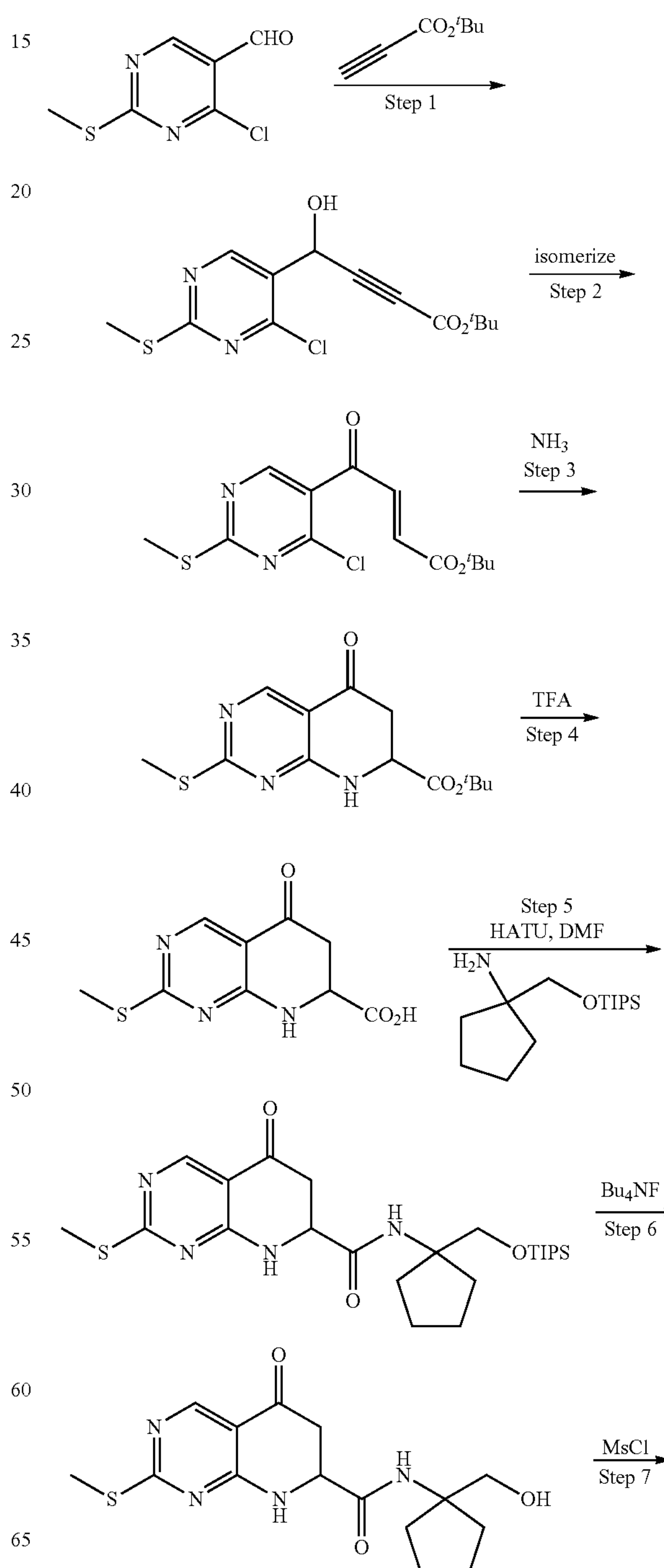
Scheme 10
