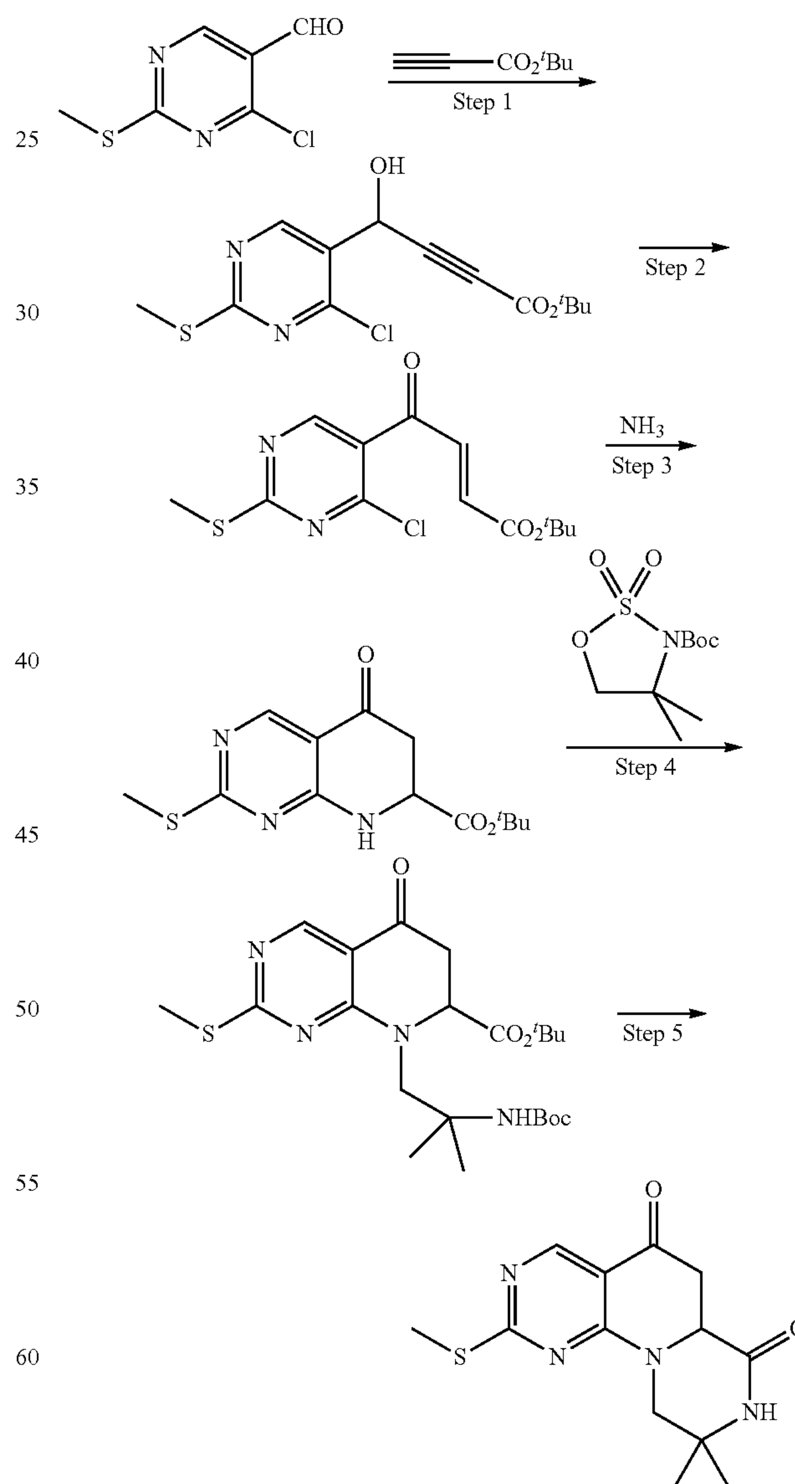
Scheme 11
