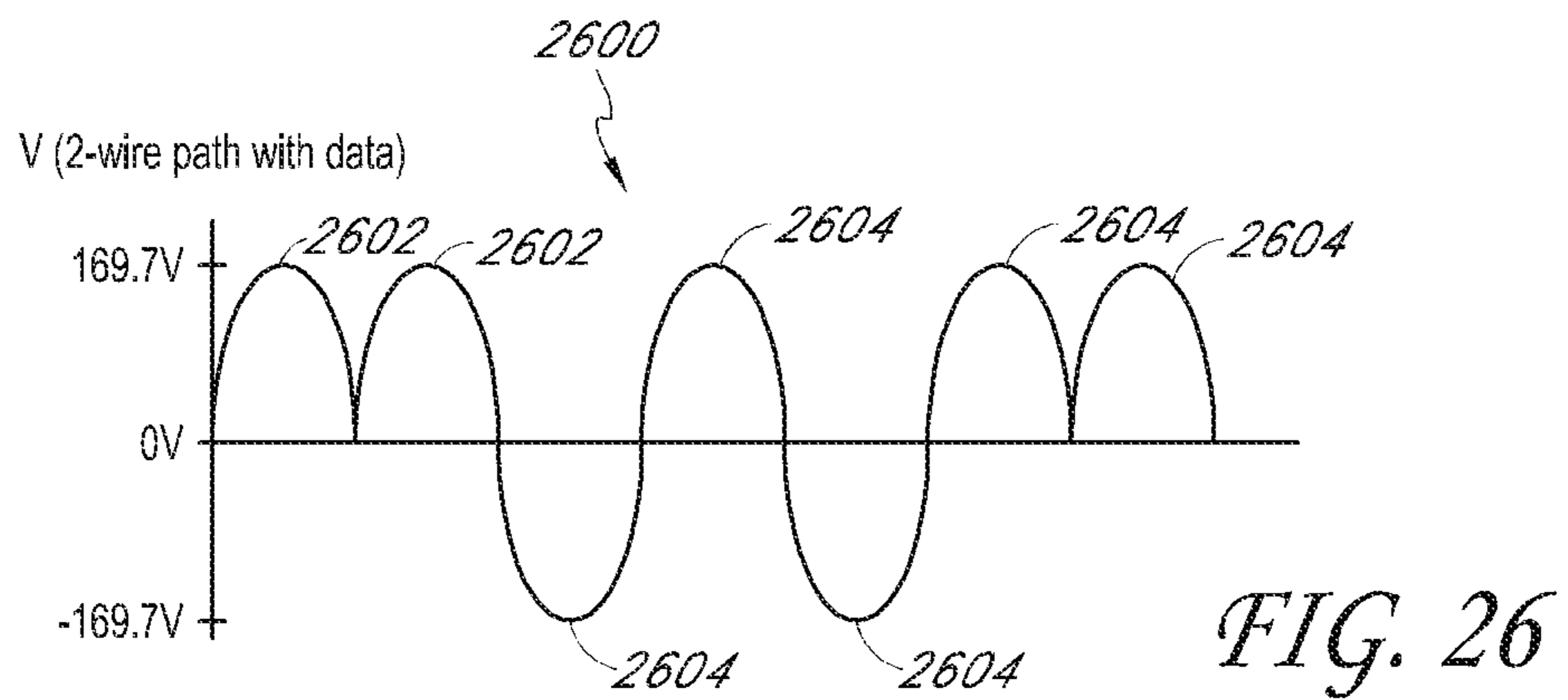
Bridge Waveforms
