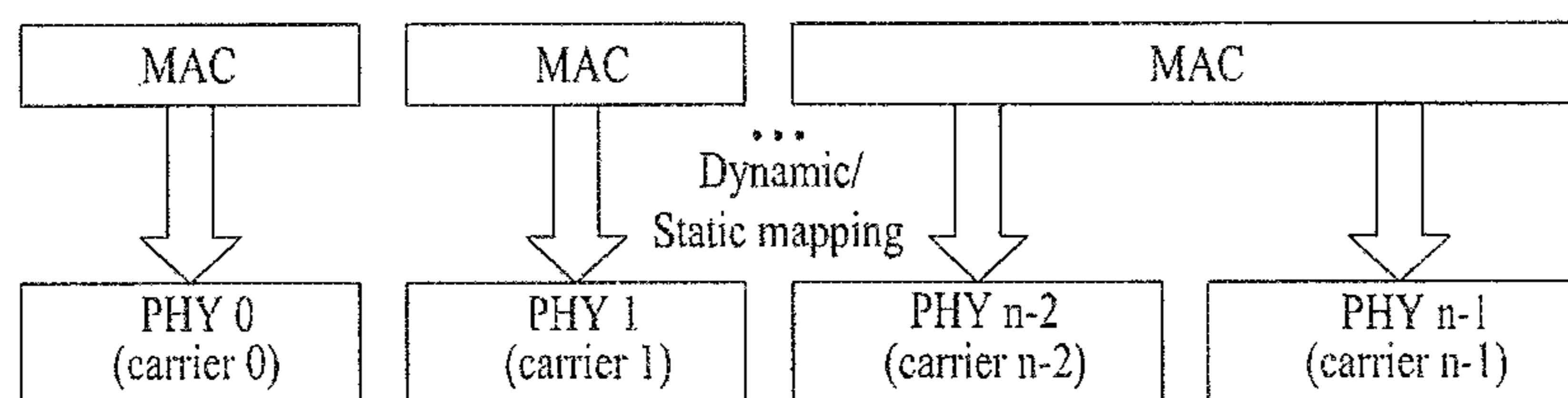
(a) Transmitter
