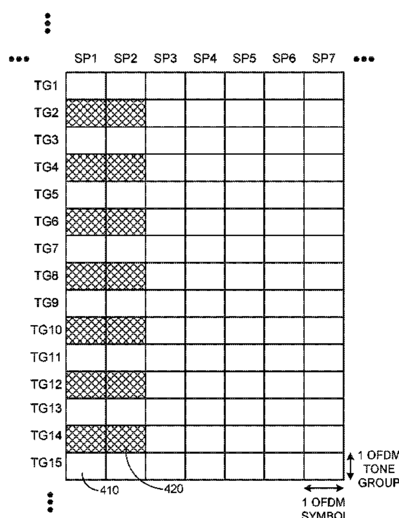
SHORT COMMON CONTROL CHANNEL (CCH) FORMAT
