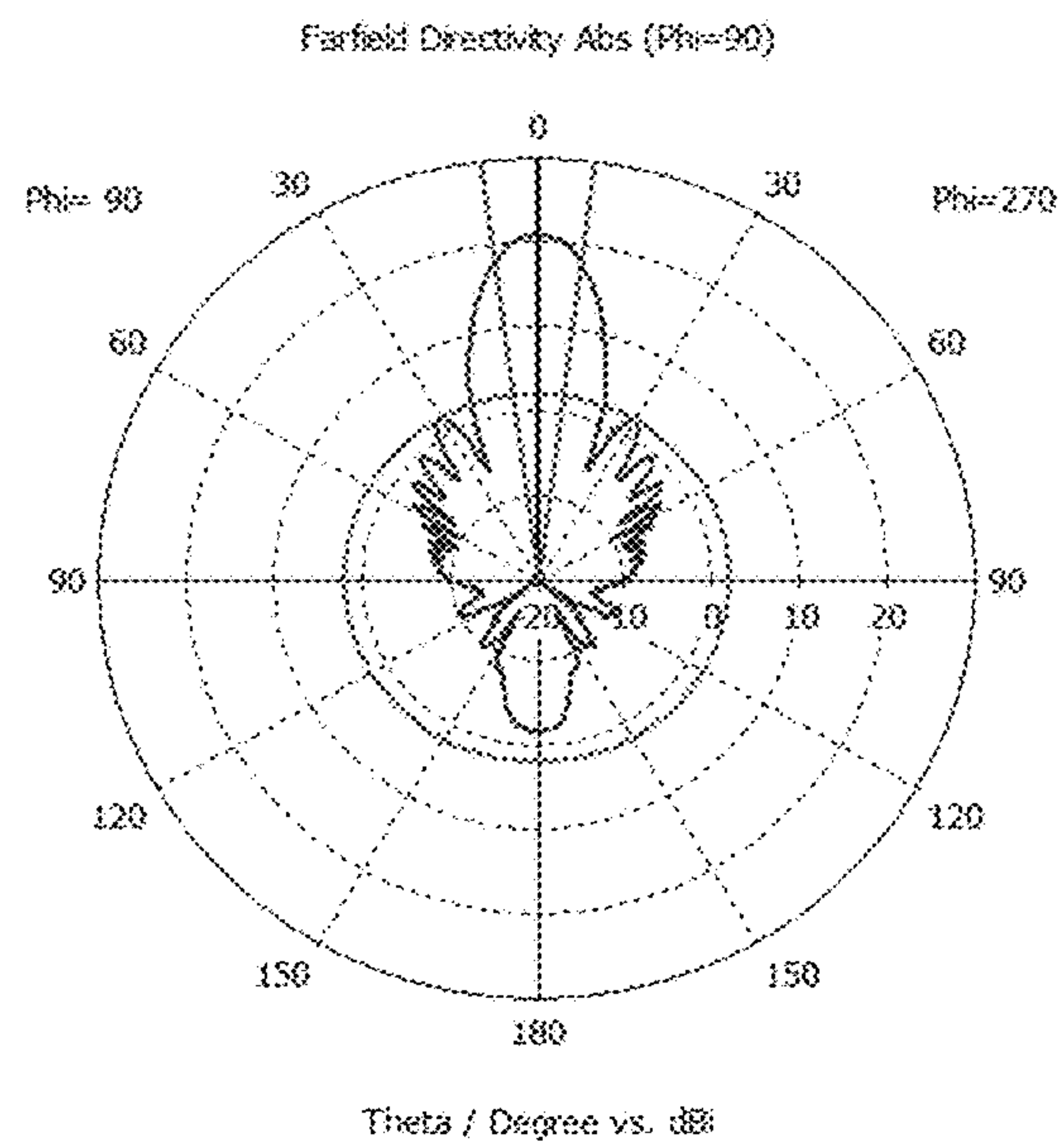
Antenna Gain Pattern
