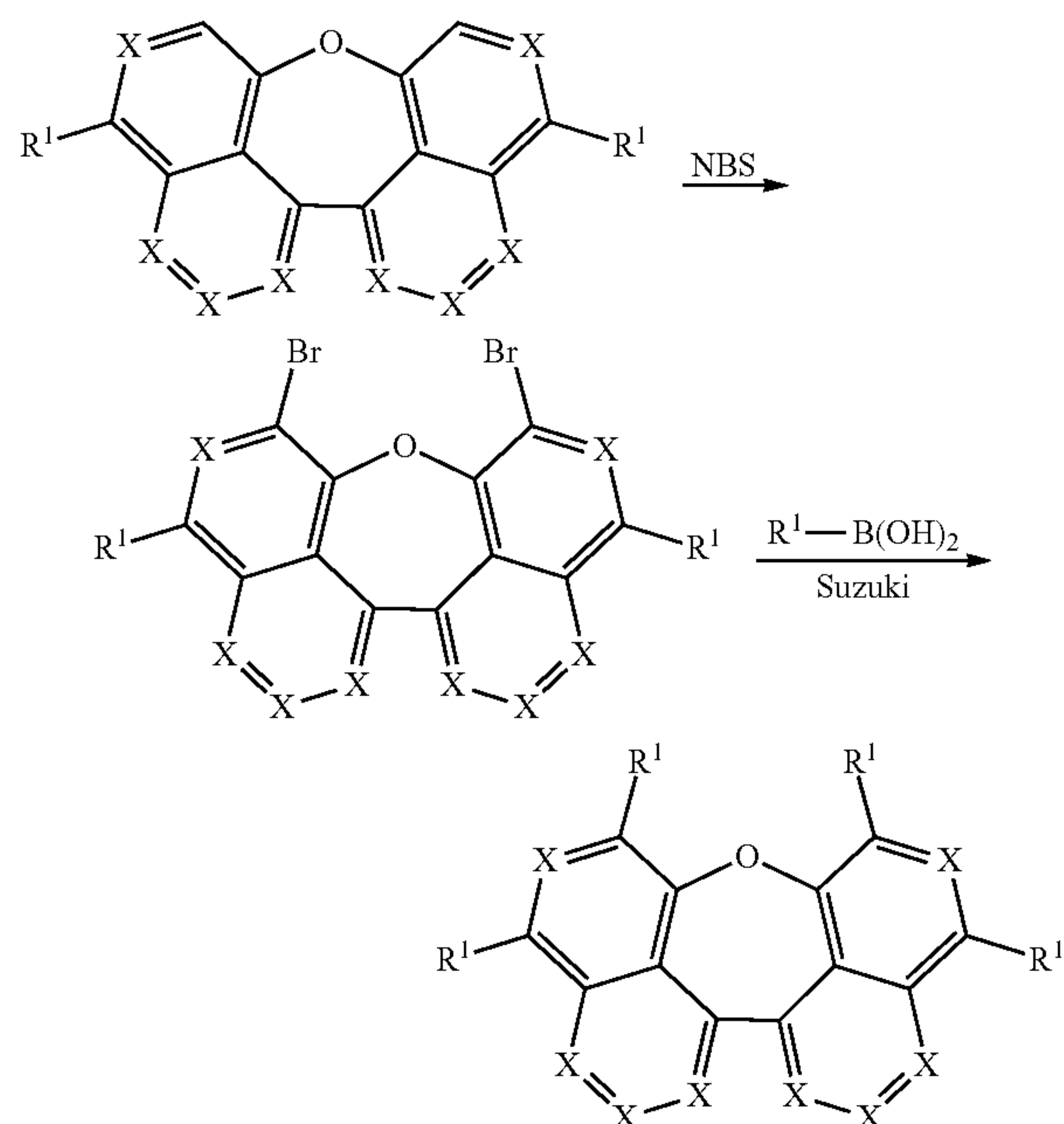
Scheme 2
