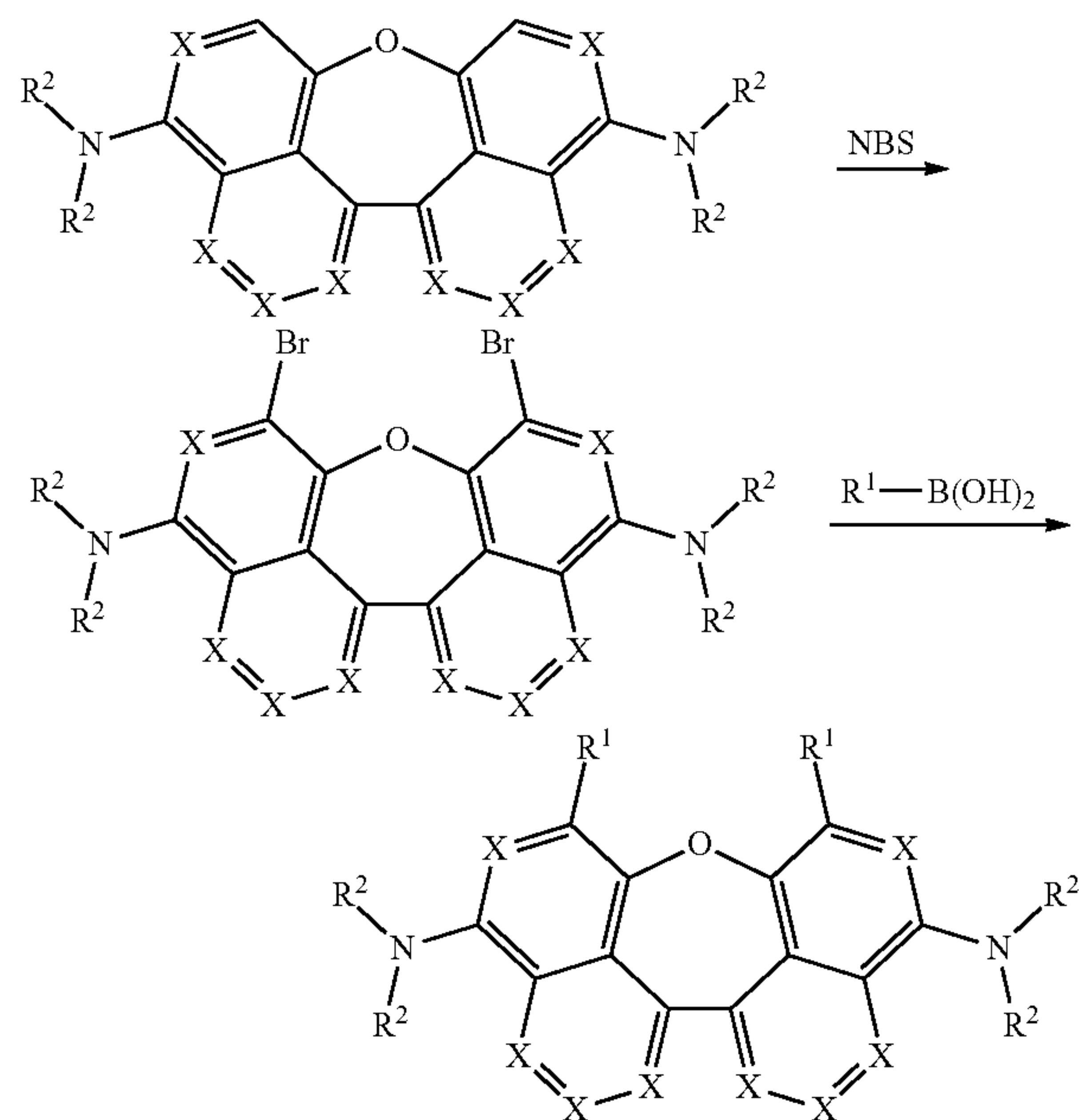
Scheme 3
