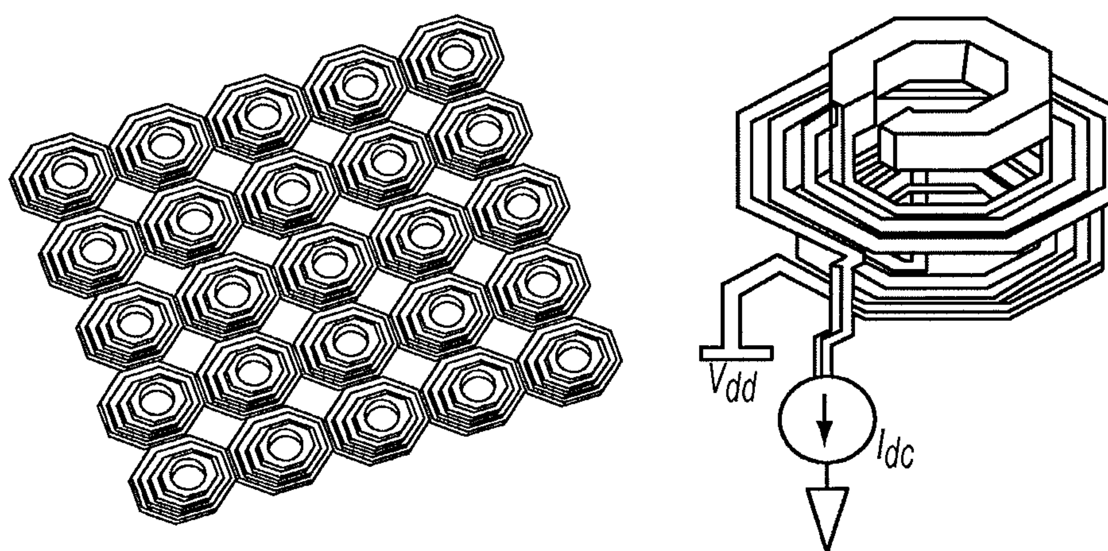
The coil array and coil layout
