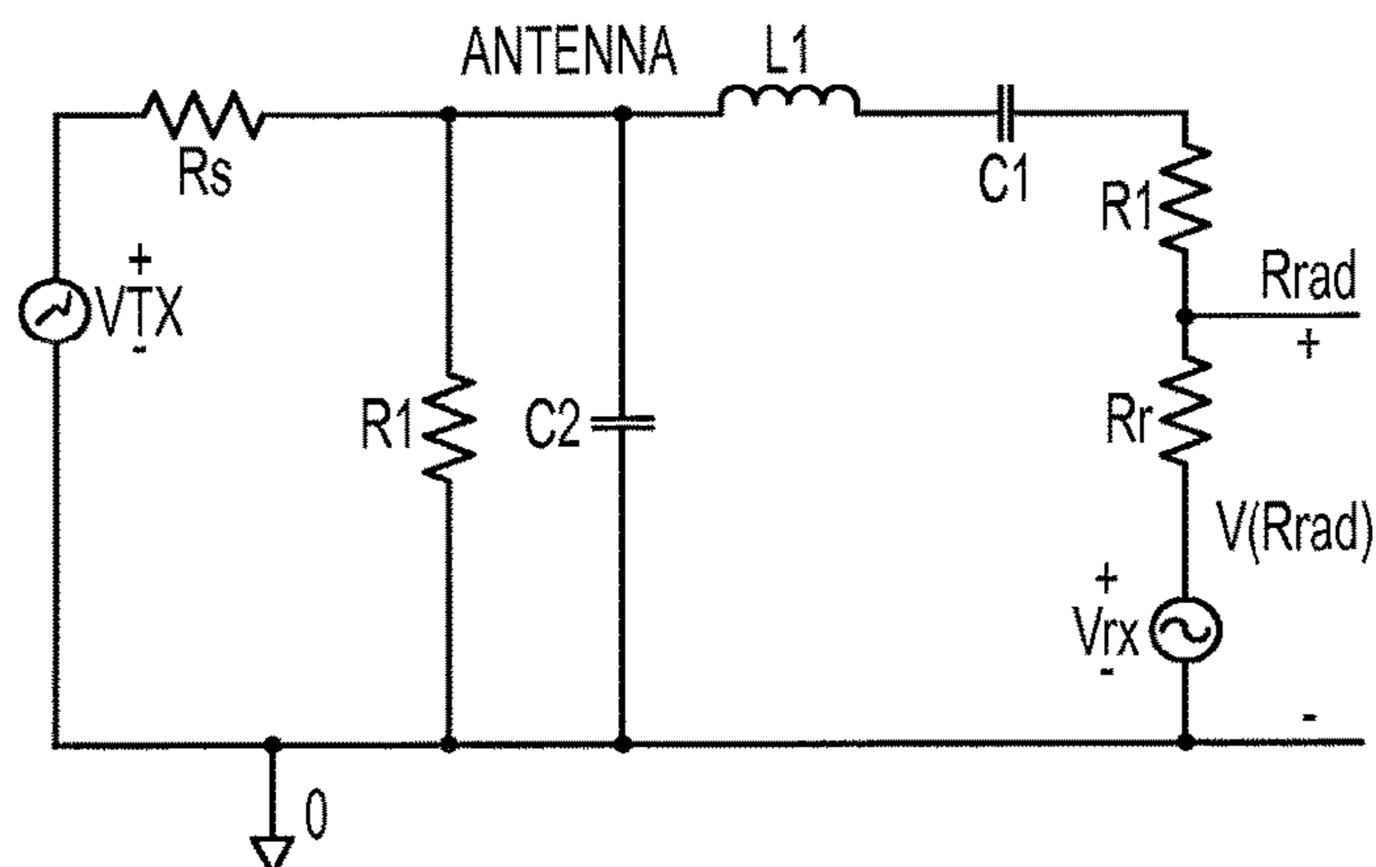
ELECTRICAL EQUIVALENT OF A HALF WAVELENGTH DIPOLE ANTENNA CONNECTED TO A-50 OHM SOURCE
