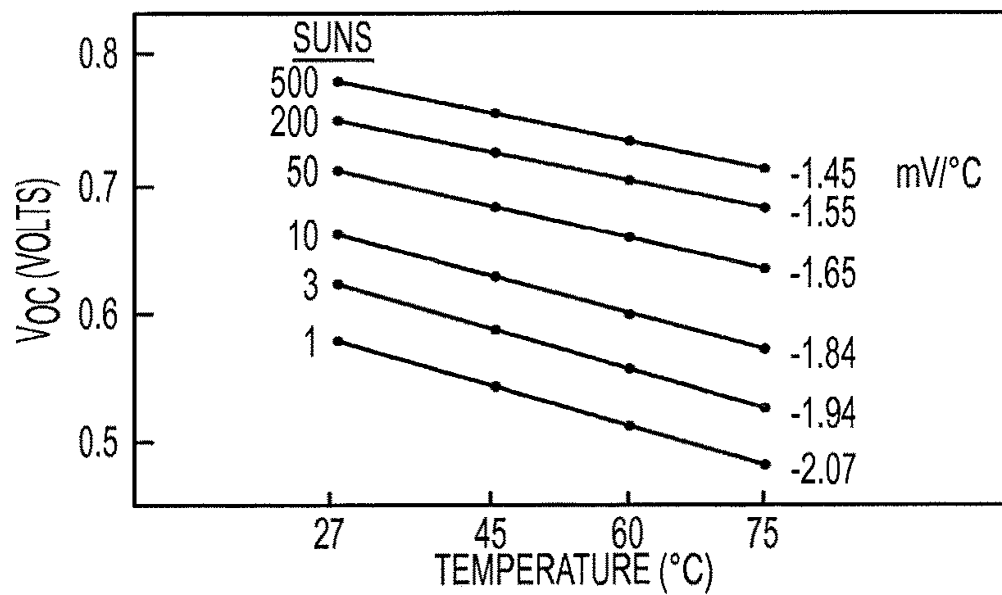
V_{oc} TEMPERATURE DEPENDENCY OF SOLAR DEVICES LEFT FIG. 7F
