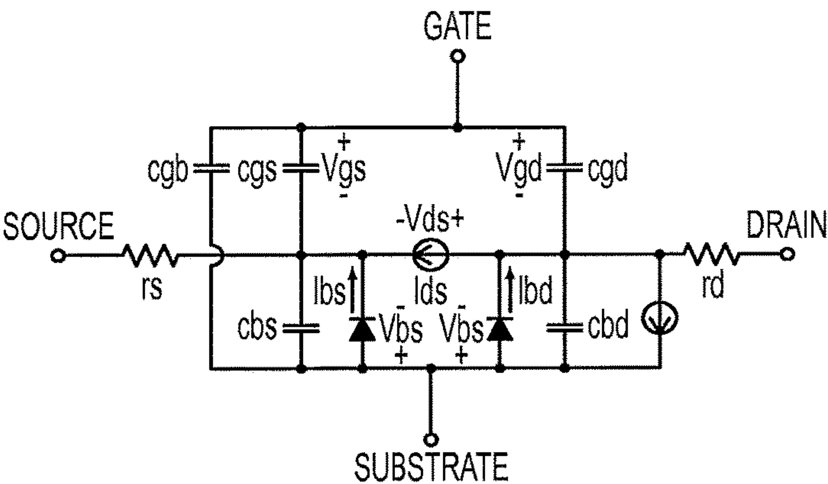
MOS TRANSISTOR EQUIVALENT CIRCUIT FIG. 18B
