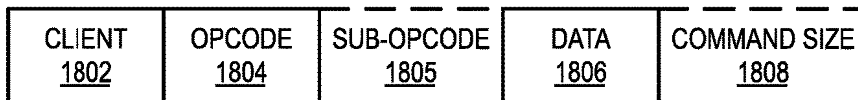
FIG. 18A GRAPHICS PROCESSOR COMMAND FORMAT 1800
