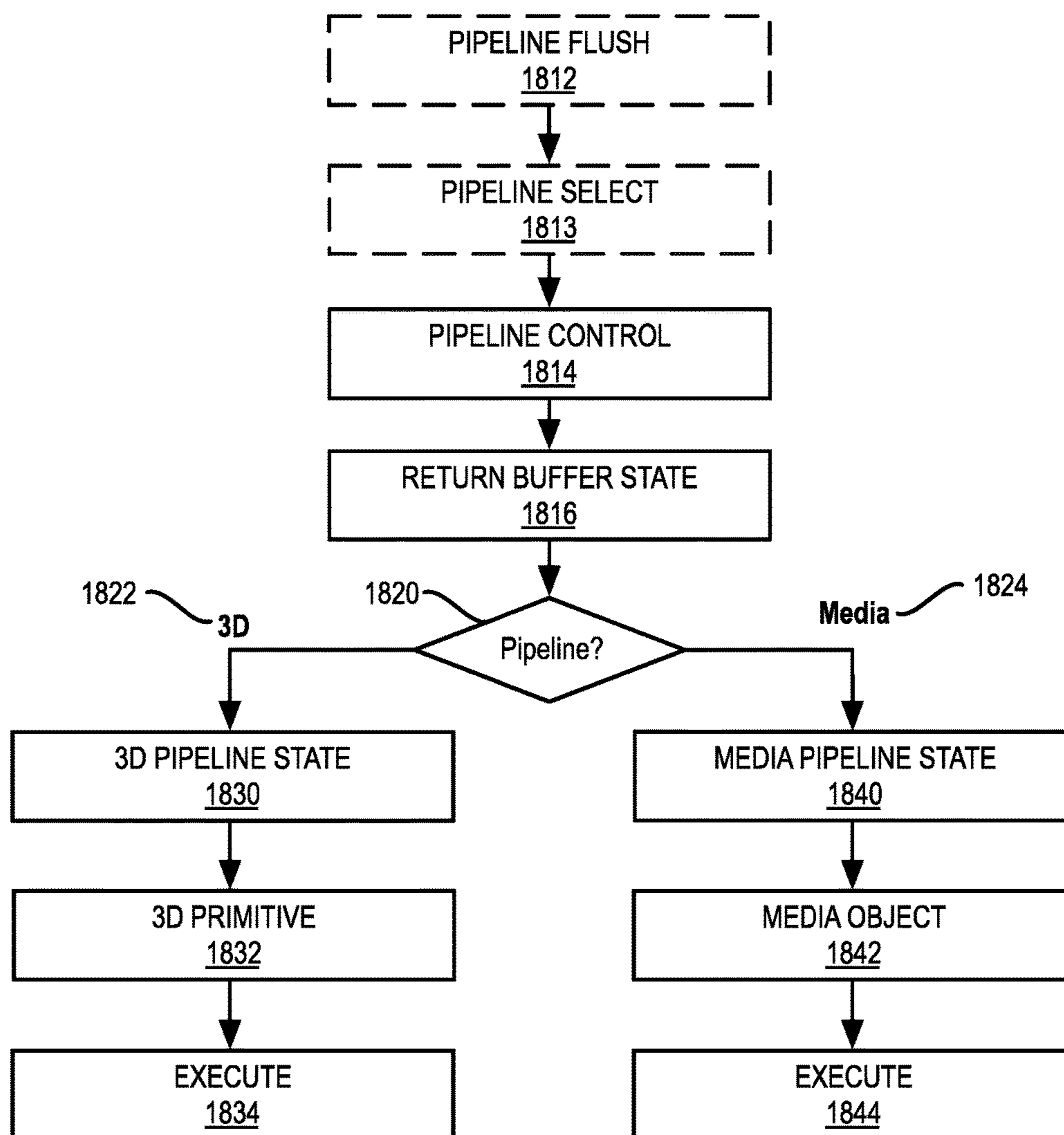
FIG. 18B GRAPHICS PROCESSOR COMMAND SEQUENCE 1810
