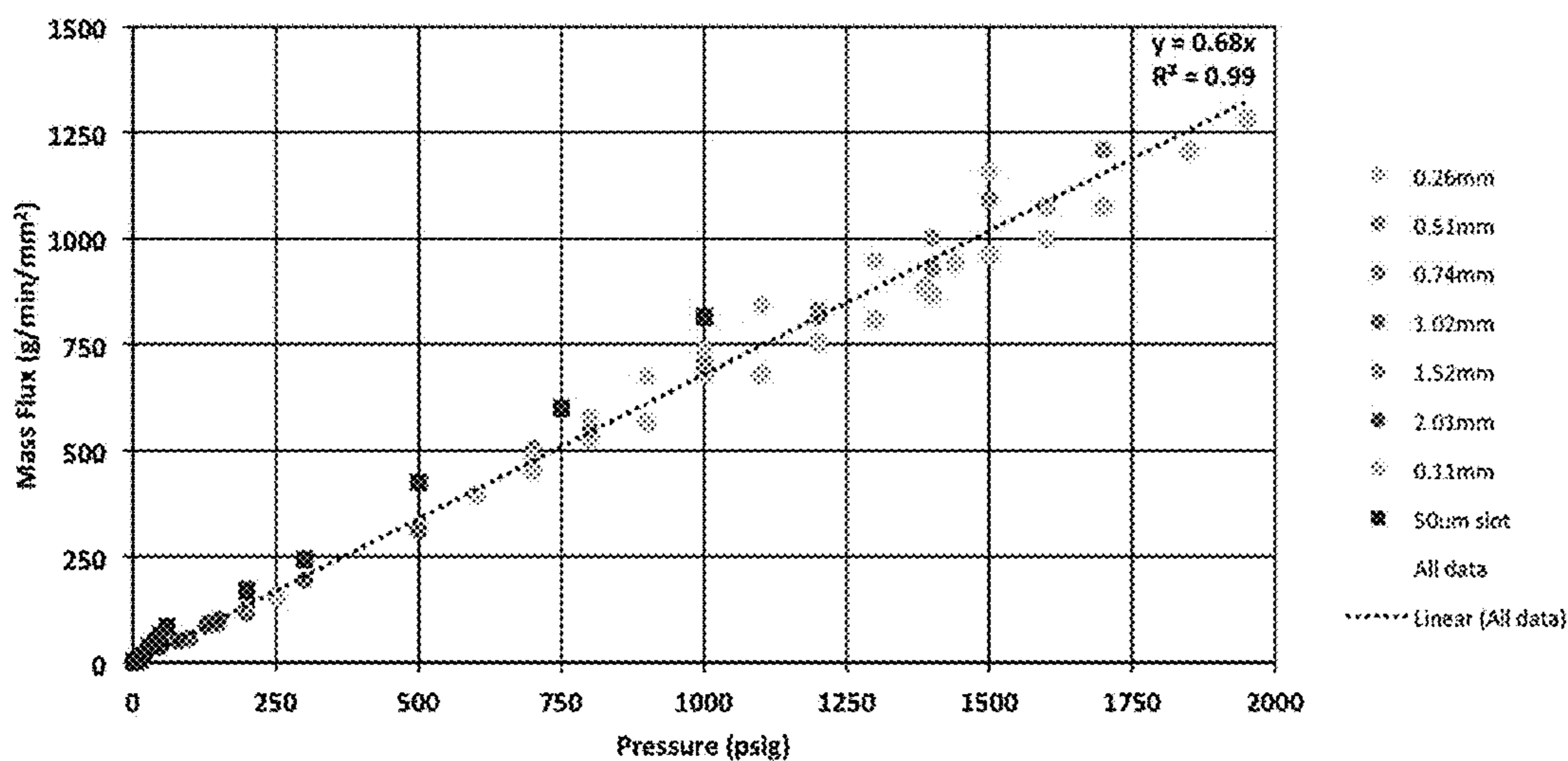
Mass Flux vs. Pressure for Round Holes & Slots
