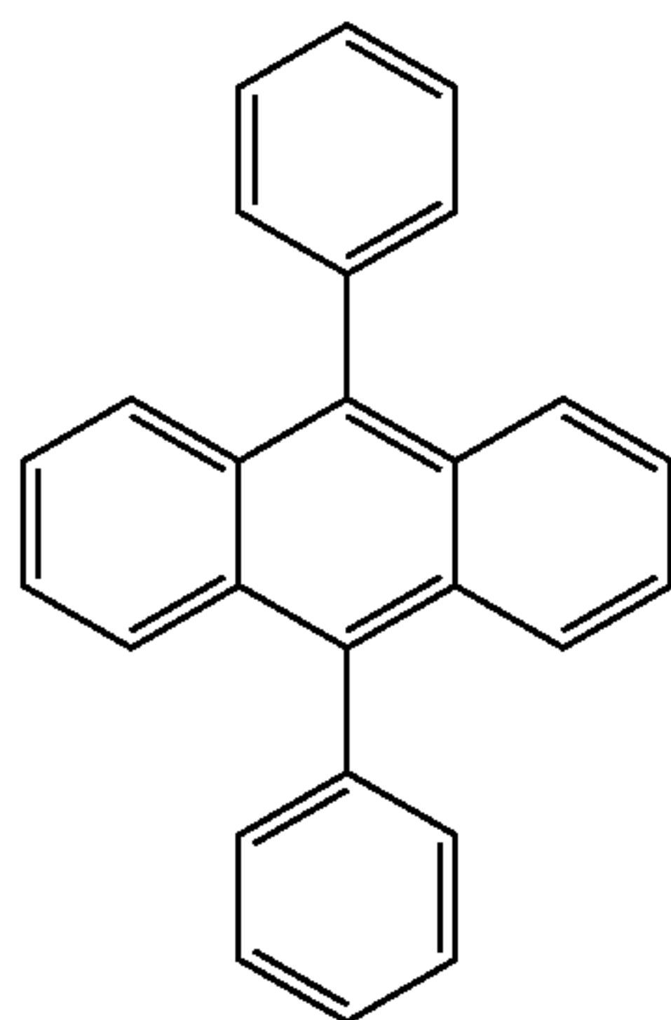
9,10-diphenylanthracene
