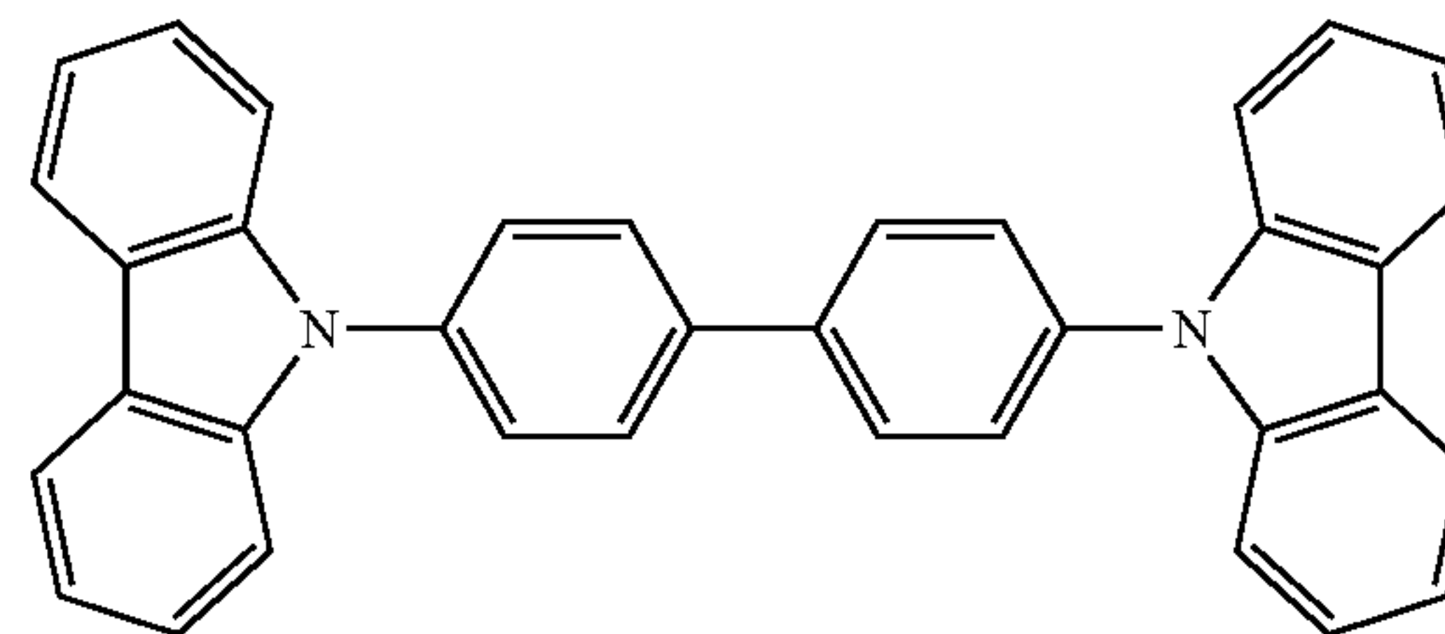
Carbazole derivative 2
