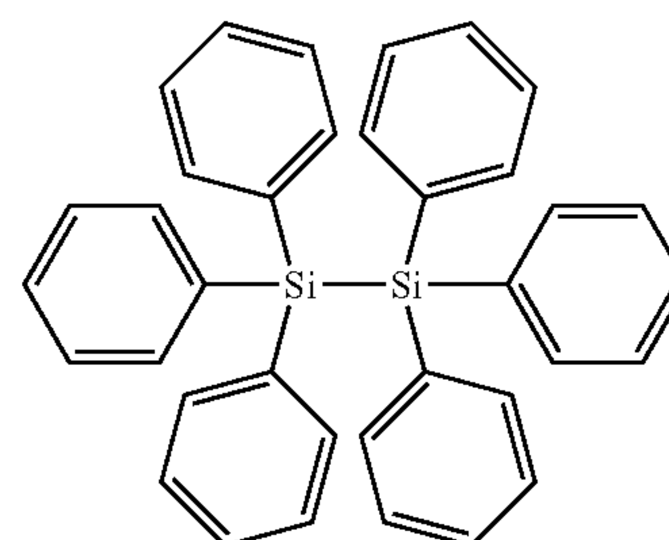
Hexaphenyldisilane
