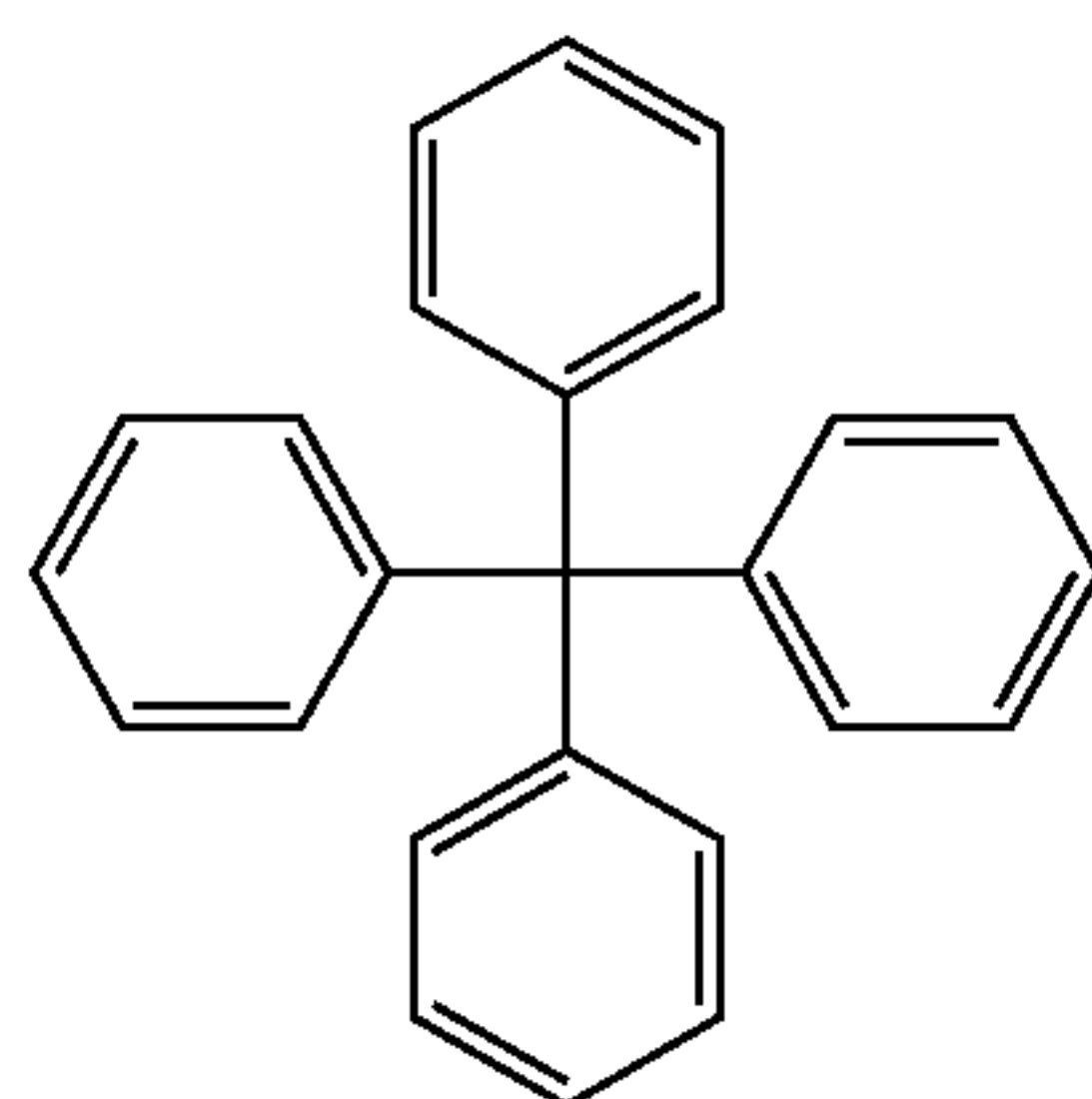
Tetraphenylmethane
