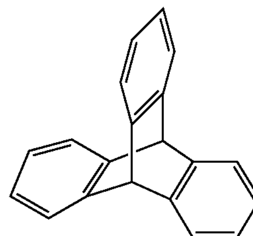
Triptycene (9,10-o-Benzene-9,10-dihydroanthracene)
