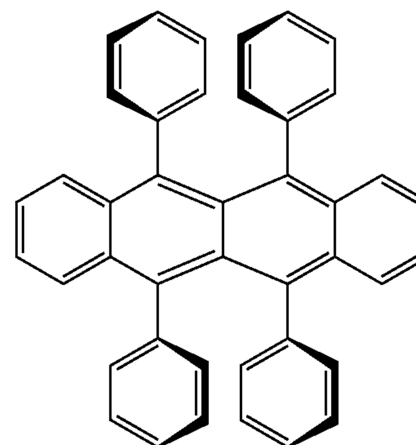
Rubrene (5,6,11,12-tetraphenyltetracene)
