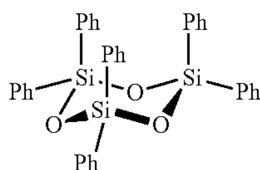
Hexaphenylcyclotrisiloxane
