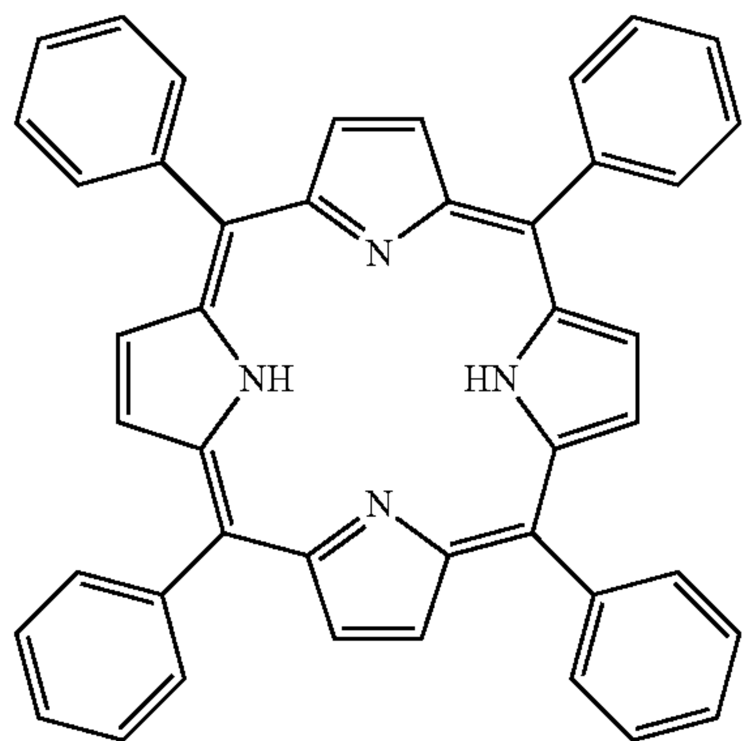
Tetrakisphenyl-porphyrin
