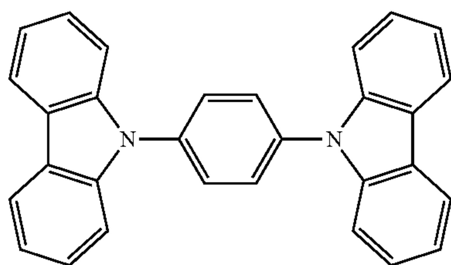
Carbazole Derivative 1
