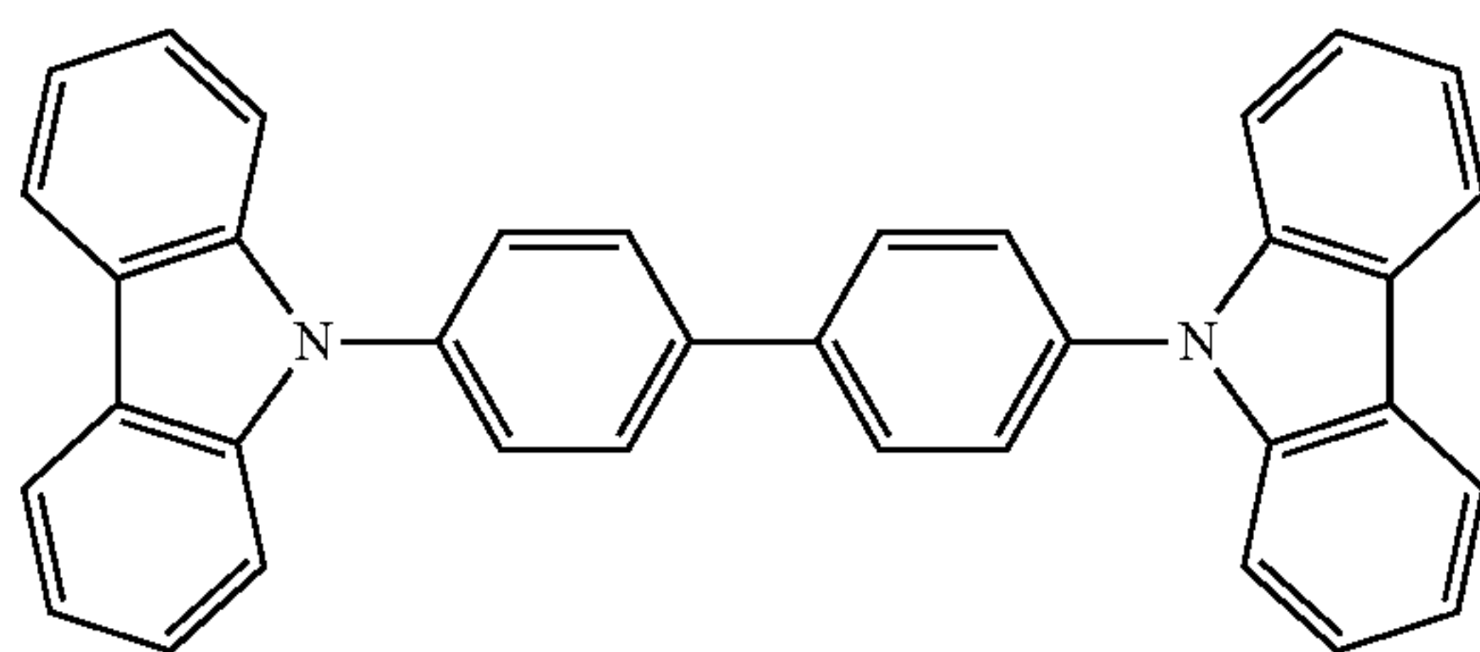
Carbazole derivative 2
