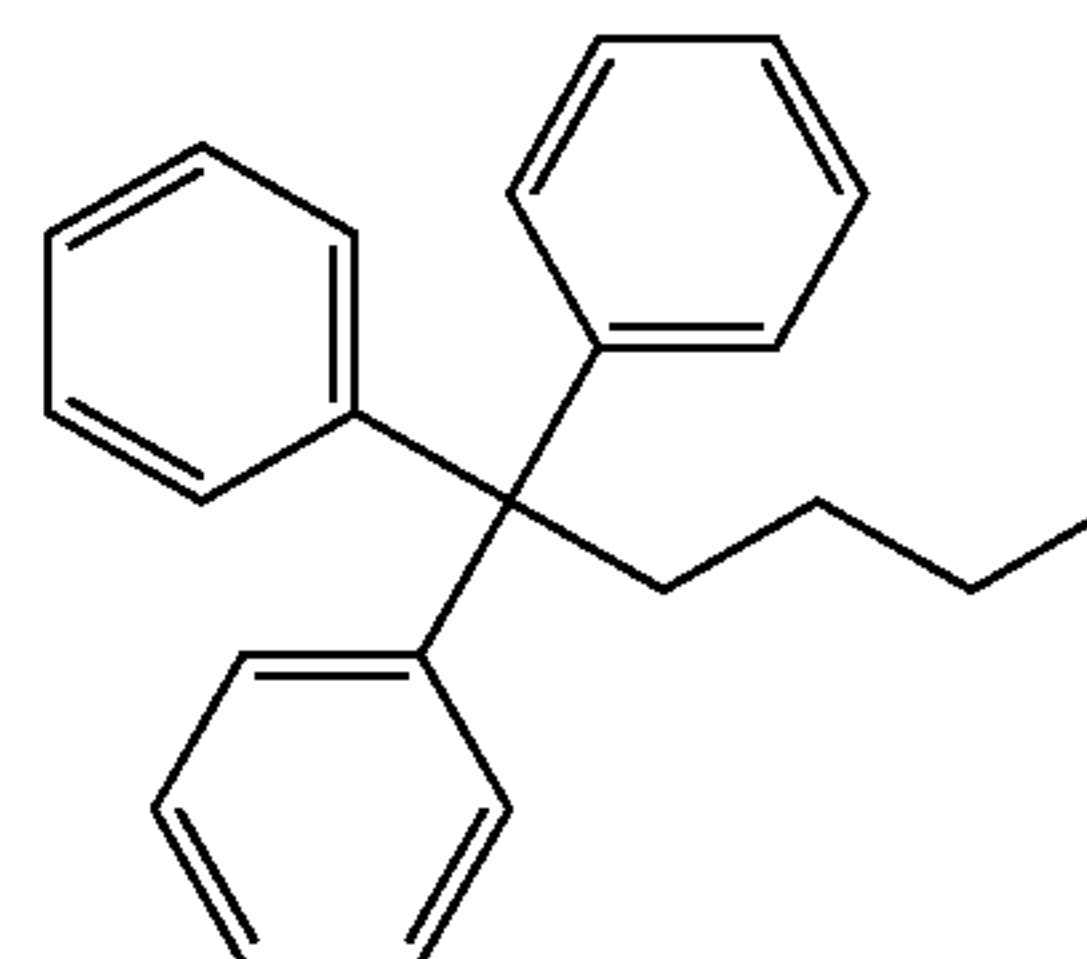
Triphenyl-n-pentane
