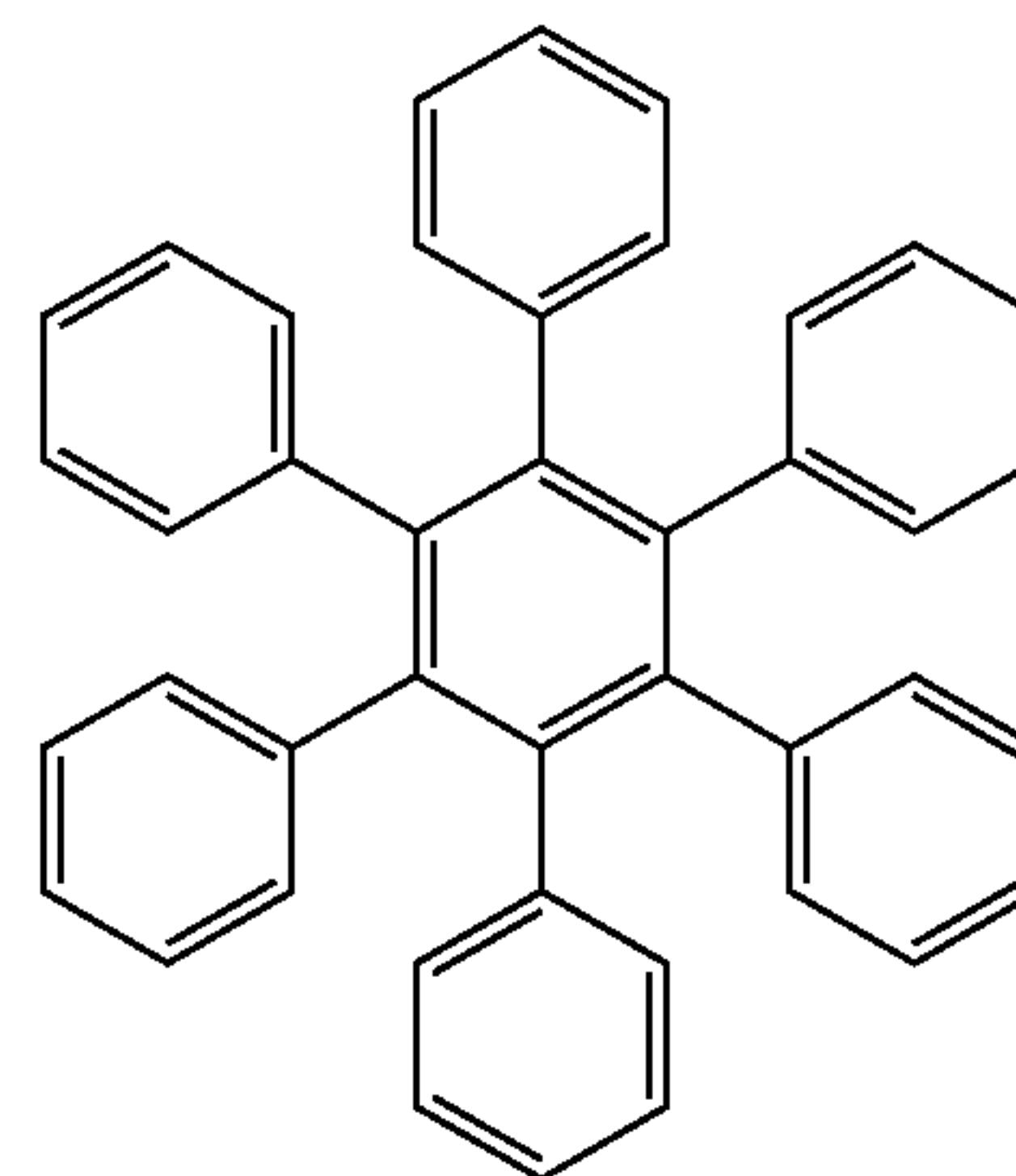
Hexaphenylbenzene
