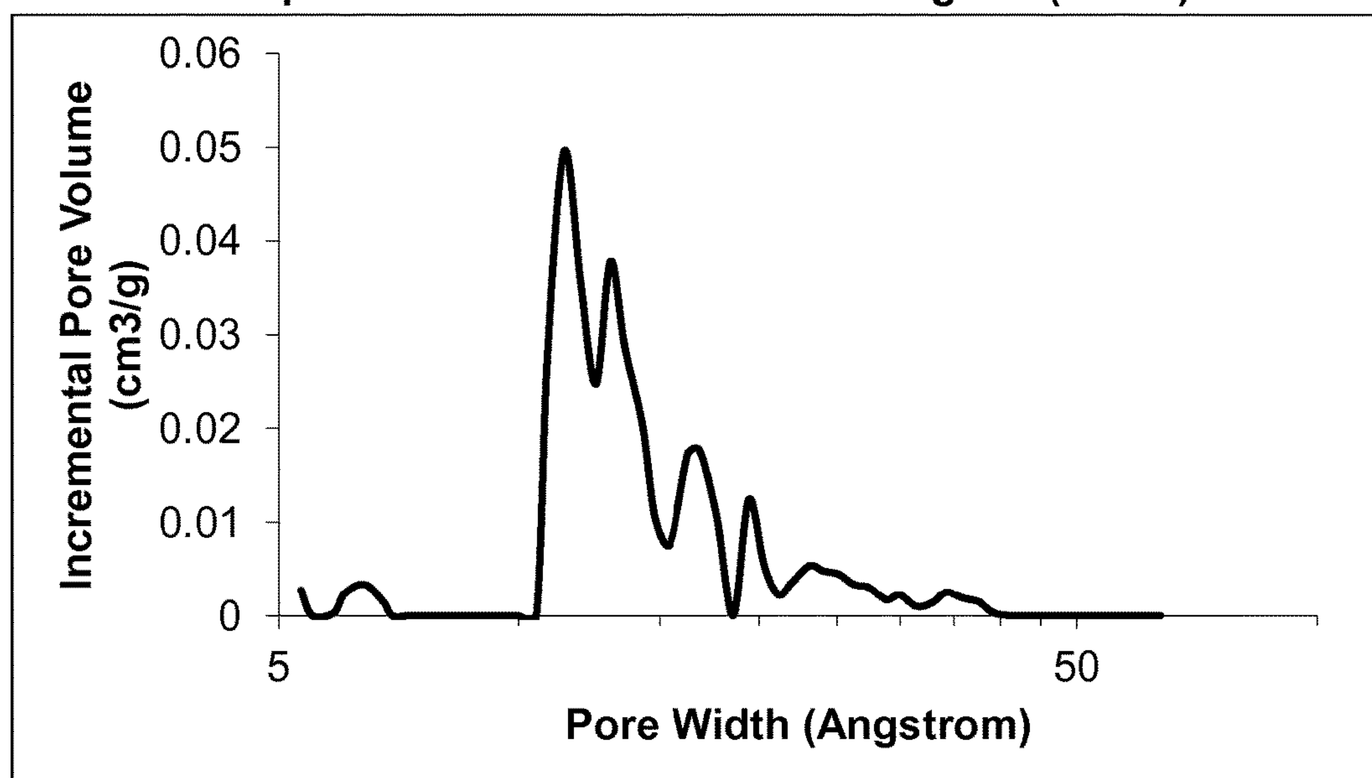
Example of Pore Size Distribution Diagram (MIB-7)
