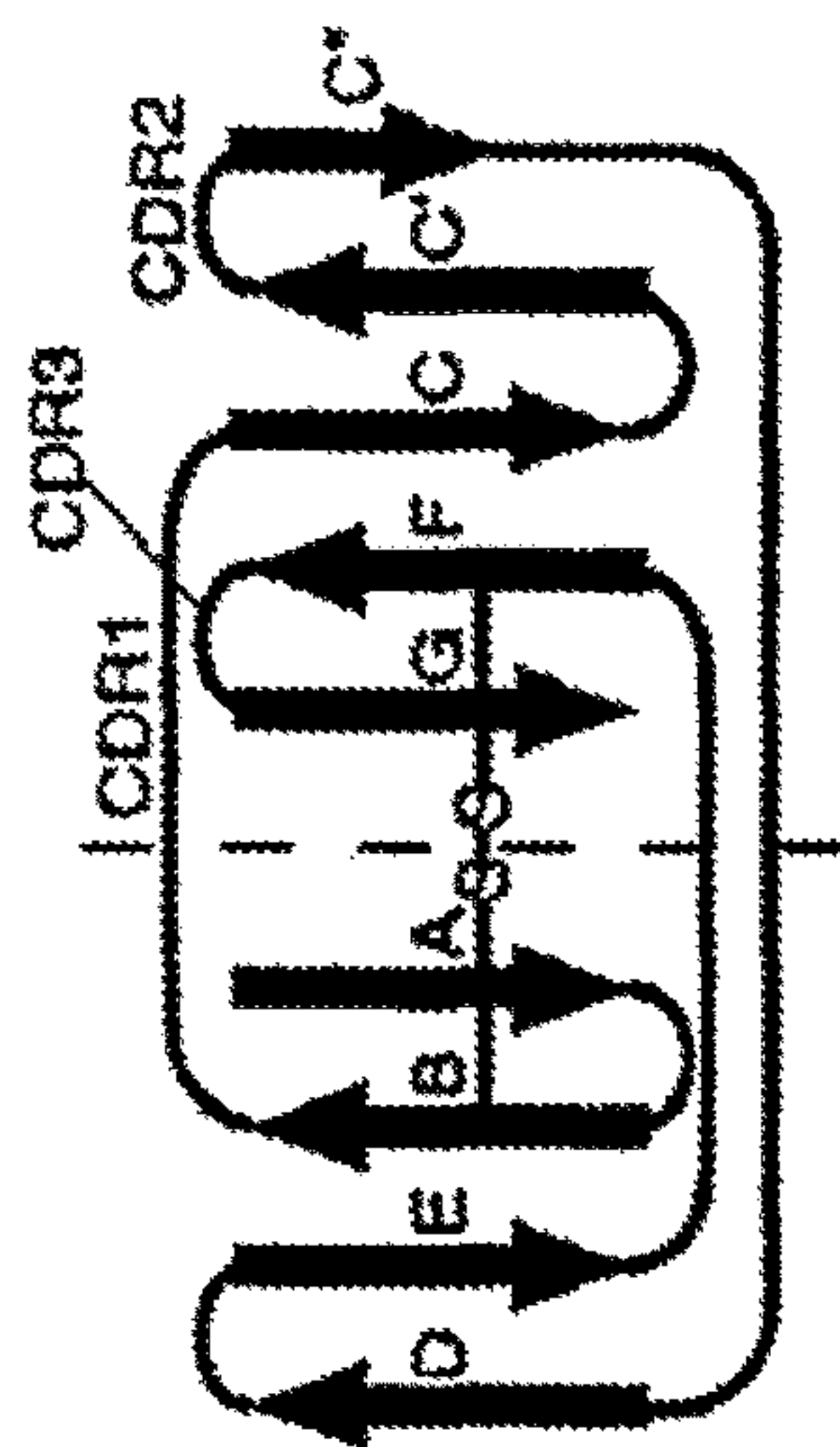
Immunoglobulin VH
