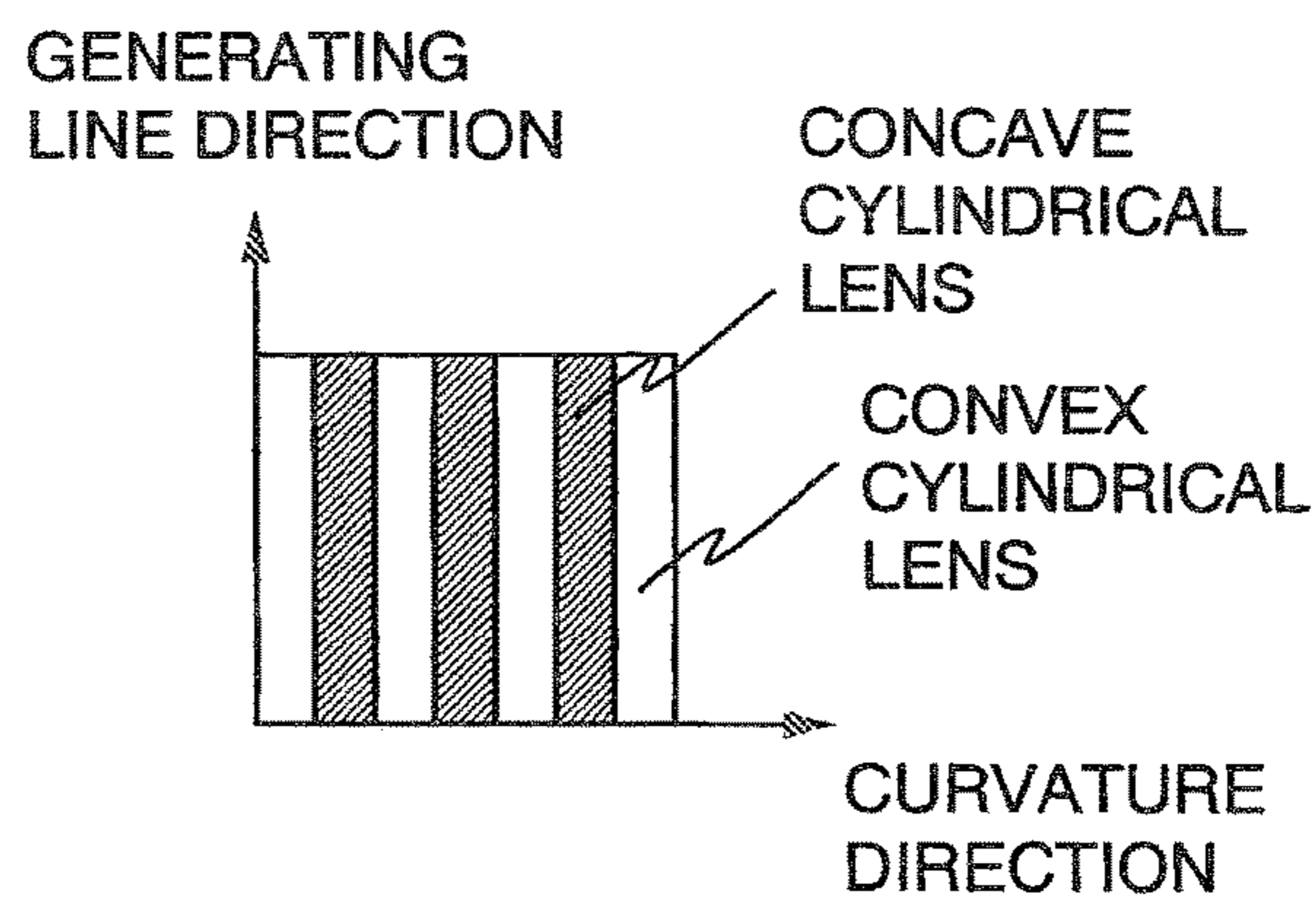
FRONT VIEW
