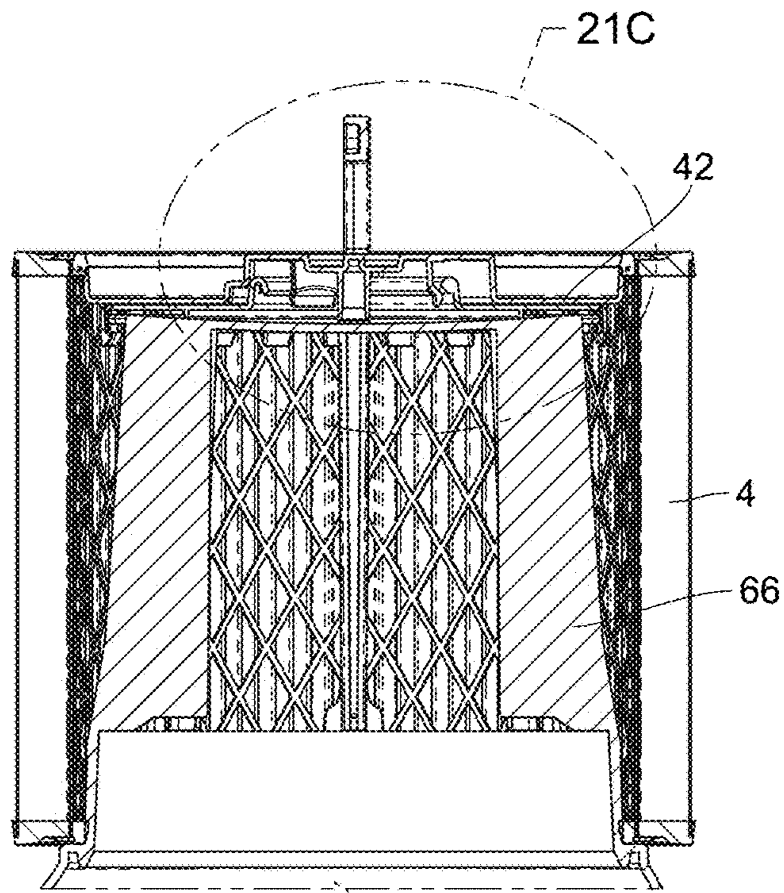
SECTION C1-C1
