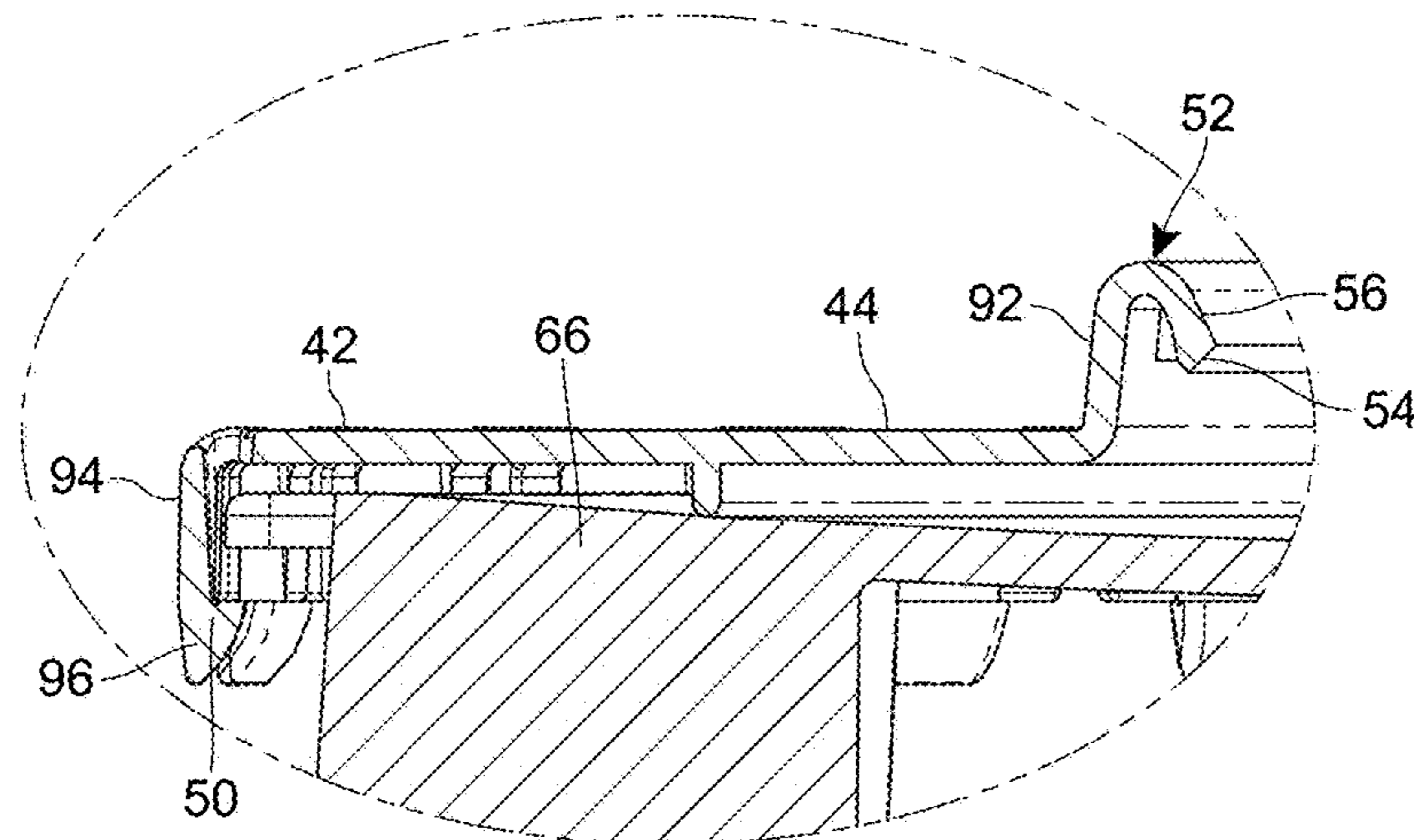
DETAIL B
