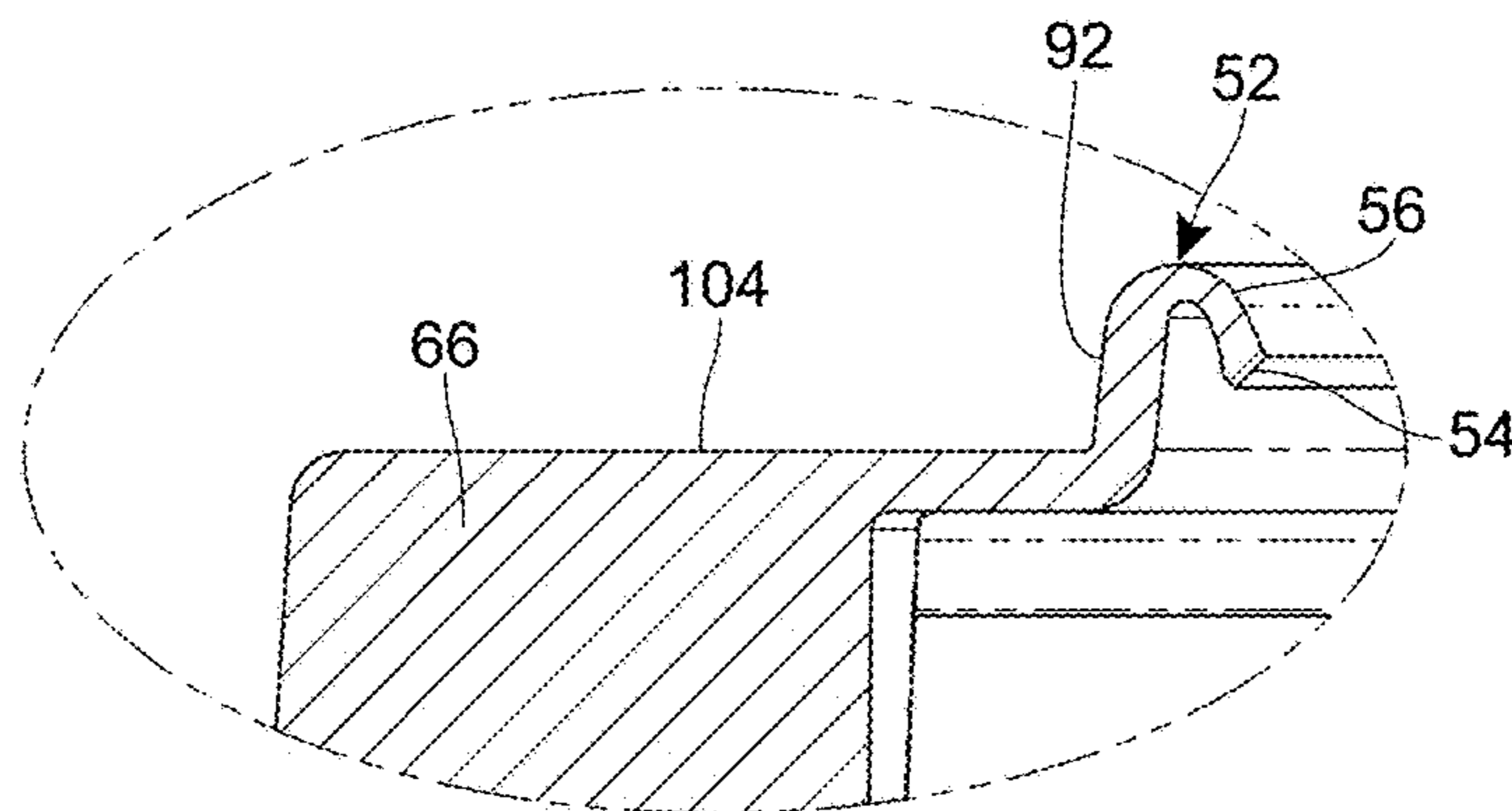
DETAIL B
