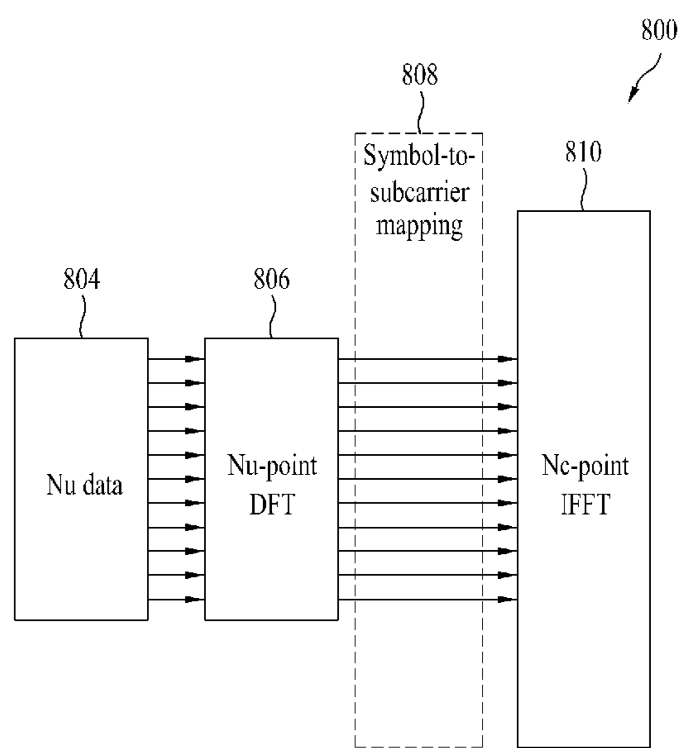
Localized DFT-s-OFDMA
