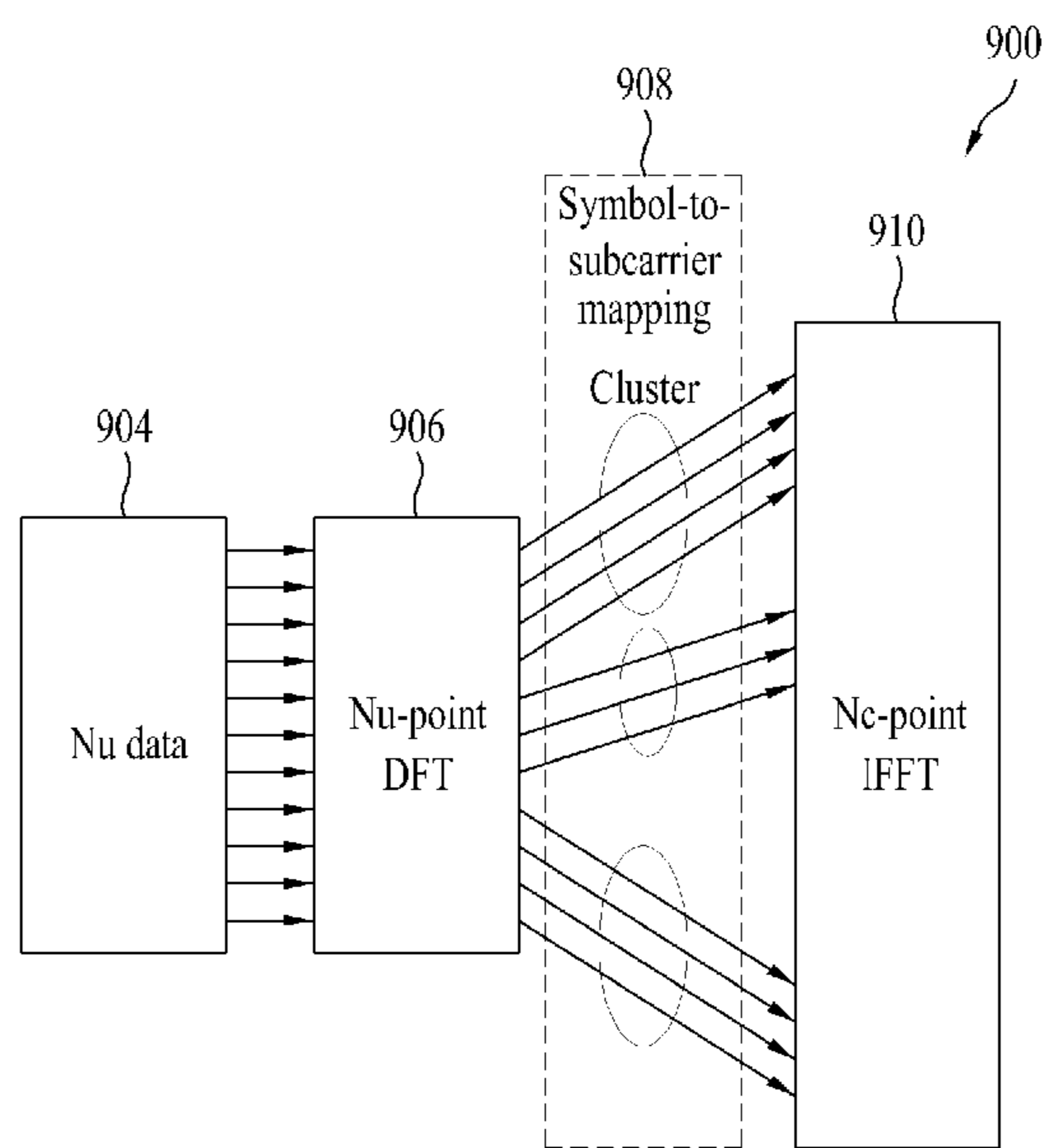
Clusters DFT-s-OFDMA
