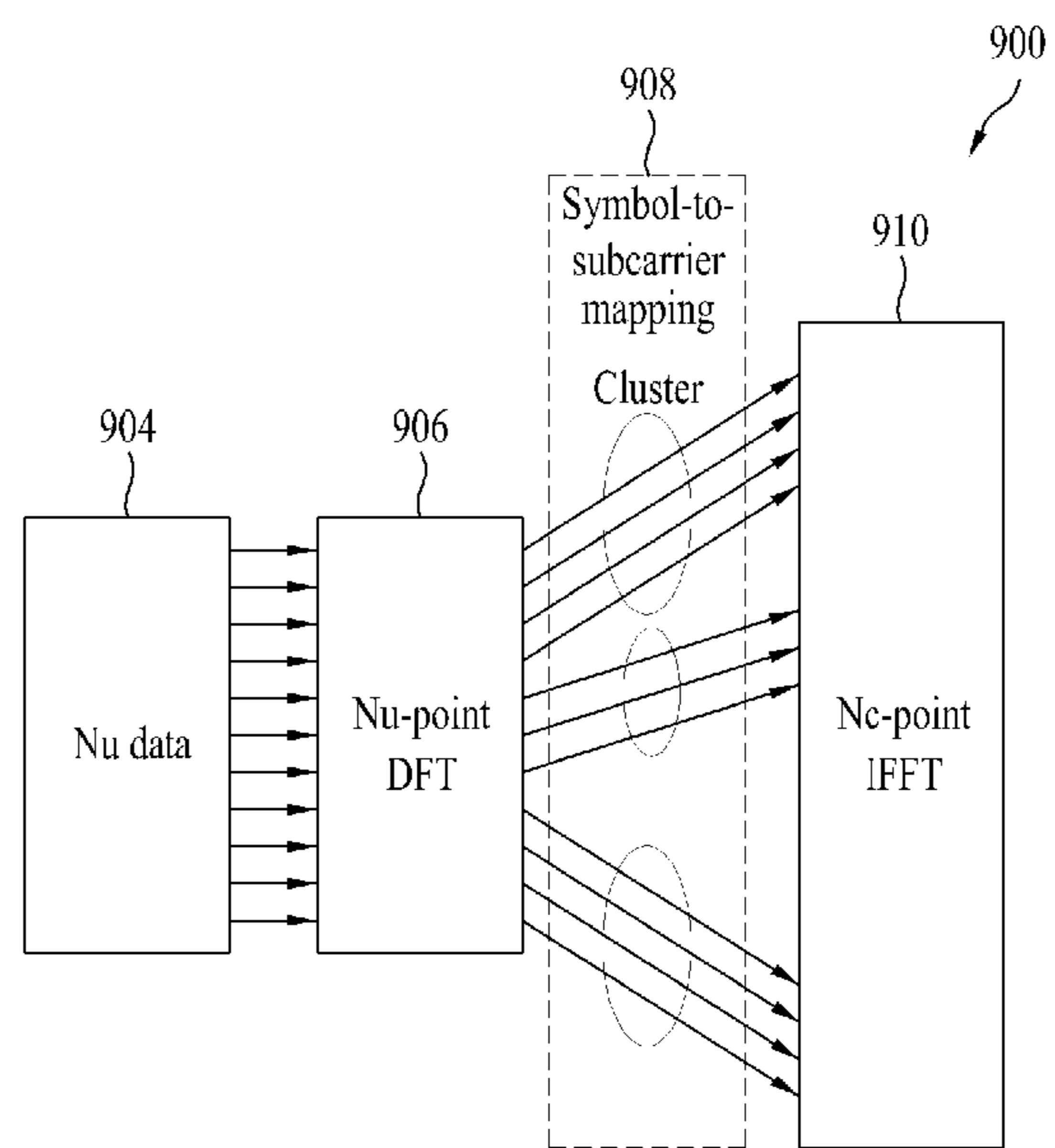
Clusted DFT-s-OFDMA
