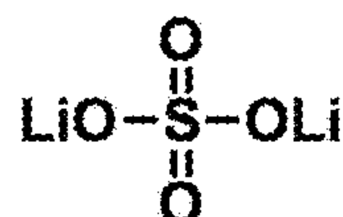
lithium sulfate
