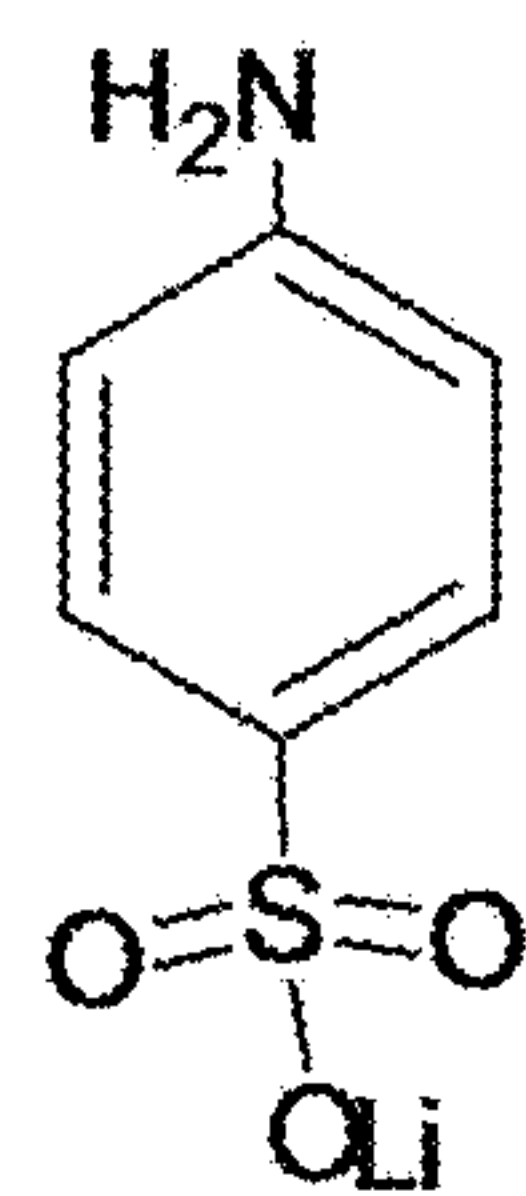
Poly(lithium-4-styrenesulfonate)
