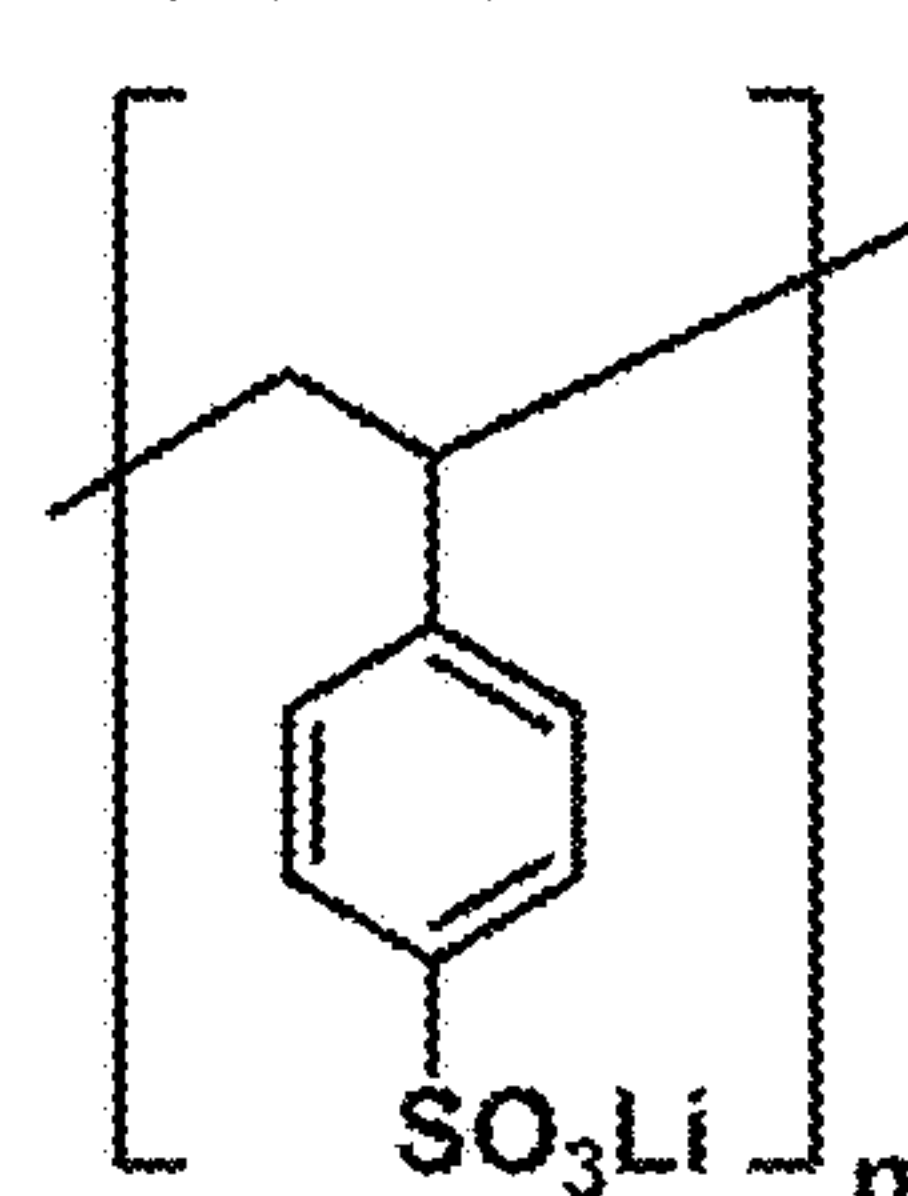
Poly(lithium-4-styrenesulfonate)
