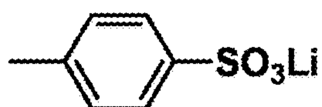
lithium 4-methylbenzenesulfonate
