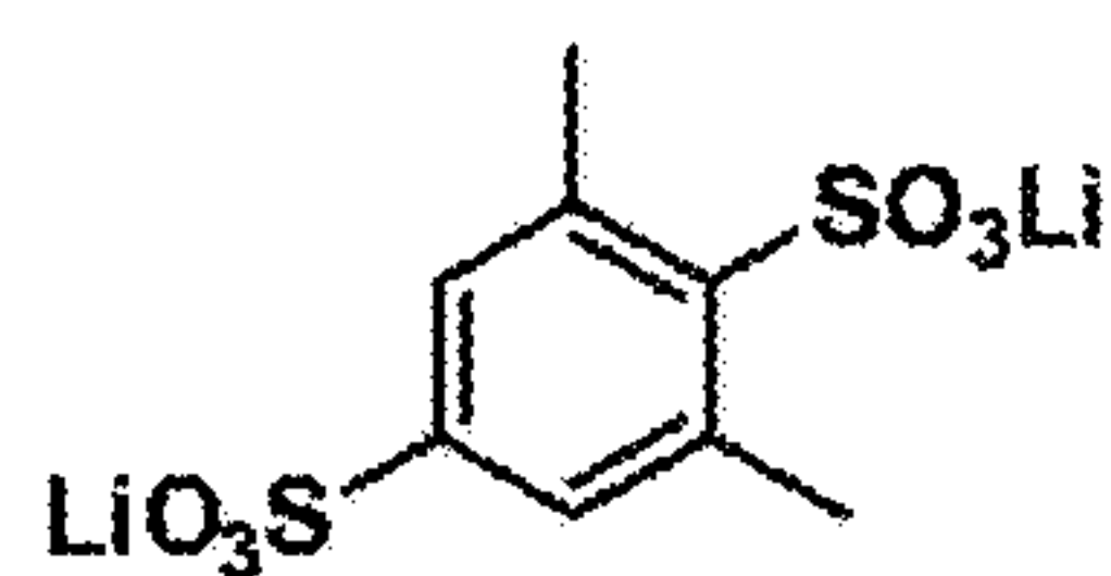
lithium 2,6-dimethylbenzene-1,4-disulfonate
