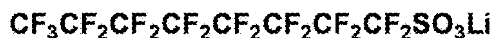
lithium 1,1,2,2,3,3,4,4,5,5,6,6,7,7,8,8,8-heptafluorooctane-1-sulfonate
