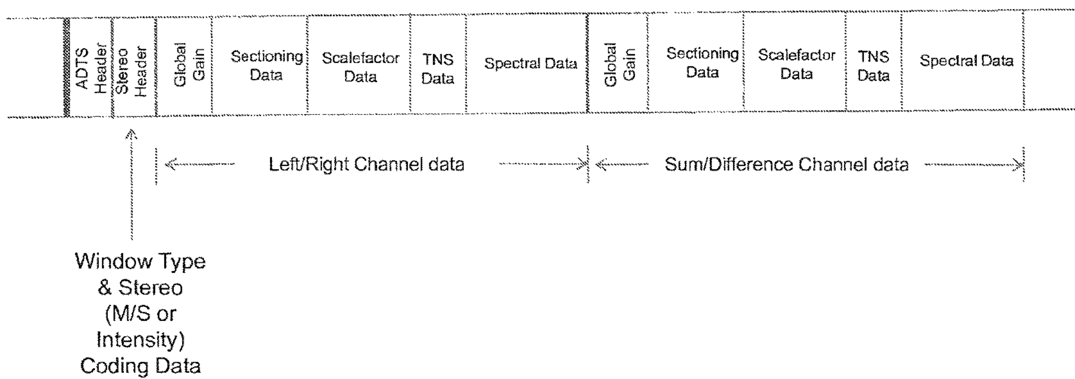
Fig. 8 – AAC Core Stereo Bitstream Packet Format
