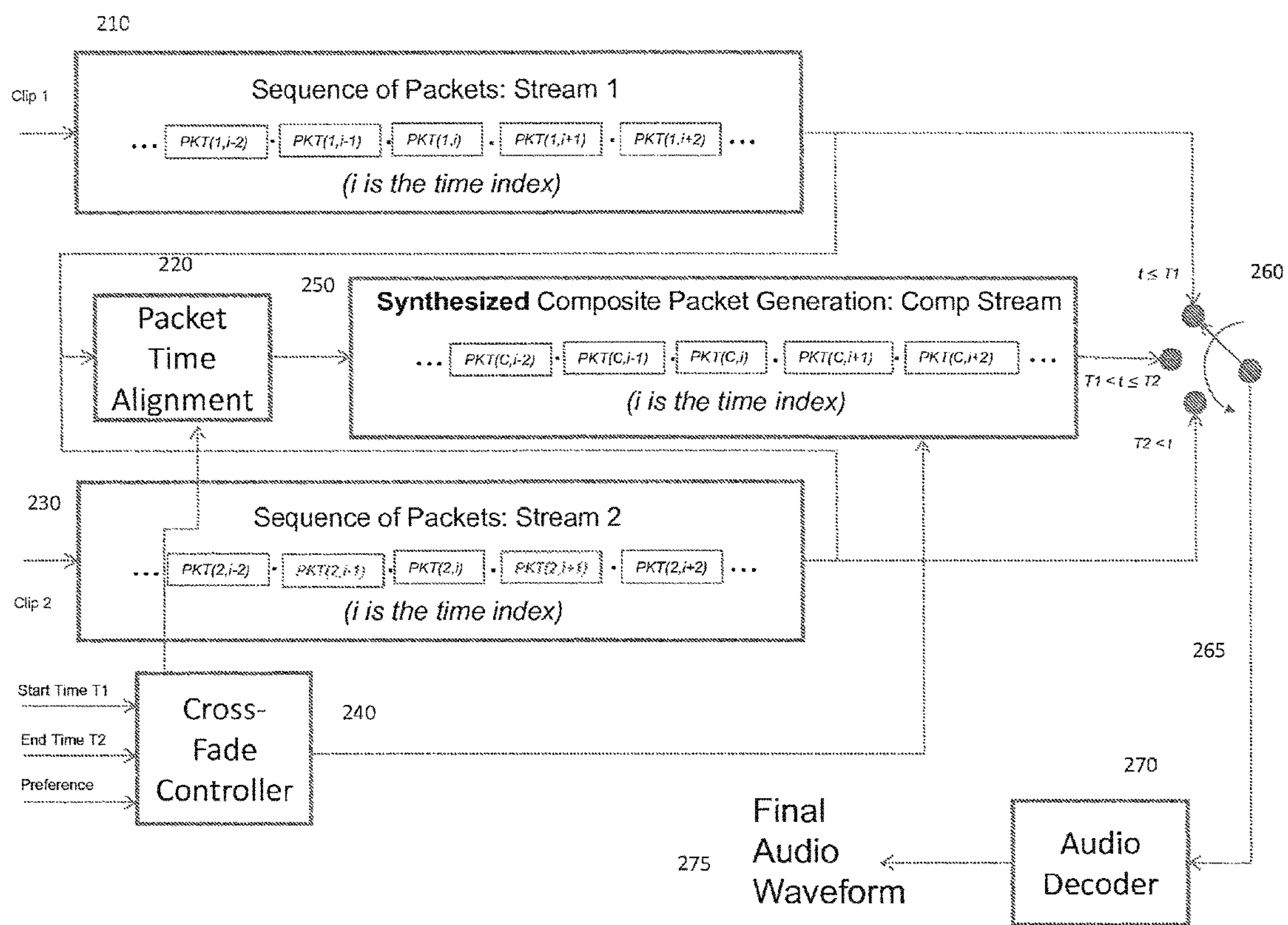
Fig. 2 - Conceptual Diagram for the Efficient Compressed Domain Cross-Fade of 2 Compressed Streams
