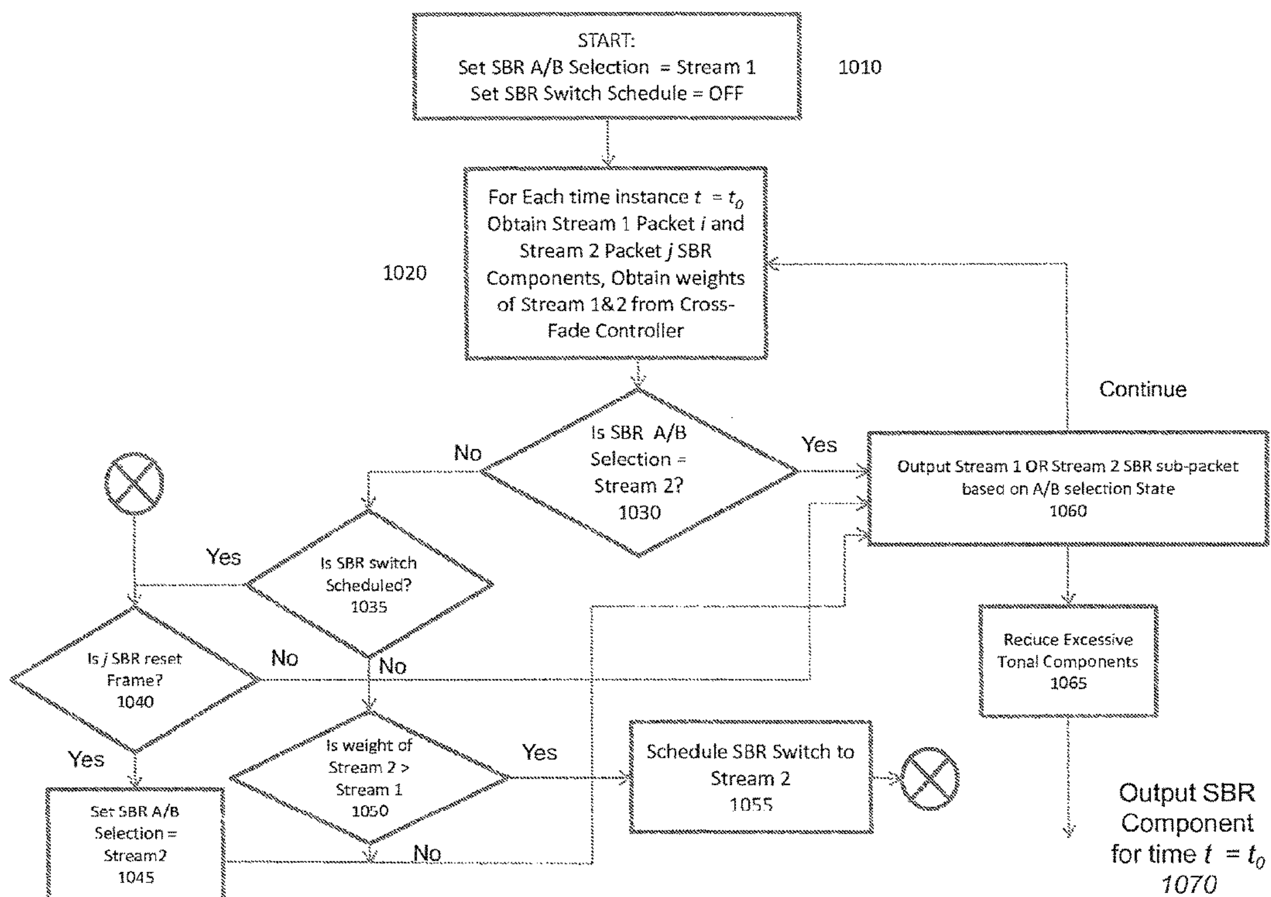
Fig. 10 - Decision Logic for the synthesis SBR component of the Composite Packet
