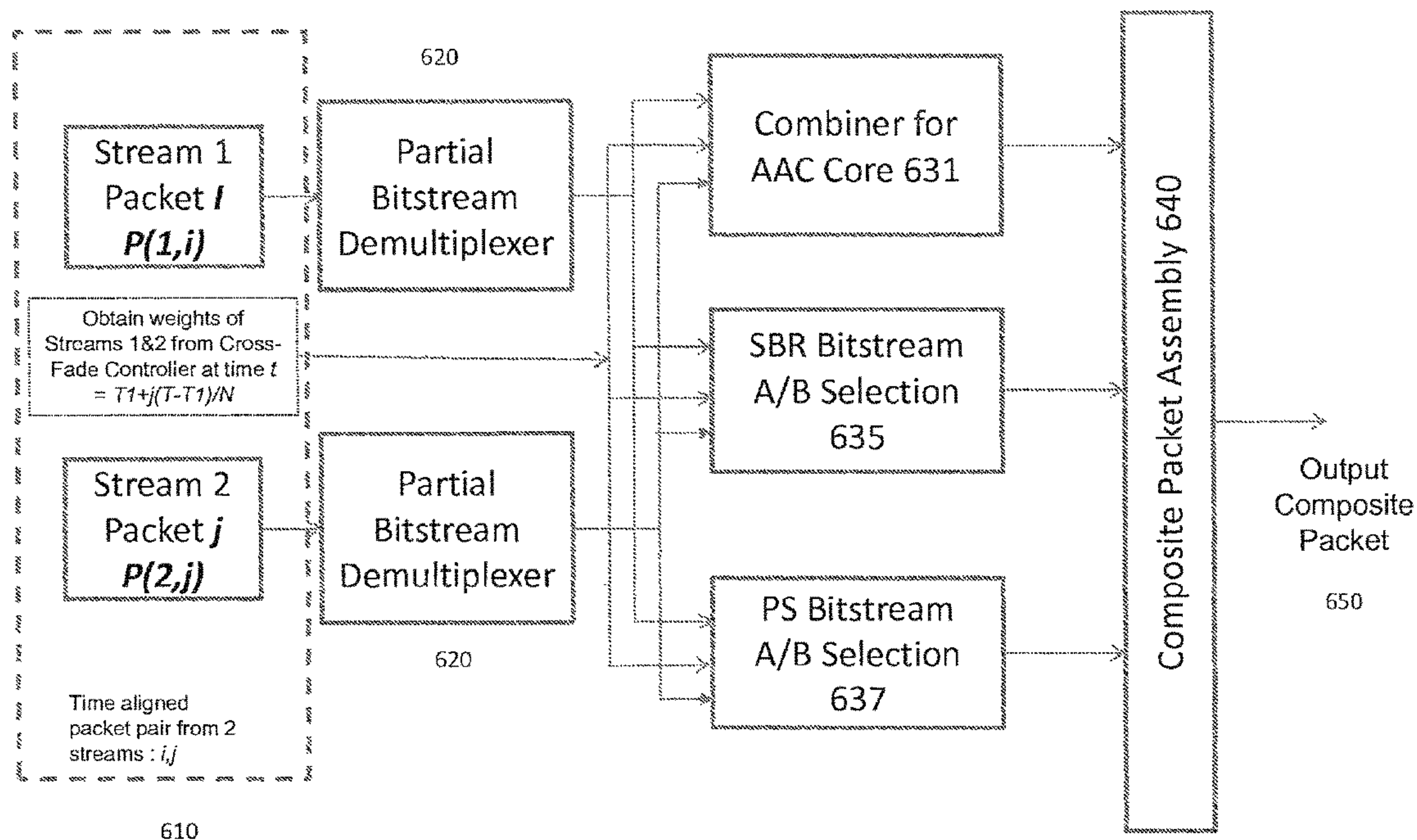
Fig. 6 – Overview of Composite Compressed Packet Synthesis Scheme for Enhanced AAC Plus Streams
