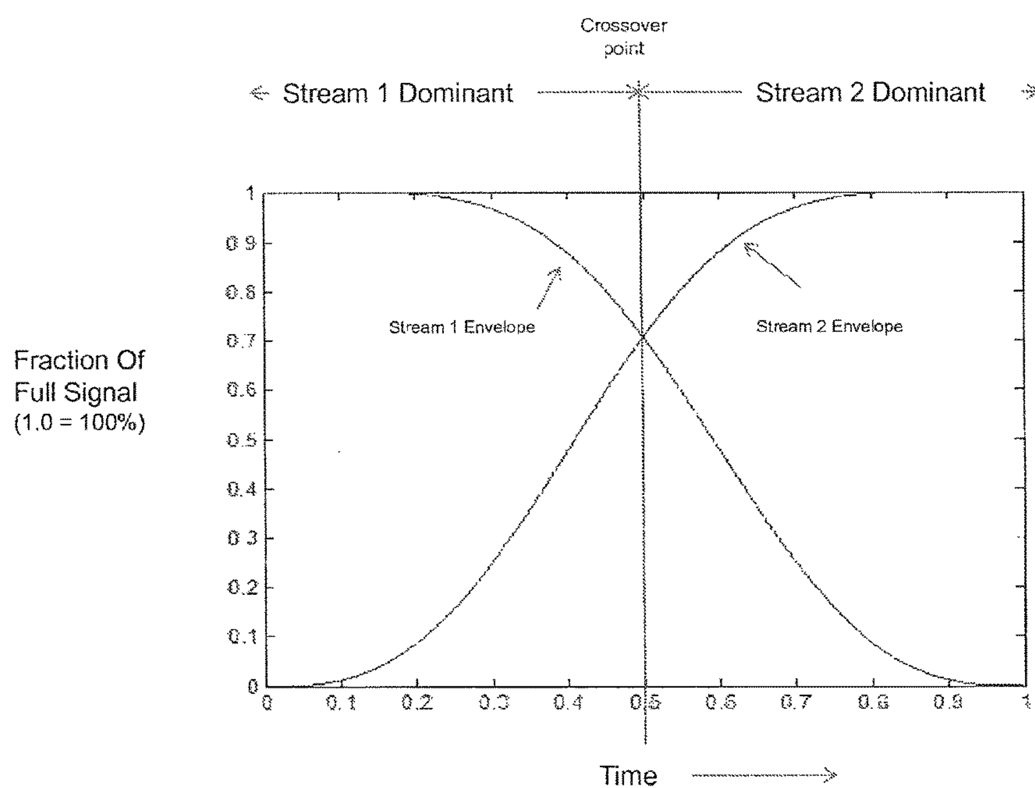
Fig. 7 – Exemplary Power-Complementary Smooth Cross-fade Window Of Order 3 Maximizing The Duration Of A Dominant Stream
