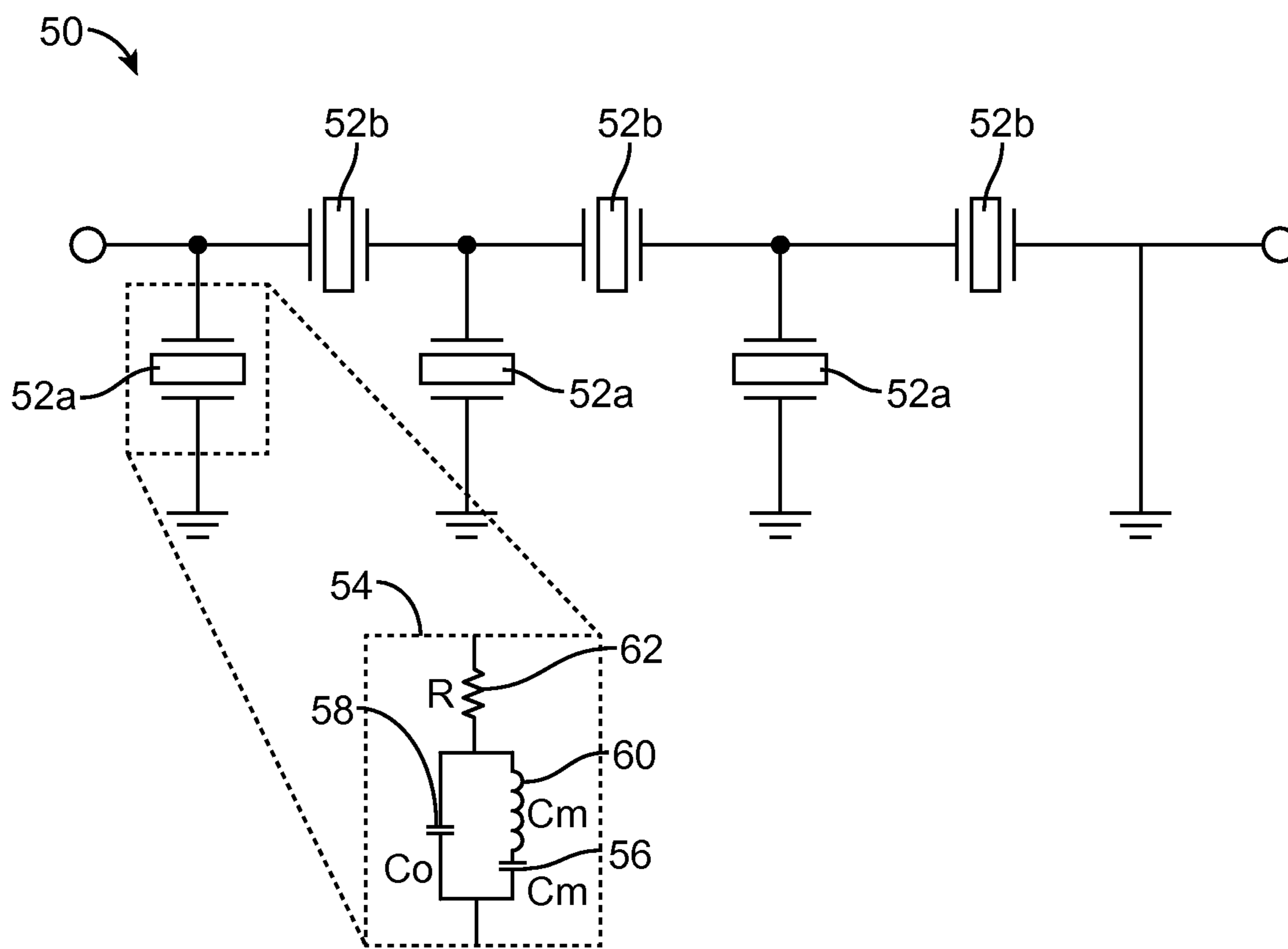
FIG. 2 (PRIOR ART)
