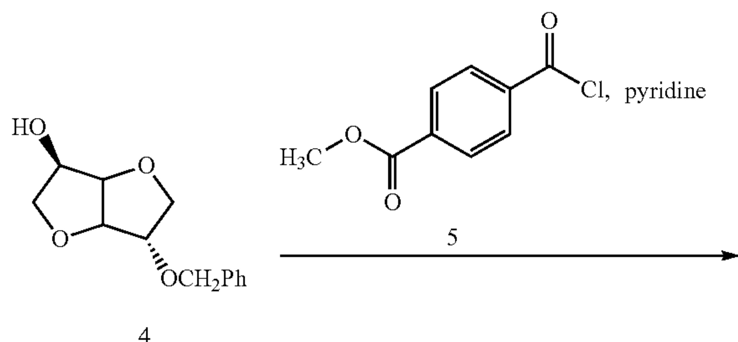
Scheme 1: Isosorbide 5-(4-carbomethoxybenzoate), Isosorbide 5-TA AB monomer 1
