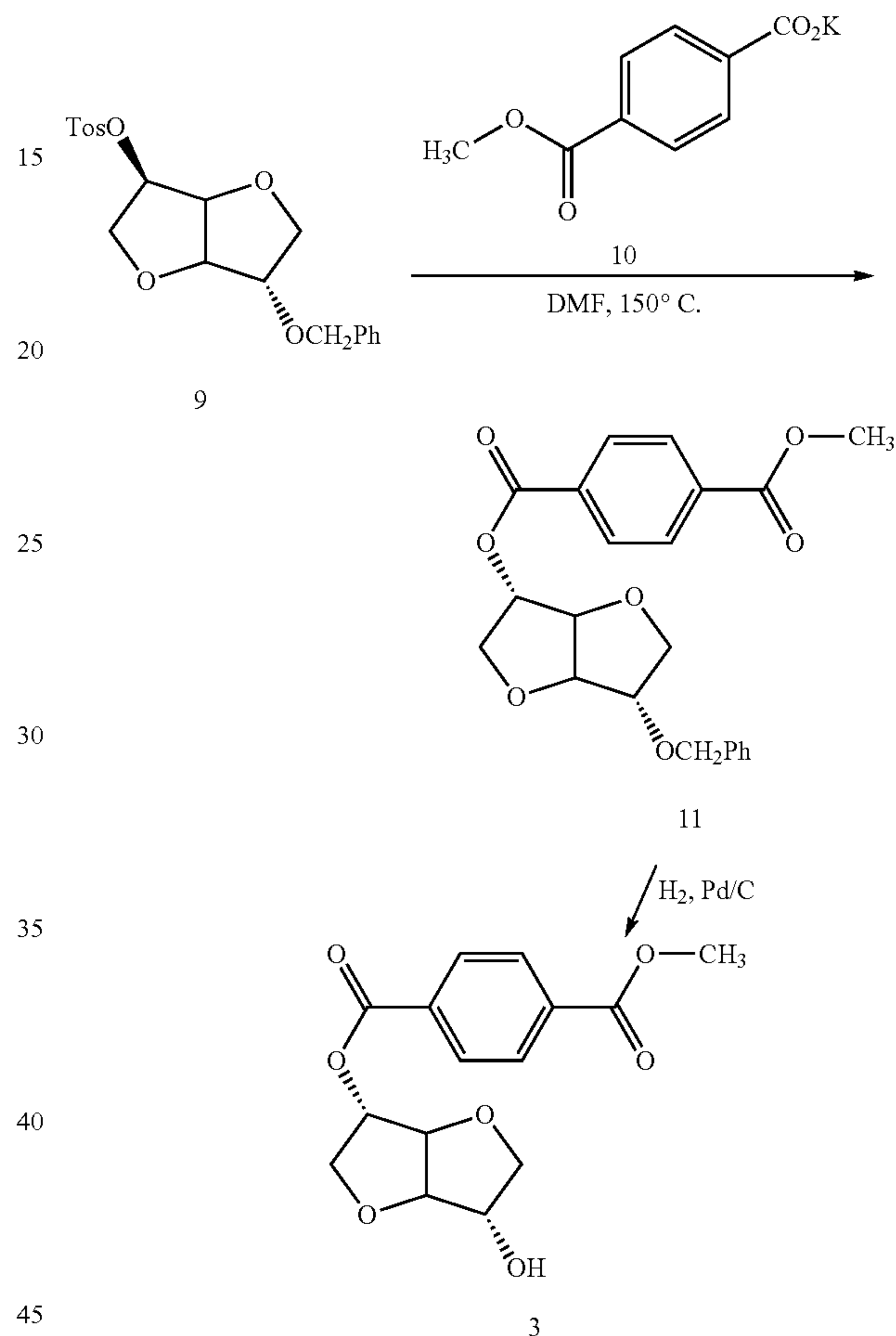
Scheme 3: Isoidide 2-(4-carbomethoxybenzoate), Isoidide 2-TA AB monomer
