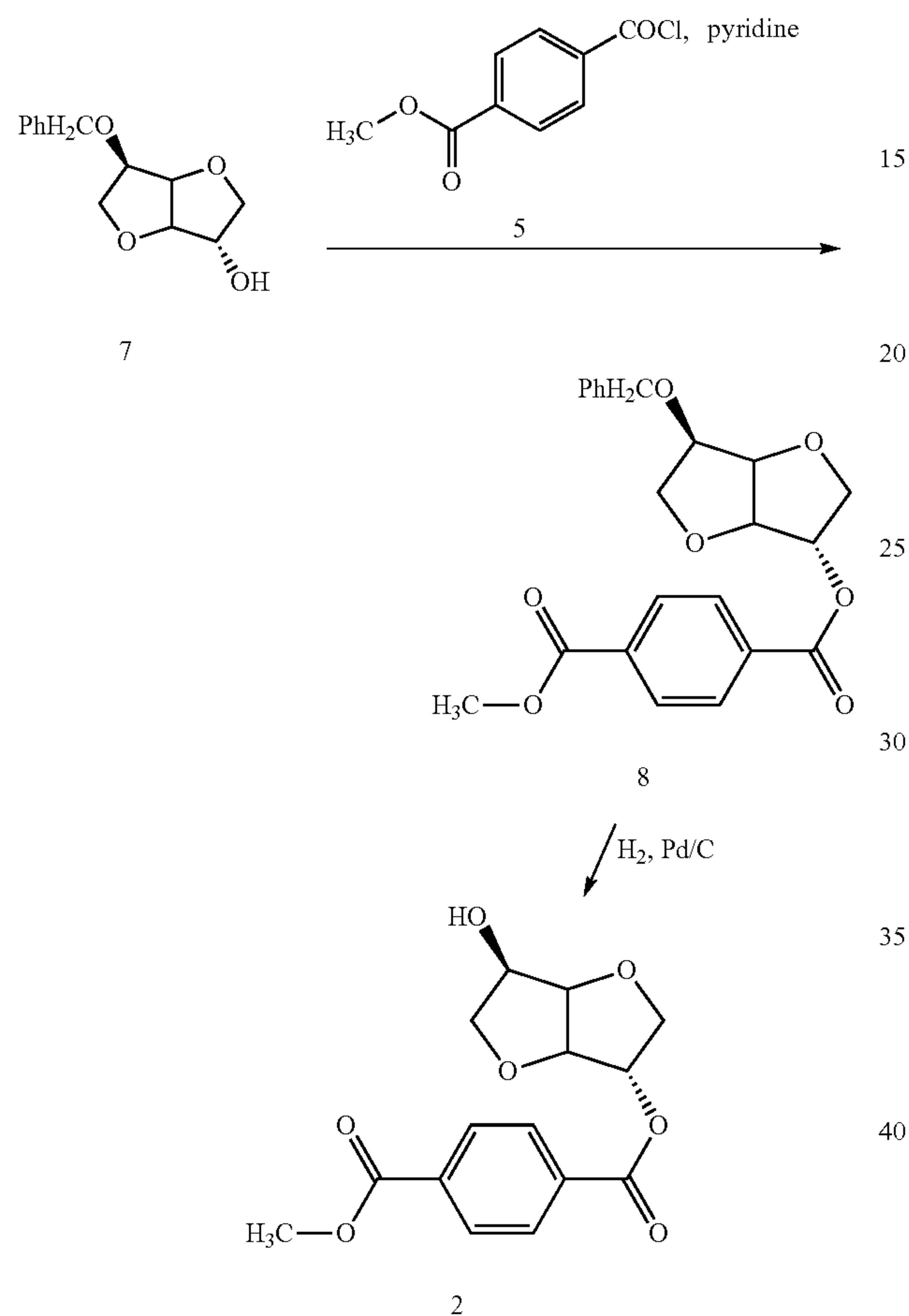
Scheme 2: Isosorbide 2-(4-carbomethoxybenzoate), Isosorbide 2-TA AB monomer (2)
