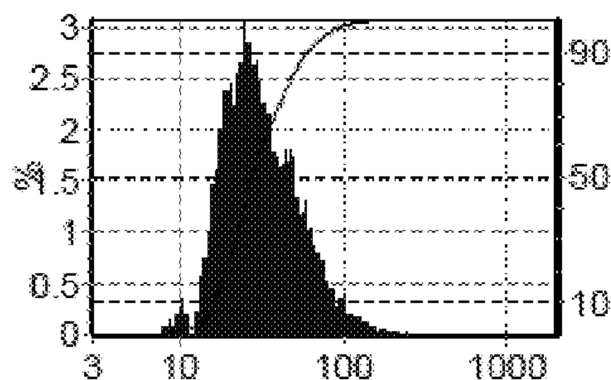
Feret Length
