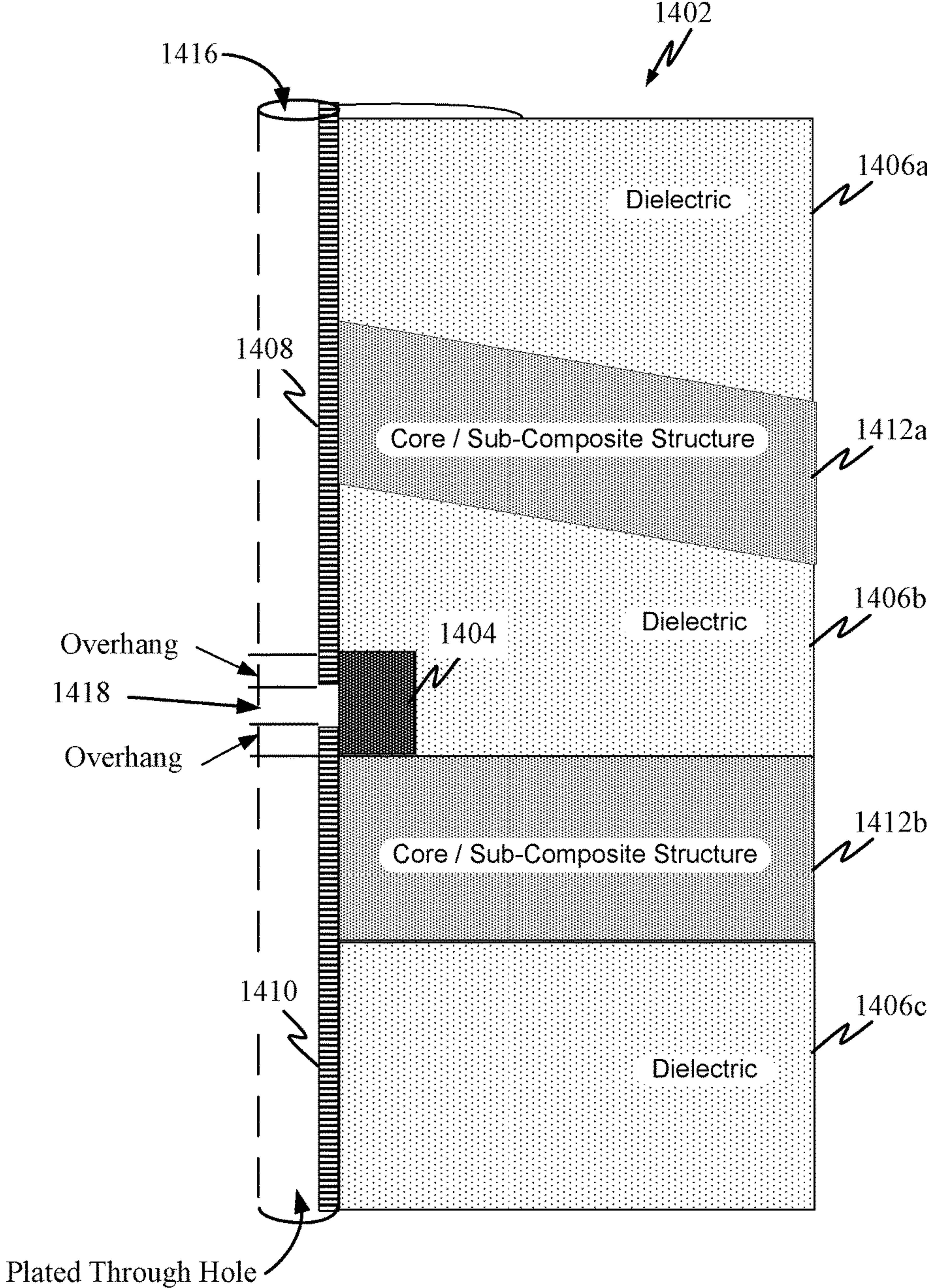
FIG. 14 (Practical Structure)
