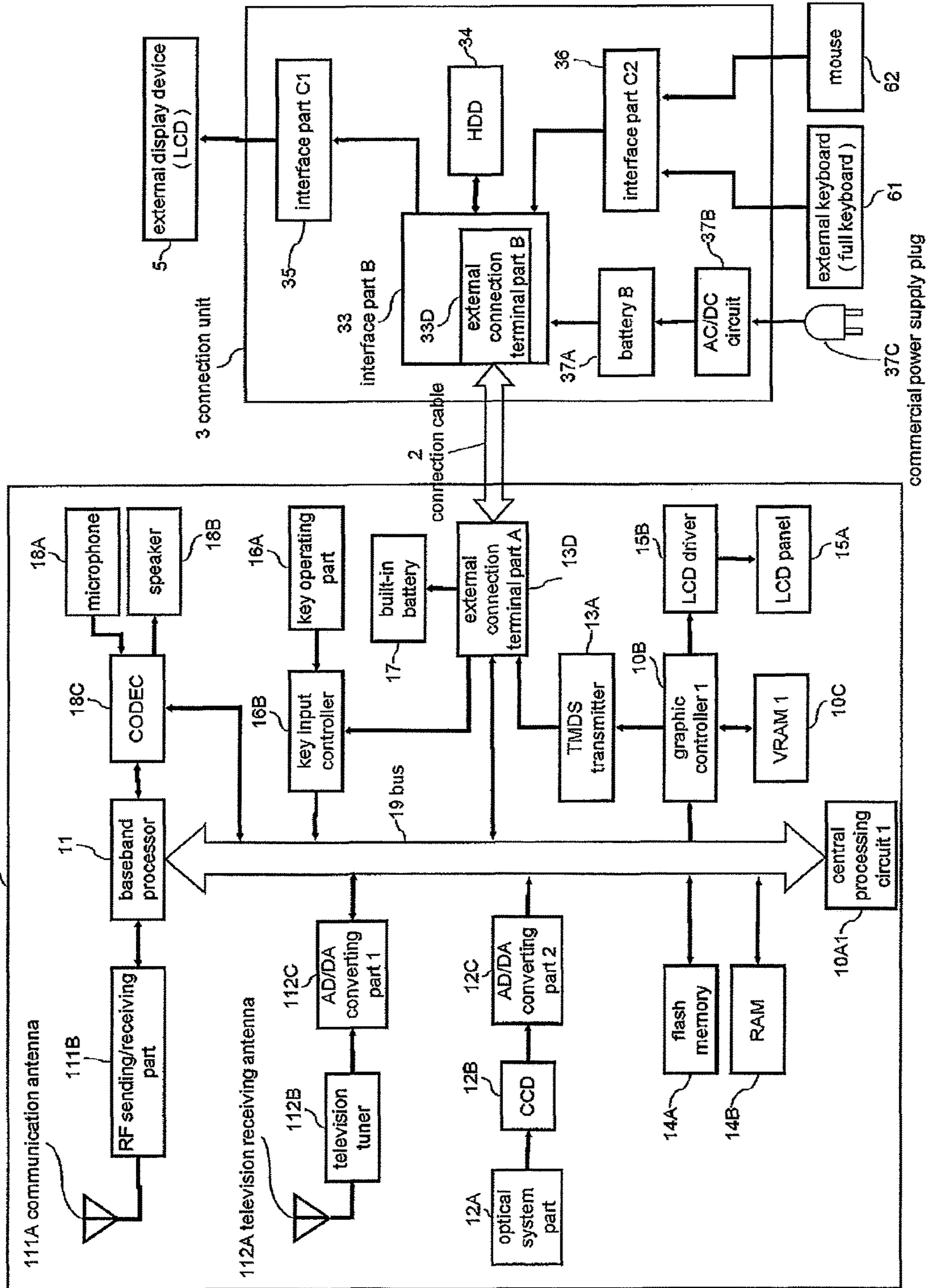
FIG. 1 1 mobile telephone unit
