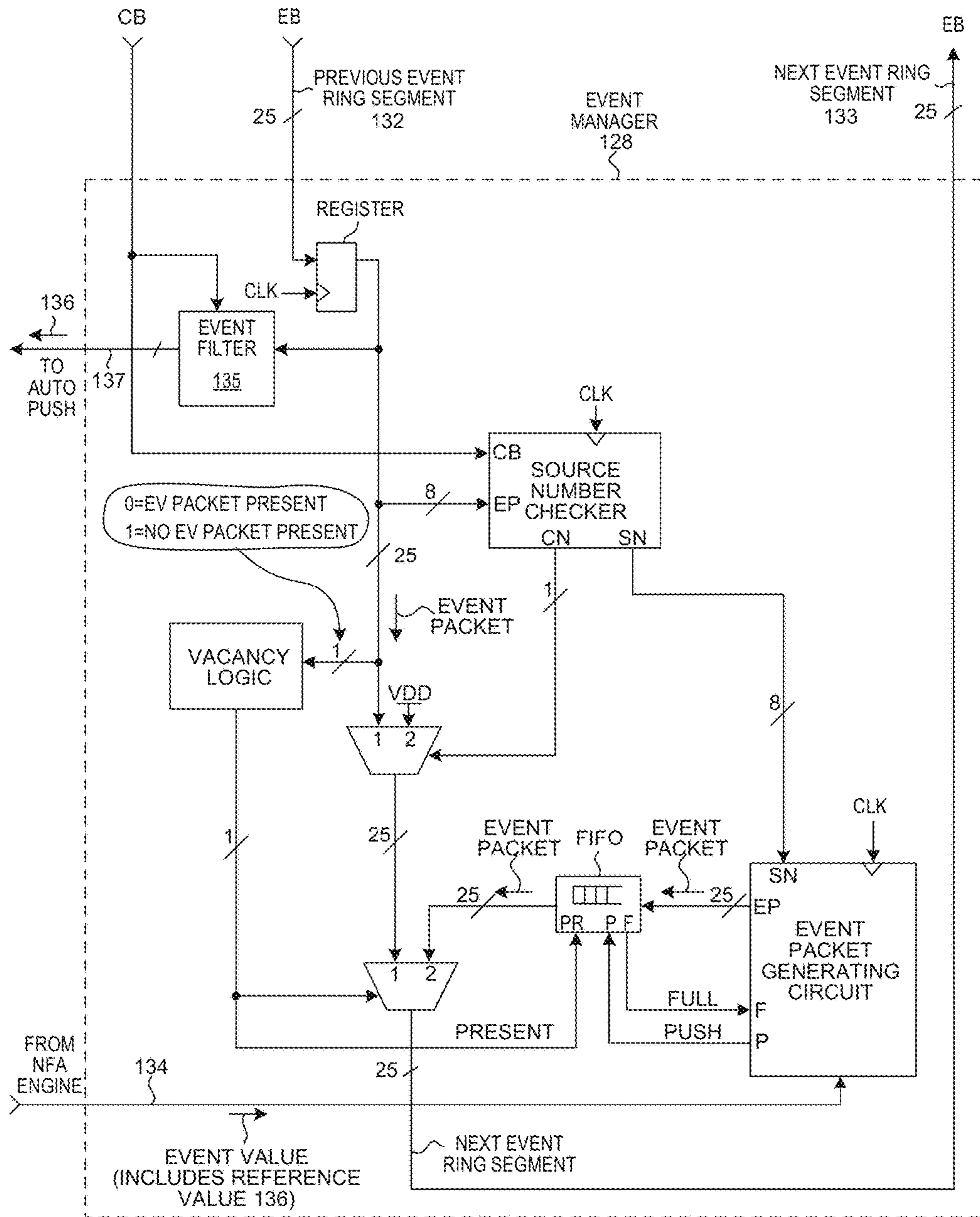
EVENT MANAGER ("EVENT RING CIRCUIT") FIG. 7
