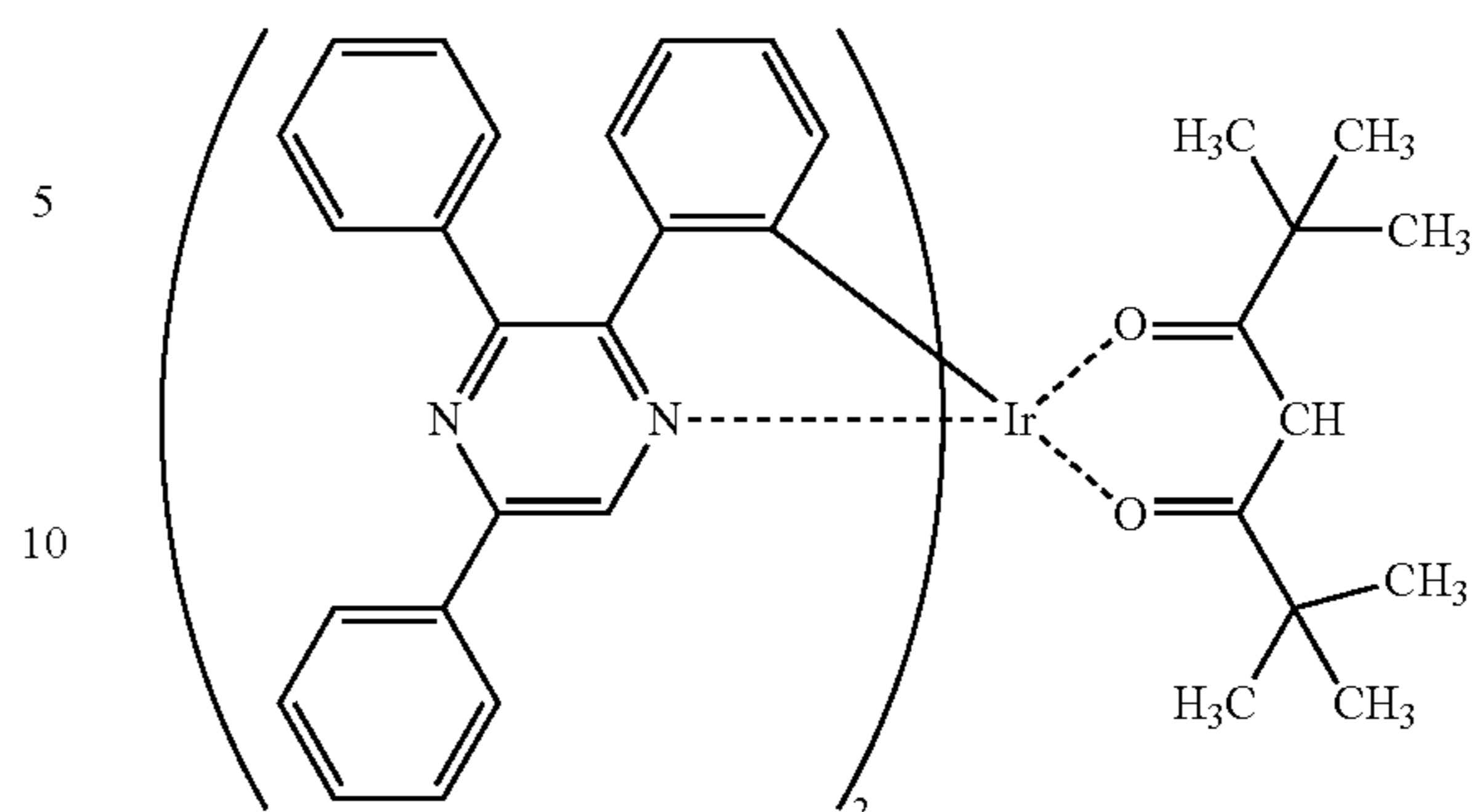
Ir(tppr) 2 (dpm)
