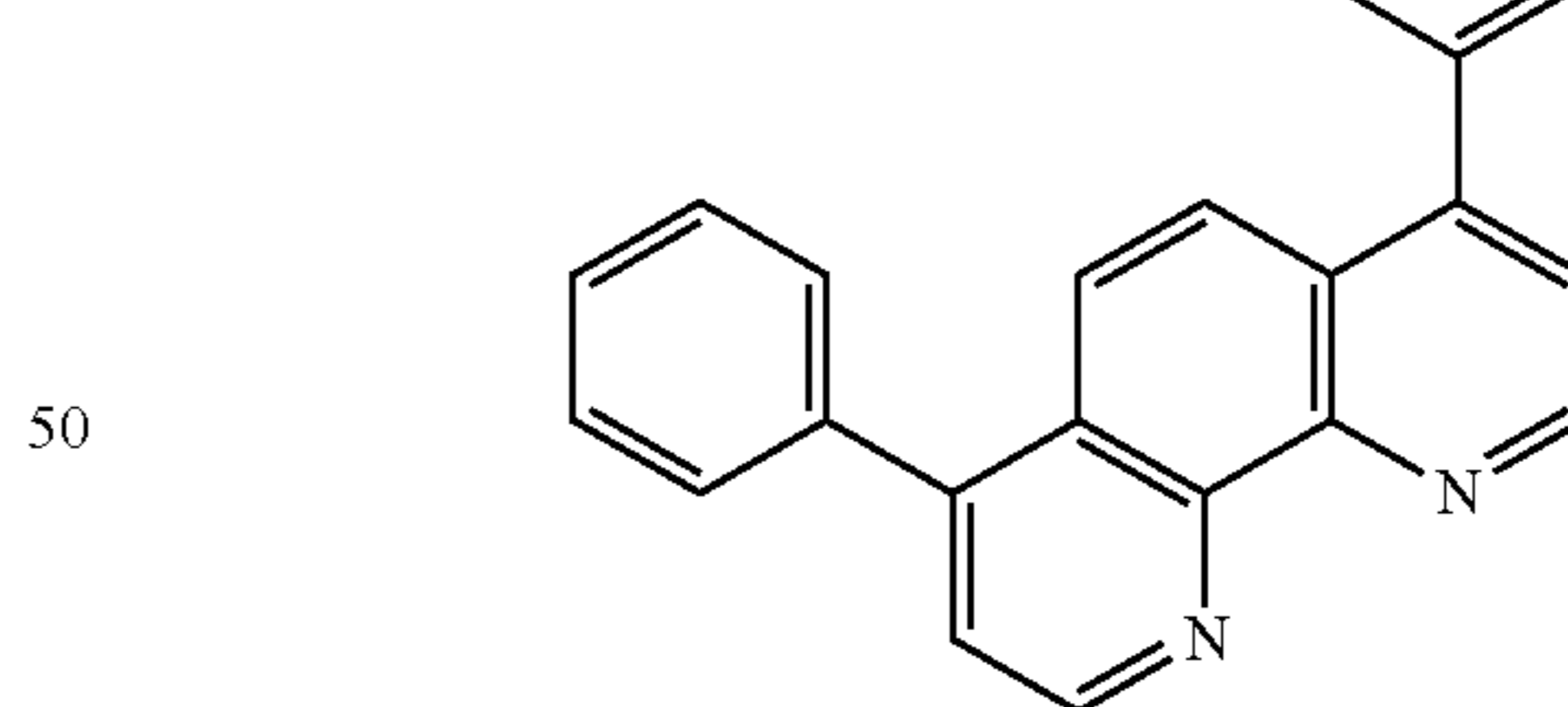
BPhen
