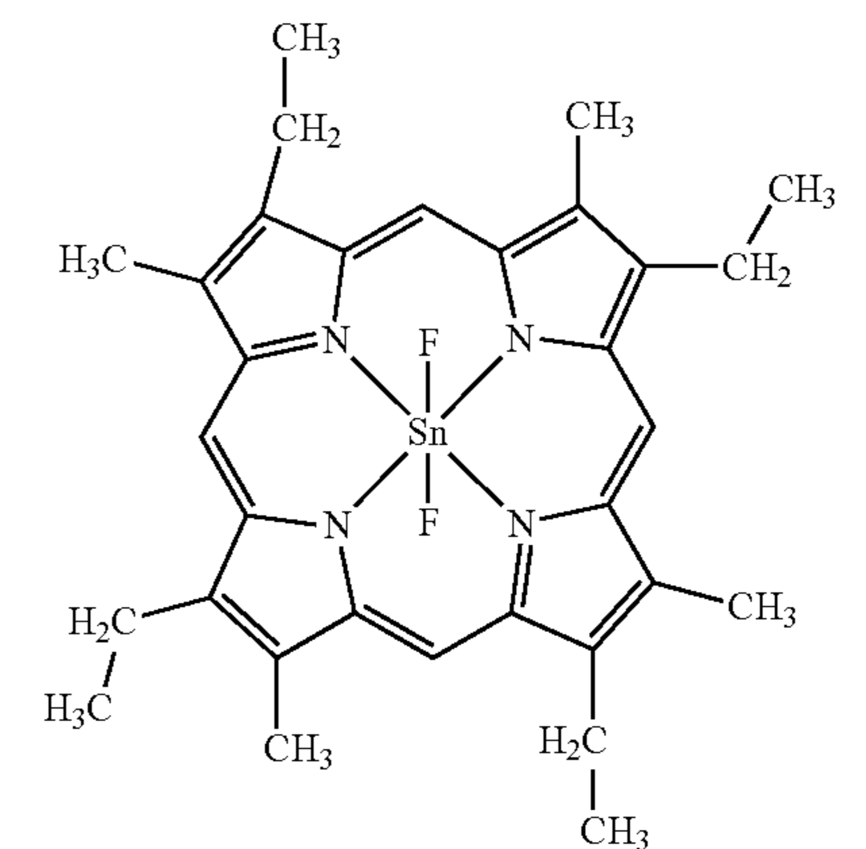
\text{SnF}_2(\text{Etio I})
