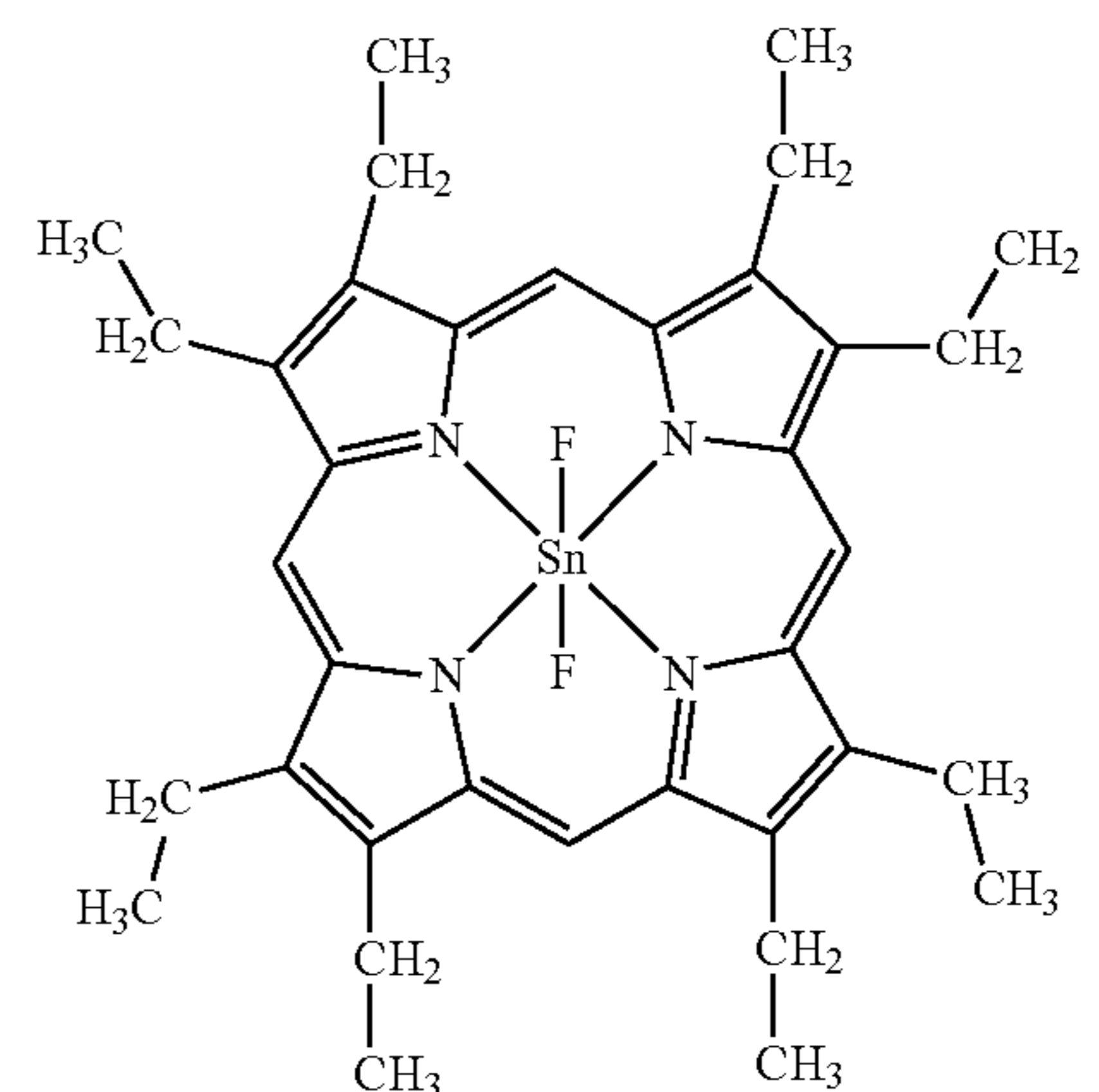
\text{SnF}_2(\text{OEP})
