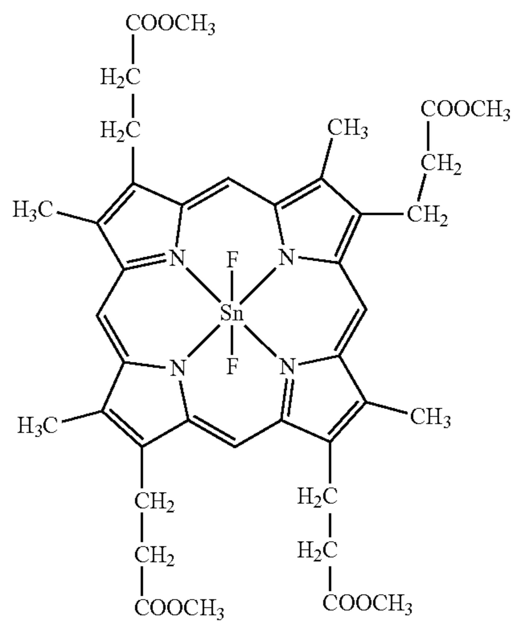
\text{SnF}_2(\text{Copro III-4Me})
