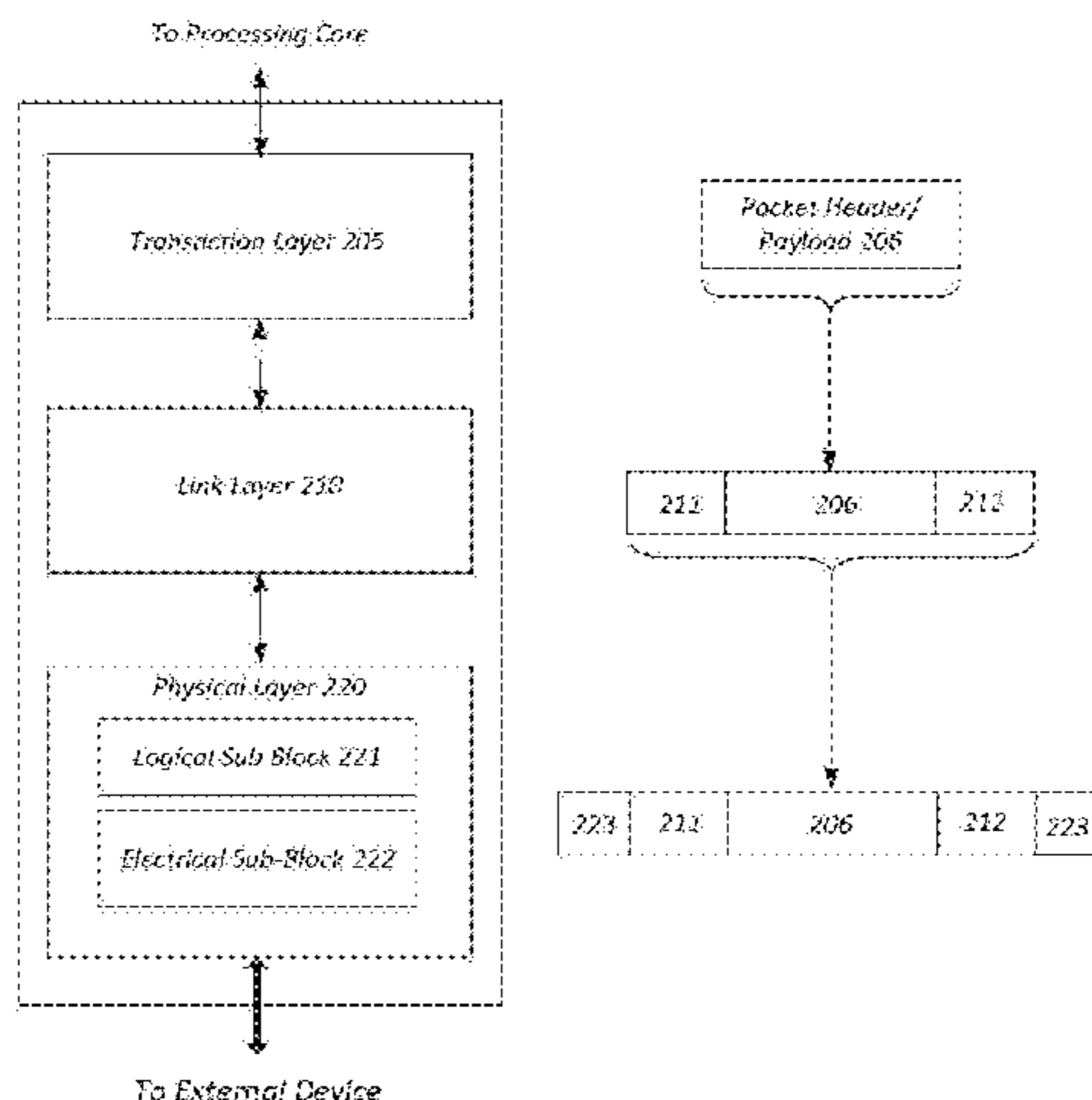
Layered Protocol Stack 208
