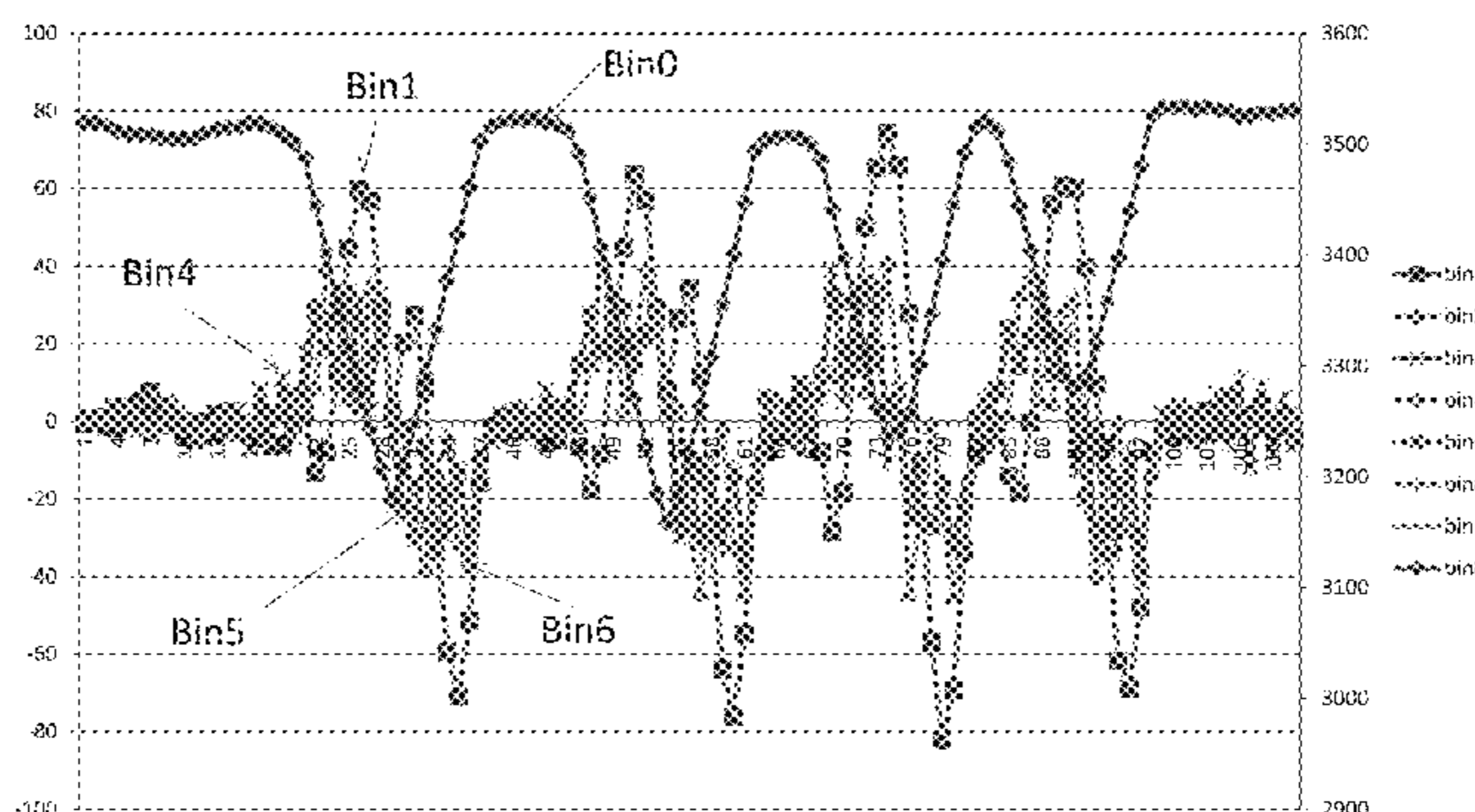
FFT of Fig 3 (Real data shown bins 0-7)
