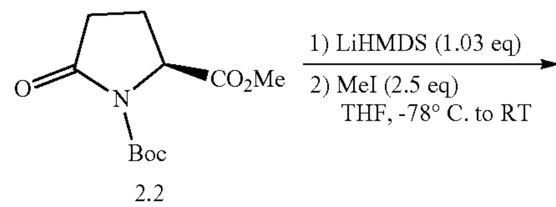
Scheme 8: Synthesis of methyl substituted pyrrolidinone intermediates
