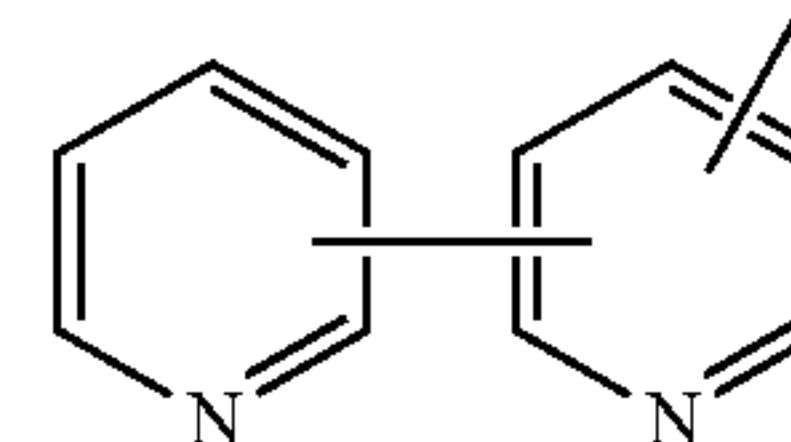
bipyridinyl
