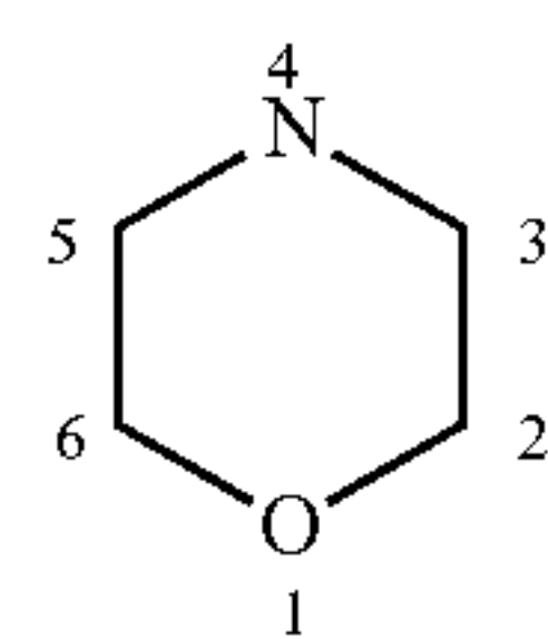
morpholinyl
