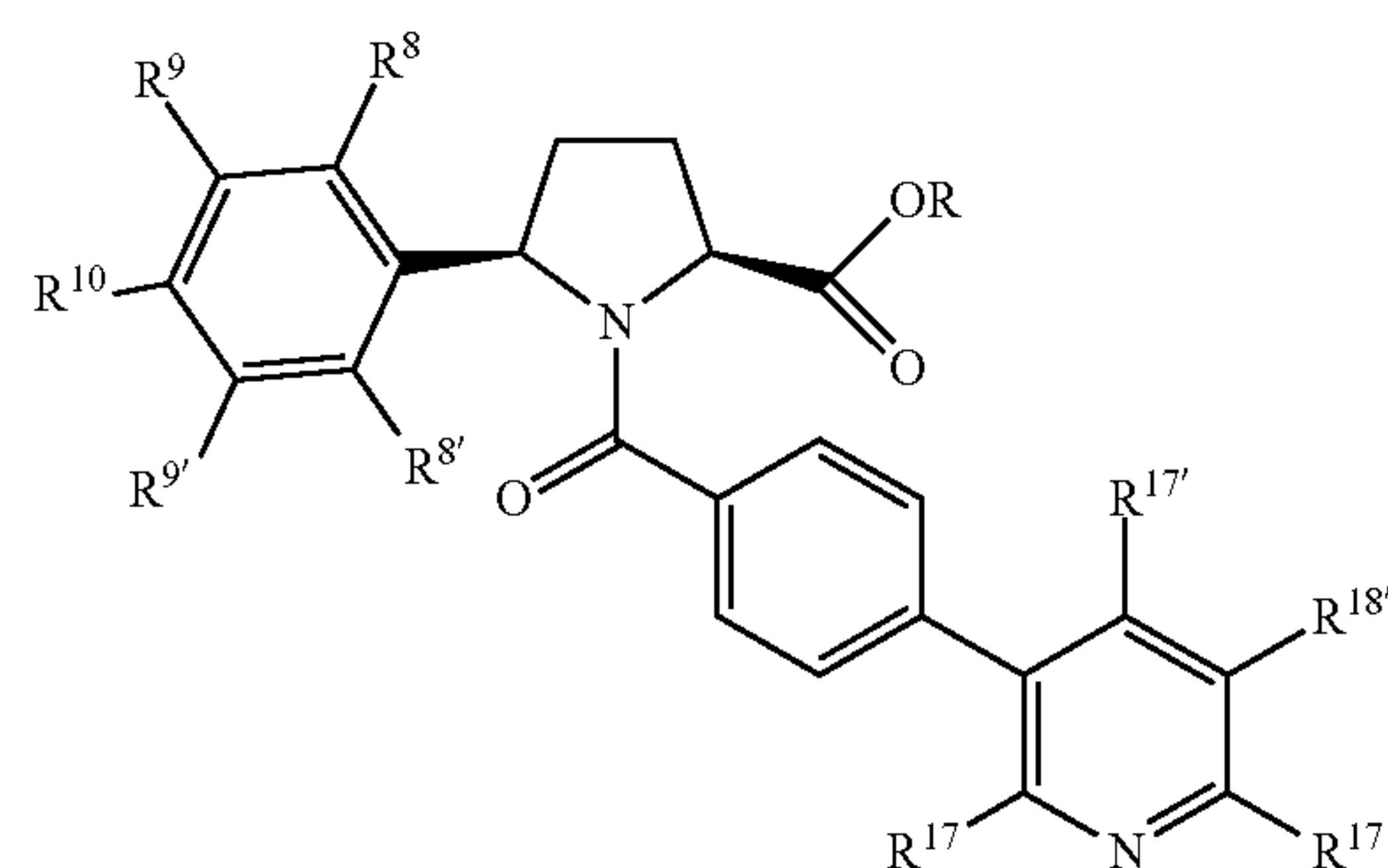
Ib-1g1a
