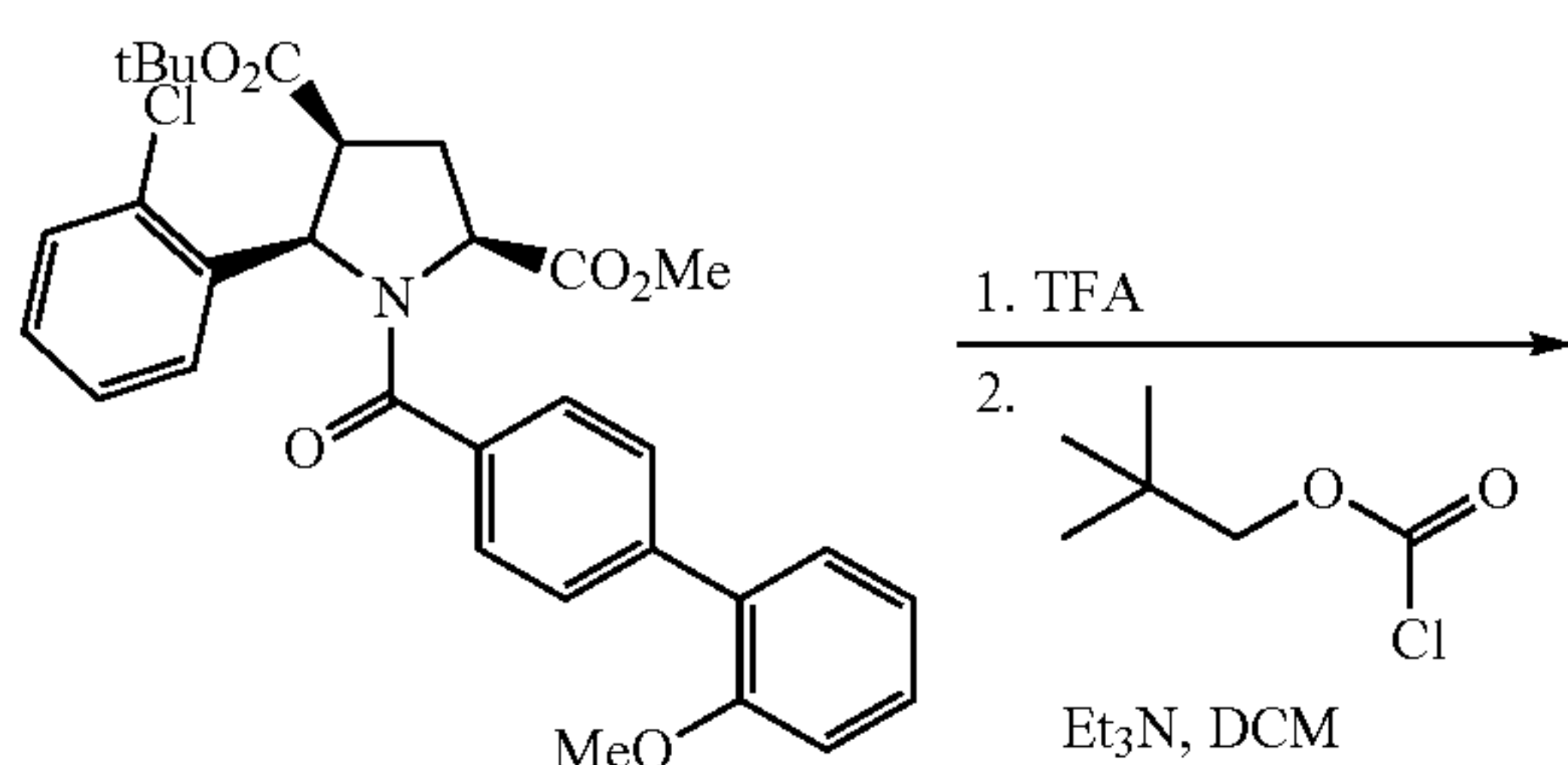
Scheme 14: synthesis of compound n°279
