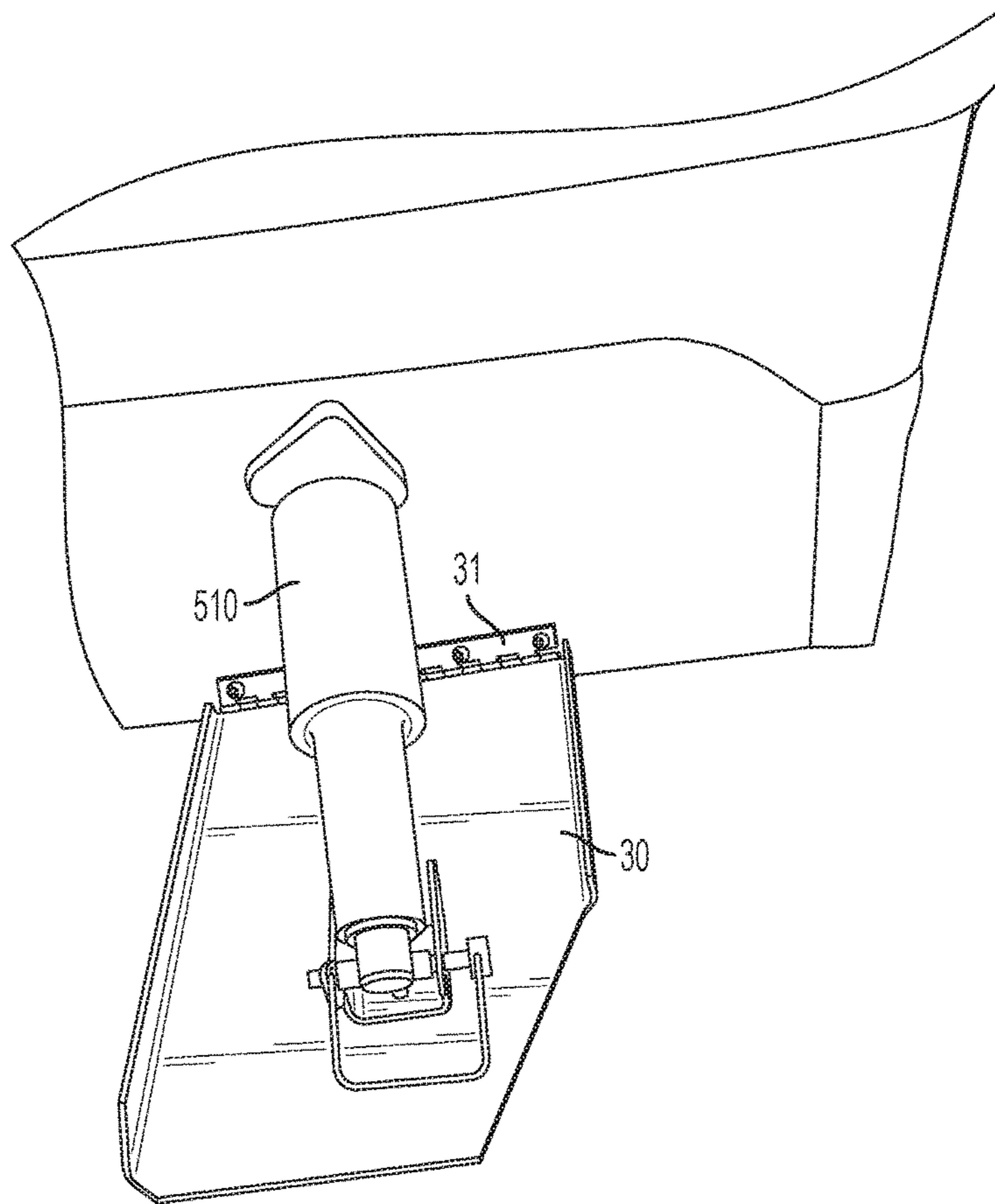
FIG. 2 PRIOR ART
