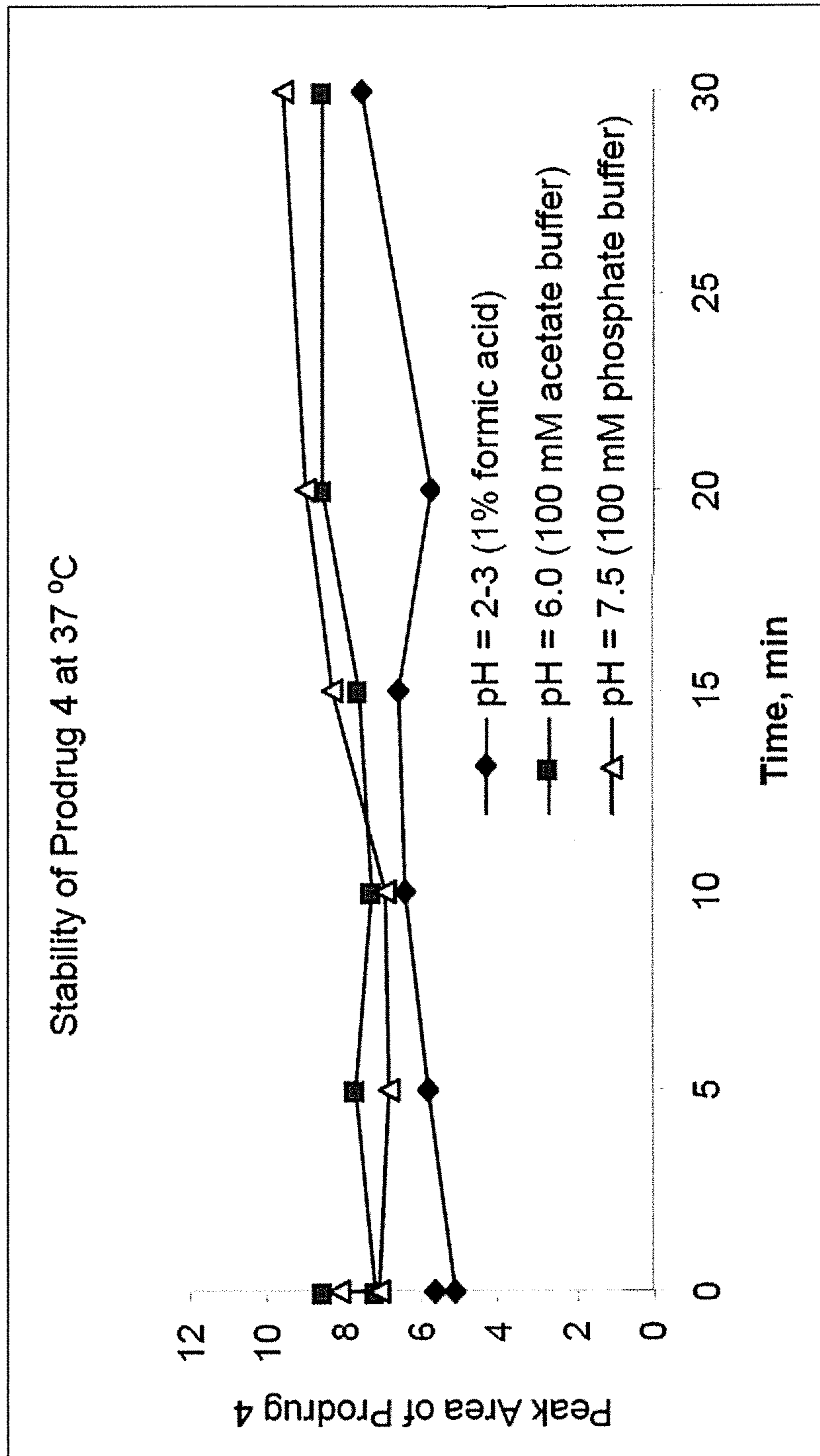
FIG. 8 Chemical Stability of Prodrug 4
