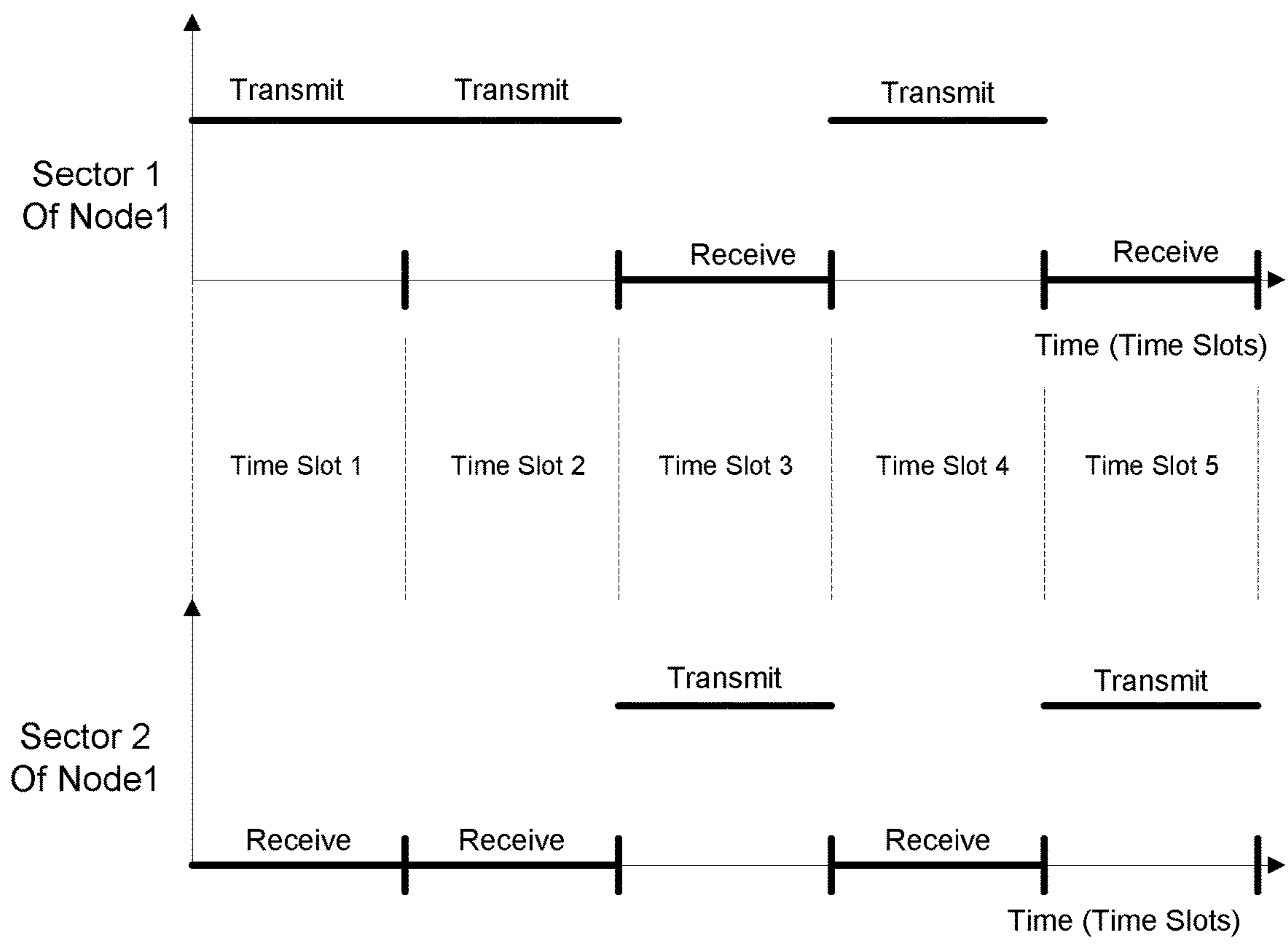
Scheduled Transmission/Reception of Node 1
