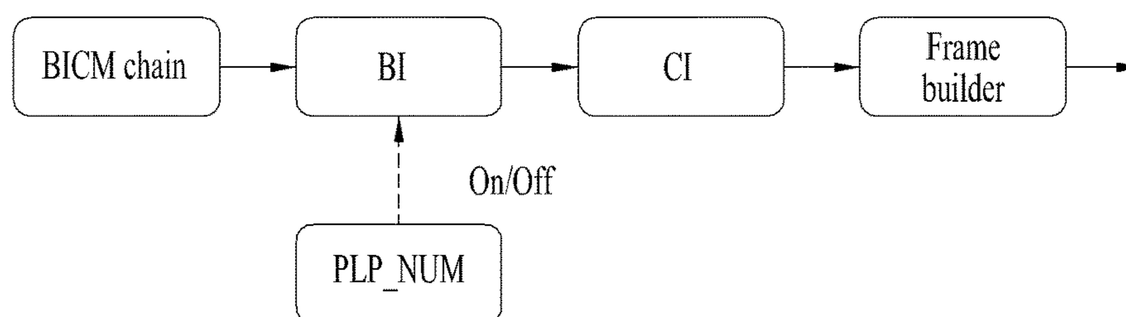
<Hybrid TI structure: example-1>
