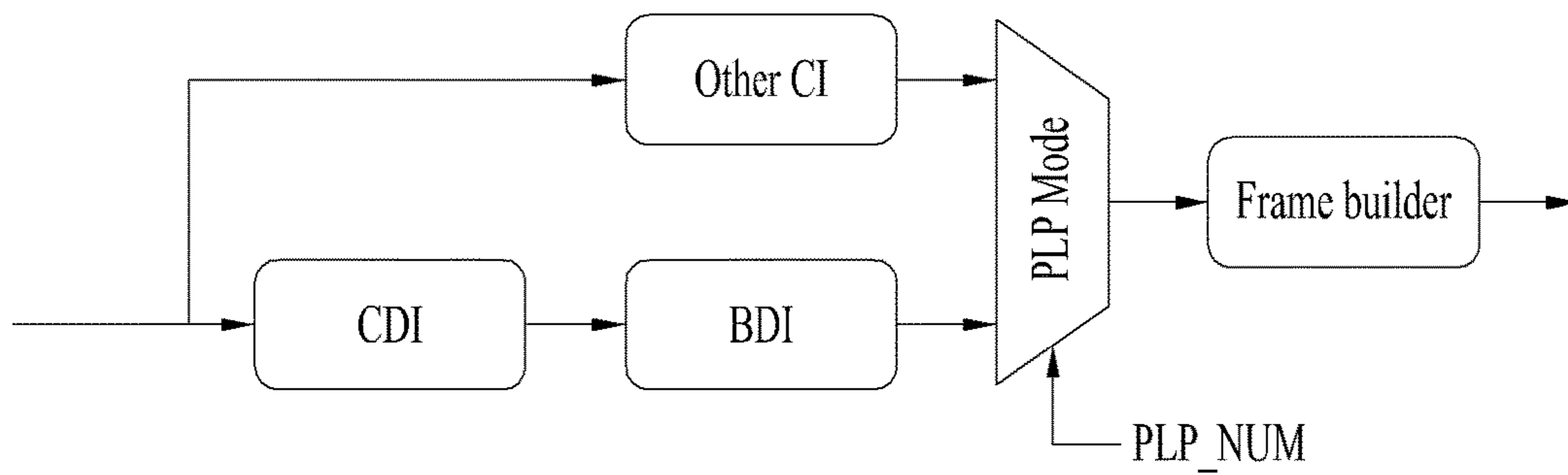
<Hybrid TDI structure: example-2>
