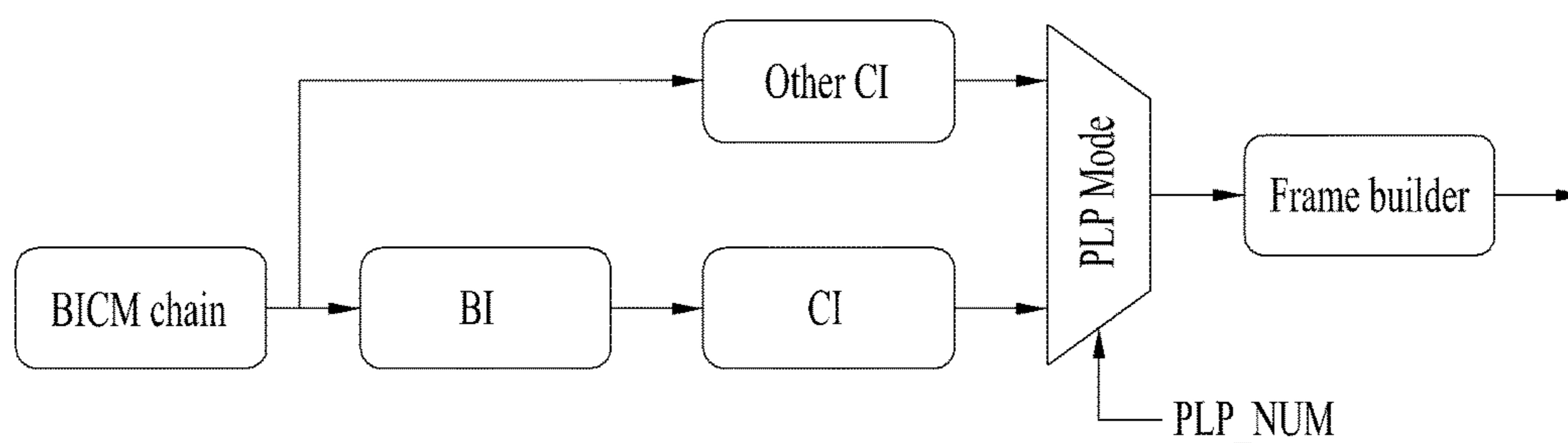
<Hybrid TI structure: example-2>
