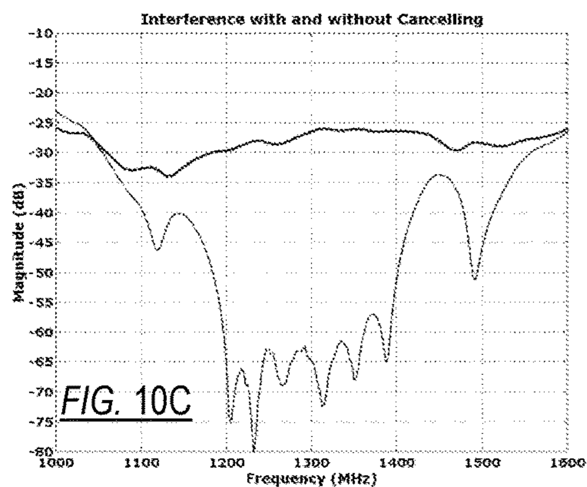
30 dB Cancellation from 1200 to 1400 MHz
