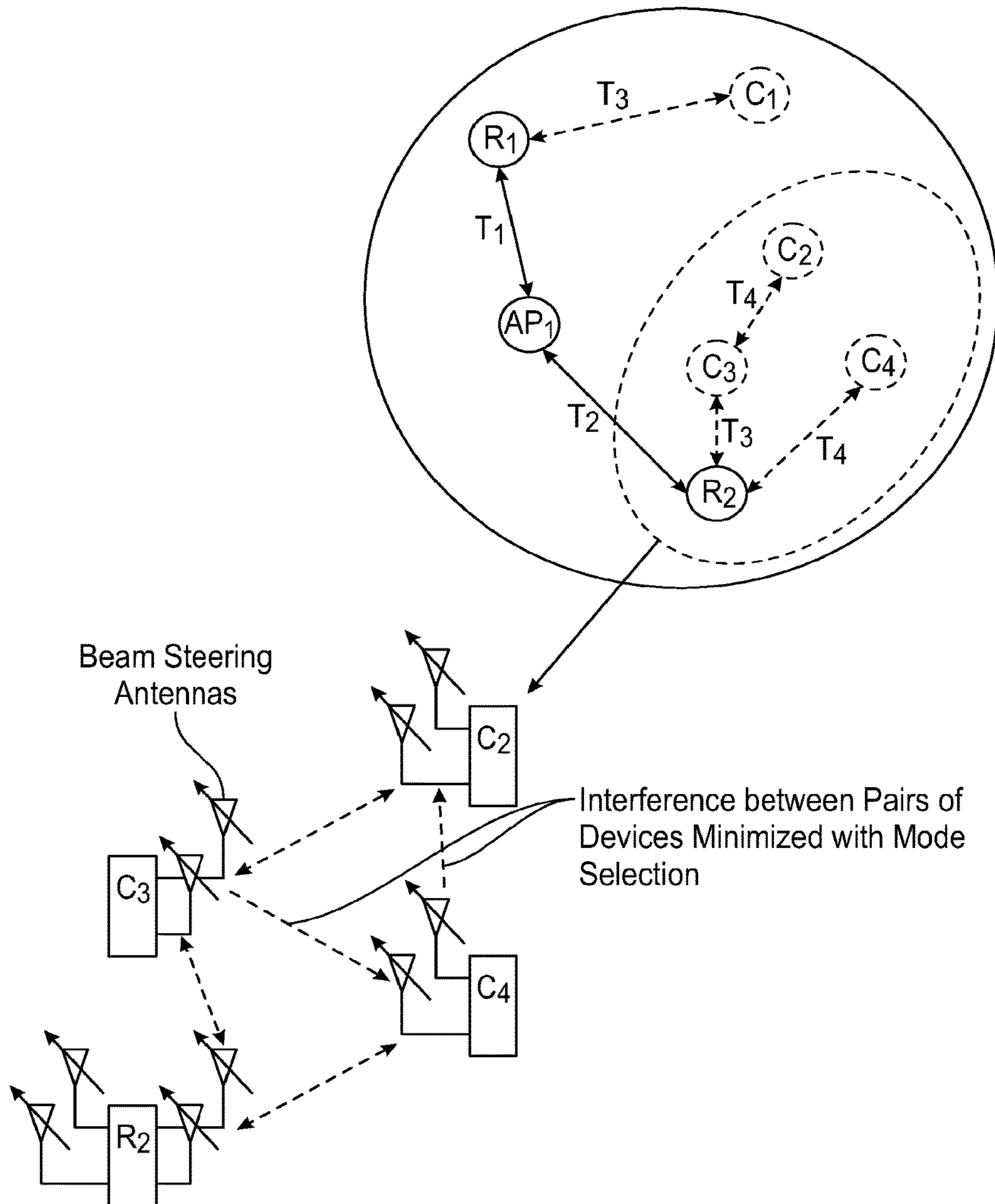
Beam Steering at Access Point, Repeaters and Clients Clients Enabled with Repeater Functionality
