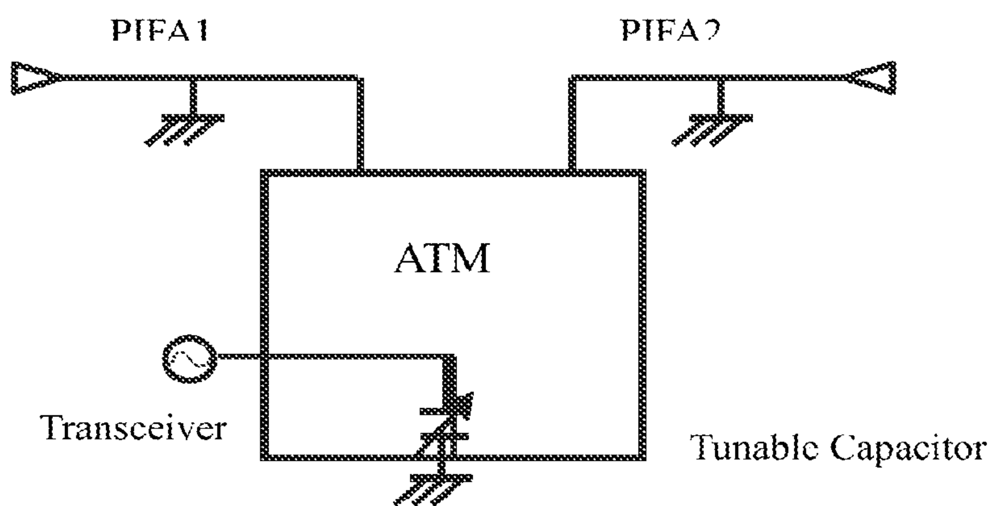
Two antenna configuration utilizing a single tunable capacitor and coupled to a common transceiver port
