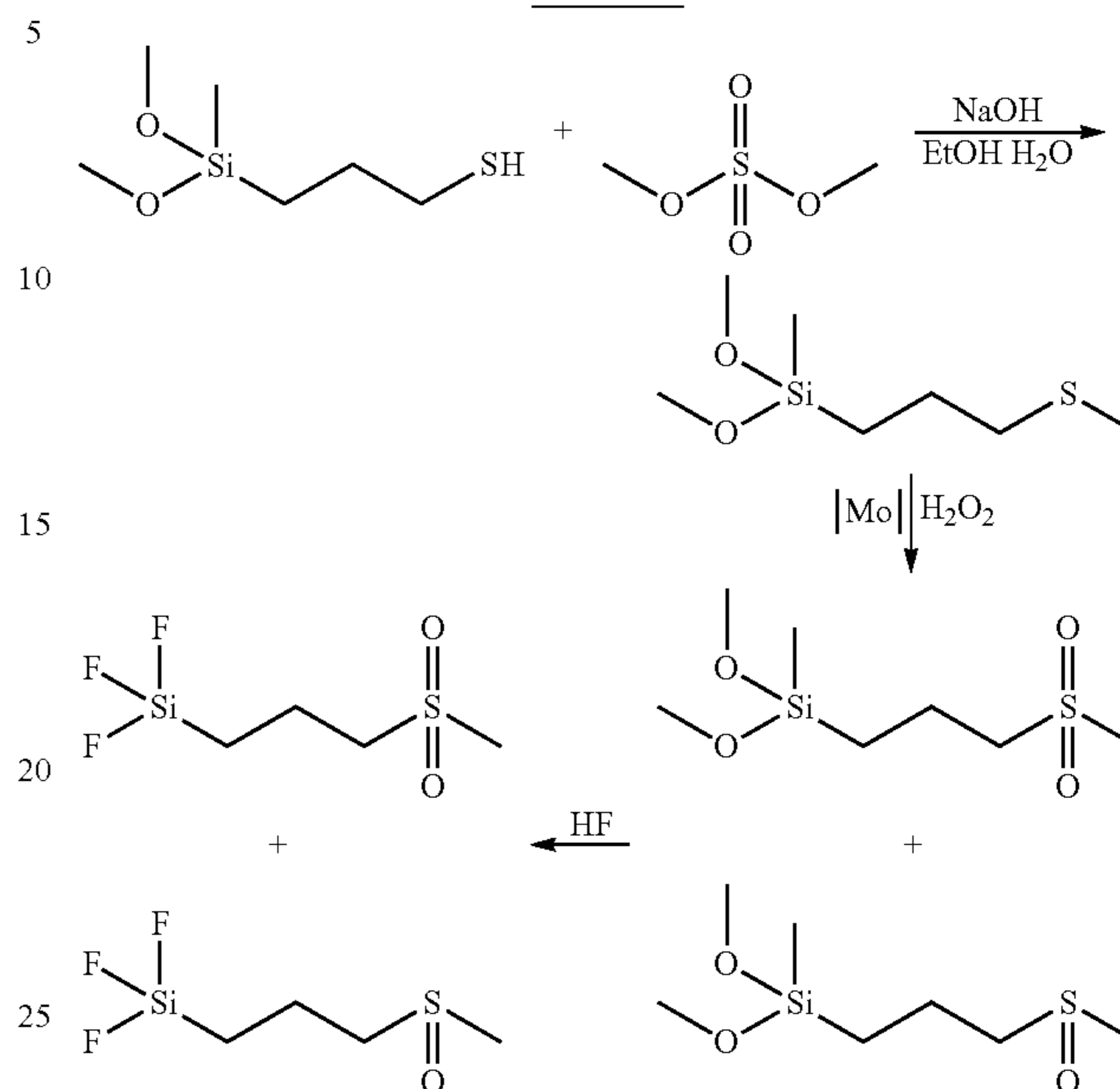
Scheme 11
