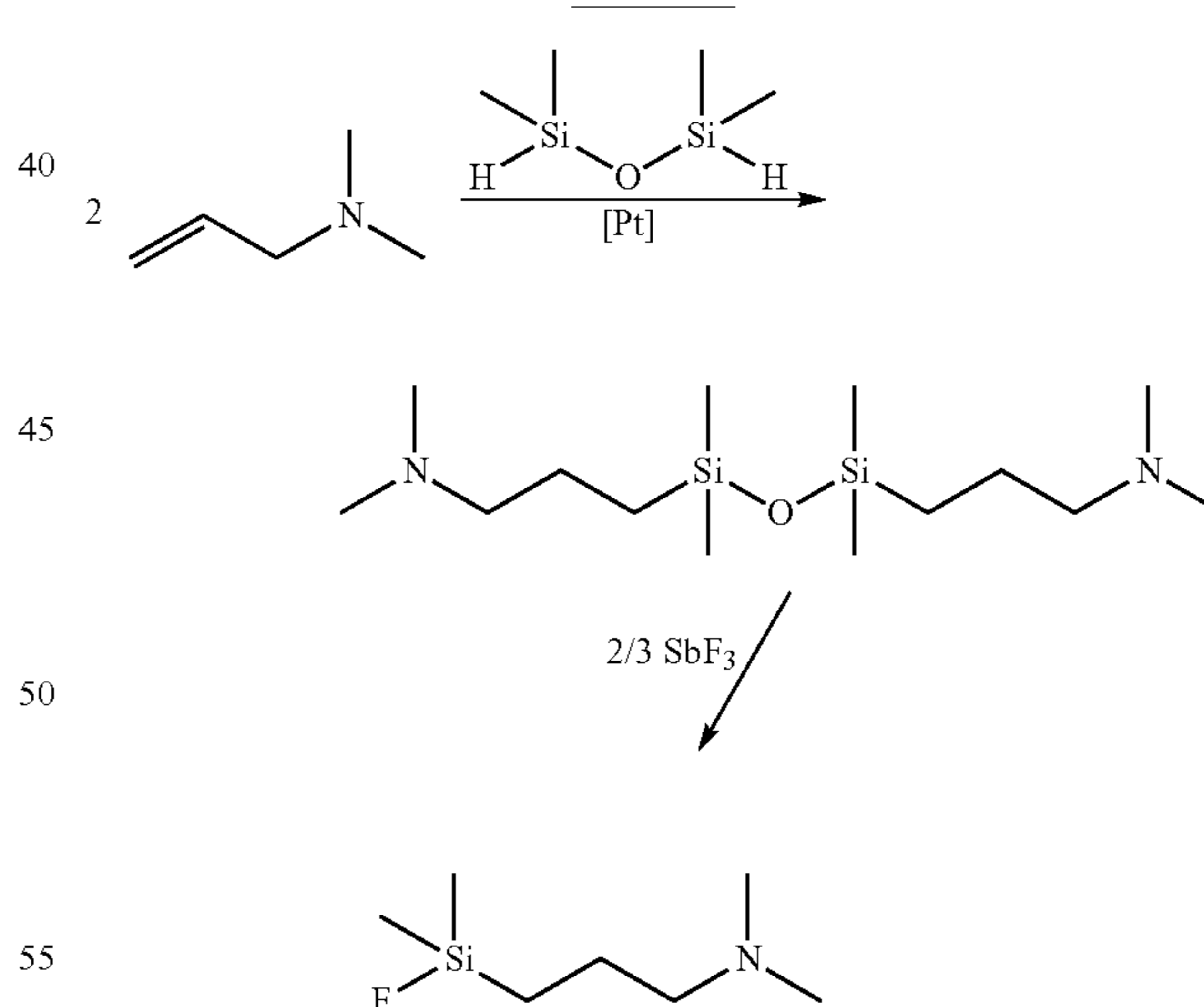
Scheme 12
