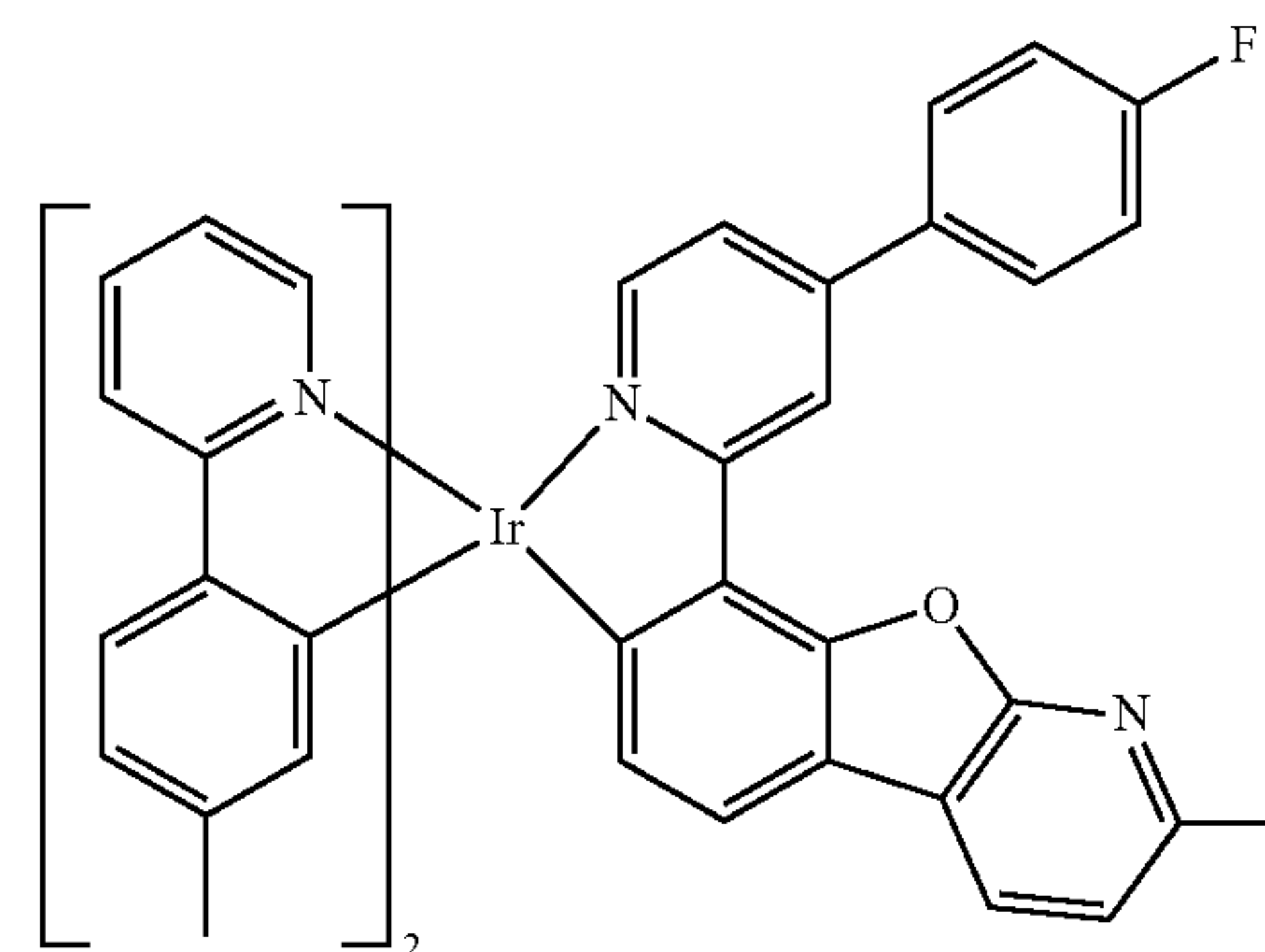
Compound I-1
