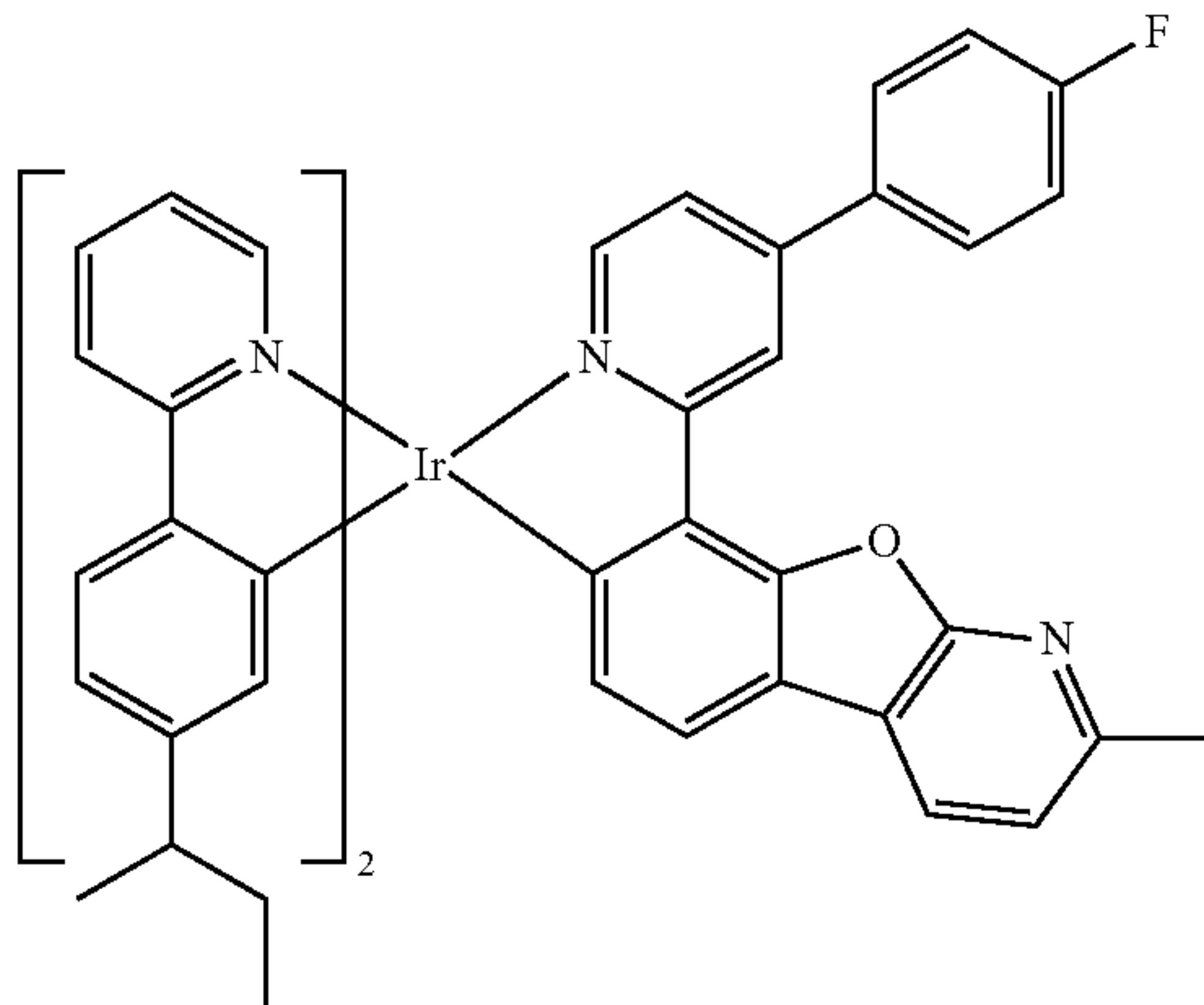
Compound I-13
