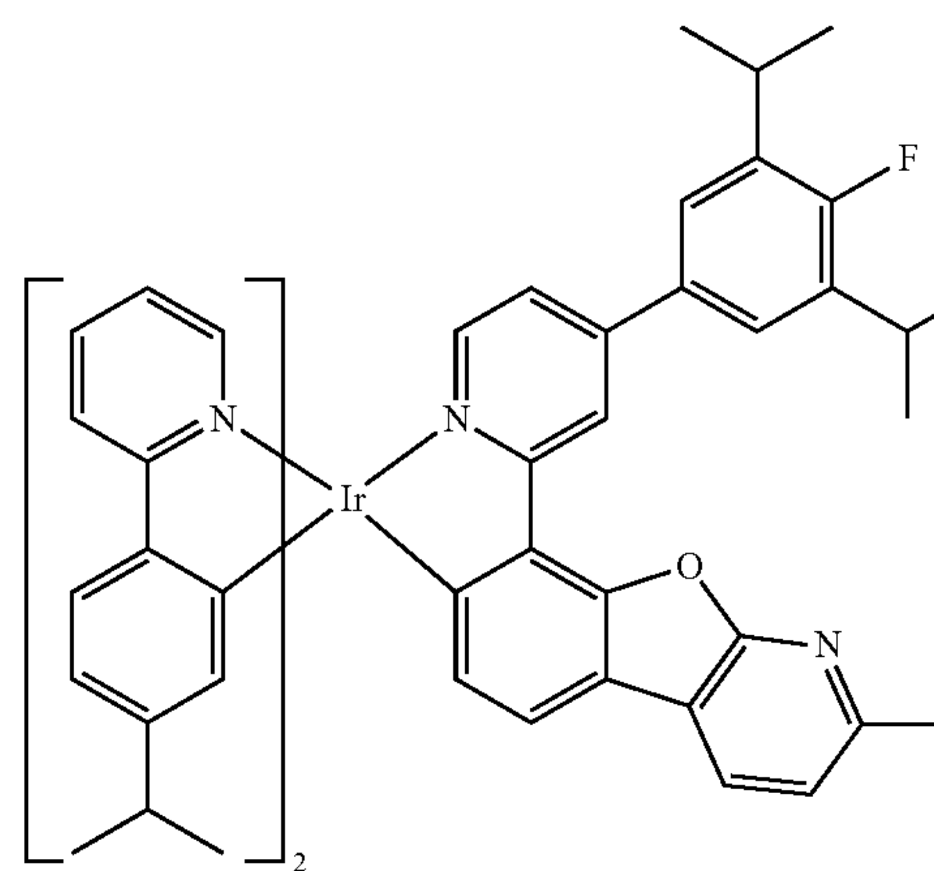
Compound I-8
