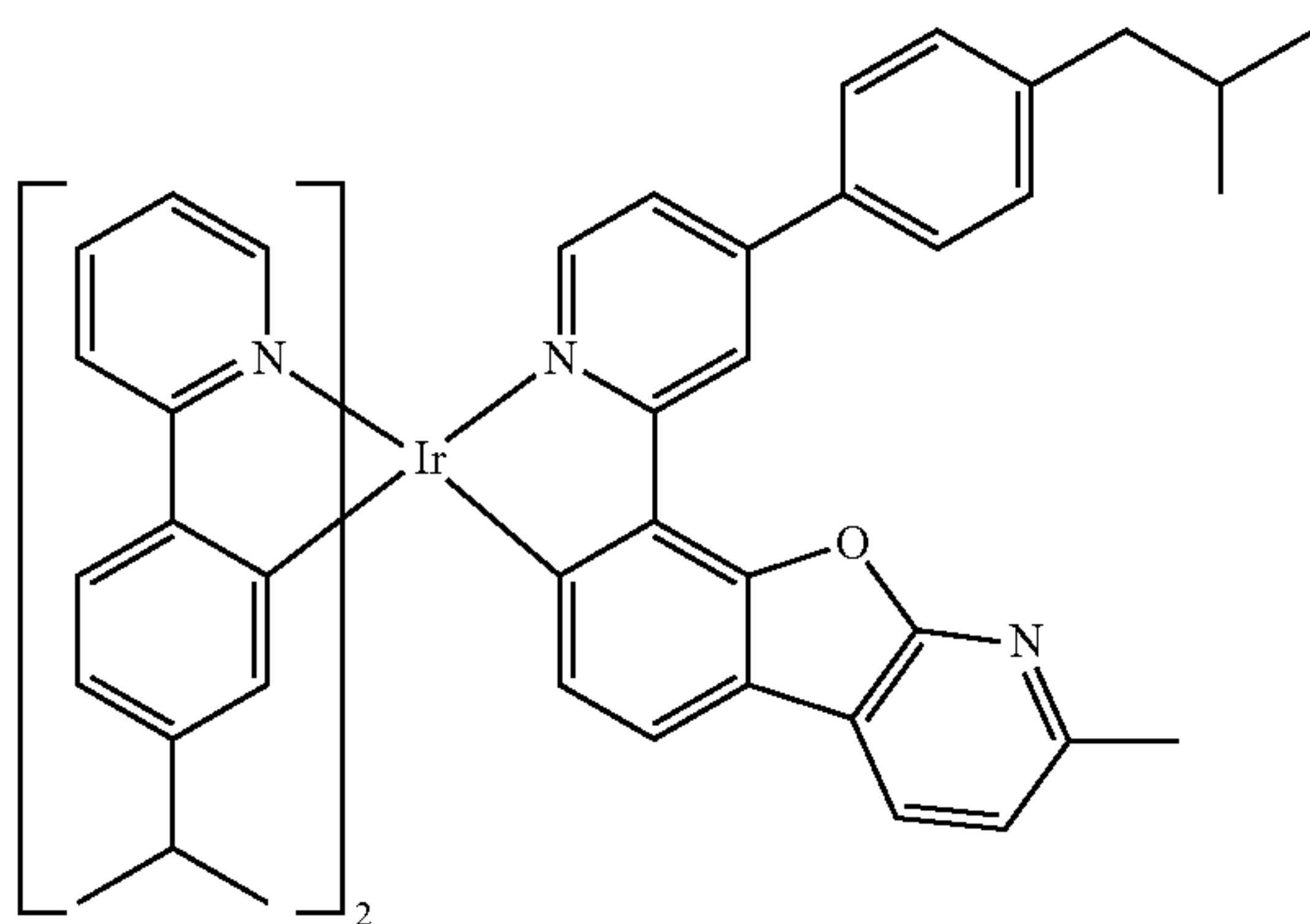
Compound I-5
