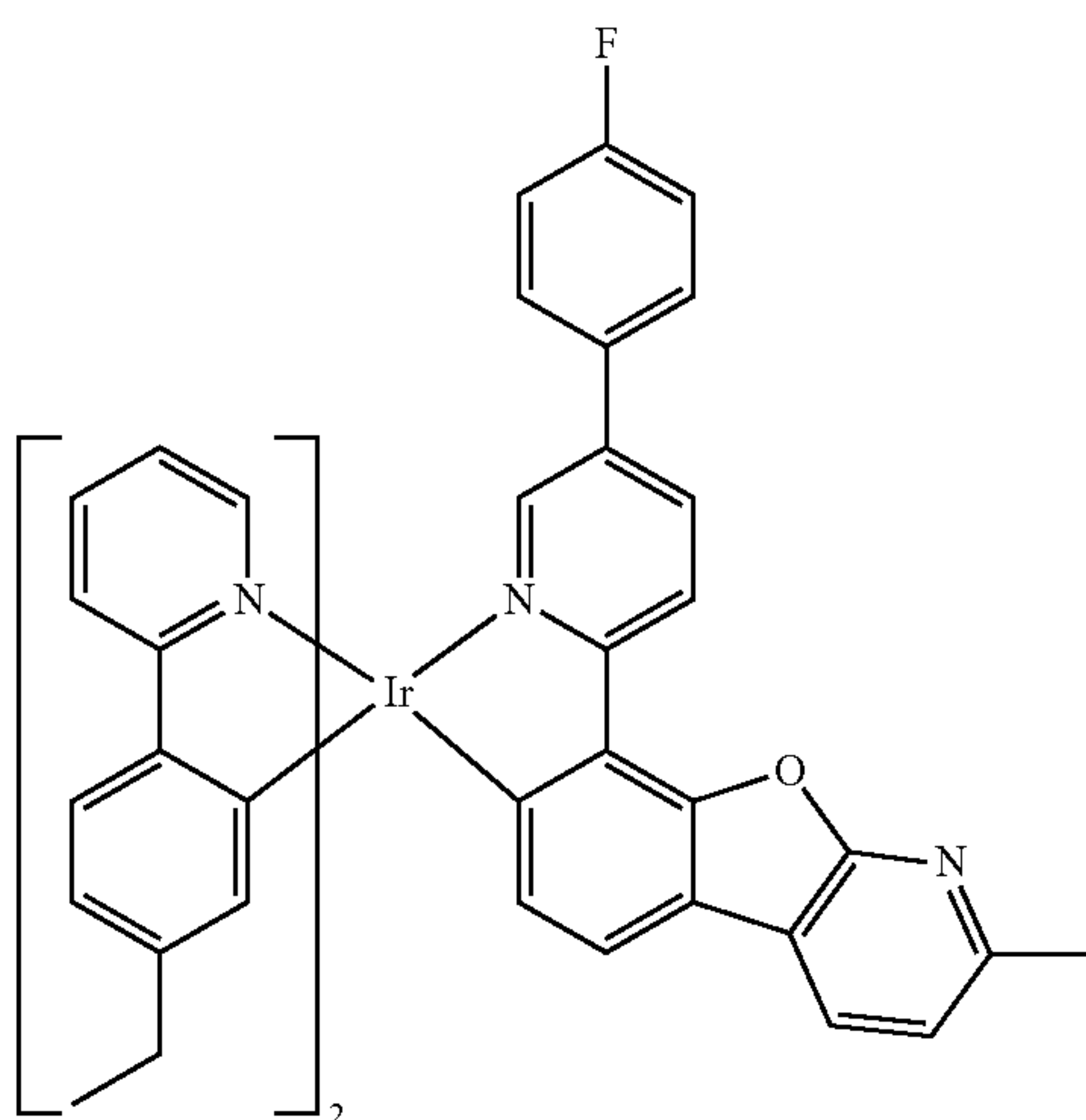
Compound I-4
