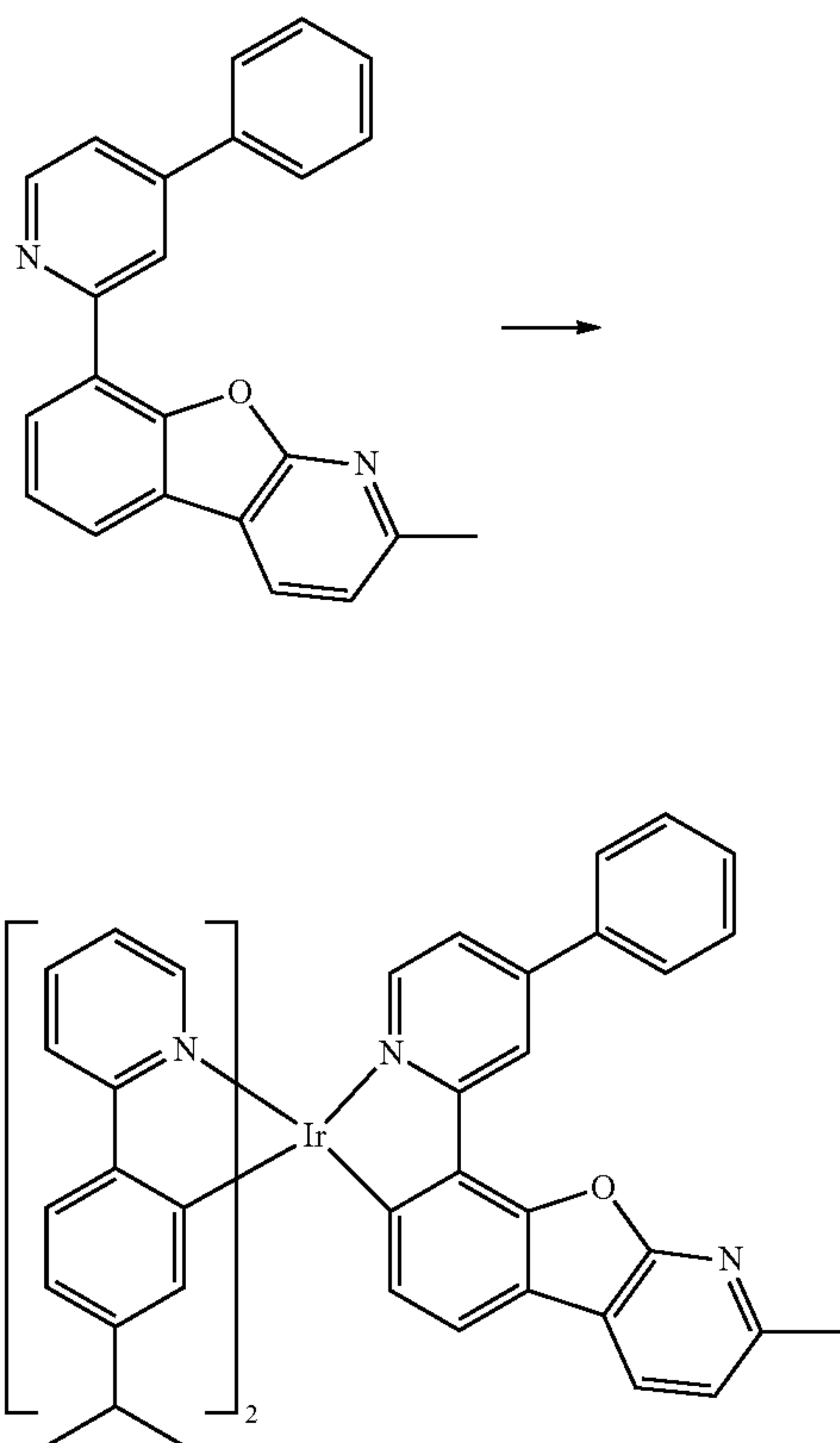
Compound I-6
