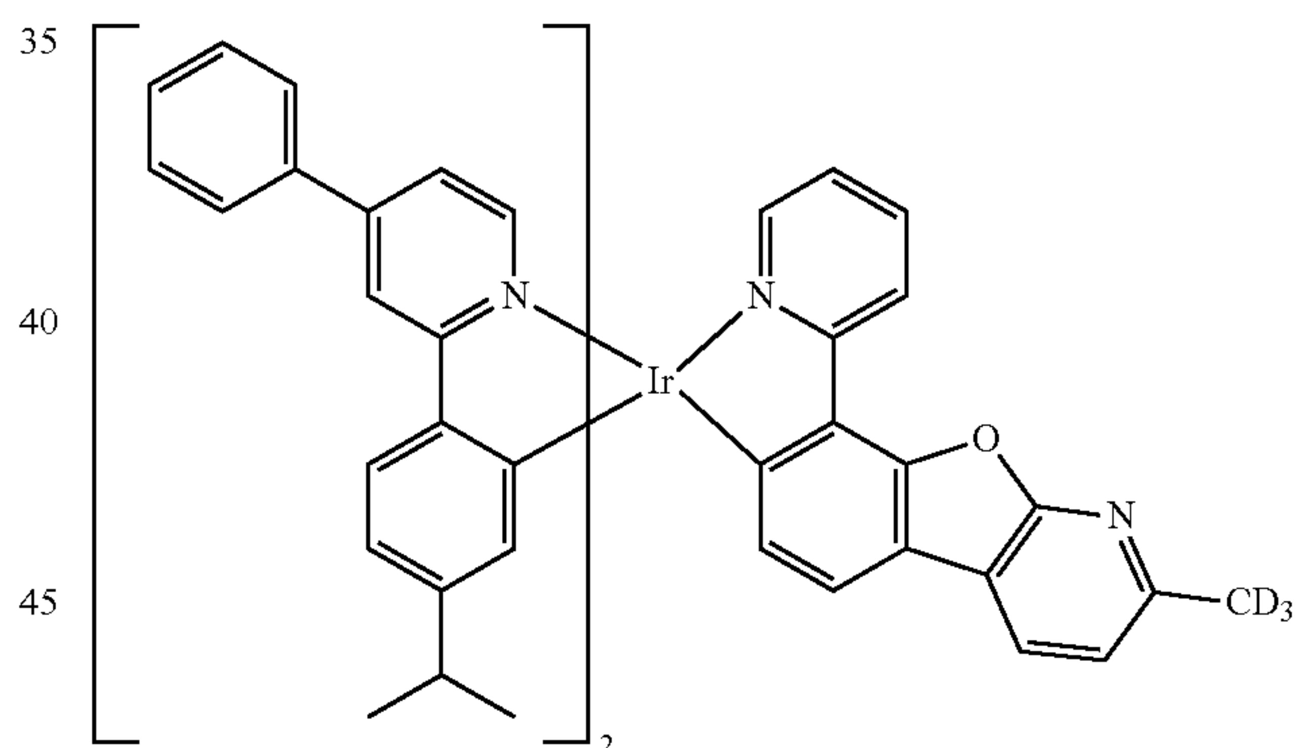
Compound I-19
