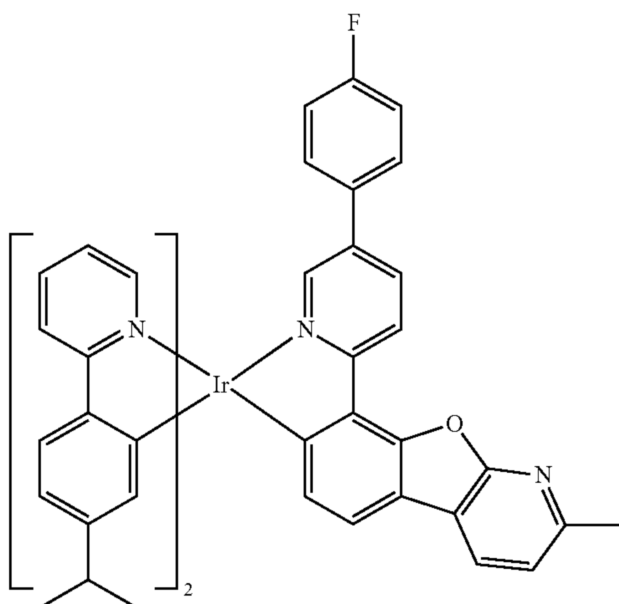
Compound I-9
