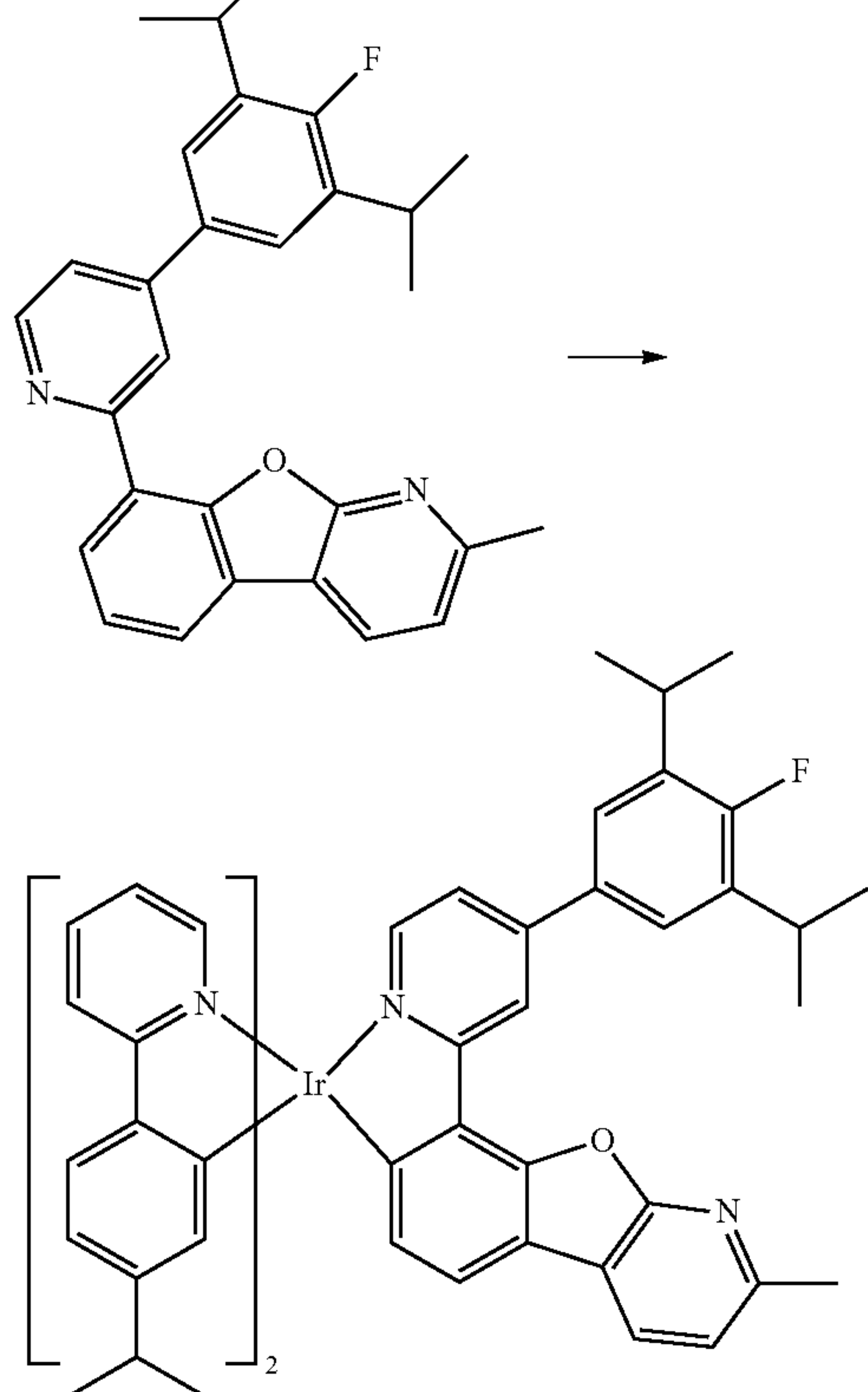
Compound I-8
