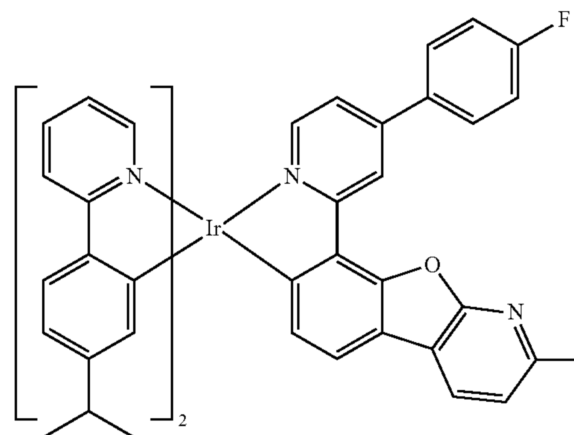
Compound I-5
