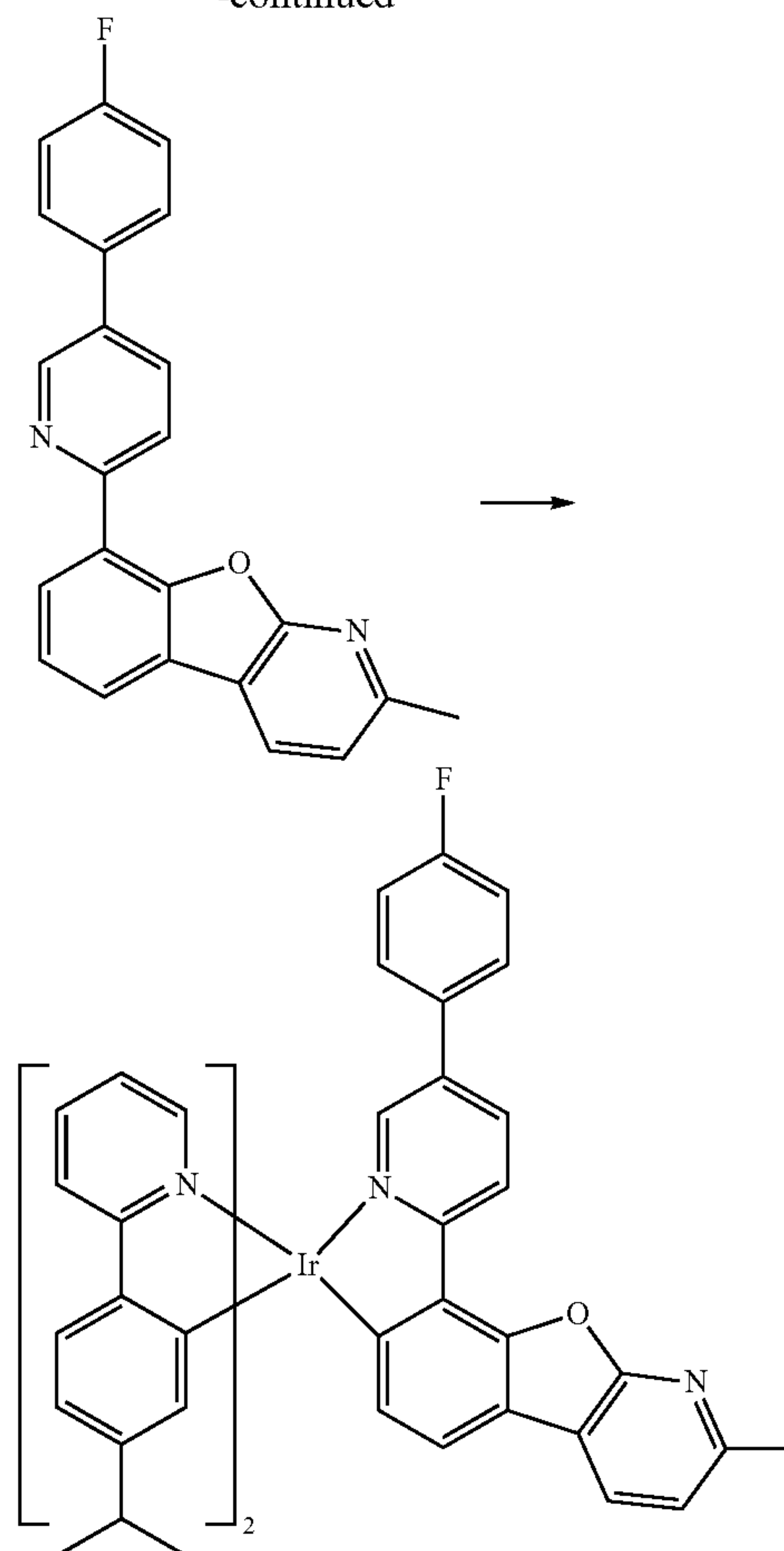
Compound I-9
