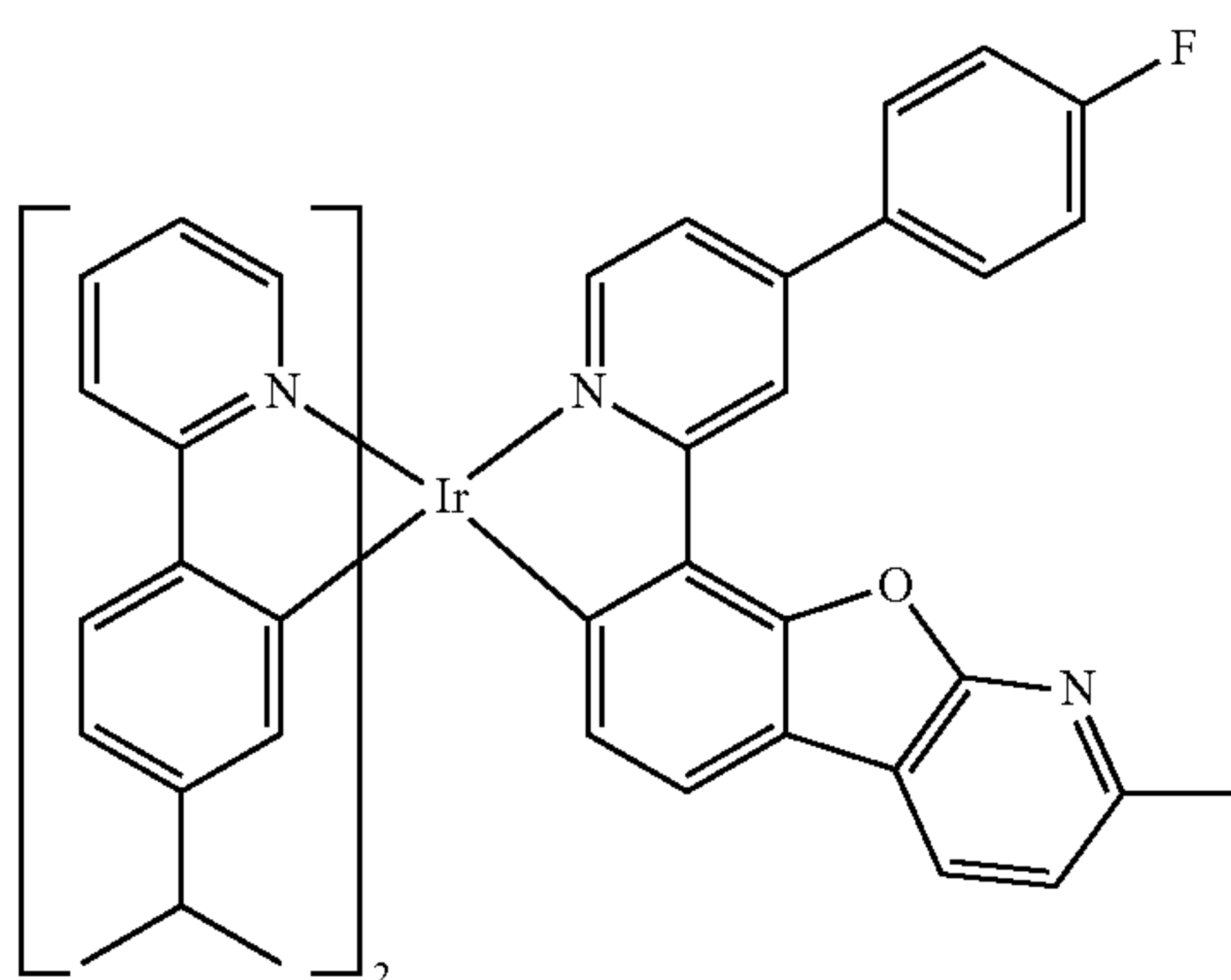
Compound I-5
