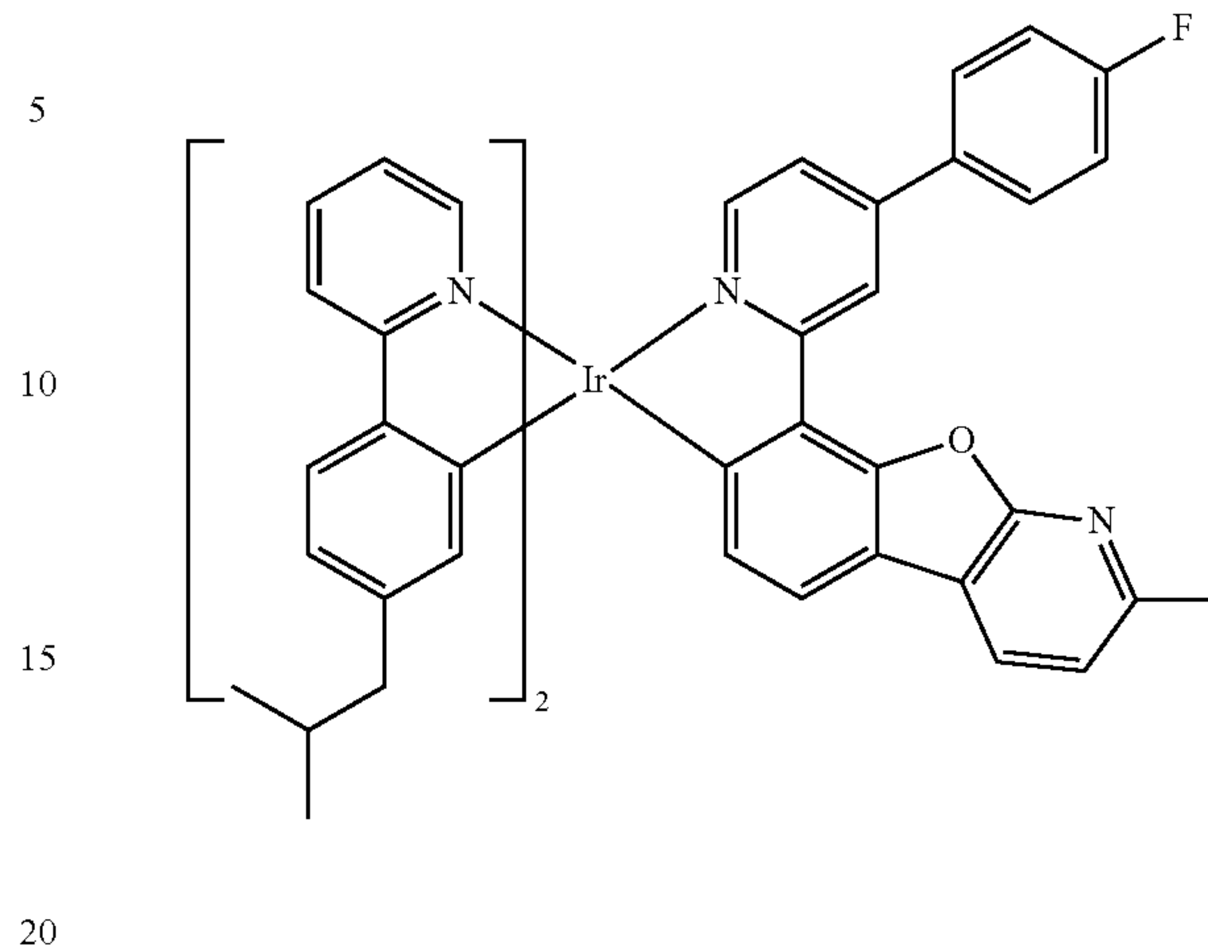
Compound I-10
