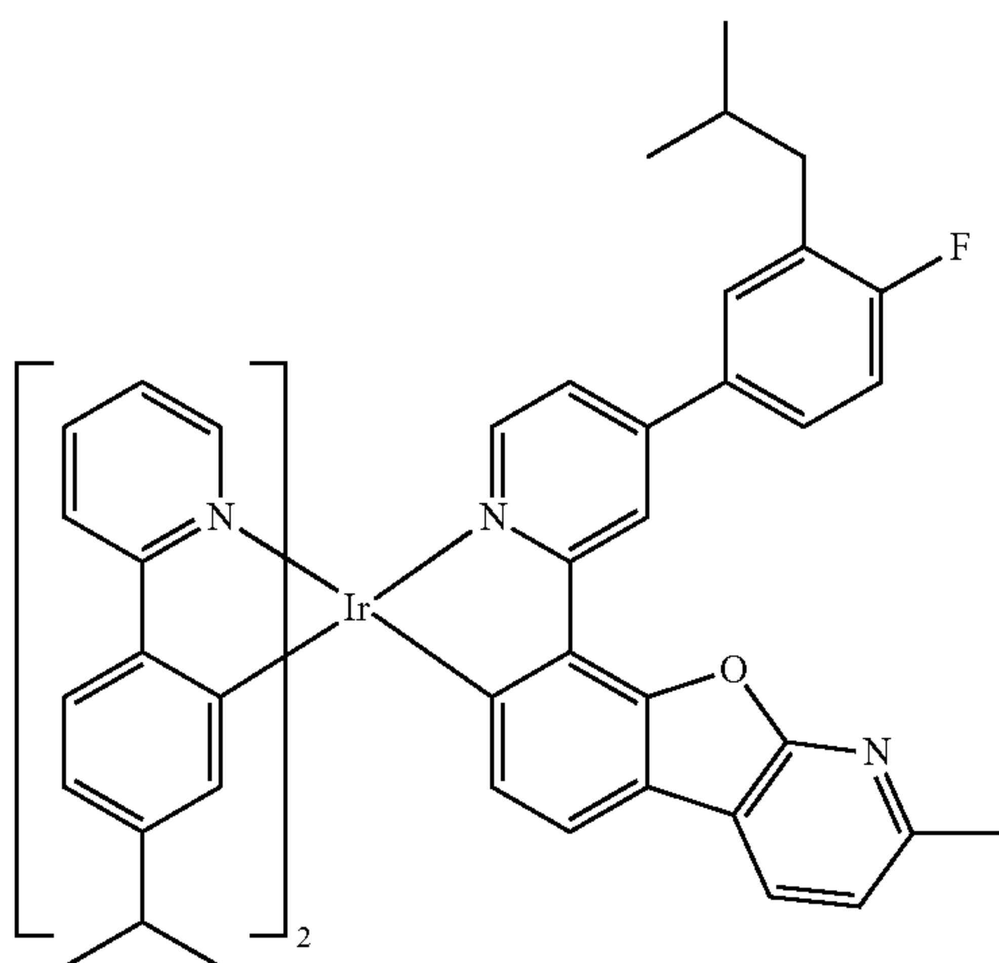
Compound I-7
