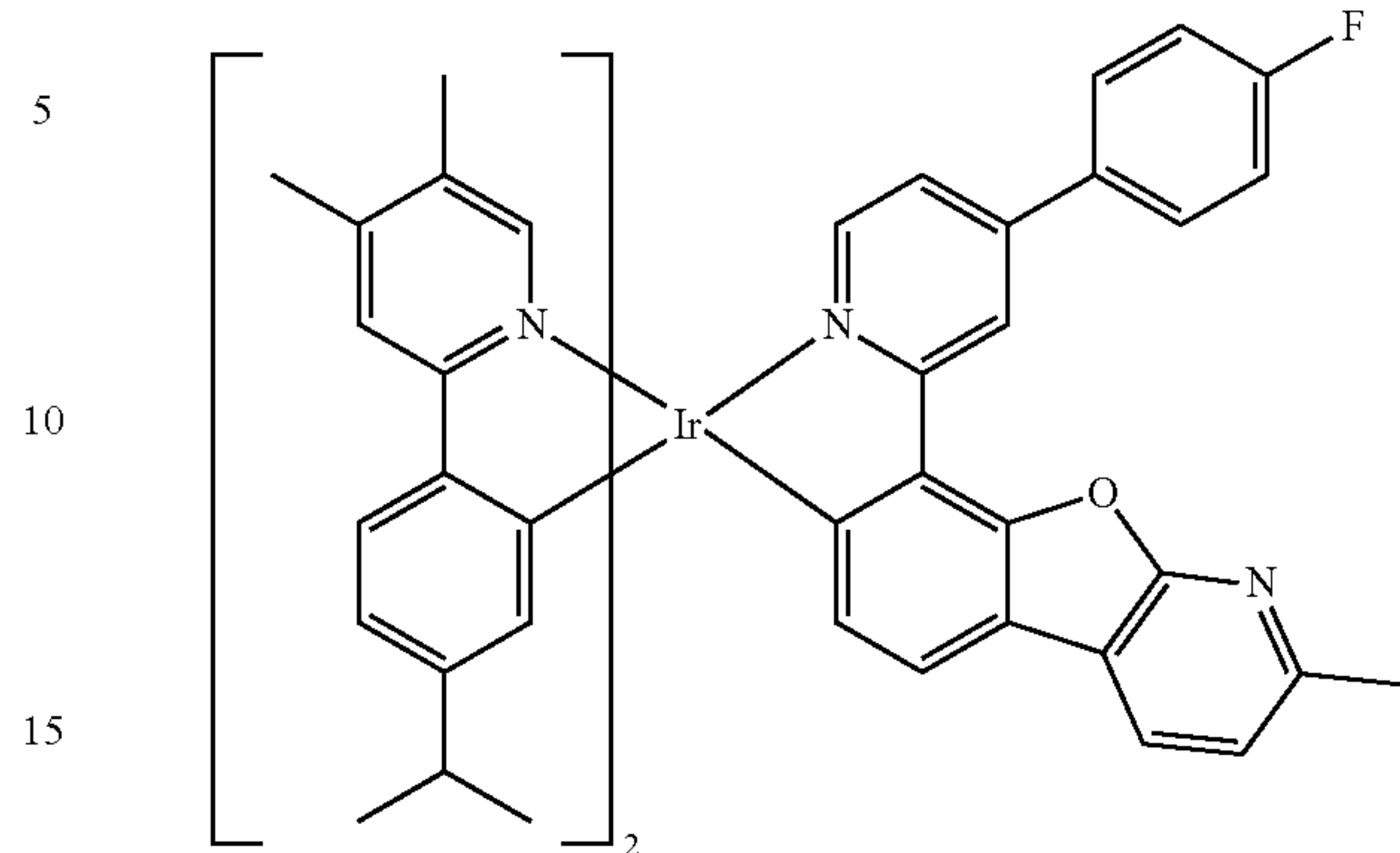
Compound I-17
