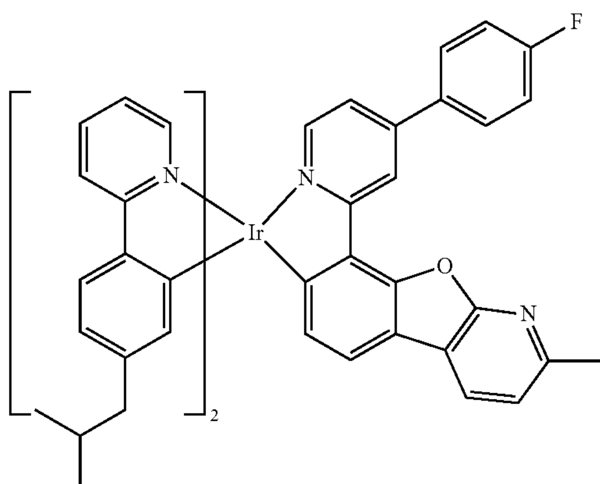
Compound I-10
