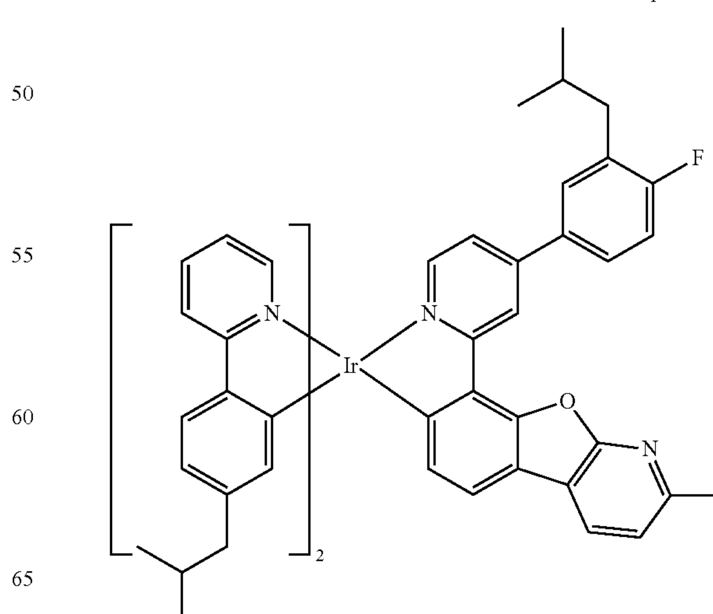
Compound I-12
