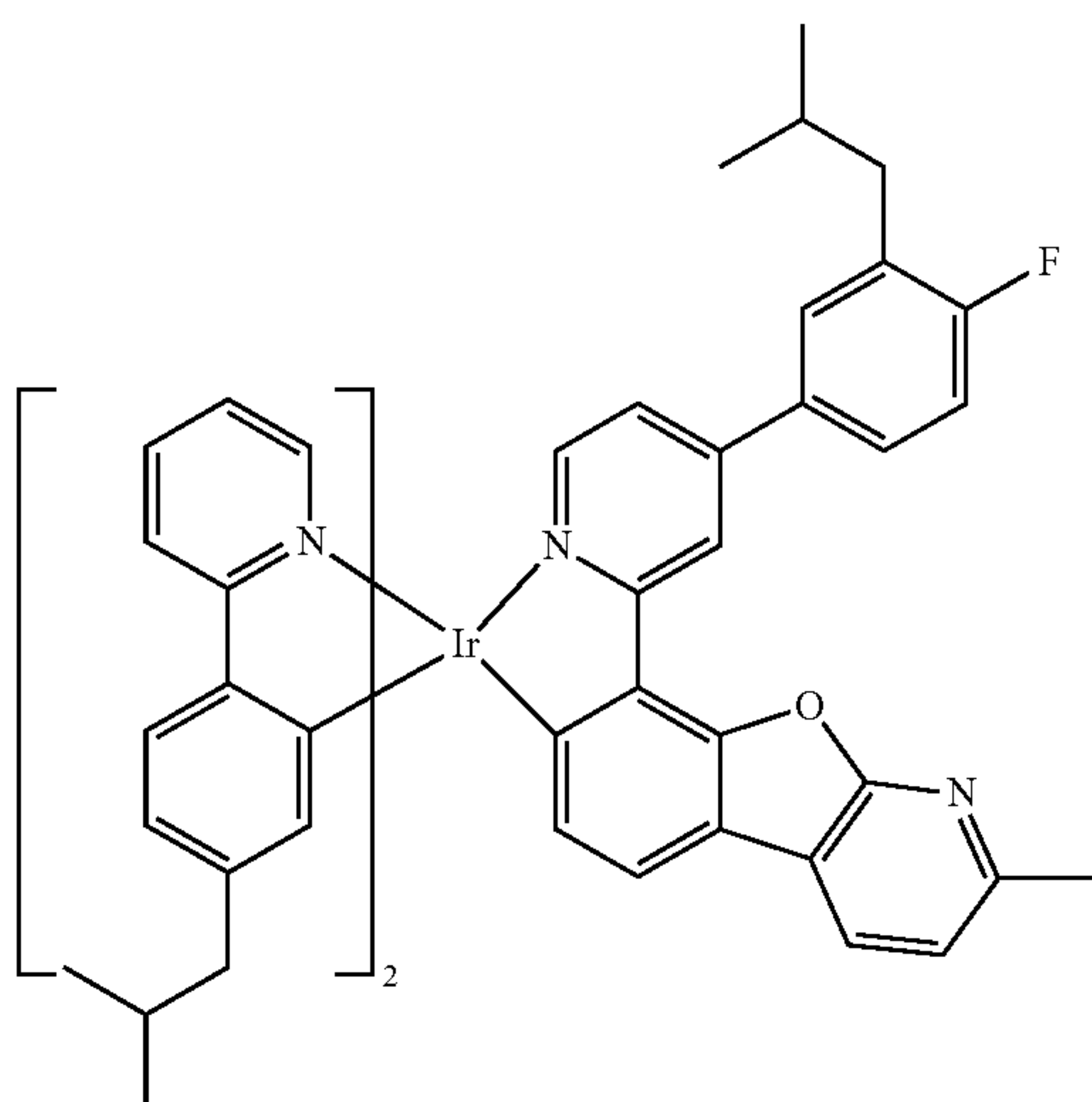
Compound I-12
