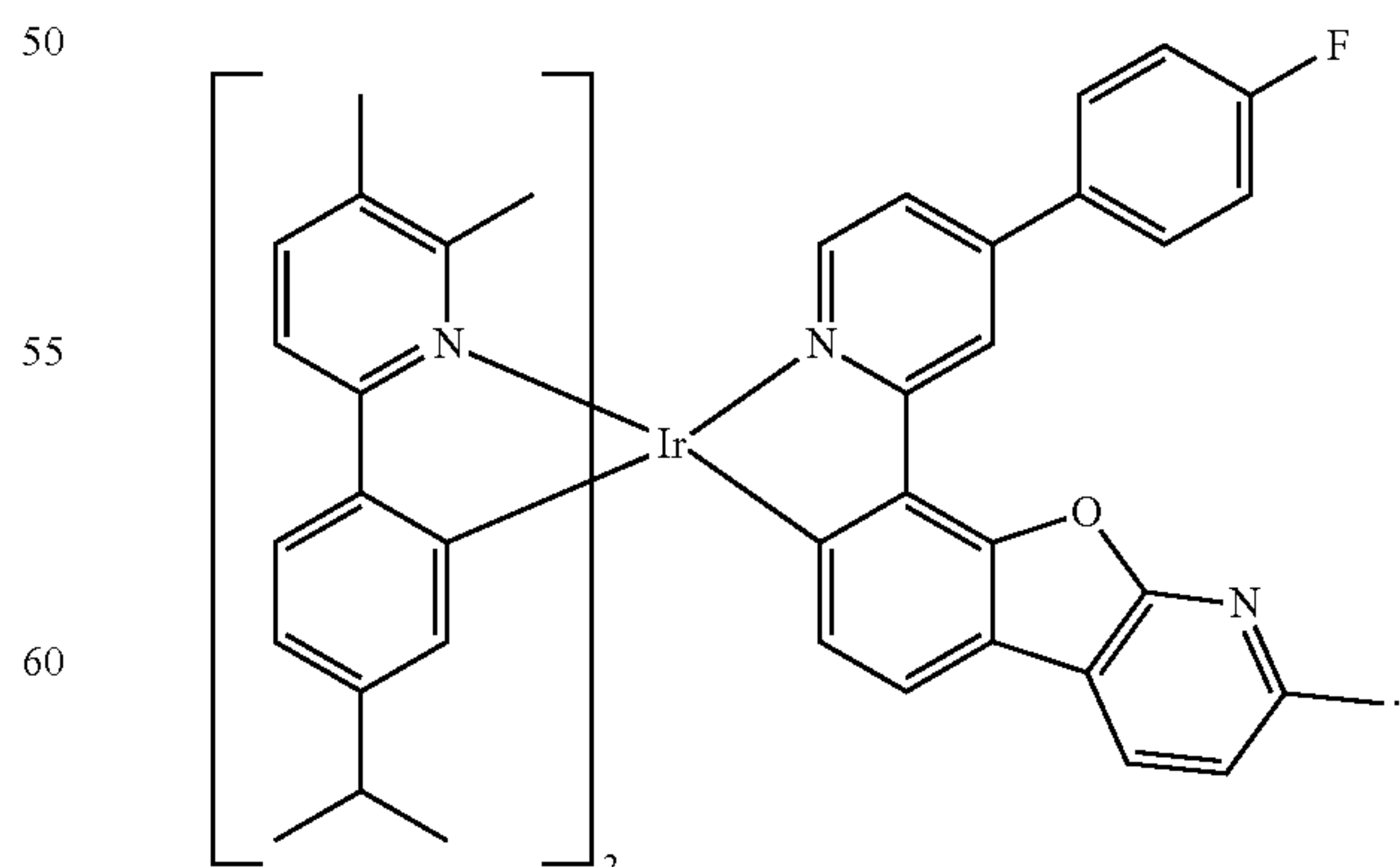
Compound I-19
