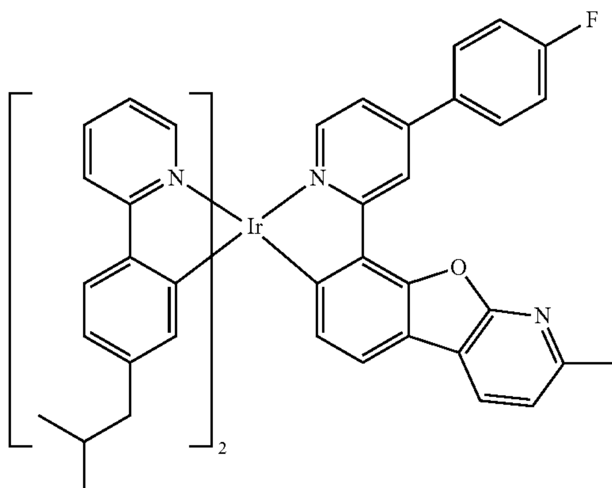
Compound I-10
