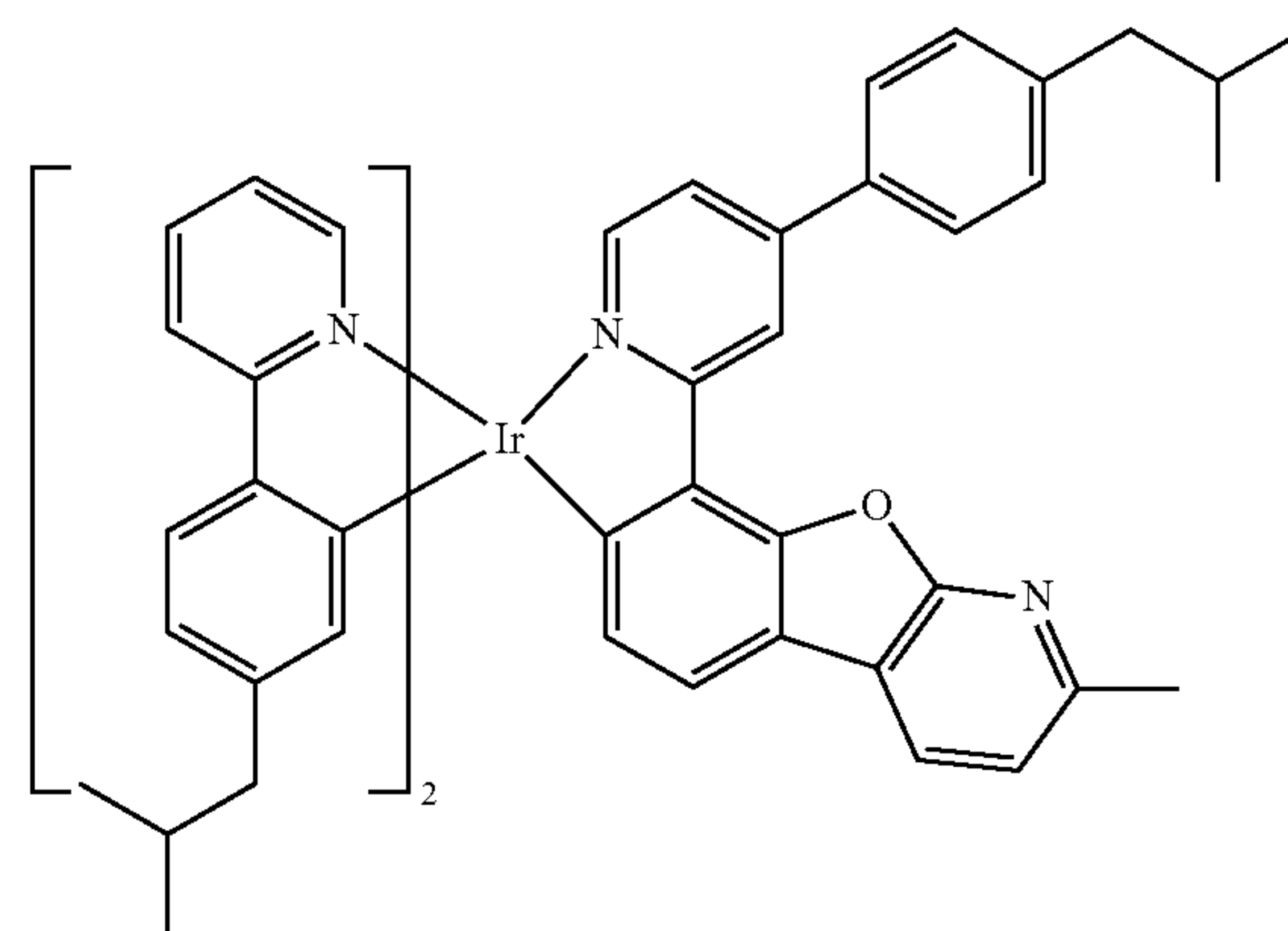
Compound I-11
