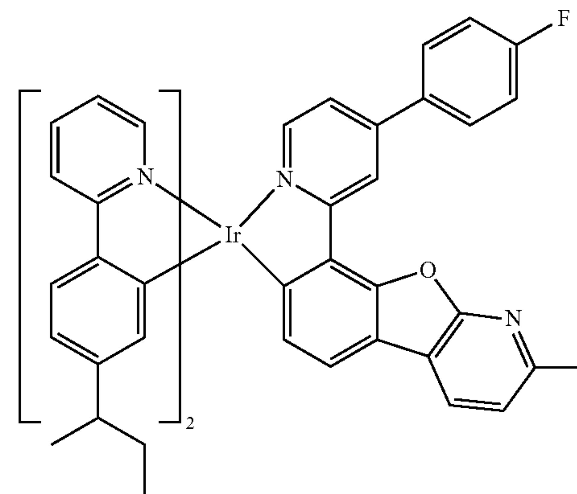
Compound I-13
