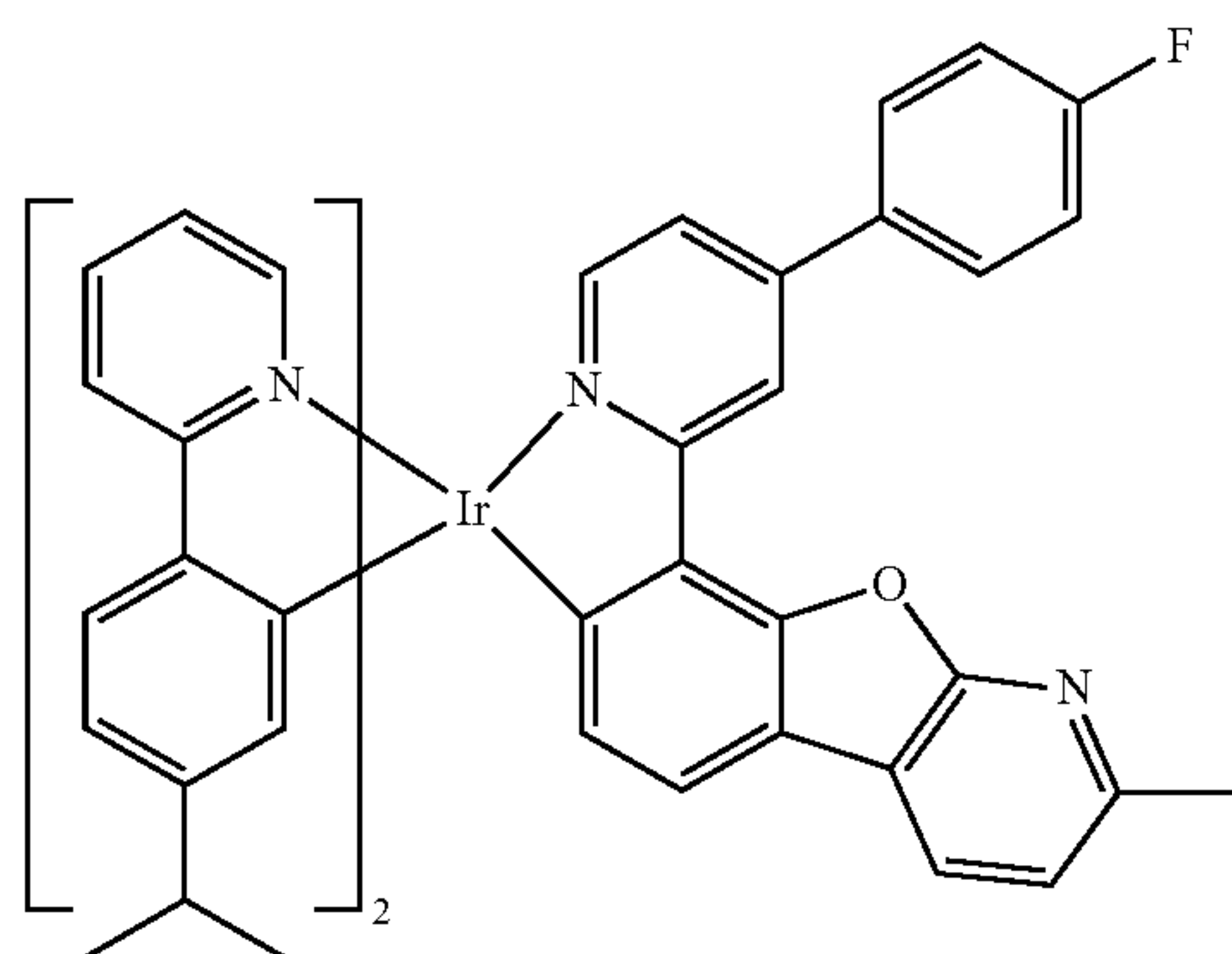
Compound I-4
