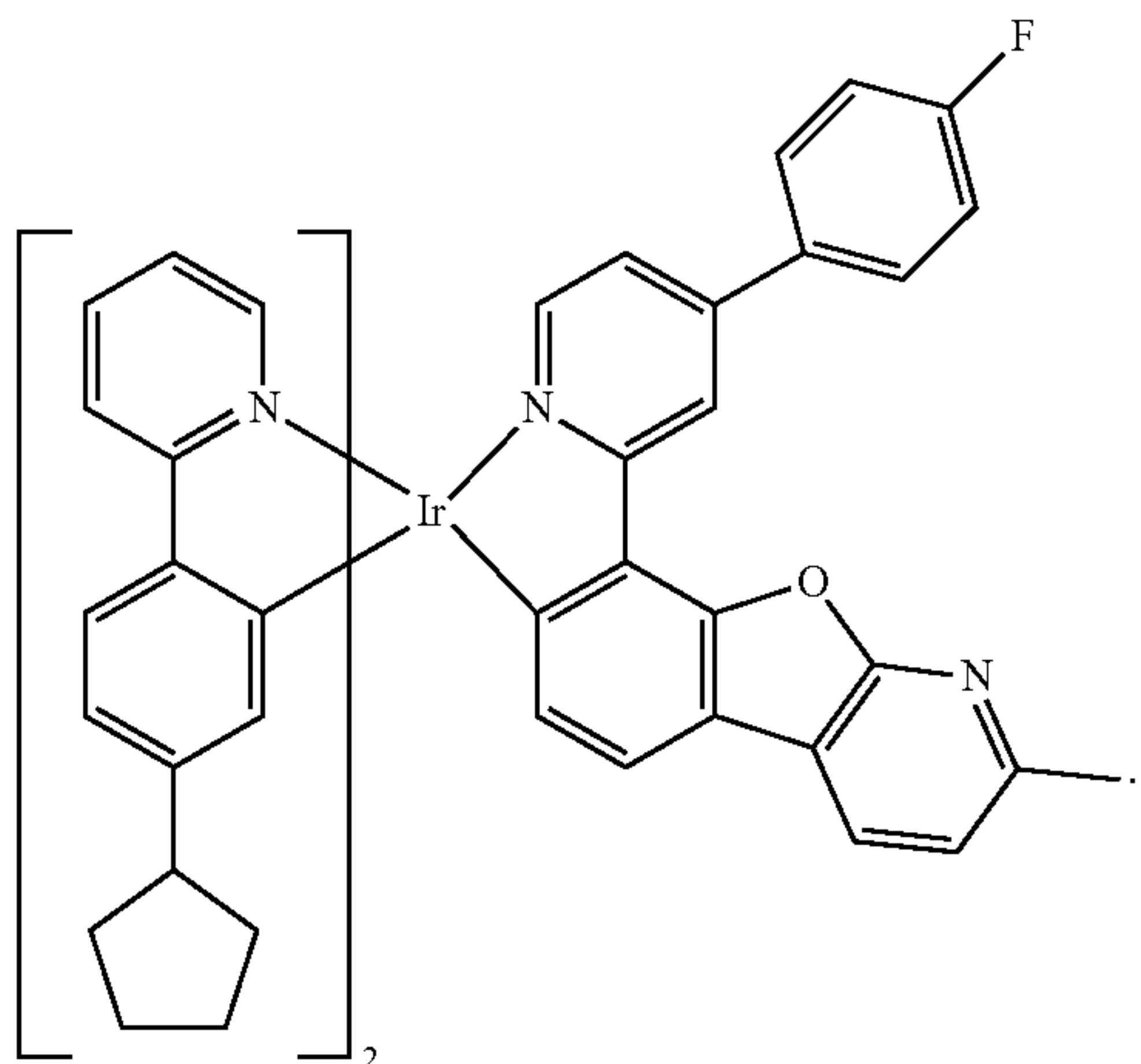
Compound I-15
