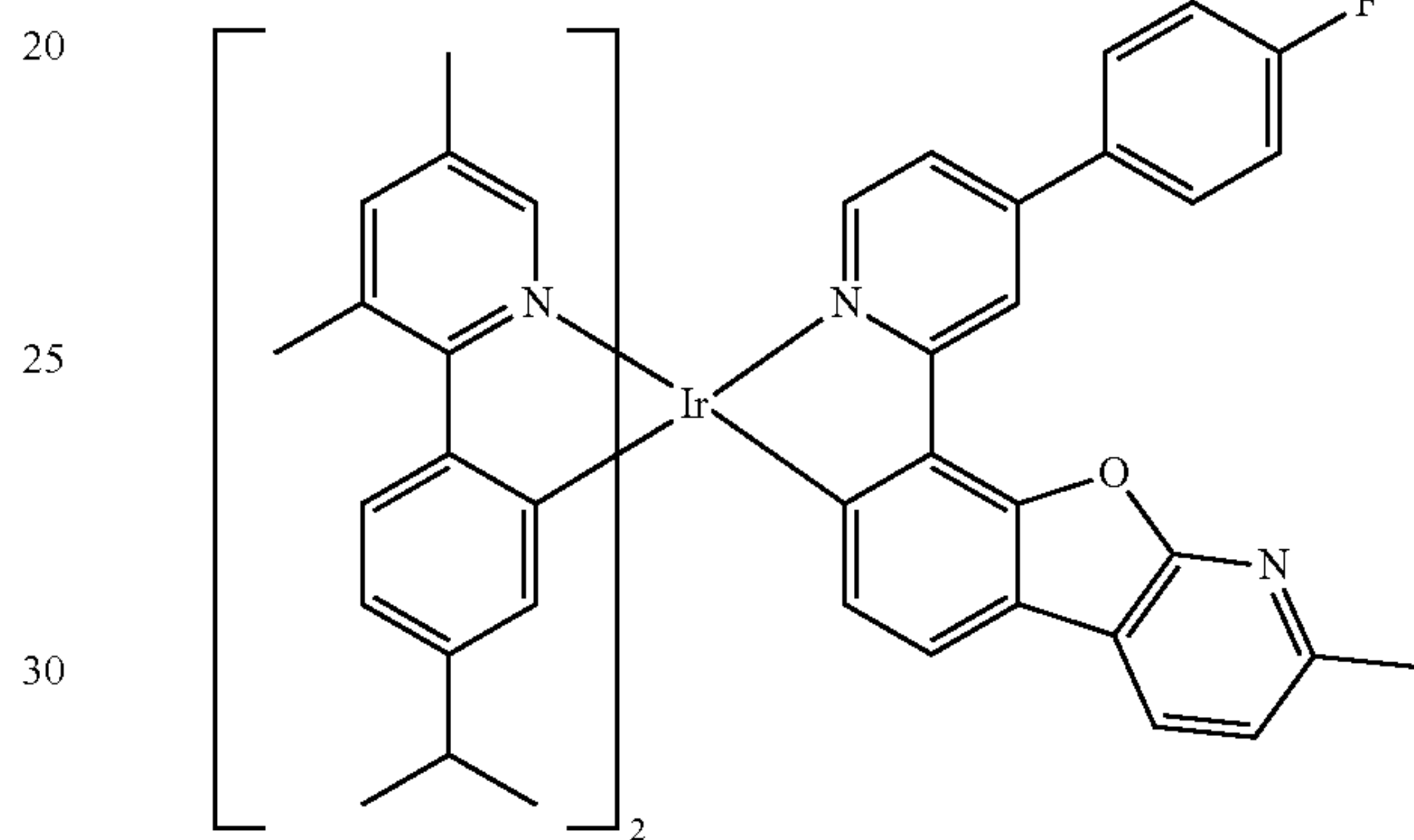
Compound I-18
