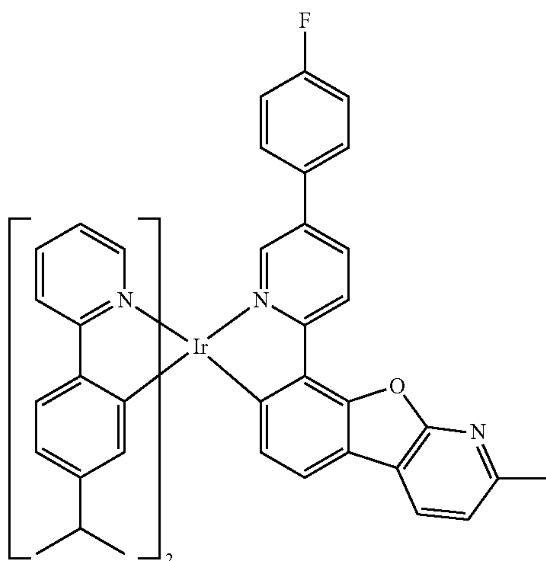
Compound I-9
