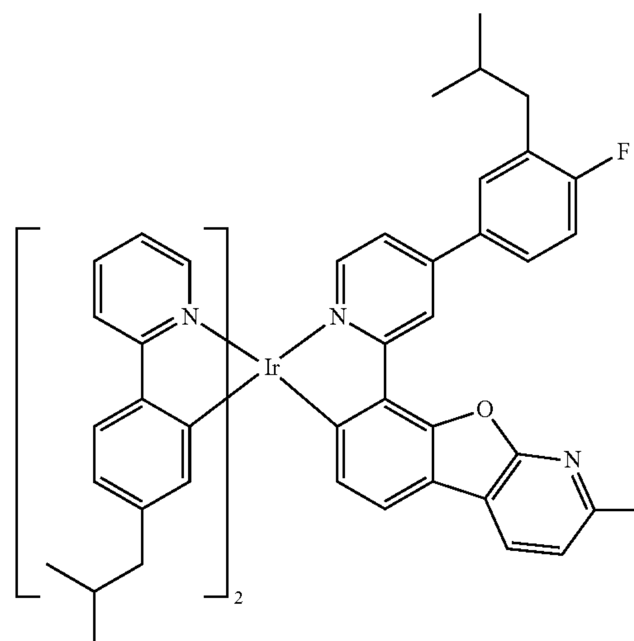
Compound I-12
