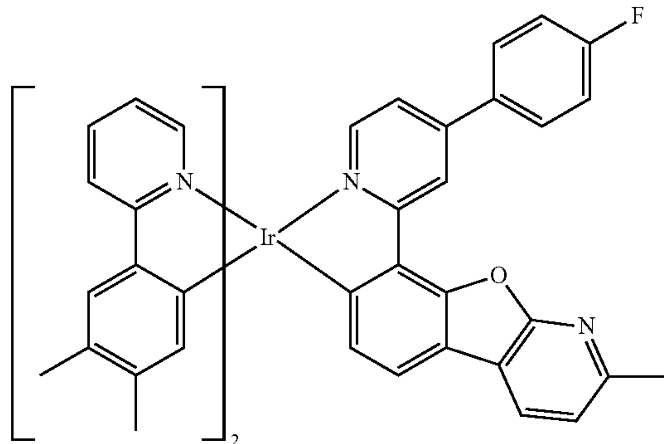
Compound I-14
