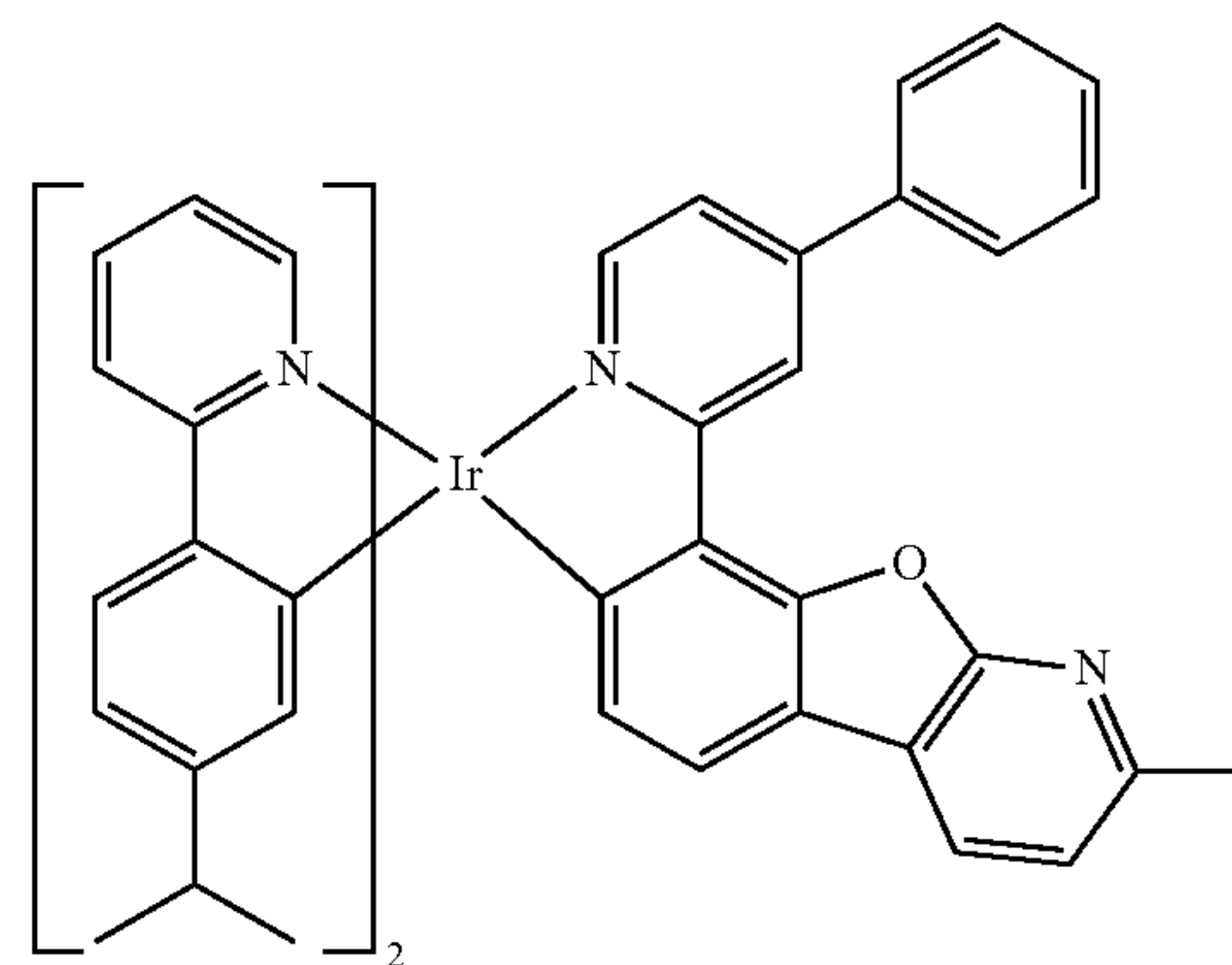
Compound I-6
