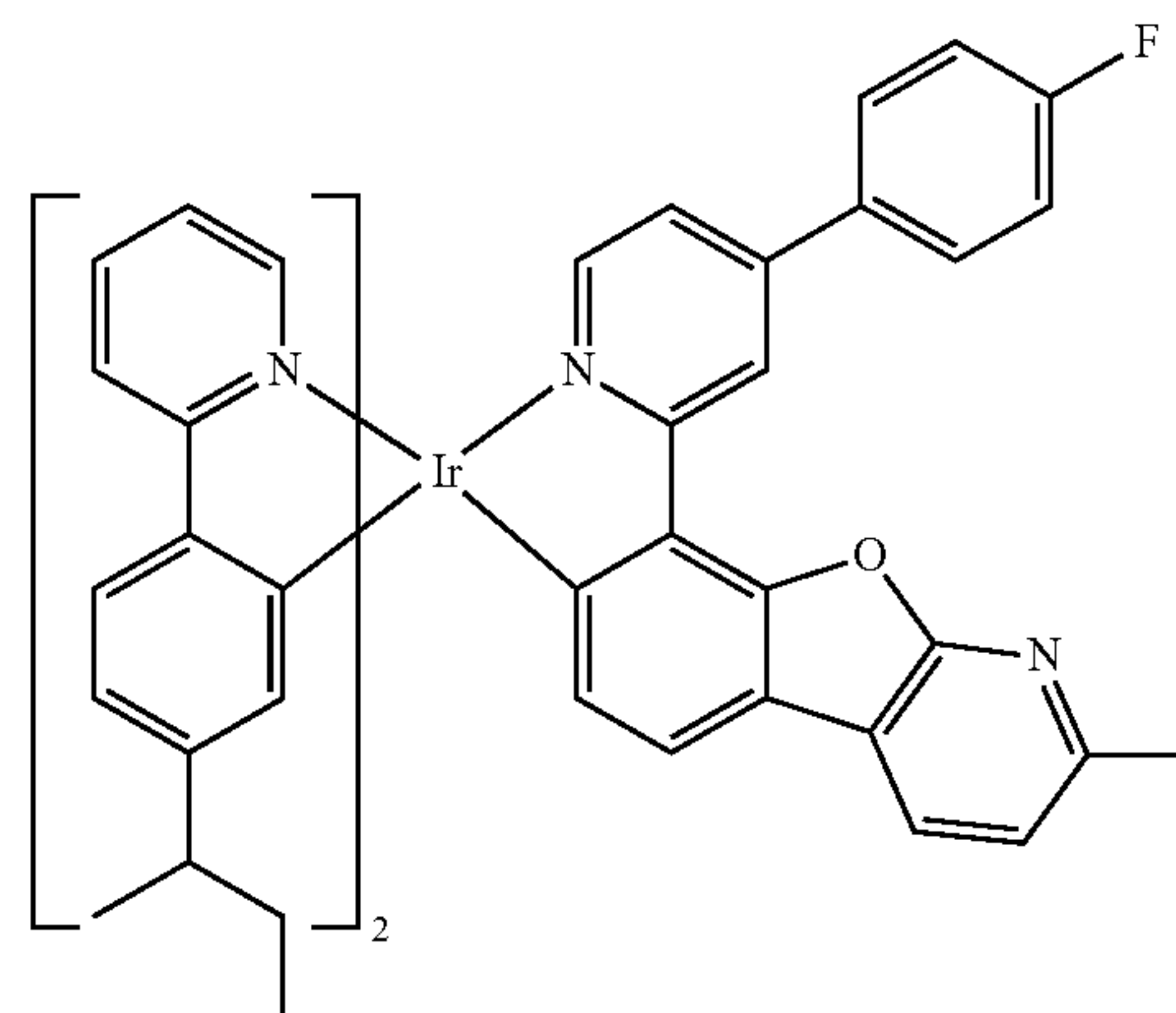
Compound I-13
