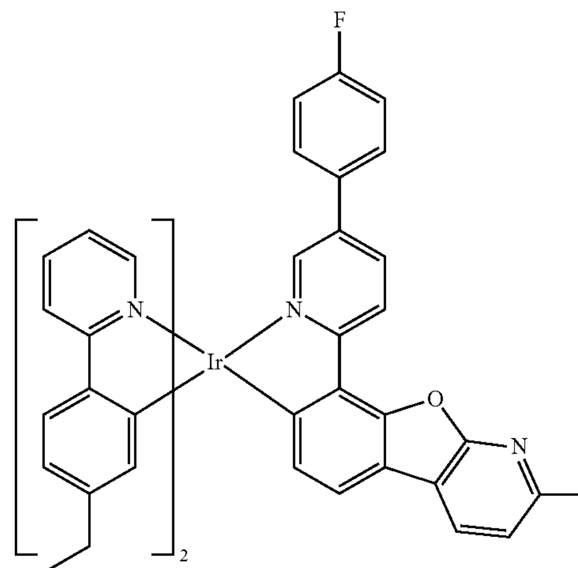
Compound I-4
