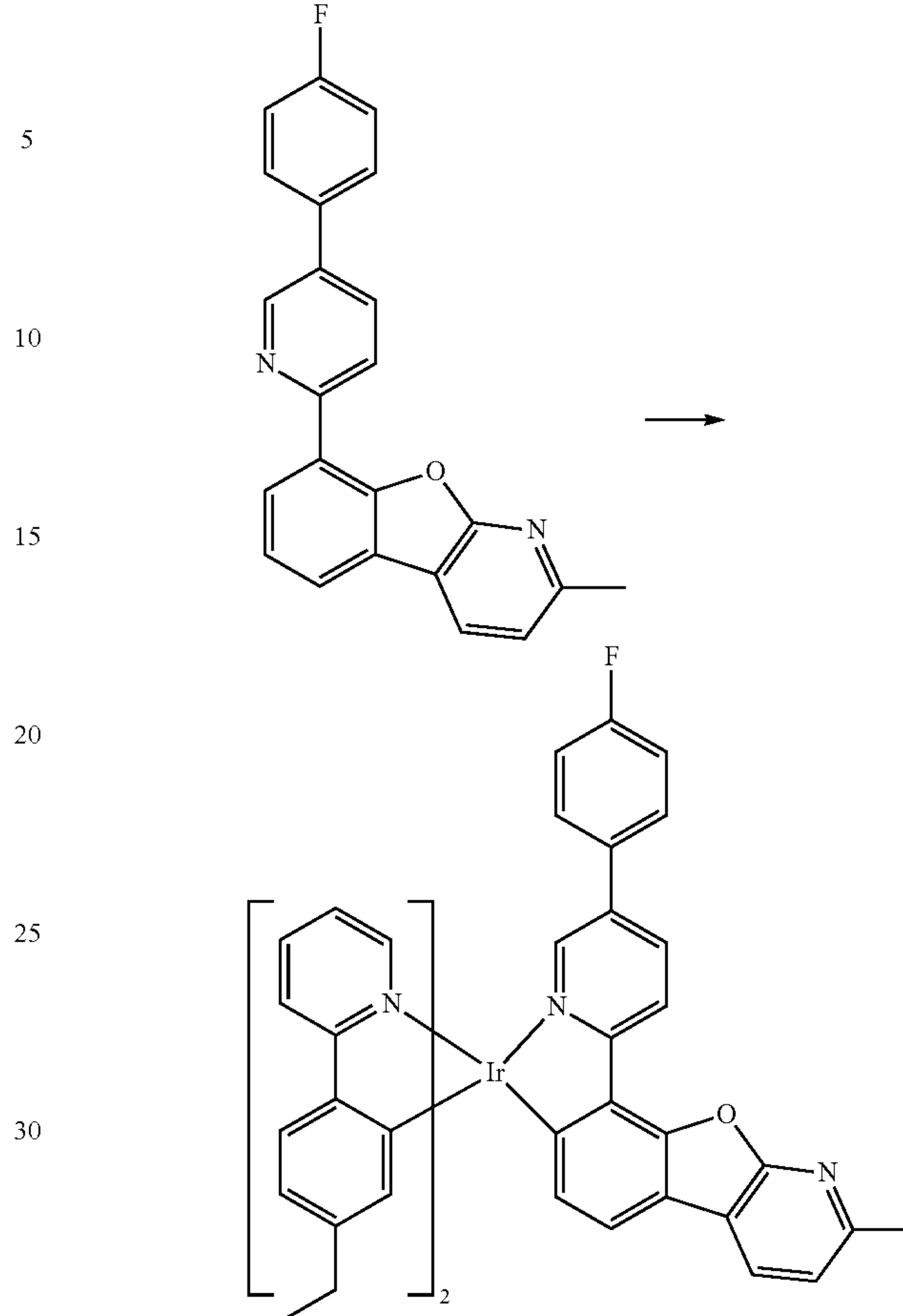
Compound I-3
