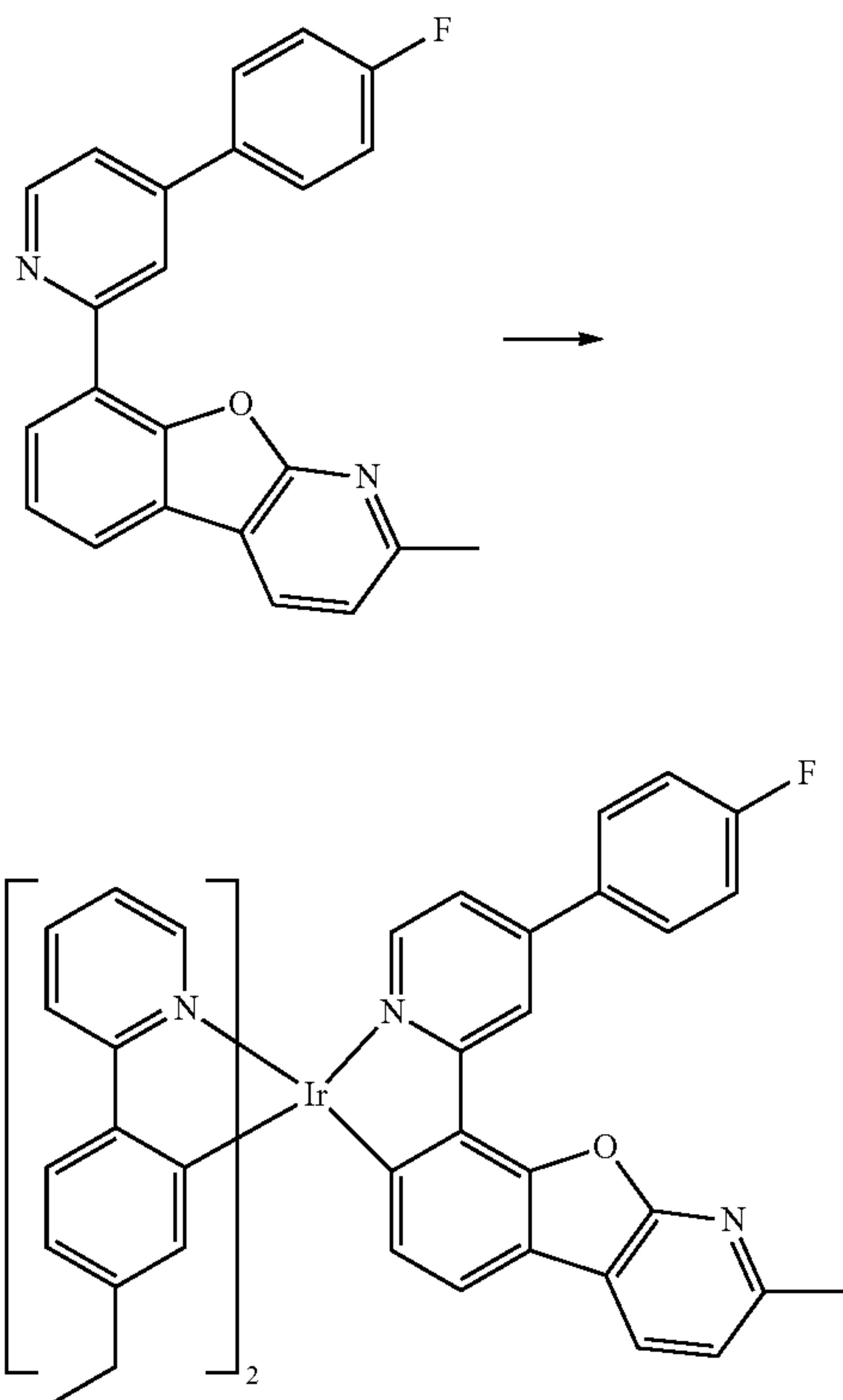
Compound I-2
