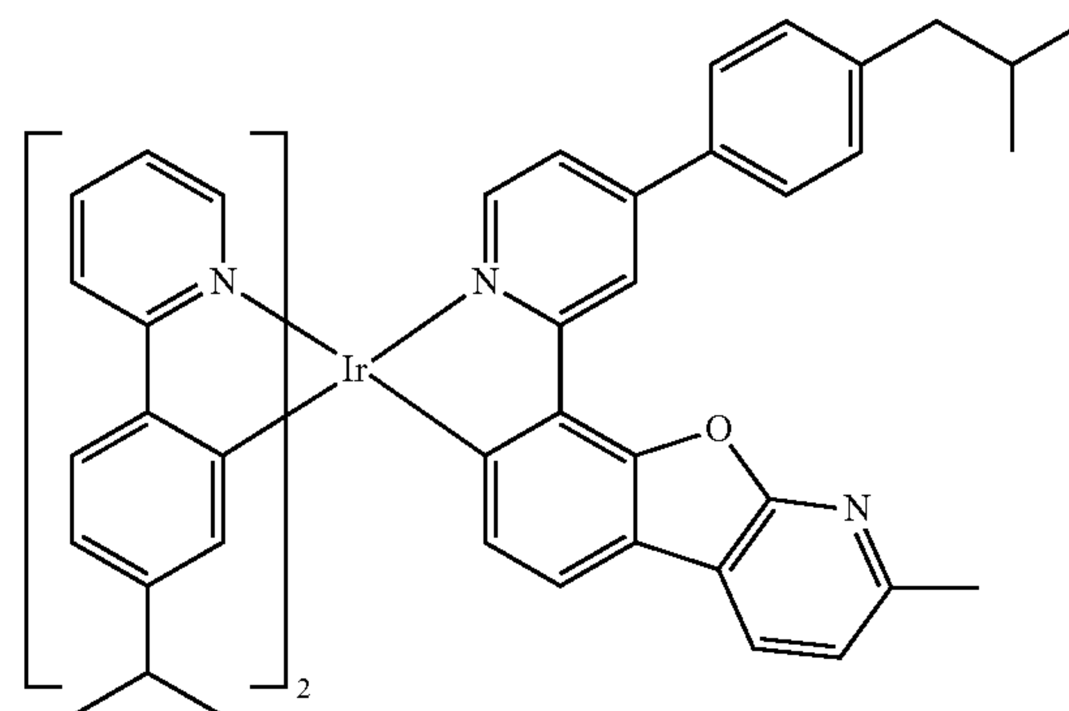
Compound I-6
