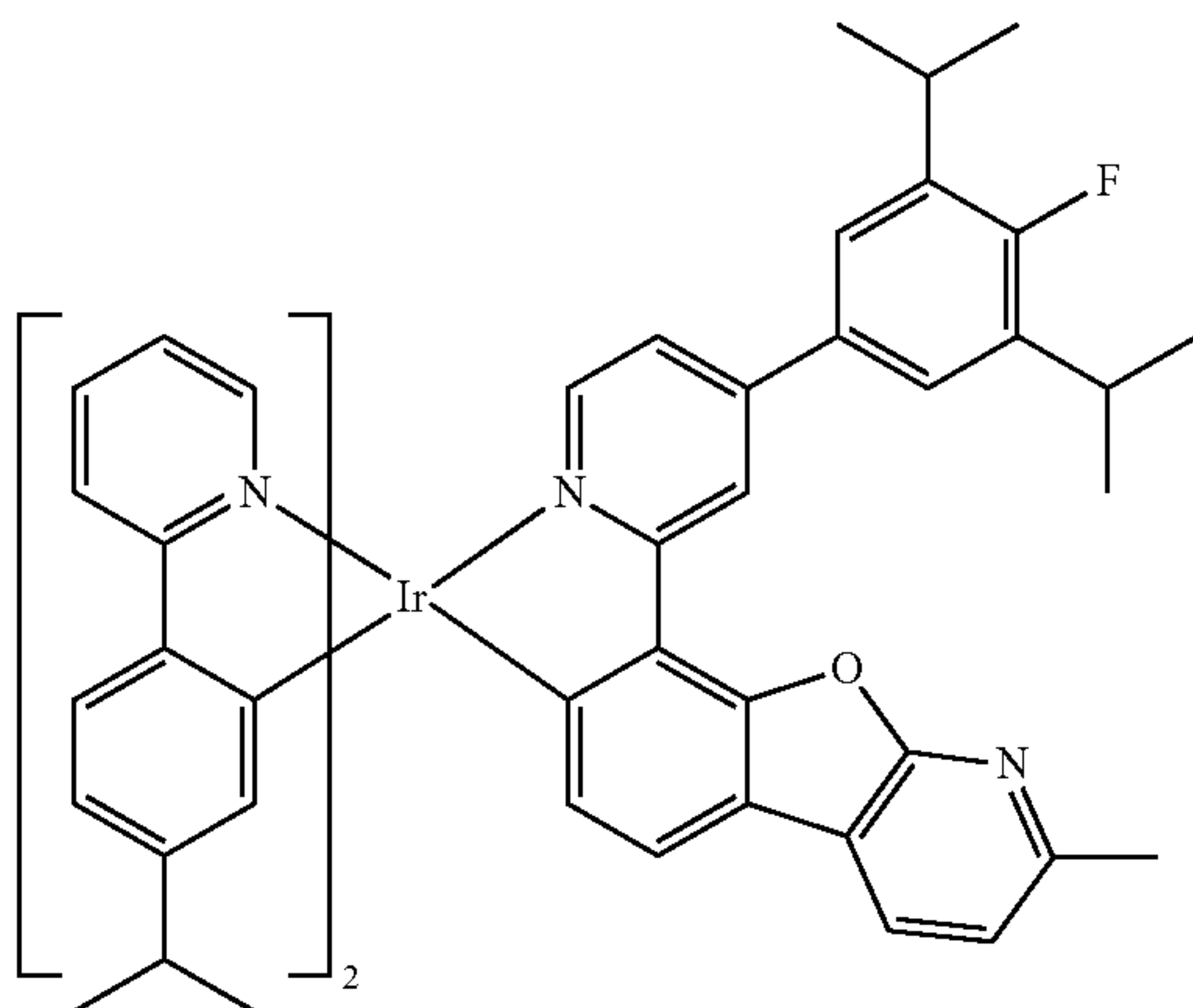
Compound I-8
