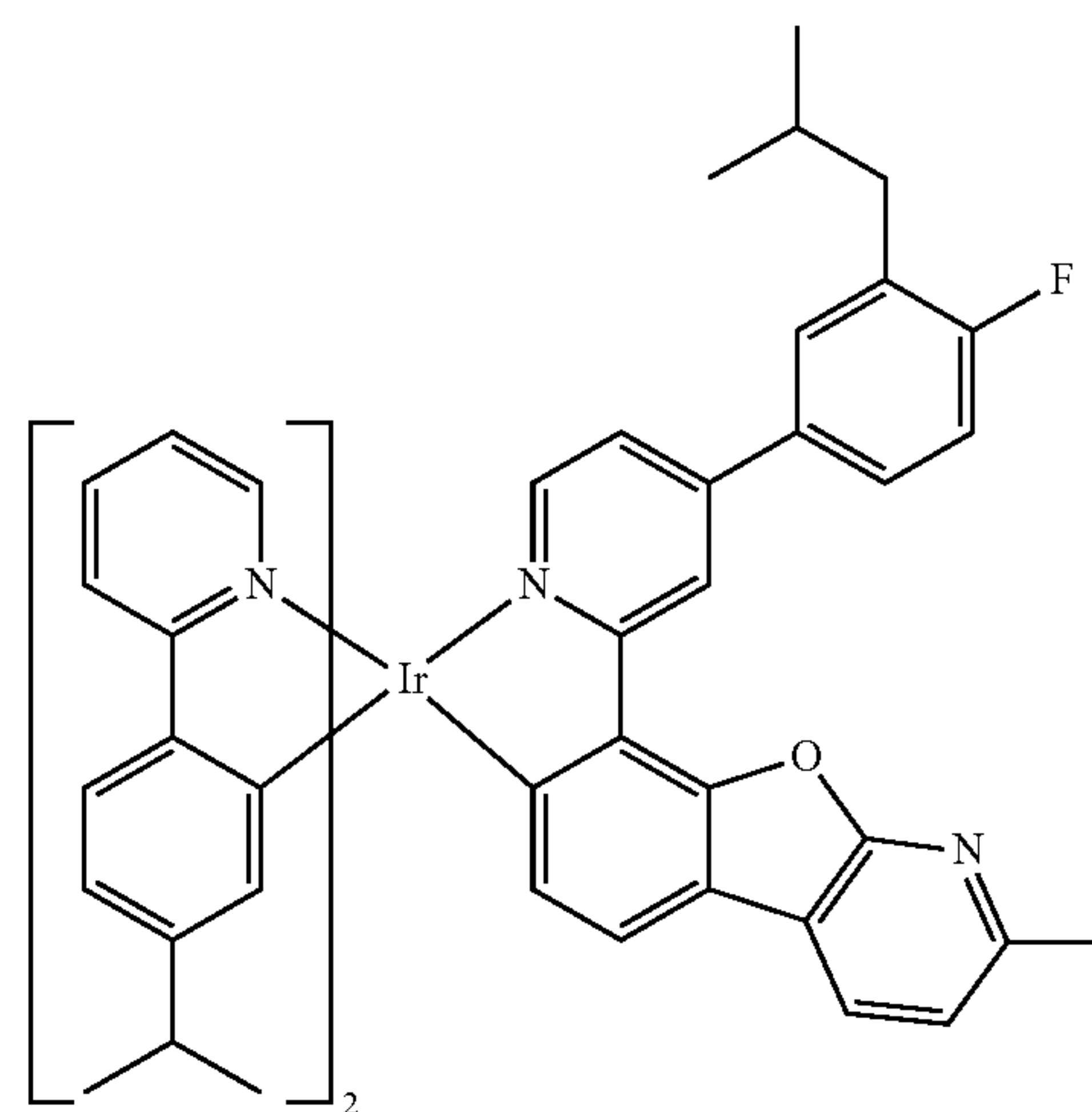
Compound I-7
