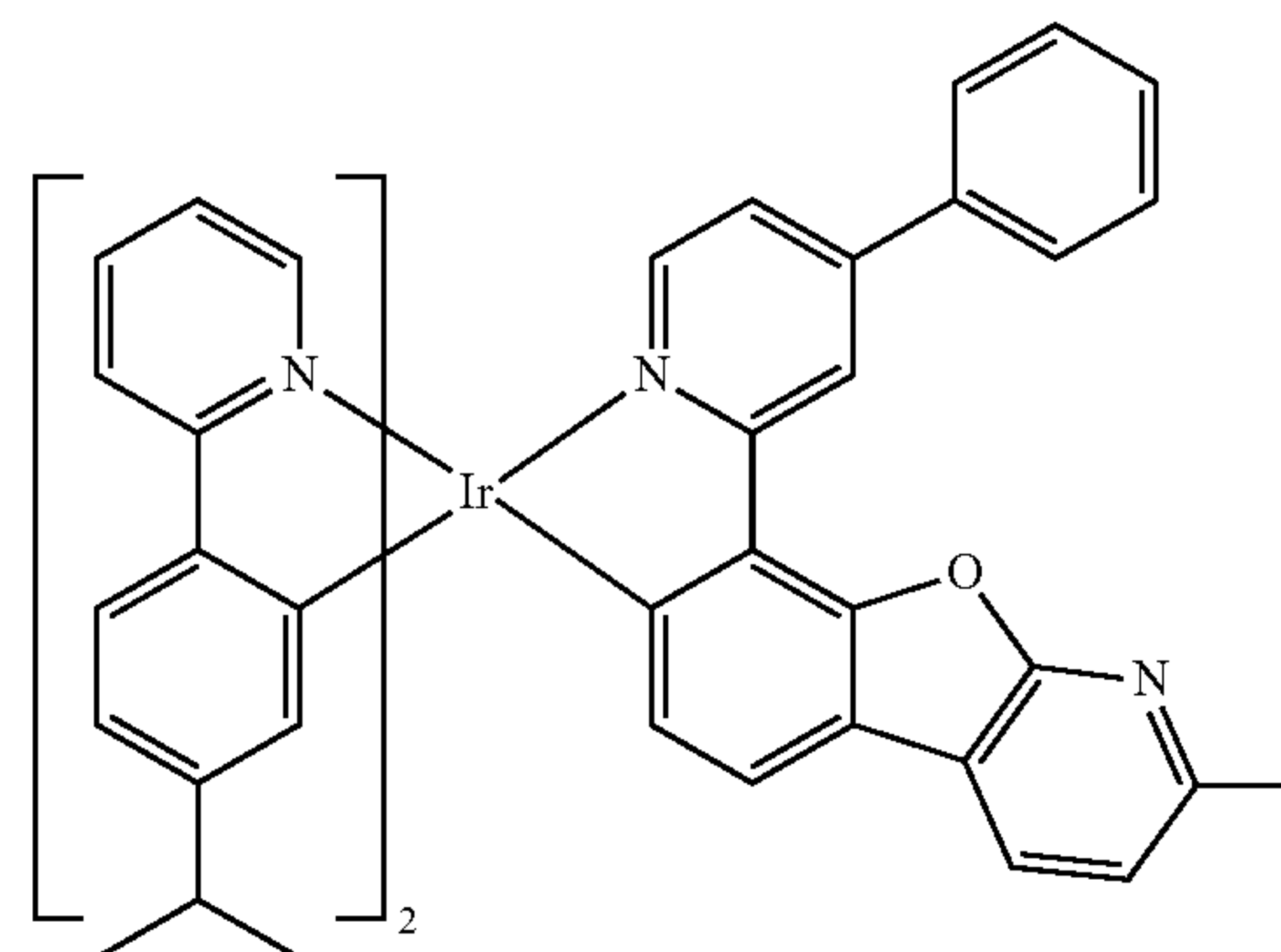
Compound I-6
