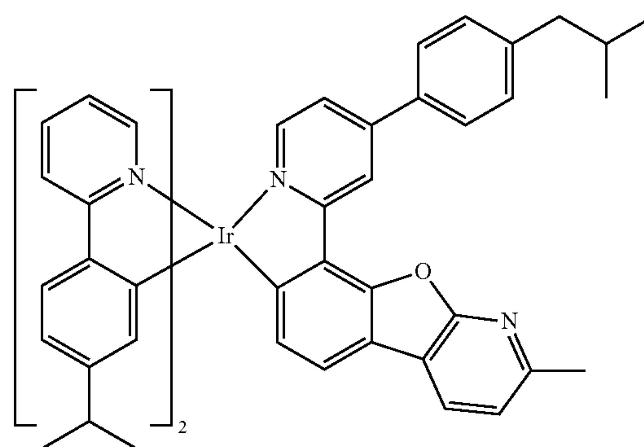
Compound I-5
