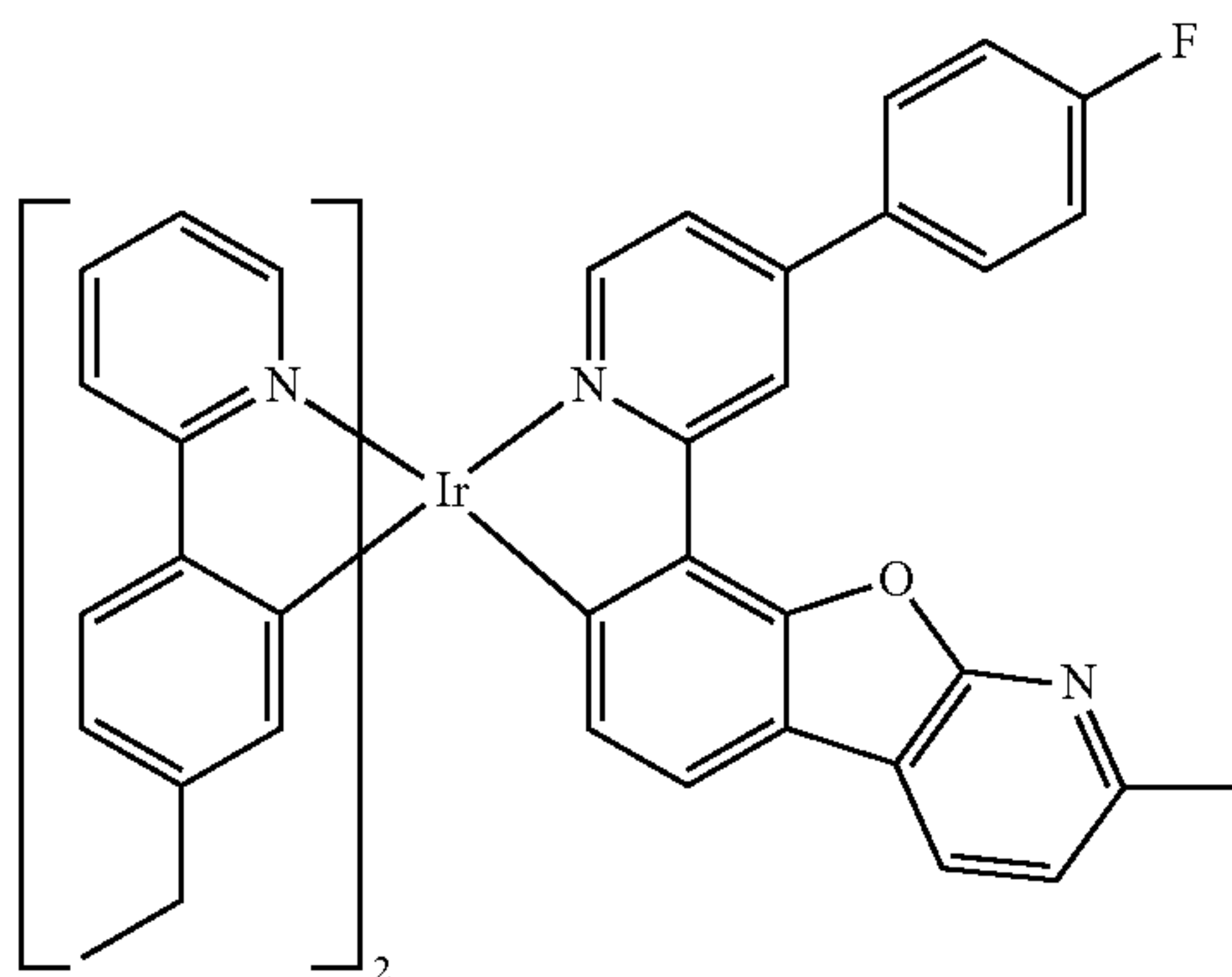
Compound I-3
