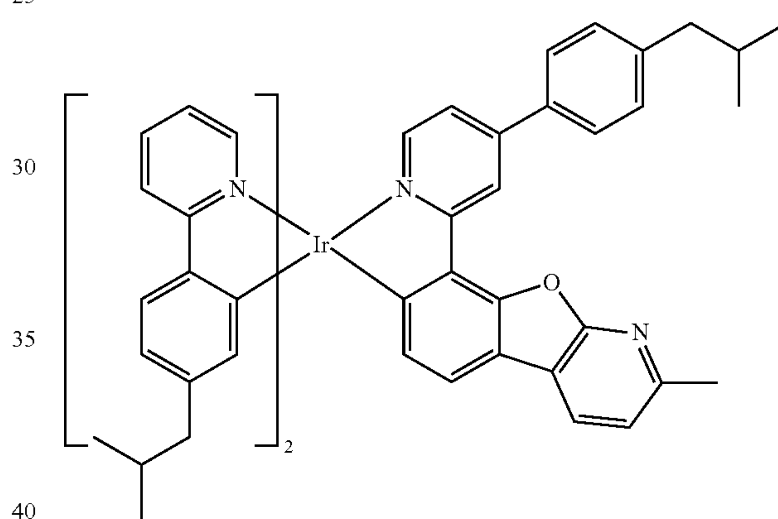
Compound I-11
