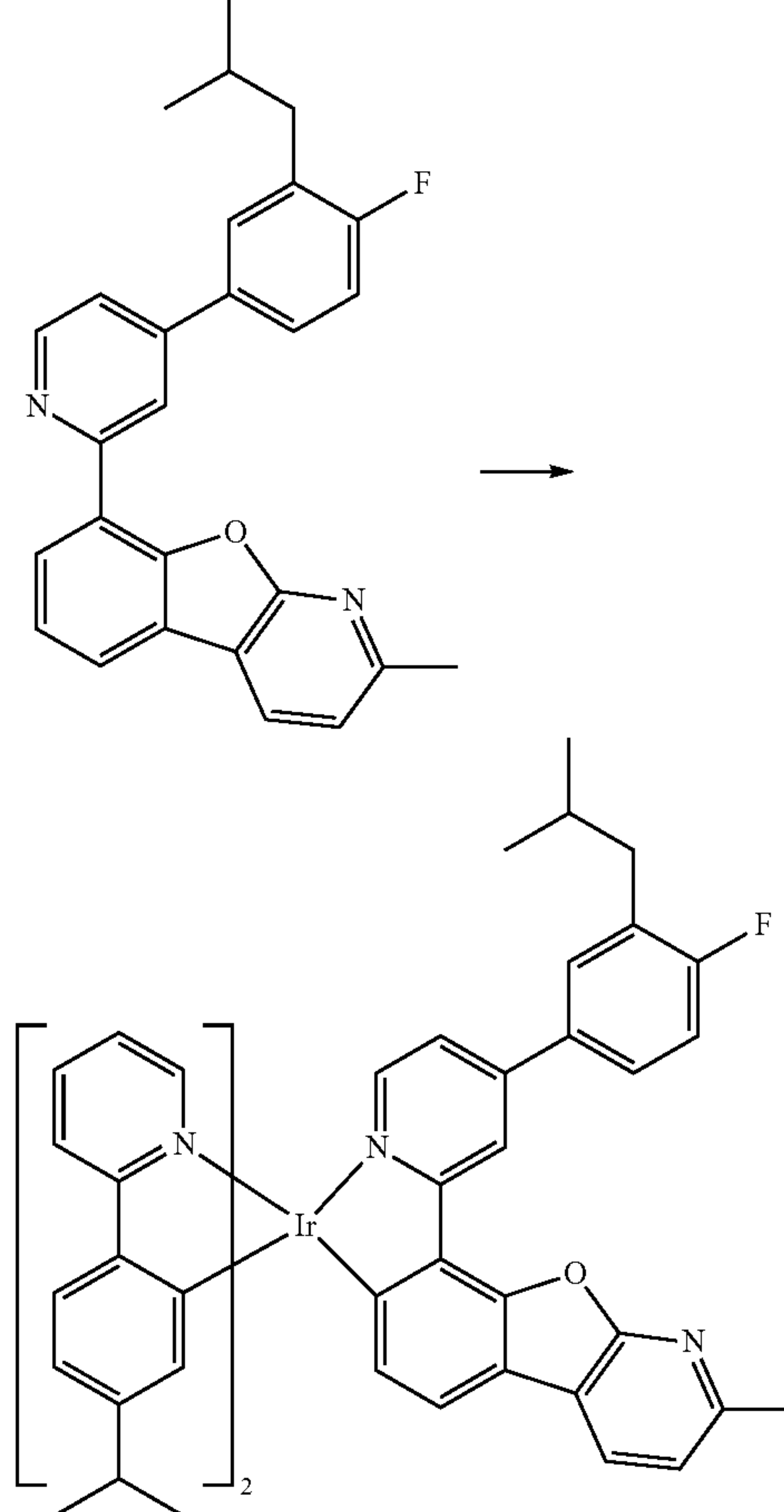
Compound I-7
