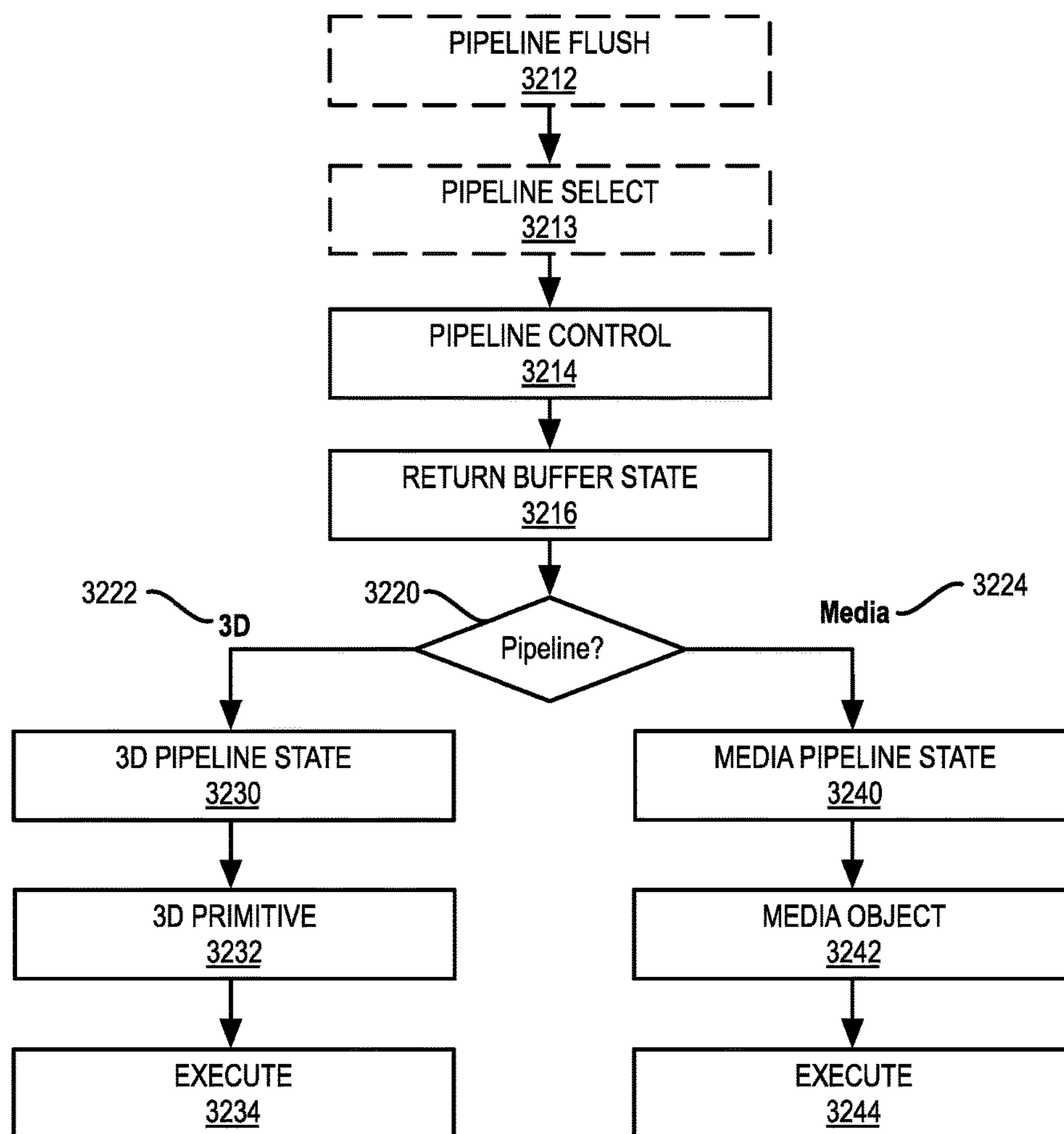
FIG. 32B GRAPHICS PROCESSOR COMMAND SEQUENCE 3210
