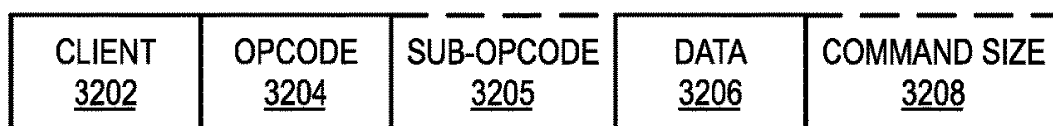
FIG. 32A GRAPHICS PROCESSOR COMMAND FORMAT 3200
