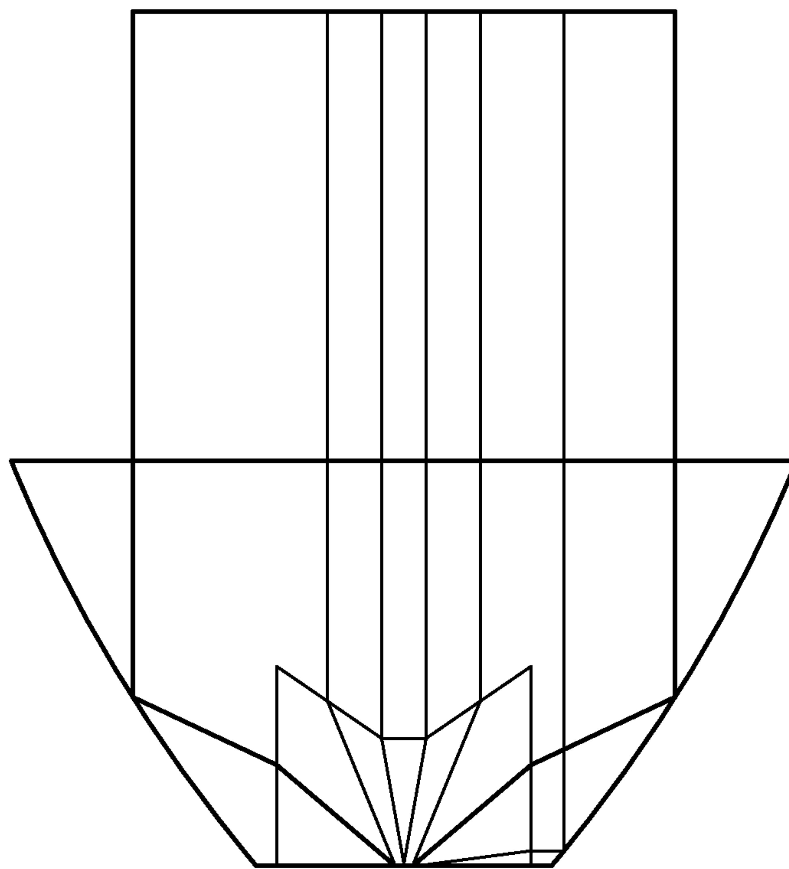
FIG. 18 (PRIOR ART)
